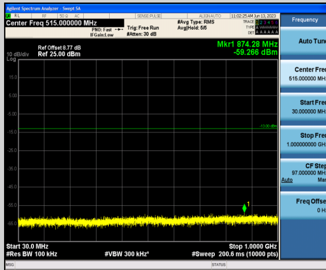
Band4-15MHz-16QAM-20025-1-0-Low-30-1000--59.27-PASS
