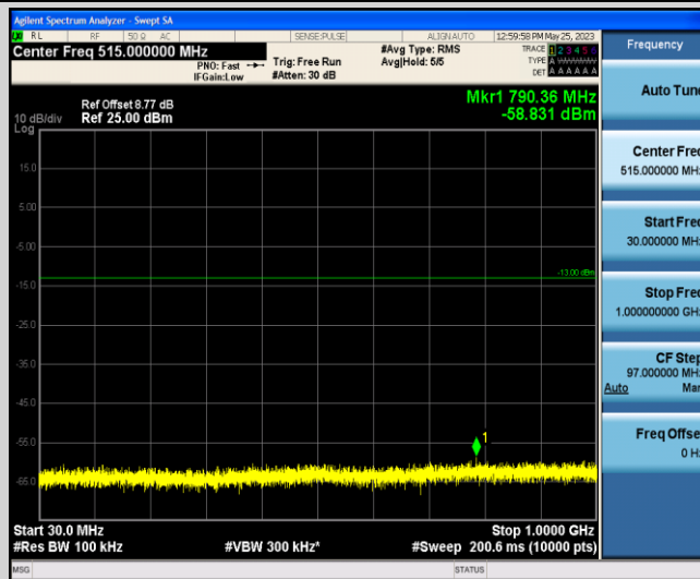
Band4-10MHz-16QAM-20000-1-0-Low-30-1000--58.83-PASS
