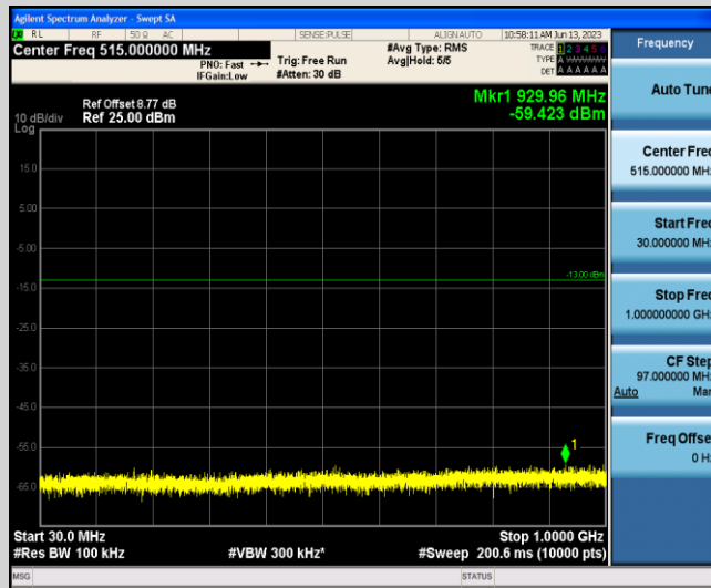
Band4-5MHz-16QAM-19975-1-0-Low-30-1000--59.42-PASS
