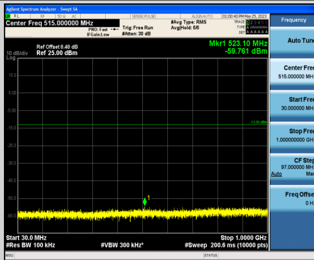
Band4-10MHz-16QAM-20175-1-0-Low-30-1000--59.76-PASS
