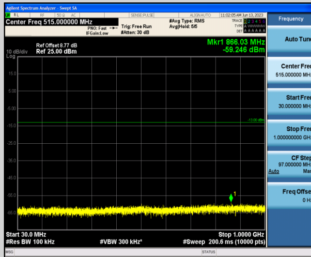
Band4-15MHz-QPSK-20025-1-0-Low-30-1000--59.25-PASS
