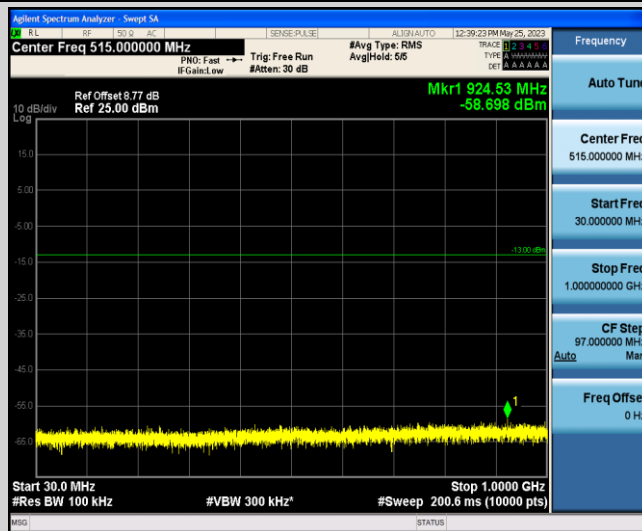
Band4-3MHz-16QAM-19965-1-0-Low-30-1000--58.7-PASS
