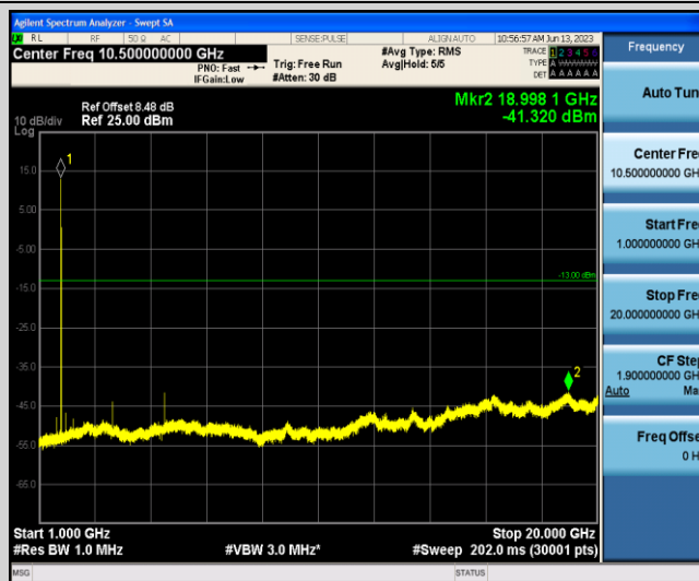
Band4-3MHz-16QAM-20385-1-0-Low-1000-20000--41.32-PASS
