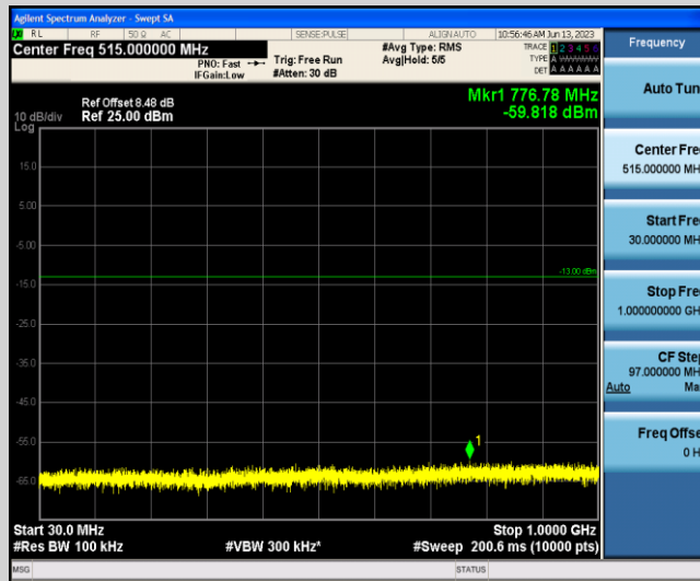
Band4-3MHz-16QAM-20385-1-0-Low-30-1000--59.82-PASS
