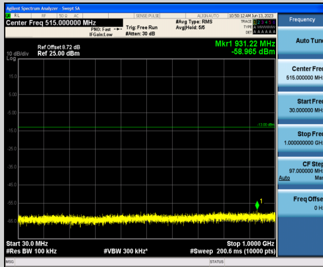
Band2-20MHz-16QAM-18700-1-0-Low-30-1000--58.97-PASS
