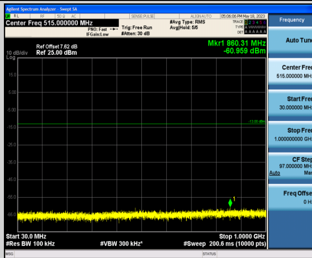
Band2-10MHz-QPSK-18650-1-0-Low-30-1000--60.96-PASS
