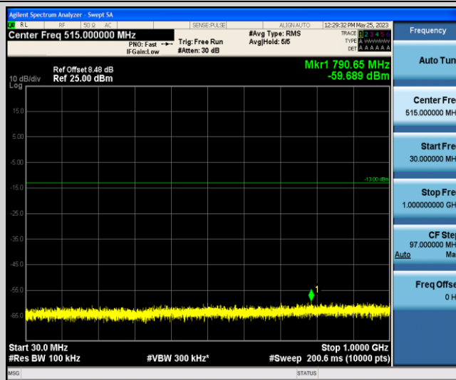
Band4-1.4MHz-16QAM-20175-1-0-Low-30-1000--59.69-PASS
