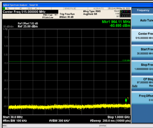
Band2-15MHz-16QAM-18900-1-0-Low-30-1000--60.7-PASS
