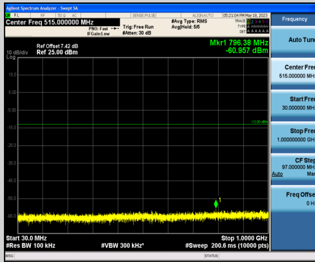
Band2-20MHz-QPSK-19100-1-0-High-30-1000--60.96-PASS
