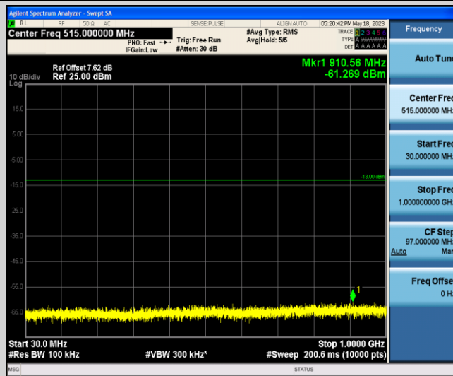
Band2-20MHz-16QAM-18900-1-0-Low-30-1000--61.27-PASS
