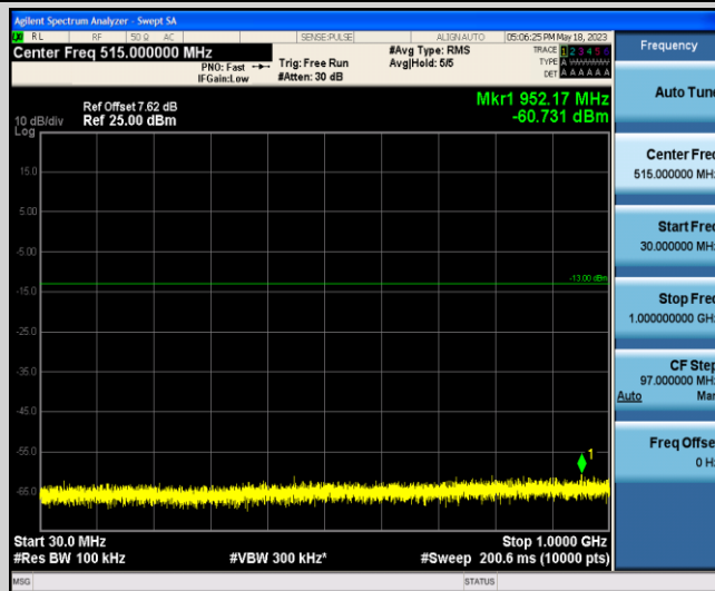
Band2-10MHz-16QAM-18650-1-0-Low-30-1000--60.73-PASS
