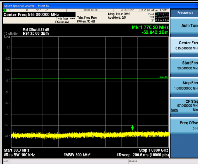
Band2-5MHz-16QAM-18625-1-0-Low-30-1000--59.84-PASS
