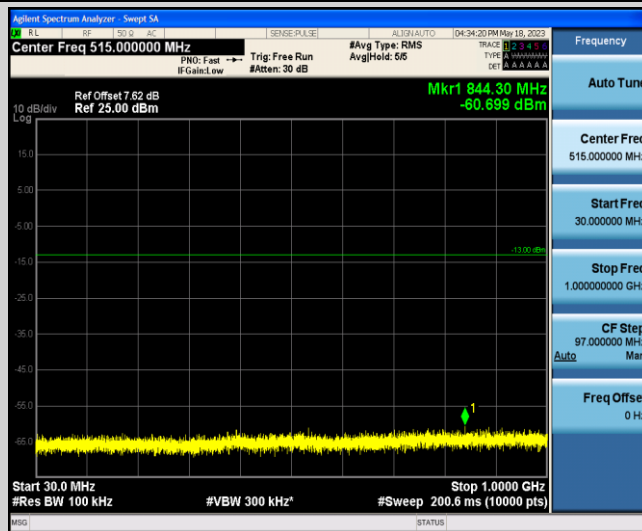
Band2-3MHz-16QAM-18615-1-0-Low-30-1000--60.7-PASS
