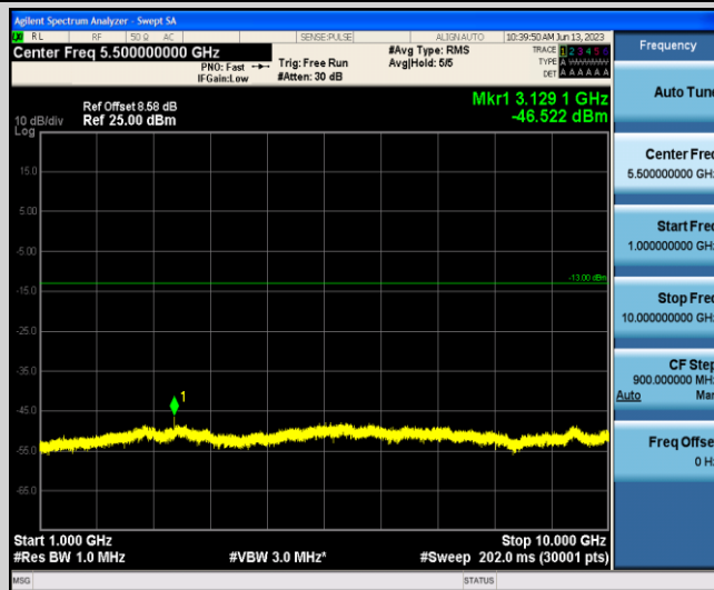
Band13-5MHz-16QAM-23255-1-0-Low-1000-10000--46.52-PASS
