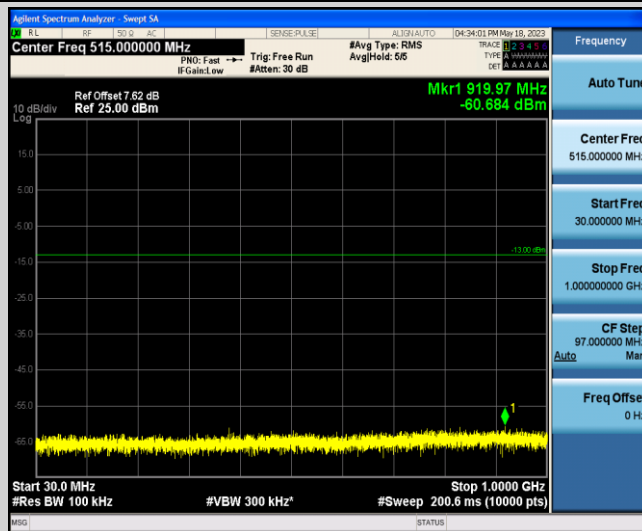
Band2-3MHz-QPSK-18615-1-0-Low-30-1000--60.68-PASS
