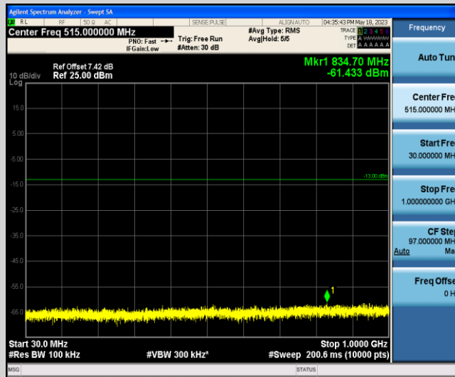
Band2-3MHz-16QAM-19185-1-0-Low-30-1000--61.43-PASS
