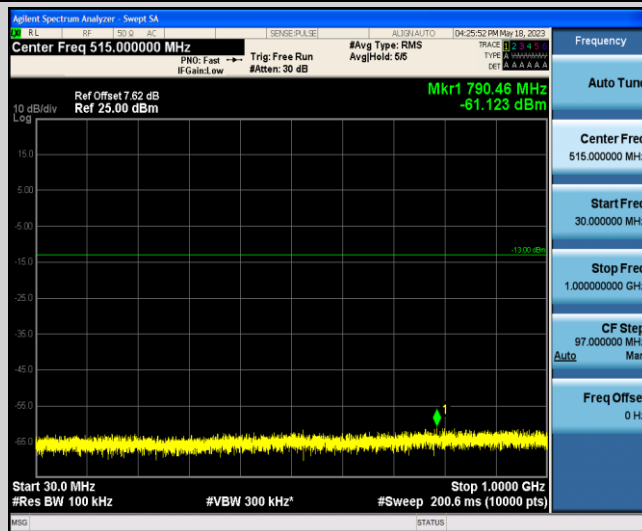
Band2-1.4MHz-16QAM-18607-1-0-Low-30-1000--61.12-PASS
