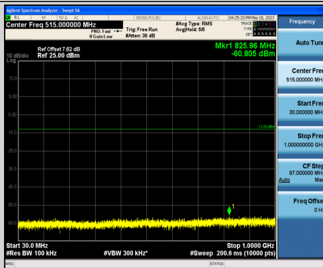
Band2-1.4MHz-QPSK-18607-1-0-Low-30-1000--60.81-PASS
