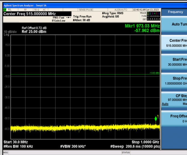
Band2-5MHz-QPSK-18625-1-0-Low-30-1000--57.96-PASS
