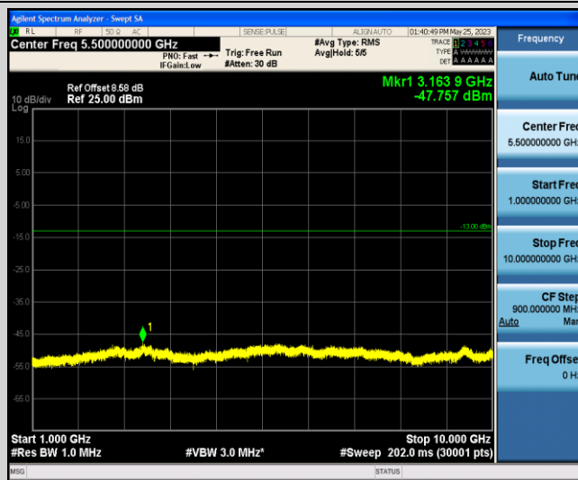
Band13-10MHz-16QAM-23230-1-0-Low-1000-10000--47.76-PASS
