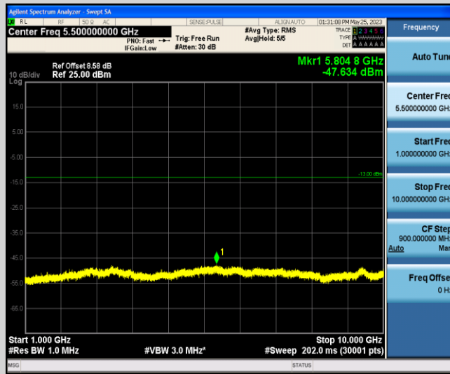
Band13-5MHz-16QAM-23205-1-0-Low-1000-10000--47.63-PASS
