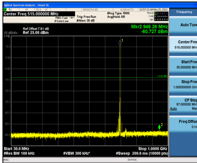
Band12-10MHz-QPSK-23095-1-0-Low-30-1000--60.73-PASS
