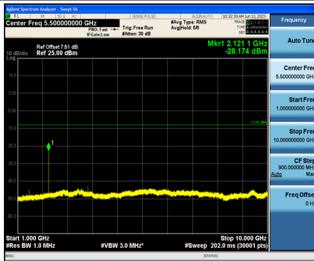
Band12-1.4MHz-16QAM-23095-1-0-Low-1000-10000--28.17-PASS
