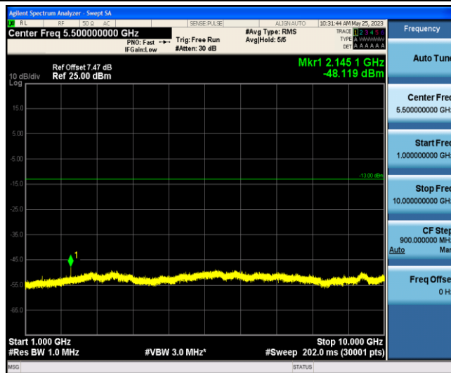
Band12-1.4MHz-16QAM-23173-1-0-Low-1000-10000--48.12-PASS
