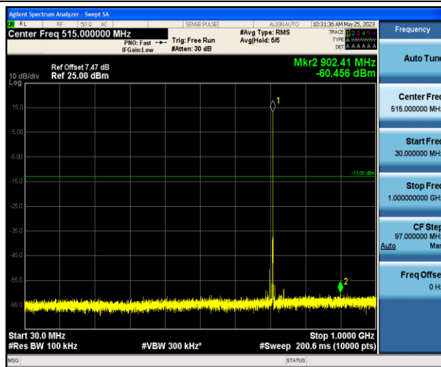
Band12-1.4MHz-16QAM-23173-1-0-Low-30-1000--60.46-PASS
