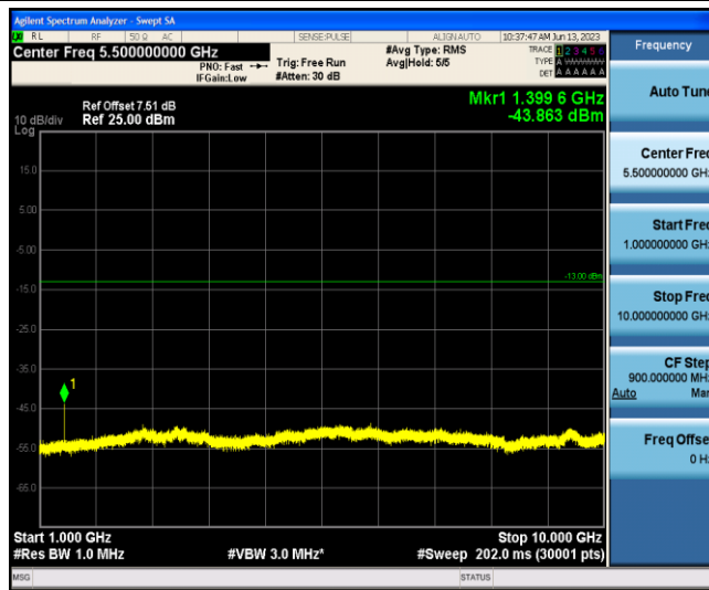
Band12-10MHz-QPSK-23060-1-0-Low-1000-10000--43.86-PASS
