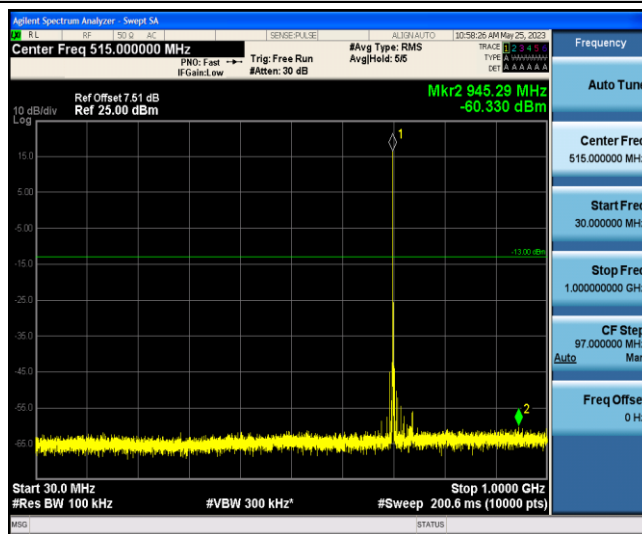
Band12-10MHz-16QAM-23130-1-0-Low-30-1000--60.33-PASS
