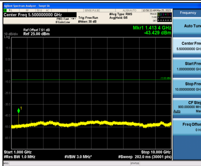
Band12-10MHz-16QAM-23130-1-0-Low-1000-10000--43.43-PASS
