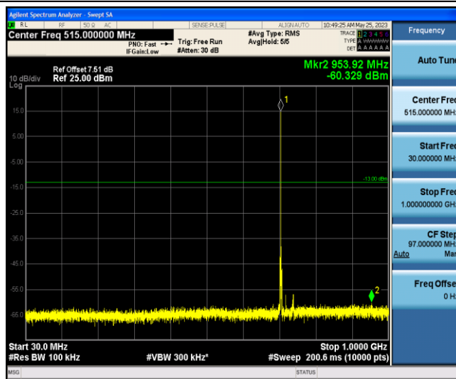
Band12-5MHz-16QAM-23155-1-0-Low-30-1000--60.33-PASS
