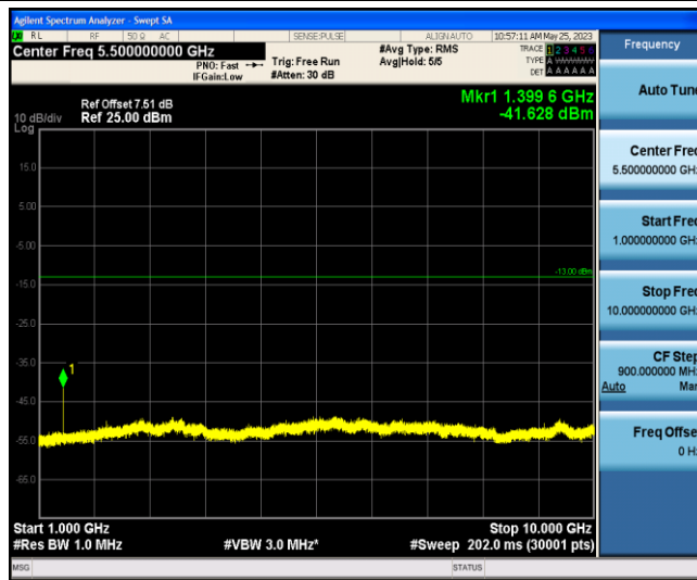
Band12-10MHz-16QAM-23060-1-0-Low-1000-10000--41.63-PASS
