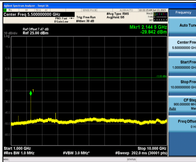
Band12-1.4MHz-QPSK-23173-1-0-Low-1000-10000--29.84-PASS
