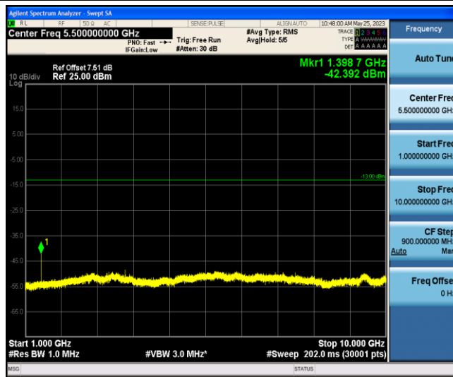
Band12-5MHz-QPSK-23035-1-0-Low-1000-10000--42.39-PASS
