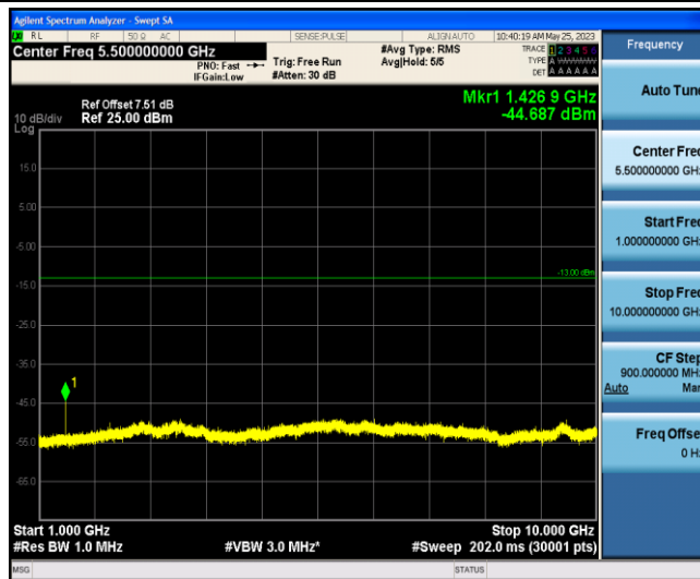
Band12-3MHz-QPSK-23165-1-0-Low-1000-10000--44.69-PASS
