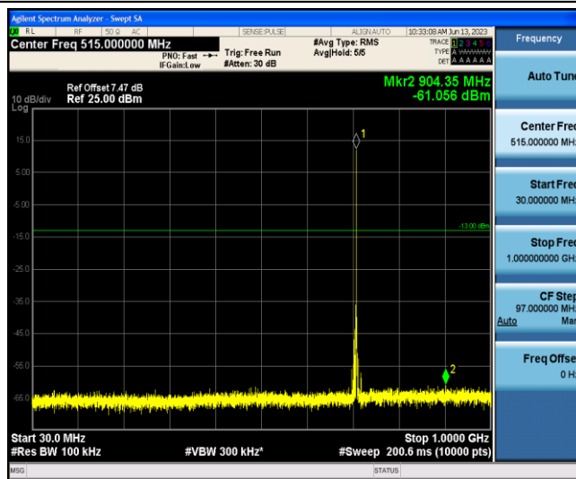
Band12-1.4MHz-QPSK-23173-1-0-Low-30-1000--61.06-PASS
