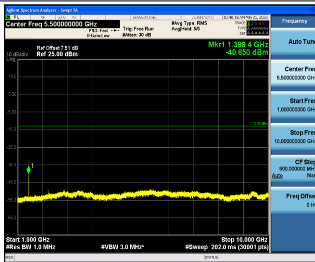
Band12-5MHz-16QAM-23035-1-0-Low-1000-10000--40.65-PASS
