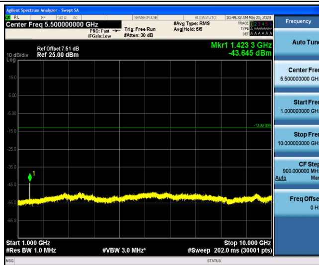
Band12-5MHz-16QAM-23155-1-0-Low-1000-10000--43.65-PASS
