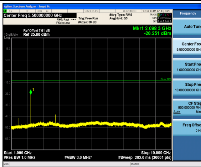
Band12-3MHz-QPSK-23025-1-0-Low-1000-10000--26.25-PASS
