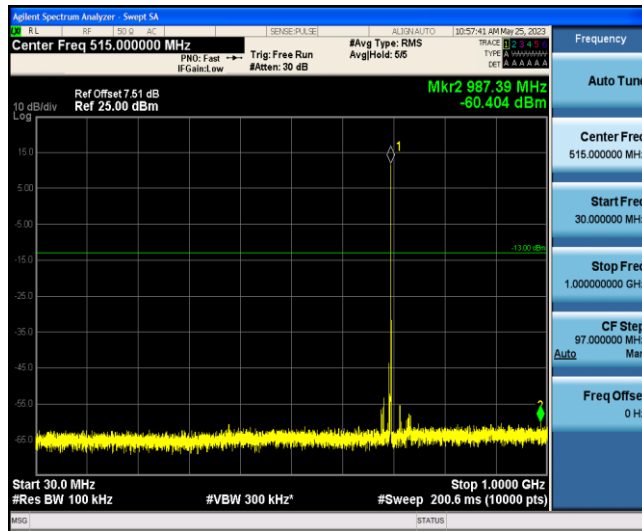
Band12-10MHz-16QAM-23095-1-0-Low-30-1000--60.4-PASS
