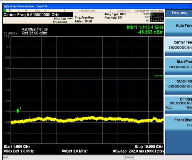
Band12-10MHz-QPSK-23130-1-0-Low-1000-10000--46.86-PASS
