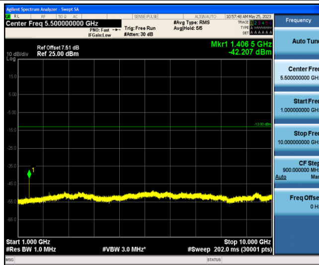
Band12-10MHz-16QAM-23095-1-0-Low-1000-10000--42.21-PASS
