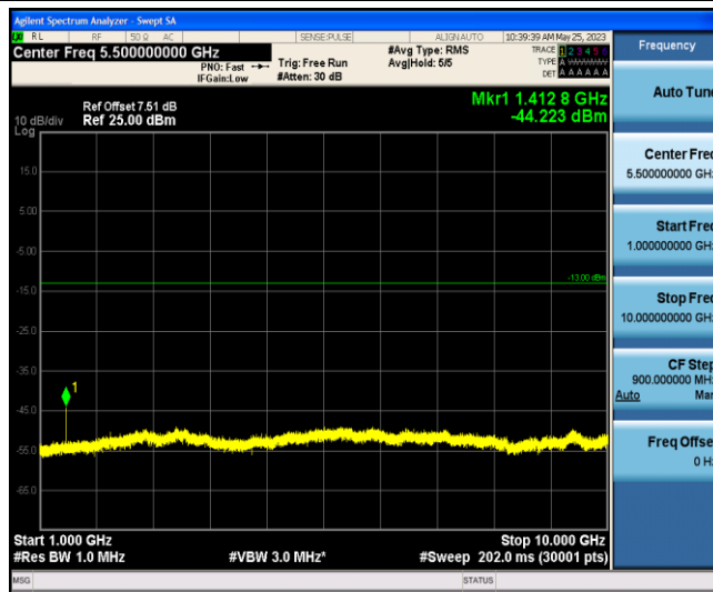
Band12-3MHz-QPSK-23095-1-0-Low-1000-10000--44.22-PASS
