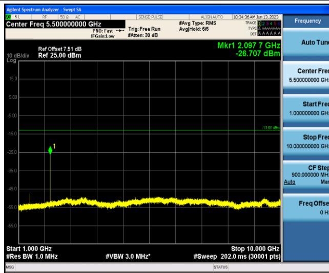
Band12-3MHz-16QAM-23025-1-0-Low-1000-10000--26.71-PASS
