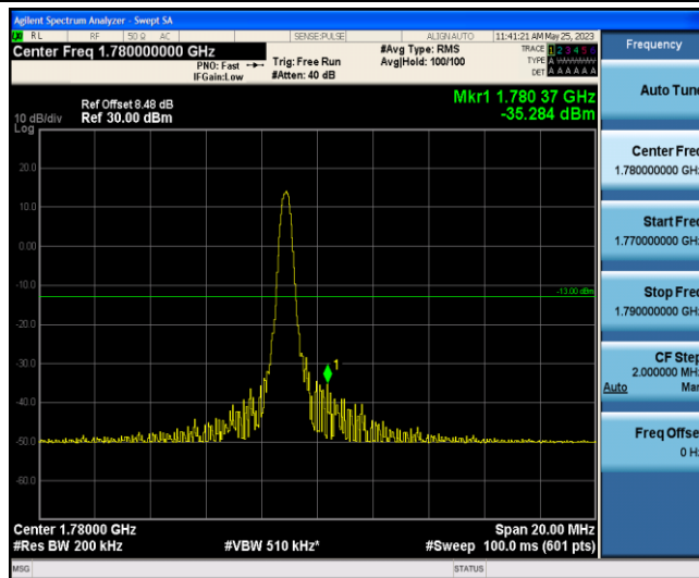
Band66-10MHz-QPSK-132622-1-5-High--35.28-PASS
