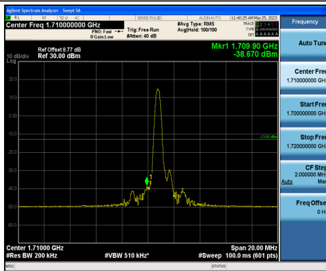
Band66-10MHz-16QAM-132022-1-0-Low--38.67-PASS
