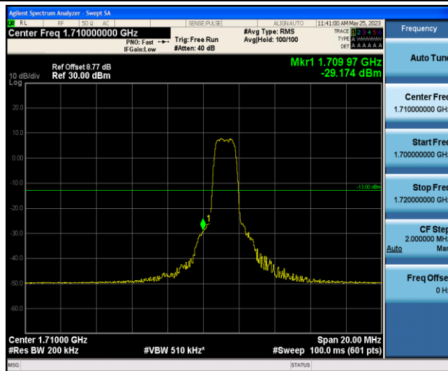
Band66-10MHz-16QAM-132022-6-0-Low--29.17-PASS
