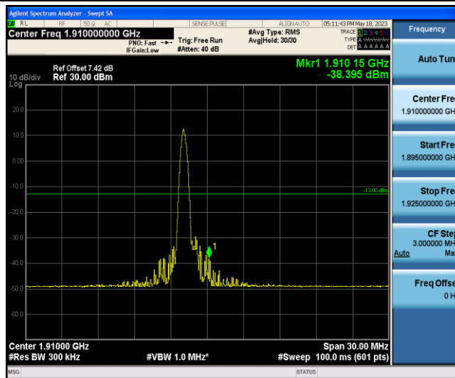
Band2-15MHz-16QAM-19125-1-0-High--38.40-PASS
