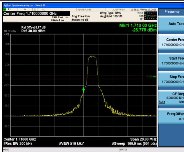
Band4-10MHz-16QAM-20000-6-0-Low--26.78-PASS
