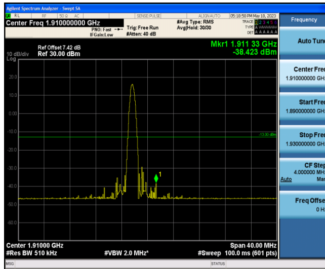
Band2-20MHz-QPSK-19100-1-0-High--38.42-PASS
