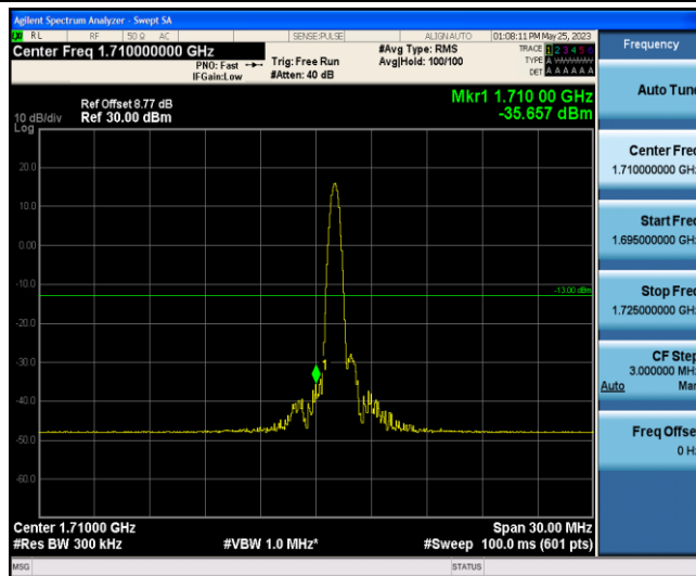
Band4-15MHz-QPSK-20025-1-0-Low--35.66-PASS
