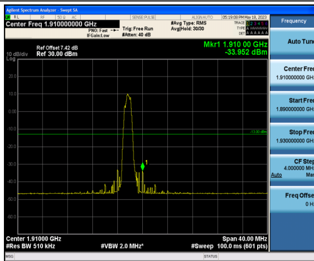
Band2-20MHz-16QAM-19100-1-0-High--33.95-PASS
