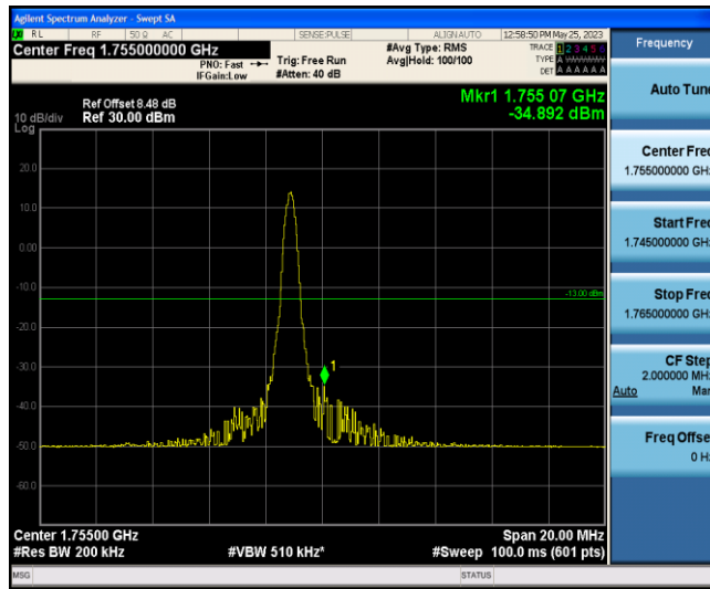
Band4-10MHz-16QAM-20350-1-5-High--34.89-PASS
