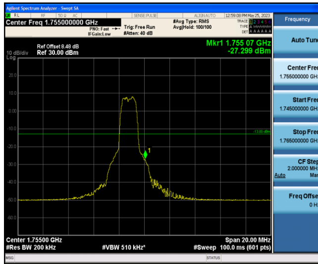
Band4-10MHz-QPSK-20350-6-0-High--27.30-PASS
