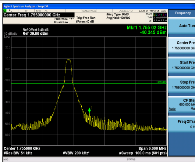
Band4-3MHz-16QAM-20385-1-5-High--40.35-PASS
