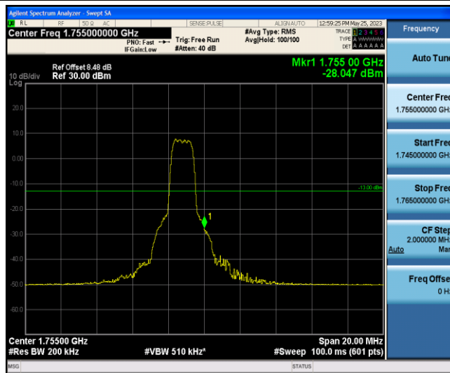
Band4-10MHz-16QAM-20350-6-0-High--28.05-PASS
