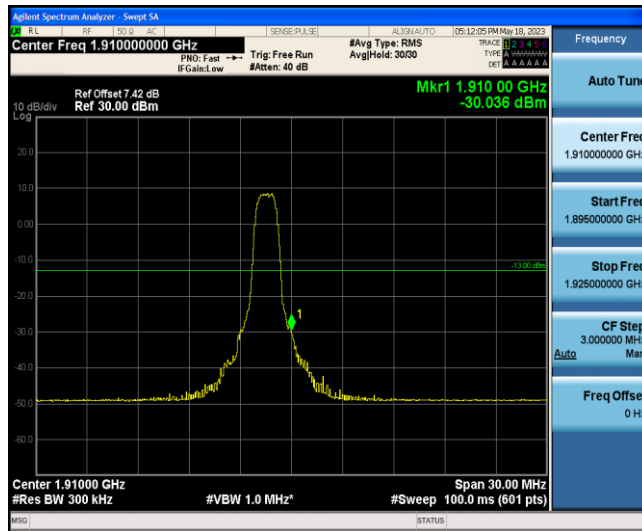
Band2-15MHz-16QAM-19125-6-0-High--30.04-PASS
