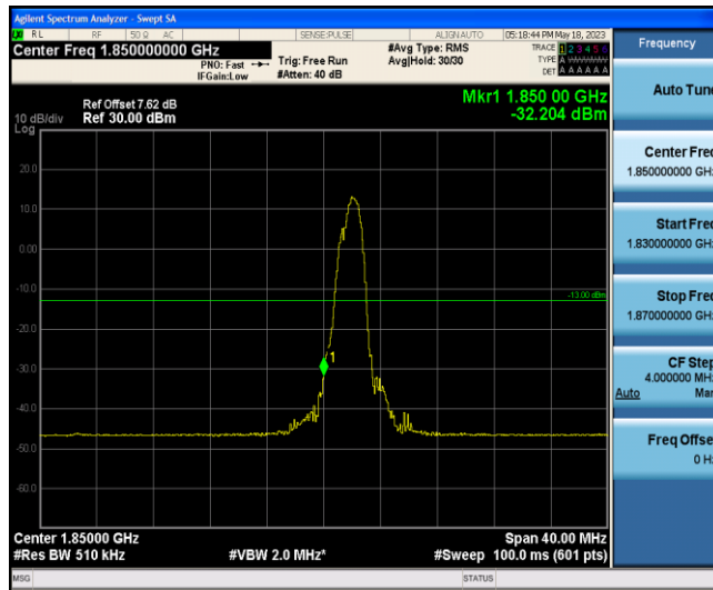
Band2-20MHz-16QAM-18700-6-0-Low--32.20-PASS
