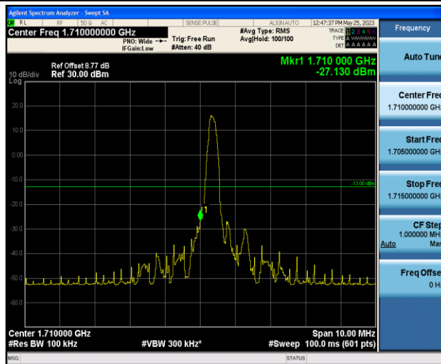
Band4-5MHz-16QAM-19975-1-0-Low--27.13-PASS
