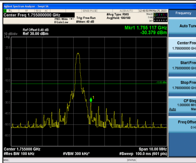
Band4-5MHz-16QAM-20375-1-5-High--30.38-PASS
