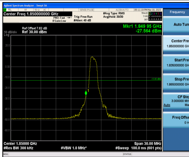
Band2-15MHz-16QAM-18675-6-0-Low--27.56-PASS
