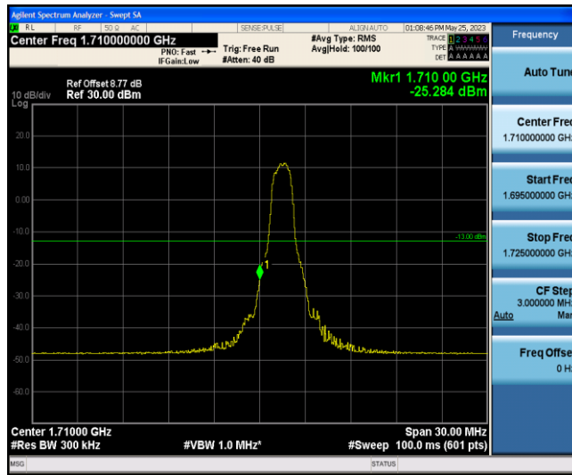
Band4-15MHz-QPSK-20025-6-0-Low--25.28-PASS
