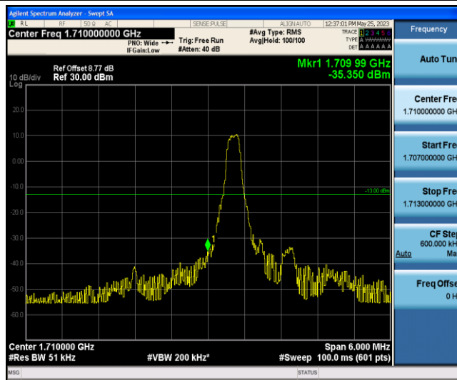
Band4-3MHz-16QAM-19965-1-0-Low--35.35-PASS
