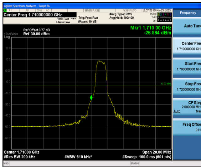
Band4-10MHz-QPSK-20000-6-0-Low--26.58-PASS
