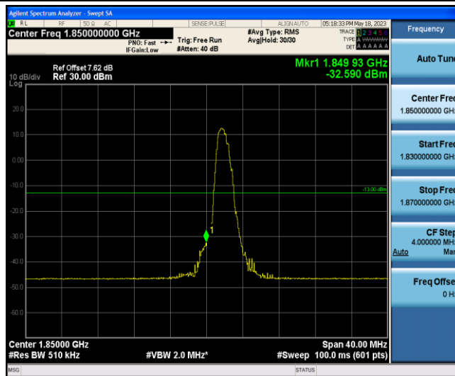
Band2-20MHz-QPSK-18700-6-0-Low--32.59-PASS
