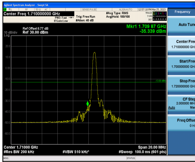
Band4-10MHz-QPSK-20000-1-0-Low--35.34-PASS
