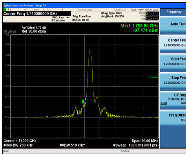
Band4-10MHz-16QAM-20000-1-0-Low--37.47-PASS
