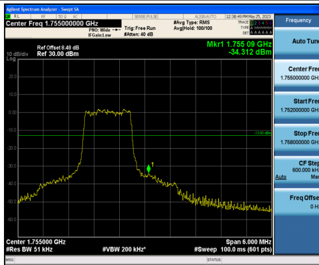
Band4-3MHz-16QAM-20385-6-0-High--34.31-PASS
