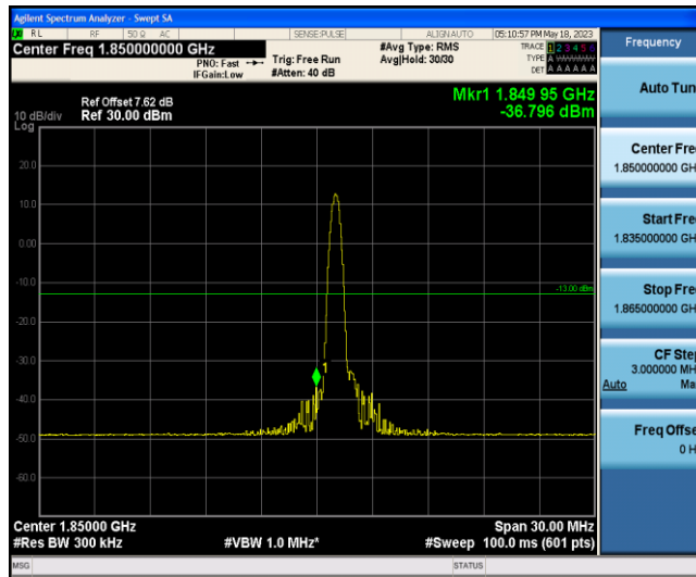
Band2-15MHz-16QAM-18675-1-0-Low--36.80-PASS
