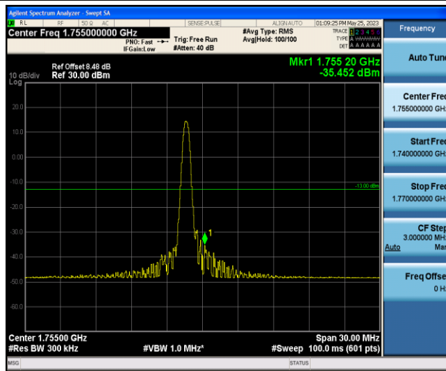
Band4-15MHz-QPSK-20325-1-5-High--35.45-PASS
