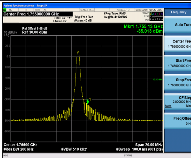
Band4-10MHz-QPSK-20350-1-5-High--35.01-PASS
