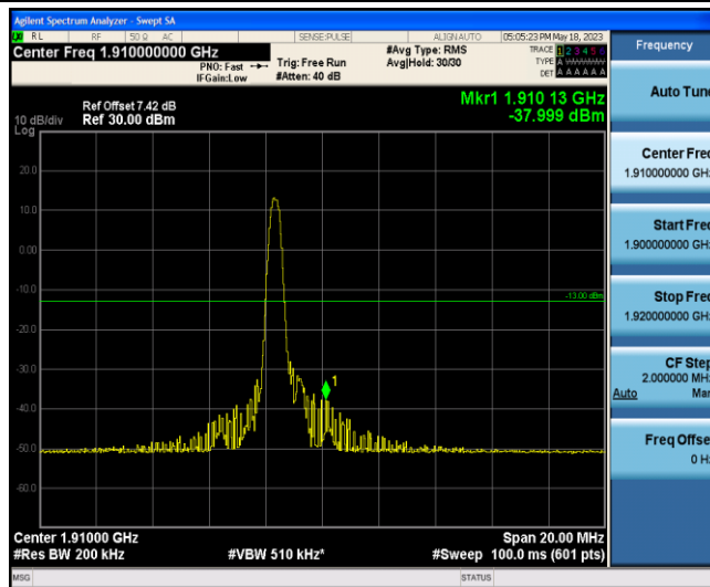
Band2-10MHz-QPSK-19150-1-0-High--38.00-PASS
