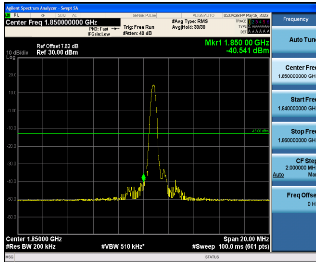
Band2-10MHz-QPSK-18650-1-0-Low--40.54-PASS
