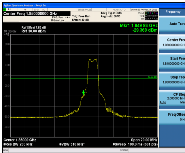
Band2-10MHz-QPSK-18650-6-0-Low--29.37-PASS
