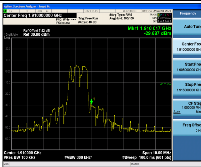
Band2-5MHz-QPSK-19175-6-0-High--29.69-PASS
