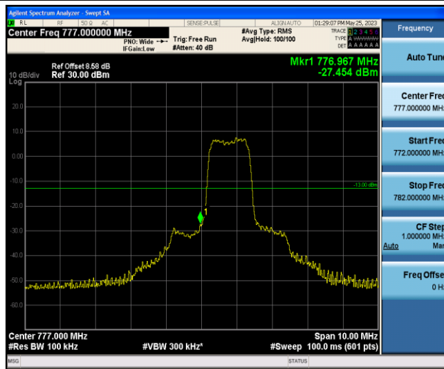
Band13-5MHz-16QAM-23205-6-0-Low--27.45-PASS
