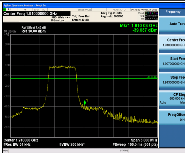
Band2-3MHz-QPSK-19185-6-0-High--39.04-PASS
