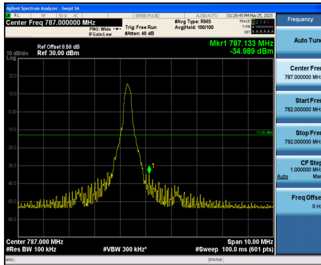
Band13-5MHz-16QAM-23255-1-5-High--34.99-PASS
