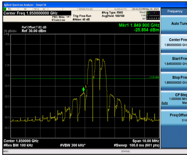
Band2-5MHz-16QAM-18625-6-0-Low--25.85-PASS
