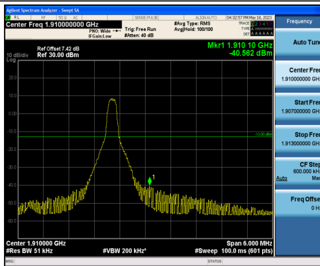
Band2-3MHz-QPSK-19185-1-5-High--40.56-PASS
