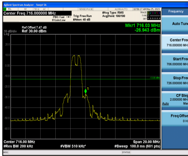
Band12-10MHz-QPSK-23130-6-0-High--26.94-PASS
