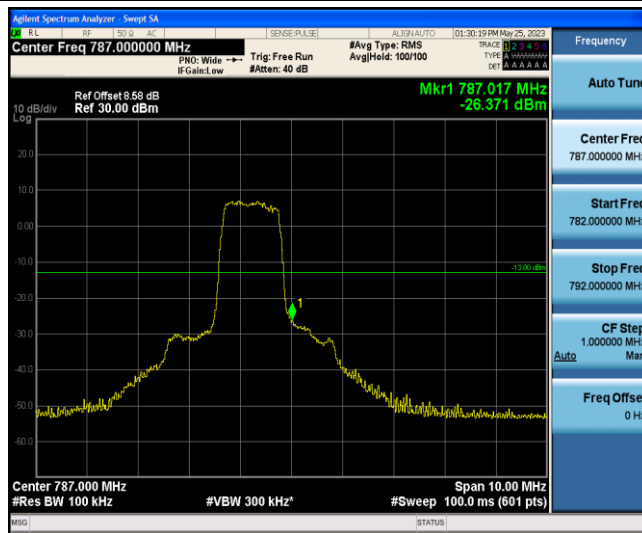
Band13-5MHz-16QAM-23255-6-0-High--26.37-PASS
