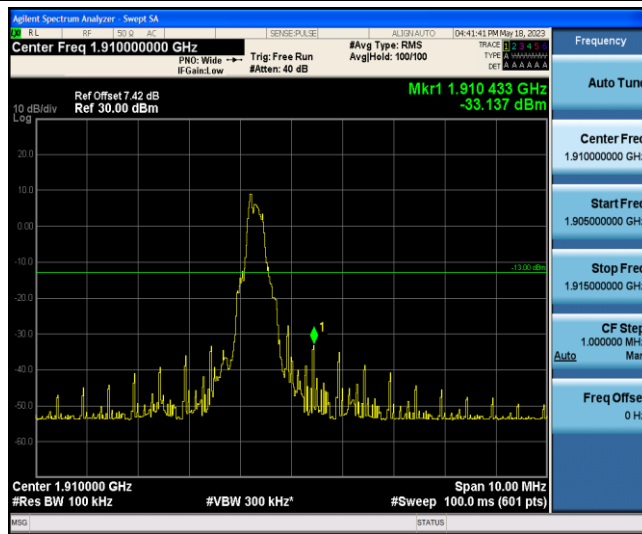
Band2-5MHz-16QAM-19175-1-5-High--33.14-PASS
