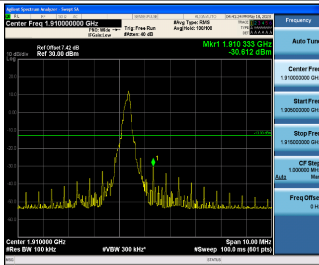
Band2-5MHz-QPSK-19175-1-5-High--30.61-PASS
