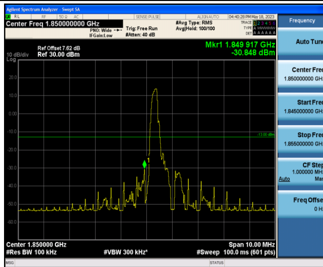
Band2-5MHz-16QAM-18625-1-0-Low--30.85-PASS
