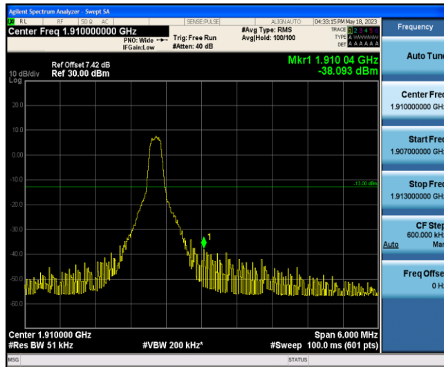
Band2-3MHz-16QAM-19185-1-5-High--38.09-PASS
