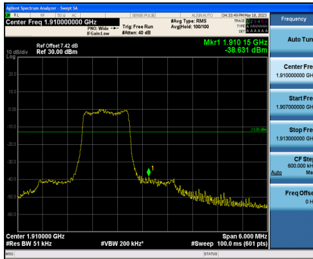
Band2-3MHz-16QAM-19185-6-0-High--38.63-PASS
