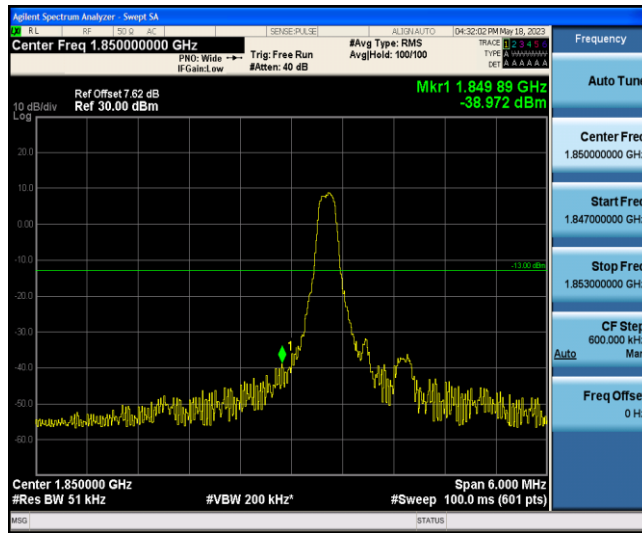
Band2-3MHz-16QAM-18615-1-0-Low--38.97-PASS
