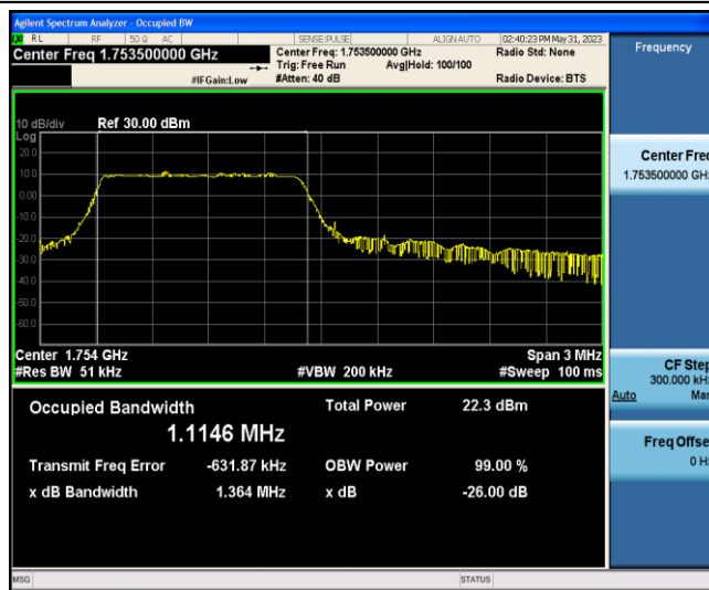
Band4-3MHz-16QAM-20385-6-0-Low-1.1146-1.364-PASS
