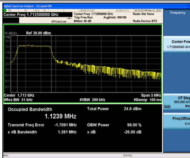
Band4-5MHz-QPSK-19975-6-0-Low-1.1239-1.381-PASS
