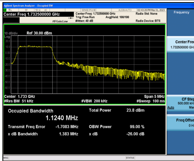
Band4-5MHz-QPSK-20175-6-0-Low-1.1240-1.383-PASS
