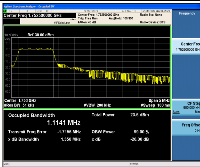
Band4-5MHz-QPSK-20375-6-0-Low-1.1141-1.350-PASS
