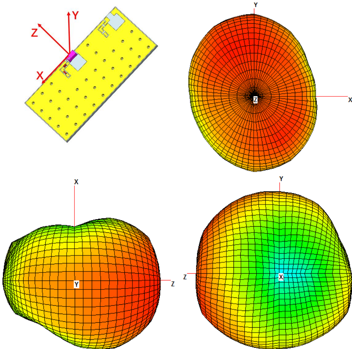
FIGURE 4.6.23 RADIATION PATTERN OF ANTENNA AT 2450MHZ IN FREE SPACE FOR CONFIGURE 2
