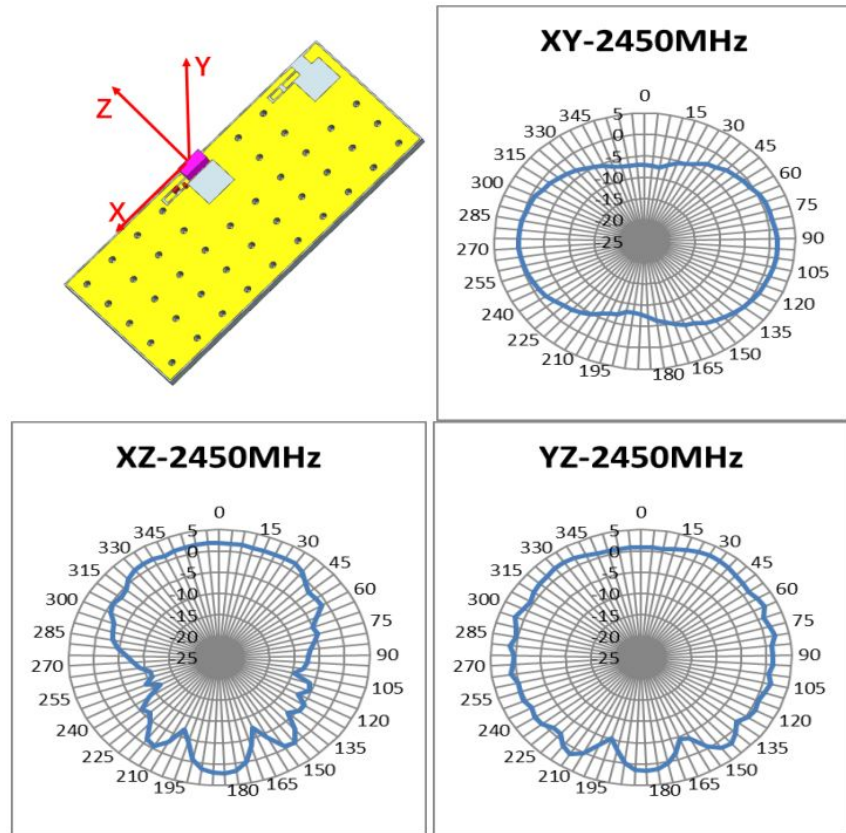
FIGURE 4.5.1 2D RADIATION PATTERN OF ANTENNA AT 2.4GHZ IN FREE SPACE FOR CONFIGURE 1
