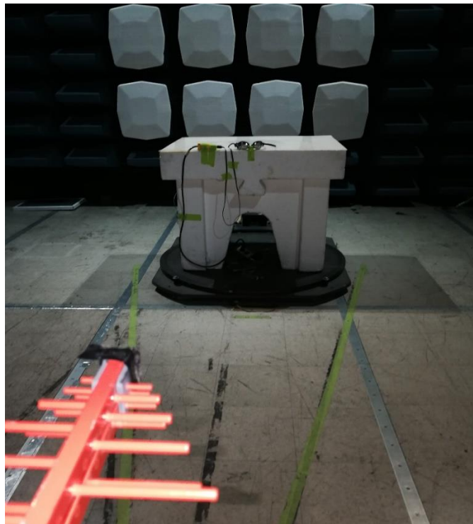
Radiated Emissions 3m SAC 30MHz – 1GHz – Photo1
