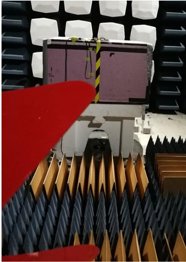
Radiated Emissions 3m SAC 1 – 18GHz – Photo1
