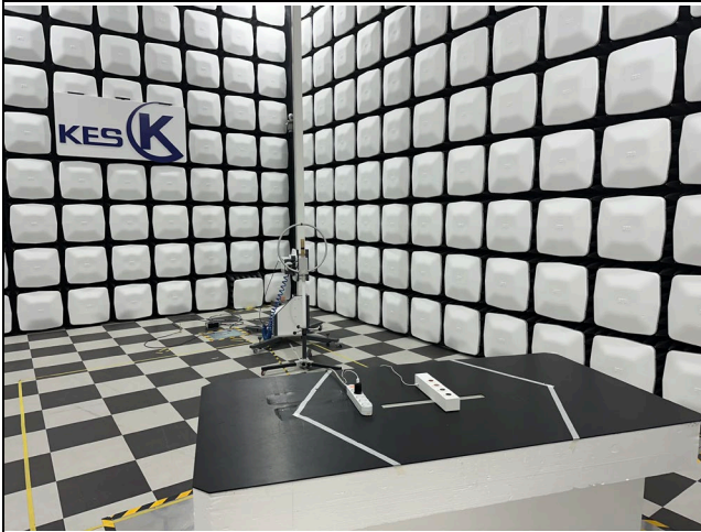
Radiated test
