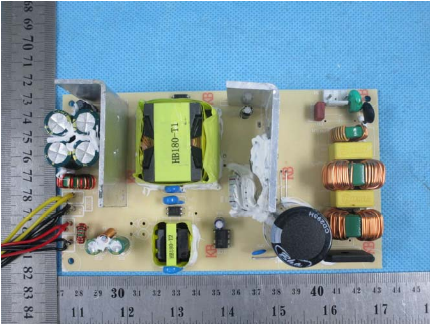
Inner Circuit Top View (Power panel “B”)
