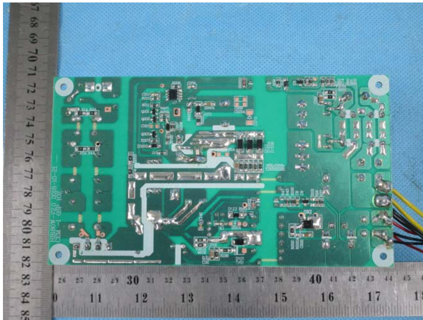
Inner Circuit Bottom View (Power panel "B")
