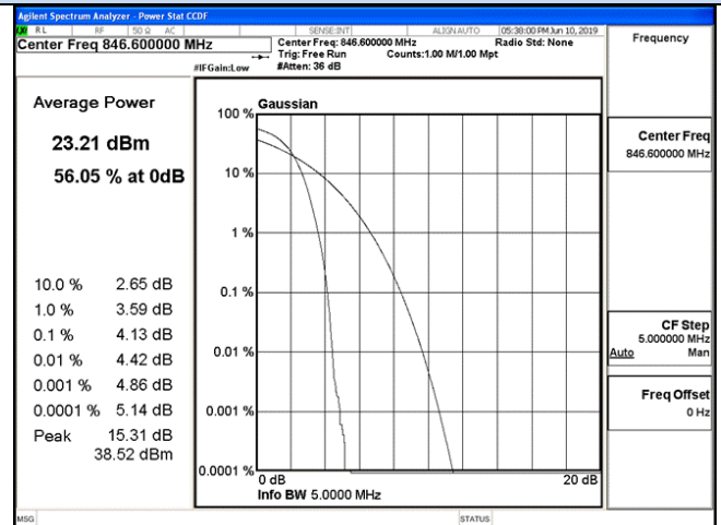
Channel 4233/ 846.6 MHz
