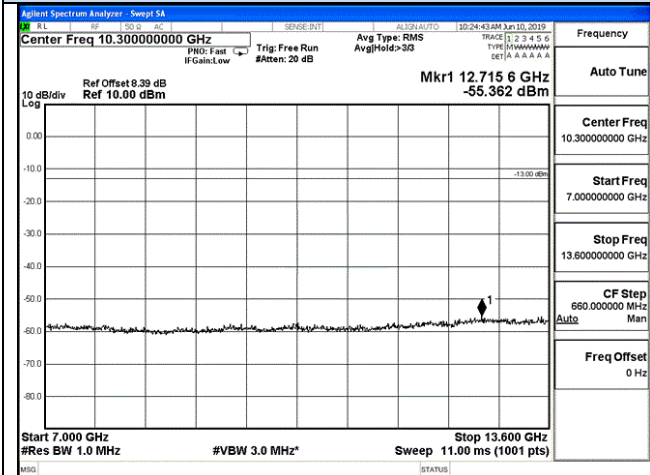
7 GHz – 13.6 GHz
