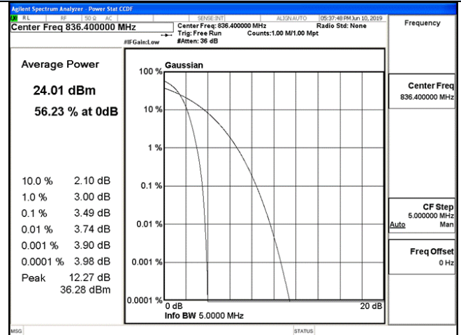
Channel 4182/ 836.4 MHz
