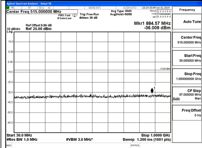
30 MHz – 1000 MHz
