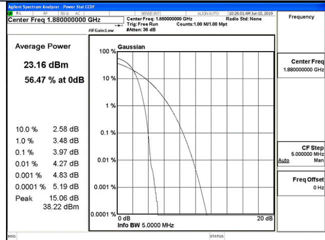
Channel 9400 / 1880.0 MHz
