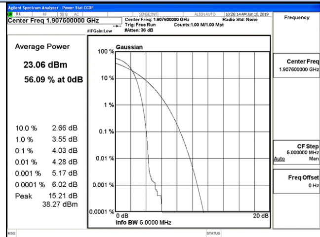
Channel 9538 / 1907.6 MHz
