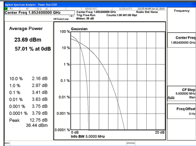
Channel 9262 / 1852.4 MHz
