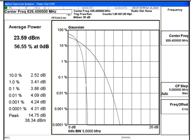
Channel 4132/ 826.4 MHz
