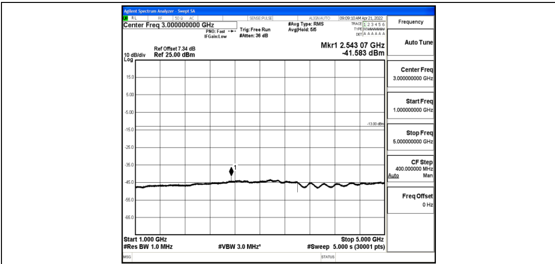
Band26-3MHz-16QAM-27025-1-0-High-1000-5000--41.58-PASS
