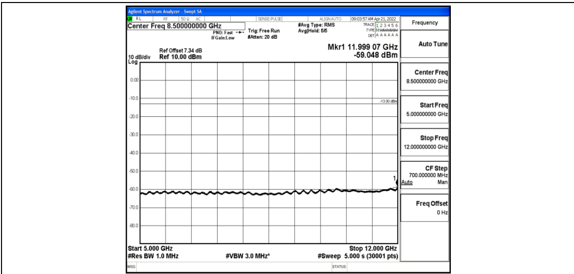
Band26-3MHz-QPSK-26915-1-0-Low-5000-12000--59.05-PASS
