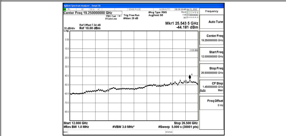
Band26-1.4MHz-16QAM-26915-1-0-Low-12000-26500--44.18-PASS
