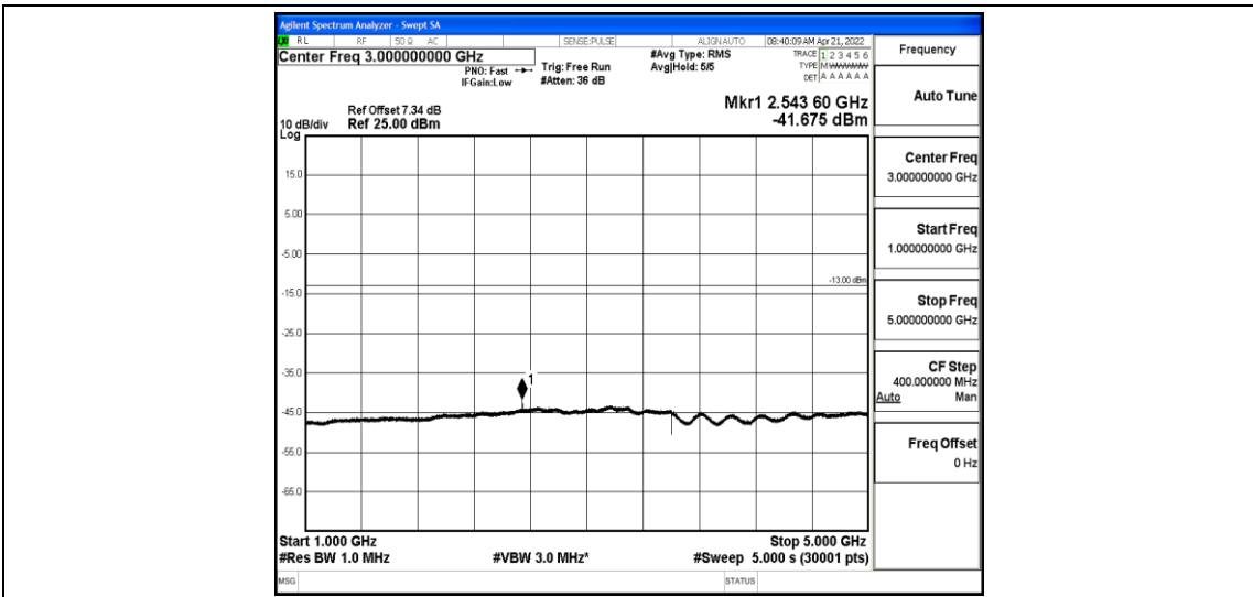
Band26-1.4MHz-QPSK-27033-1-0-High-1000-5000--41.68-PASS
