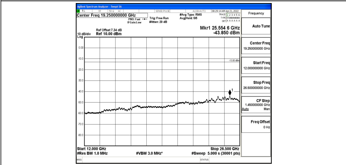
Band26-10MHz-QPSK-26990-1-0-High-12000-26500--43.85-PASS
