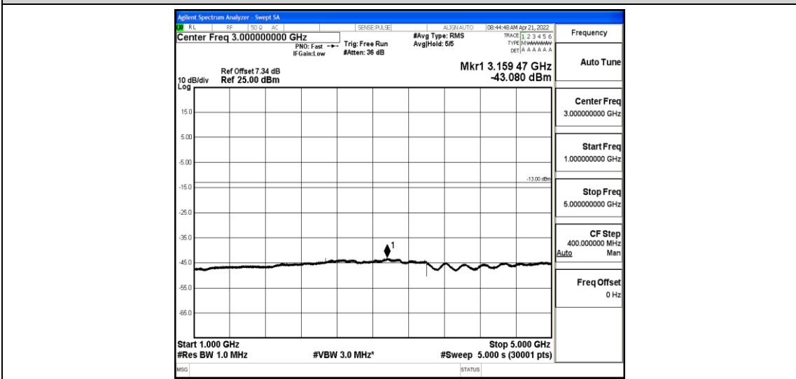
Band26-15MHz-QPSK-26865-1-0-Low-1000-5000--43.08-PASS
