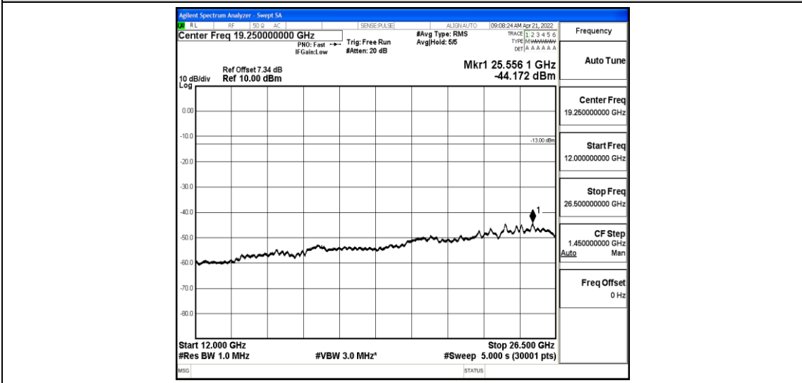
Band26-3MHz-QPSK-27025-1-0-High-12000-26500--44.17-PASS
