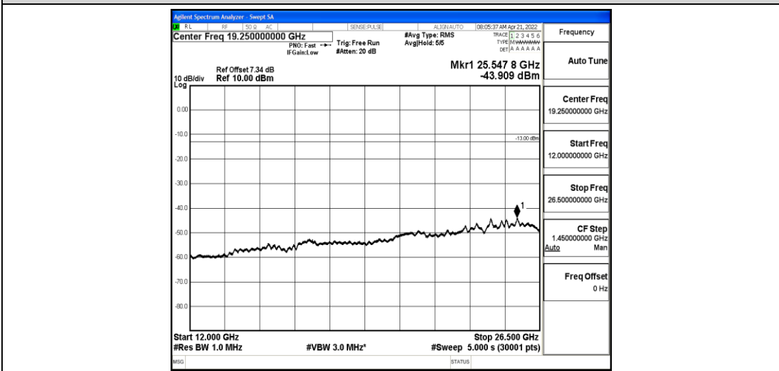
Band26-5MHz-16QAM-26915-1-0-Low-12000-26500--43.91-PASS
