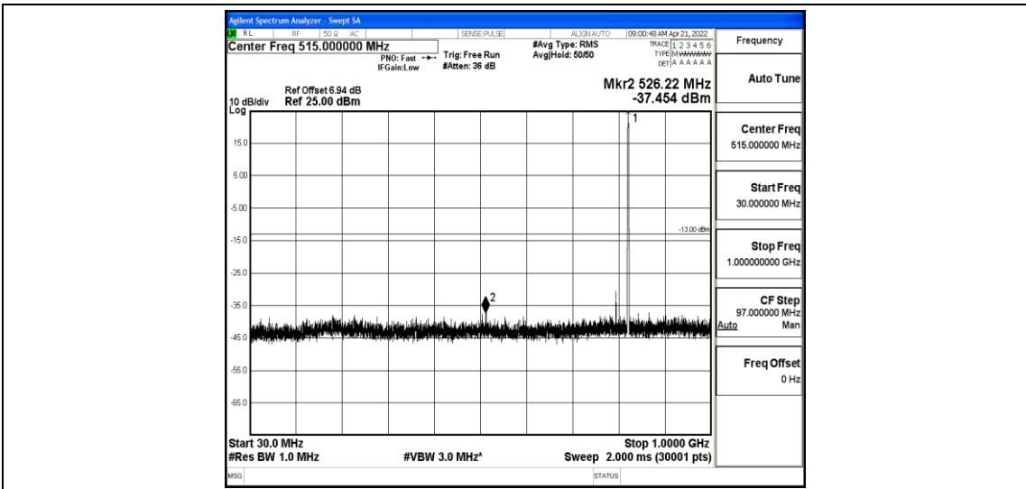
Band26-3MHz-16QAM-26805-1-0-Low-30-1000--37.45-PASS
