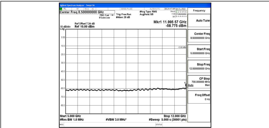
Band26-10MHz-QPSK-26915-1-0-Low-5000-12000--58.78-PASS
