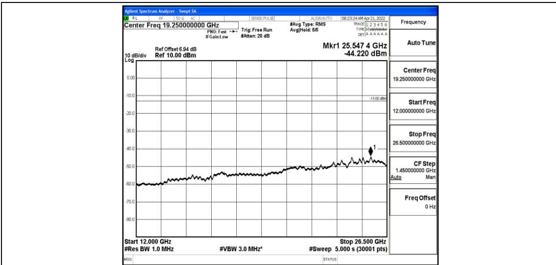
Band26-10MHz-16QAM-26840-1-0-Low-12000-26500--44.22-PASS
