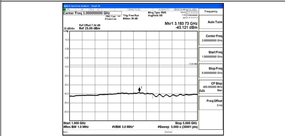
Band26-5MHz-QPSK-26915-1-0-Low-1000-5000--43.12-PASS
