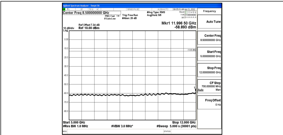
Band26-5MHz-16QAM-26915-1-0-Low-5000-12000--58.89-PASS
