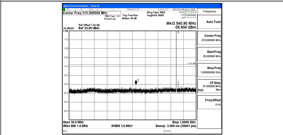
Band26-10MHz-16QAM-26990-1-0-High-30-1000--35.6-PASS
