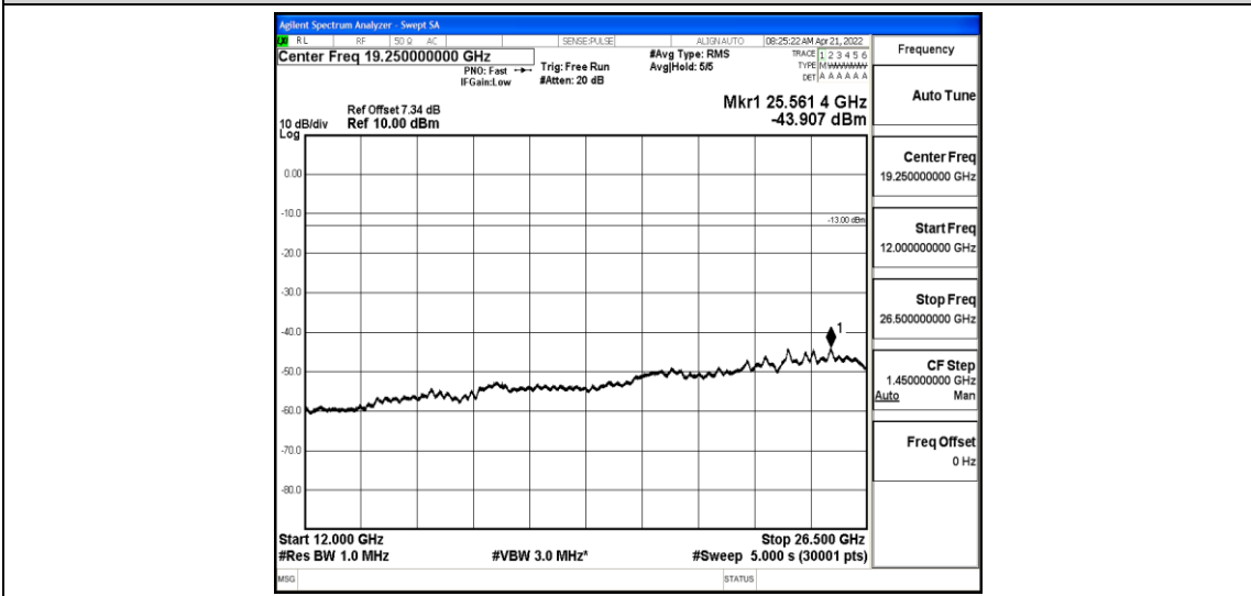
Band26-10MHz-QPSK-26915-1-0-Low-12000-26500--43.91-PASS
