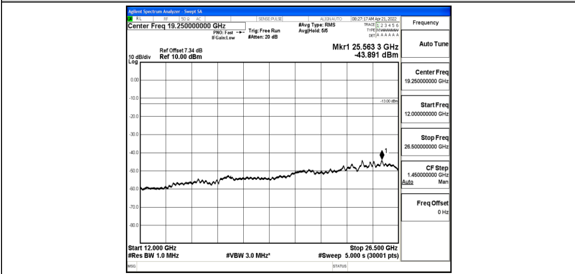
Band26-10MHz-16QAM-26915-1-0-Low-12000-26500--43.89-PASS
