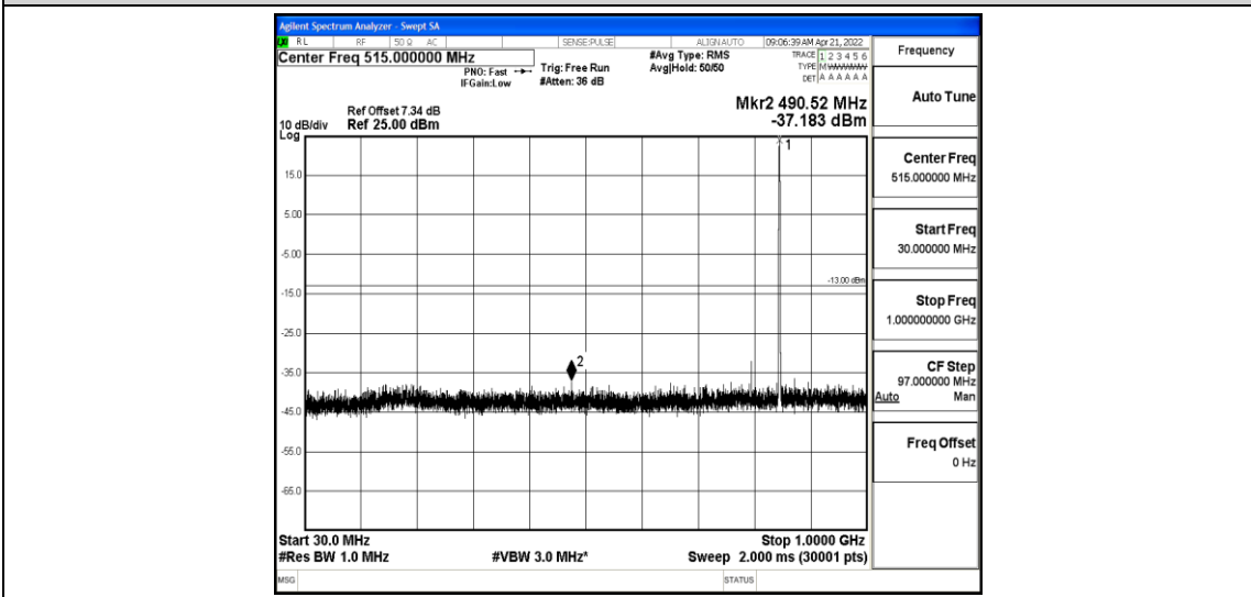
Band26-3MHz-QPSK-27025-1-0-High-30-1000--37.18-PASS
