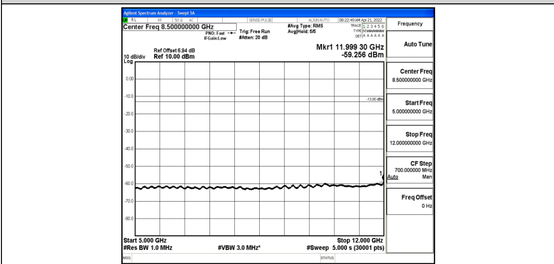
Band26-10MHz-16QAM-26840-1-0-Low-5000-12000--59.26-PASS
