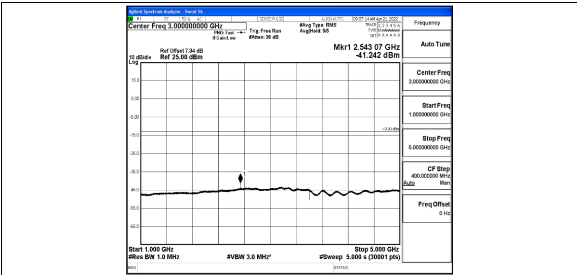
Band26-3MHz-QPSK-27025-1-0-High-1000-5000--41.24-PASS
