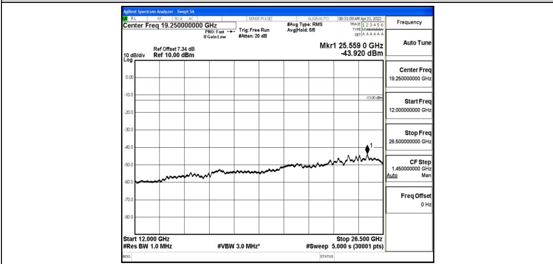
Band26-10MHz-16QAM-26990-1-0-High-12000-26500--43.92-PASS
