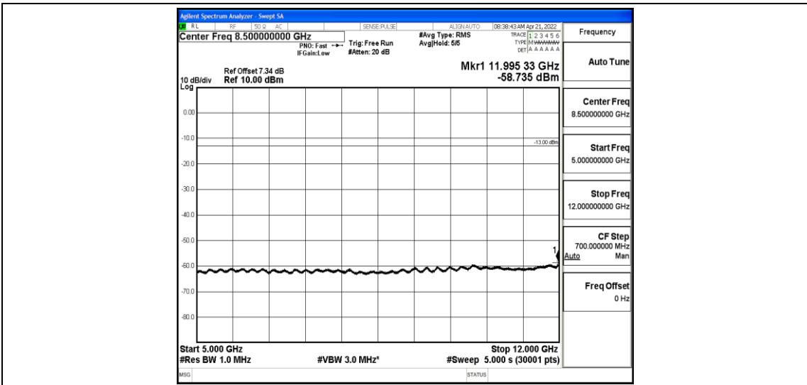
Band26-1.4MHz-16QAM-26915-1-0-Low-5000-12000--58.74-PASS
