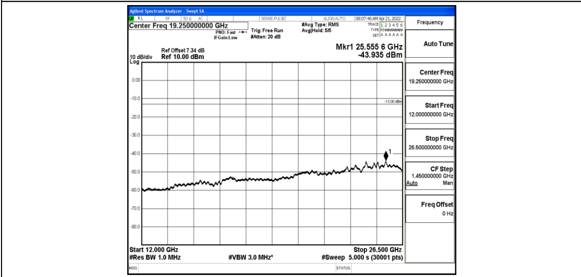
Band26-5MHz-QPSK-27015-1-0-High-12000-26500--43.94-PASS
