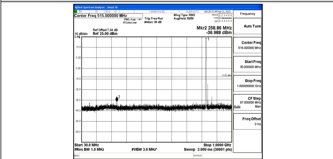
Band26-10MHz-16QAM-26915-1-0-Low-30-1000--36.99-PASS
