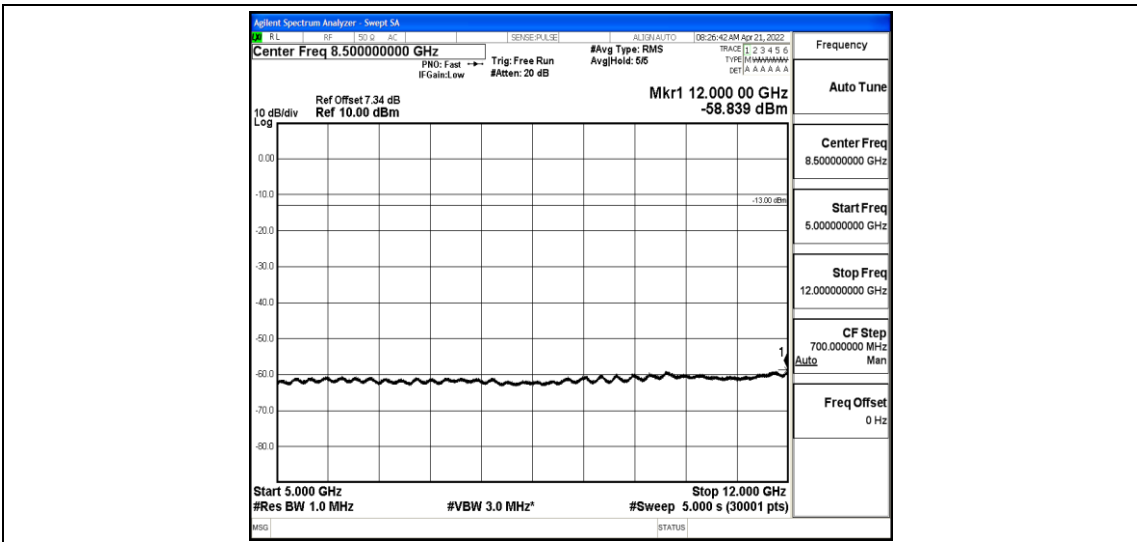
Band26-10MHz-16QAM-26915-1-0-Low-5000-12000--58.84-PASS
