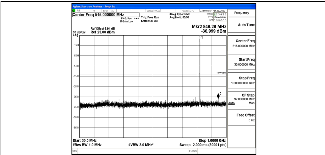
Band26-5MHz-QPSK-26815-1-0-Low-30-1000--37-PASS
