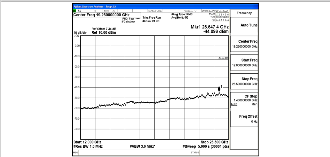
Band26-3MHz-QPSK-26915-1-0-Low-12000-26500--44.1-PASS
