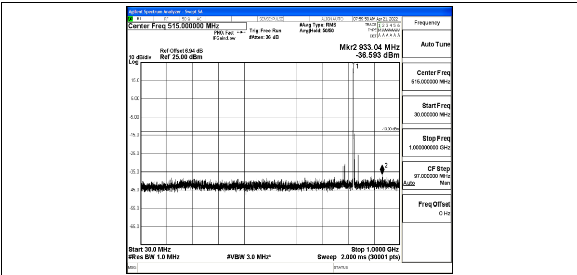
Band26-5MHz-16QAM-26815-1-0-Low-30-1000--36.59-PASS
