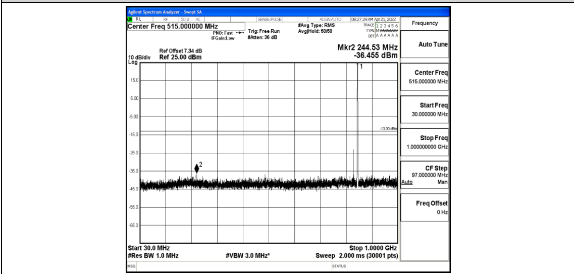
Band26-10MHz-QPSK-26990-1-0-High-30-1000--36.46-PASS
