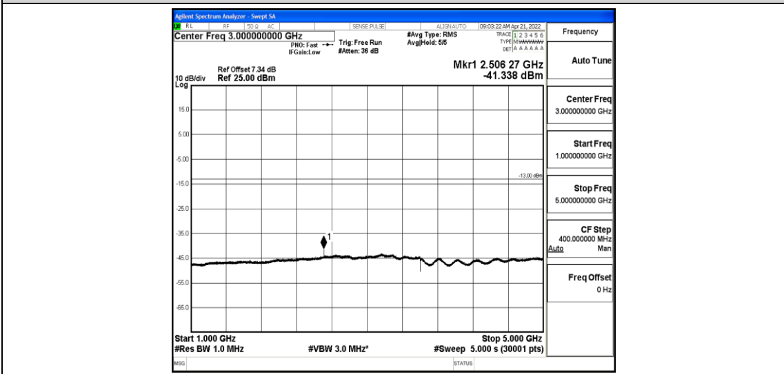
Band26-3MHz-QPSK-26915-1-0-Low-1000-5000--41.34-PASS
