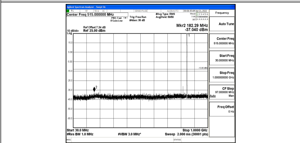
Band26-3MHz-16QAM-27025-1-0-High-30-1000--37.04-PASS
