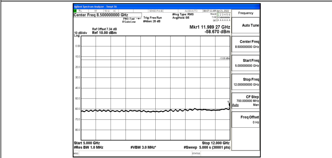
Band26-5MHz-QPSK-27015-1-0-High-5000-12000--58.67-PASS
