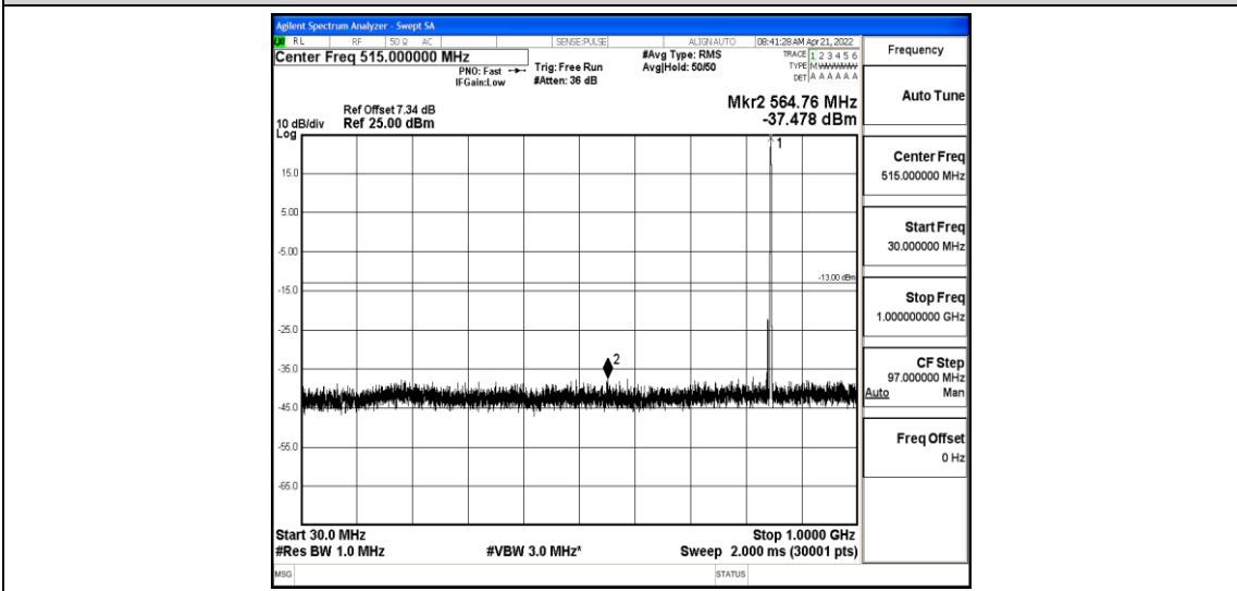
Band26-1.4MHz-16QAM-27033-1-0-High-30-1000--37.48-PASS
