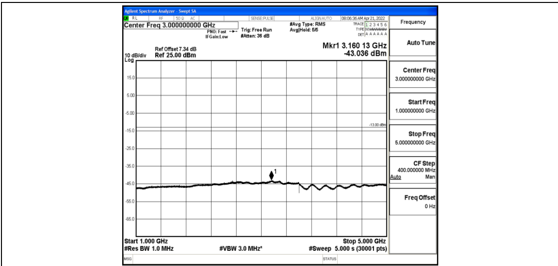
Band26-5MHz-QPSK-27015-1-0-High-1000-5000--43.04-PASS
