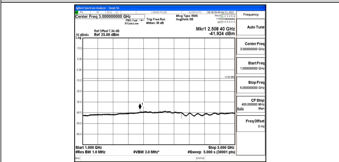
Band26-1.4MHz-16QAM-26915-1-0-Low-1000-5000--41.92-PASS
