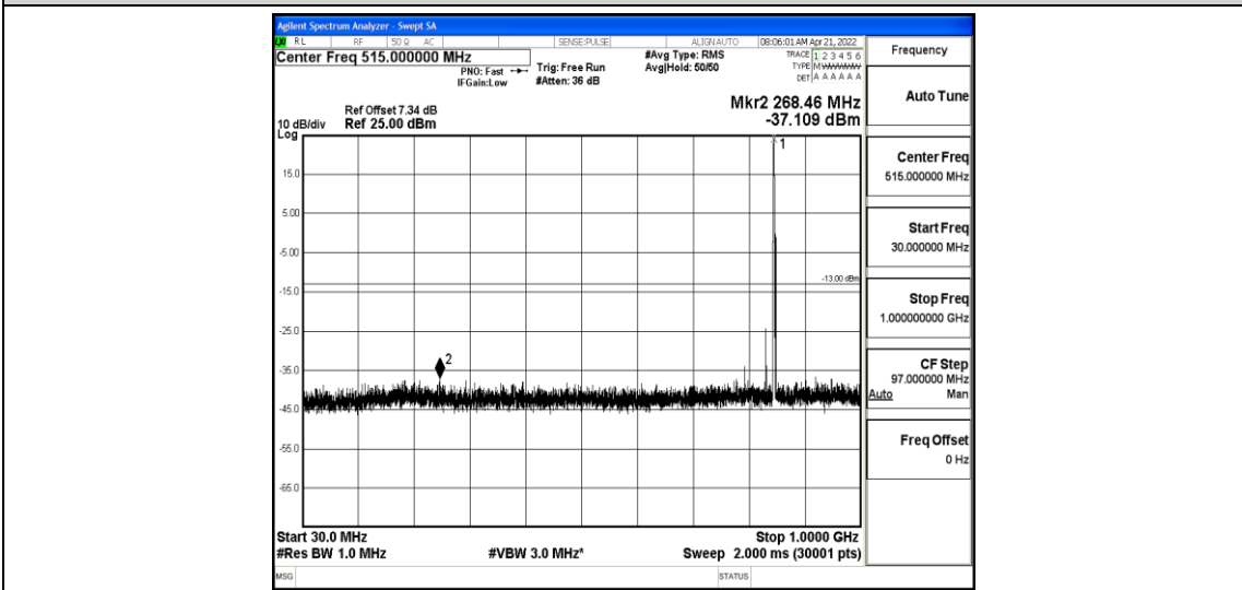
Band26-5MHz-QPSK-27015-1-0-High-30-1000--37.11-PASS
