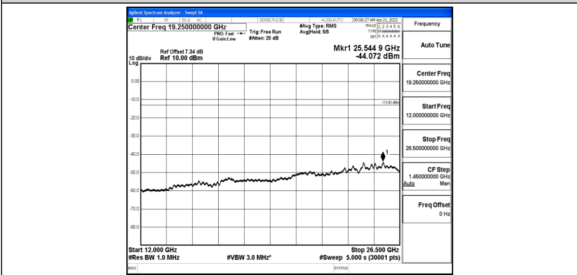
Band26-3MHz-16QAM-26915-1-0-Low-12000-26500--44.07-PASS
