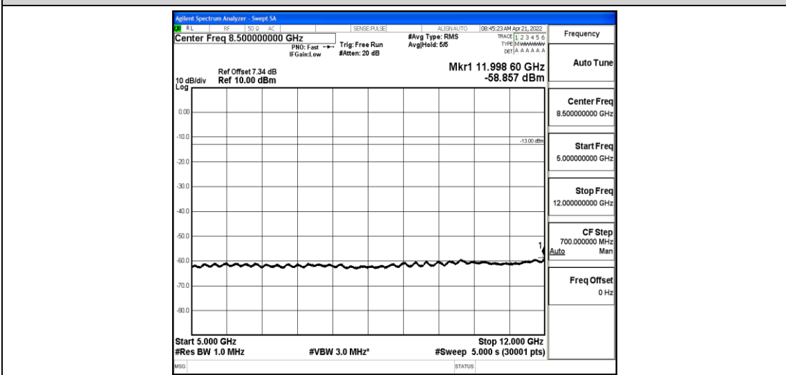
Band26-15MHz-QPSK-26865-1-0-Low-5000-12000--58.86-PASS
