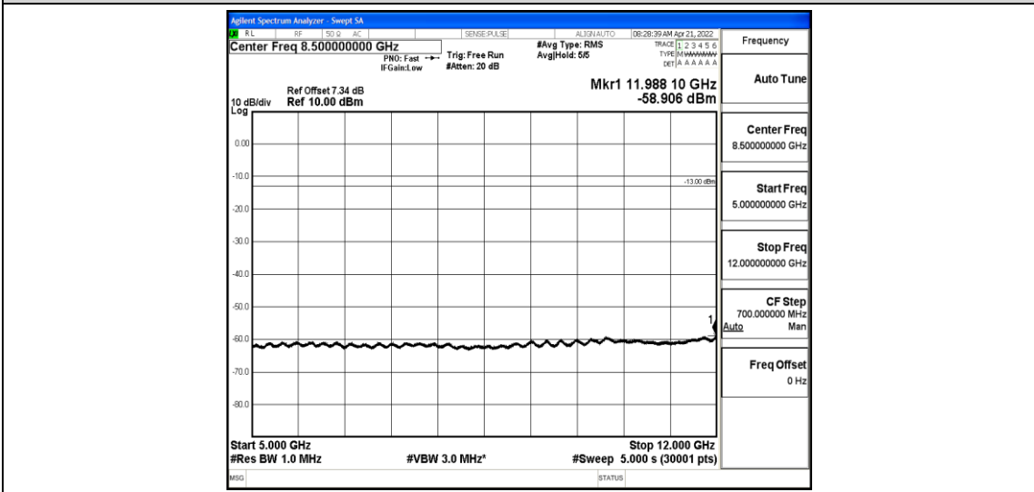
Band26-10MHz-QPSK-26990-1-0-High-5000-12000--58.91-PASS
