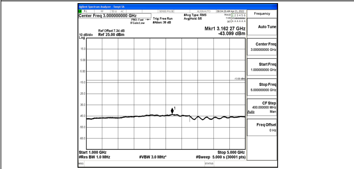
Band26-5MHz-16QAM-26915-1-0-Low-1000-5000--43.1-PASS
