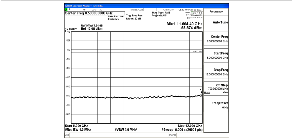
Band26-10MHz-16QAM-26990-1-0-High-5000-12000--58.87-PASS
