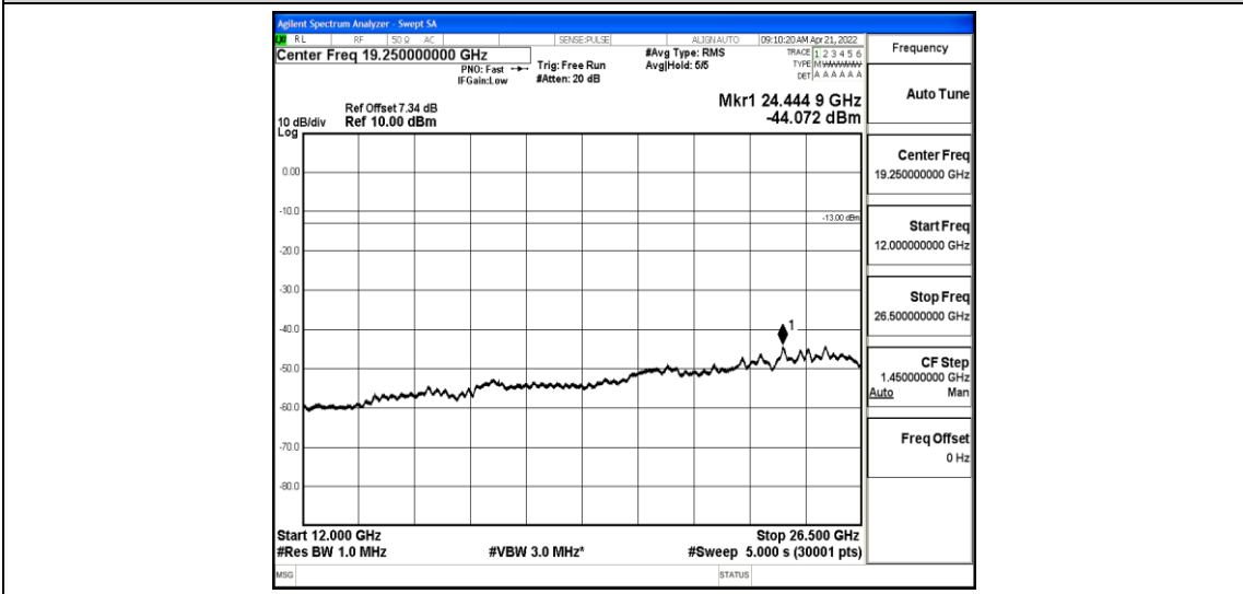
Band26-3MHz-16QAM-27025-1-0-High-12000-26500--44.07-PASS
