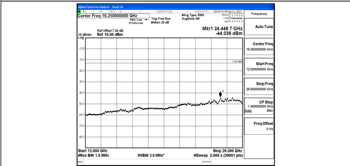
Band26-5MHz-QPSK-26915-1-0-Low-12000-26500--44.04-PASS
