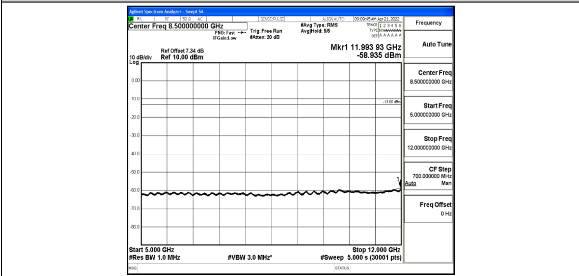
Band26-3MHz-16QAM-27025-1-0-High-5000-12000--58.94-PASS
