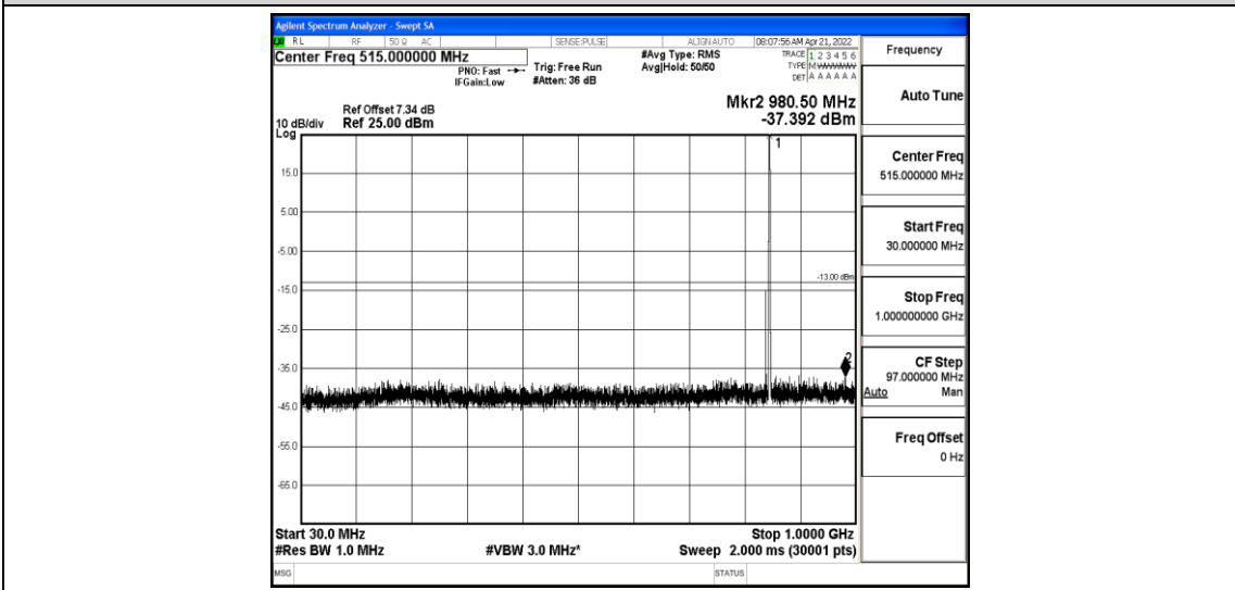
Band26-5MHz-16QAM-27015-1-0-High-30-1000--37.39-PASS
