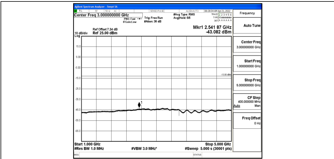
Band26-10MHz-QPSK-26990-1-0-High-1000-5000--43.08-PASS
