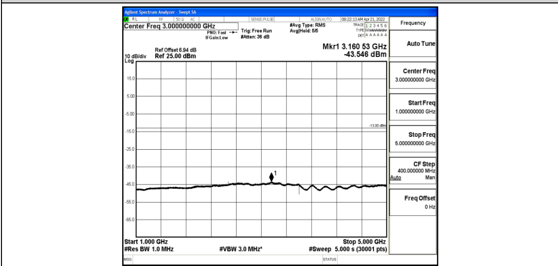
Band26-10MHz-16QAM-26840-1-0-Low-1000-5000--43.55-PASS
