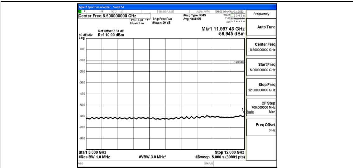
Band26-5MHz-QPSK-26915-1-0-Low-5000-12000--58.95-PASS
