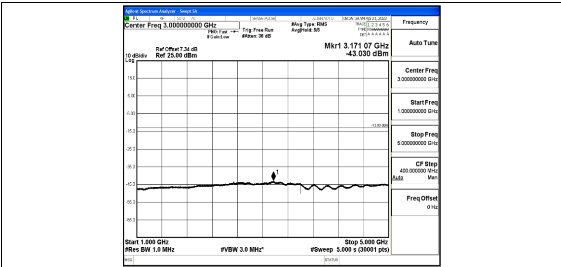
Band26-10MHz-16QAM-26990-1-0-High-1000-5000--43.03-PASS
