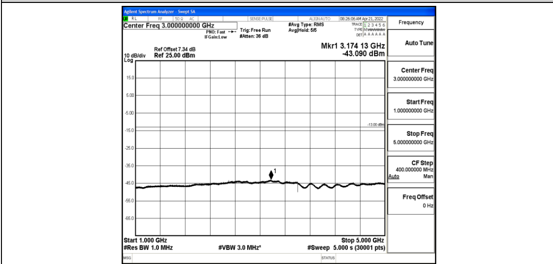
Band26-10MHz-16QAM-26915-1-0-Low-1000-5000--43.09-PASS
