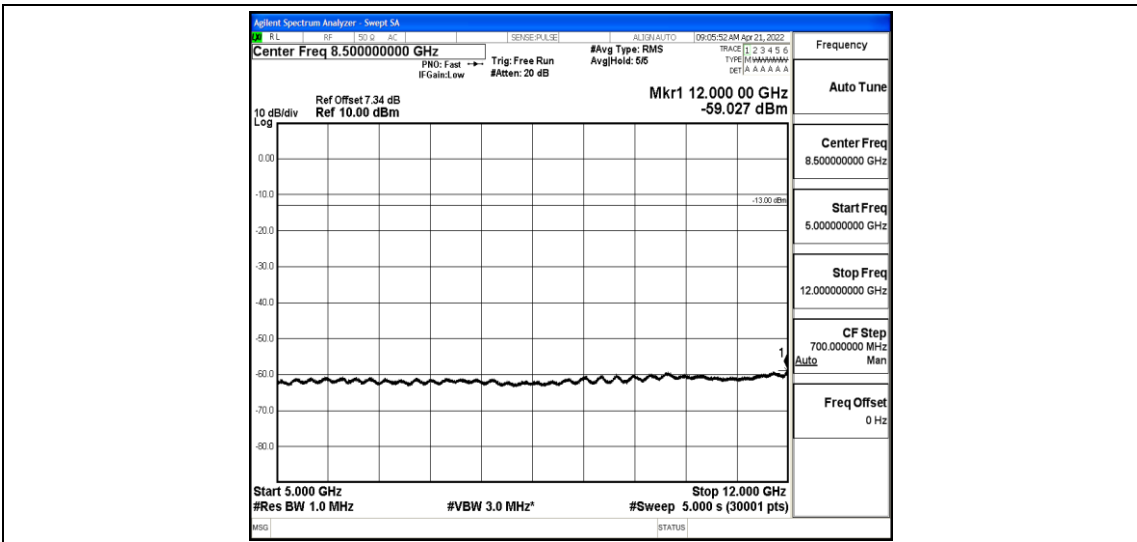
Band26-3MHz-16QAM-26915-1-0-Low-5000-12000--59.03-PASS
