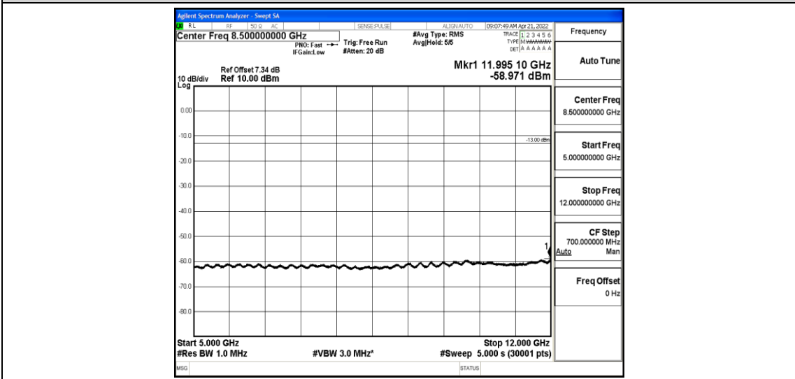
Band26-3MHz-QPSK-27025-1-0-High-5000-12000--58.97-PASS
