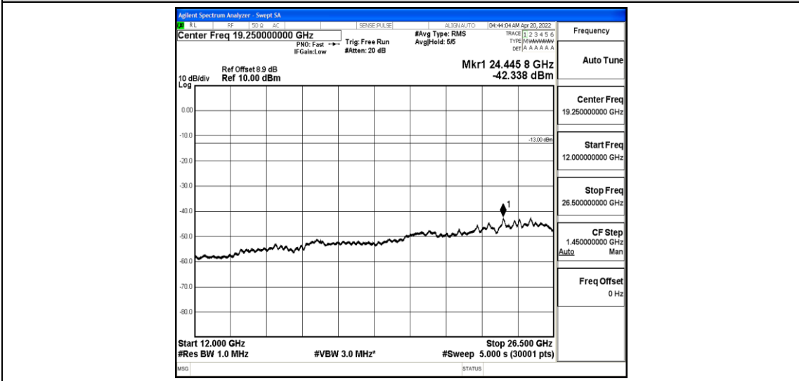
Band25-1.4MHz-16QAM-26683-1-0-High-12000-26500--42.34-PASS
