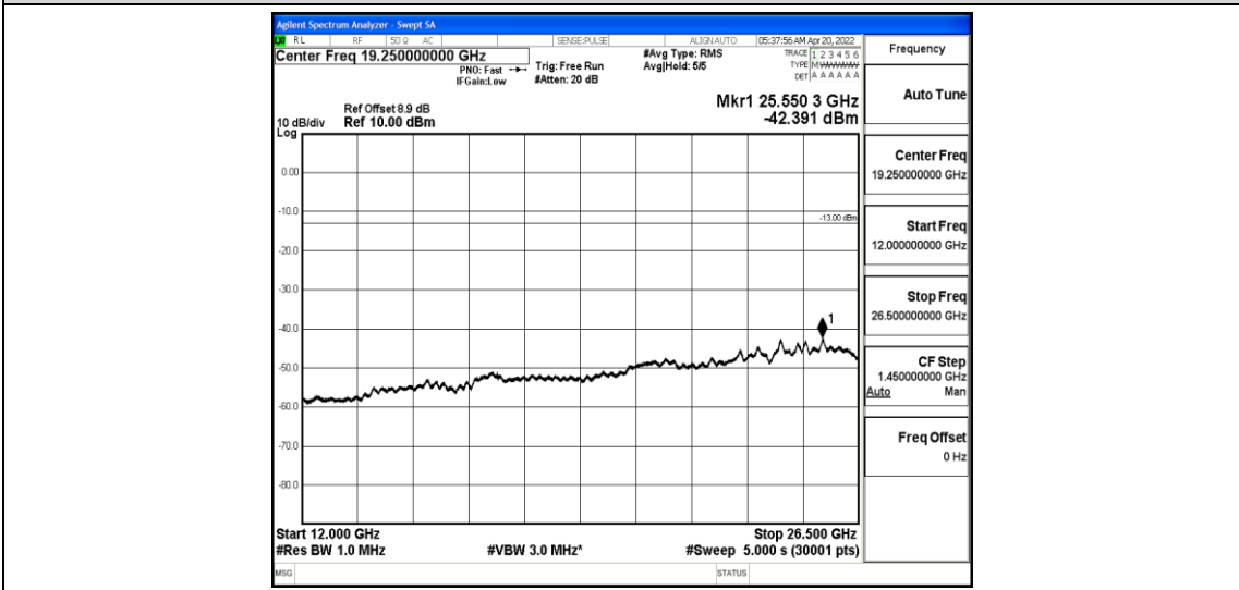
Band25-5MHz-QPSK-26365-1-0-Low-12000-26500--42.39-PASS
