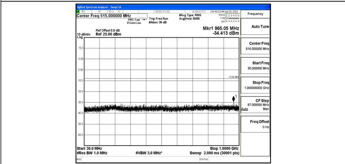
Band25-1.4MHz-QPSK-26683-1-0-High-30-1000--34.41-PASS
