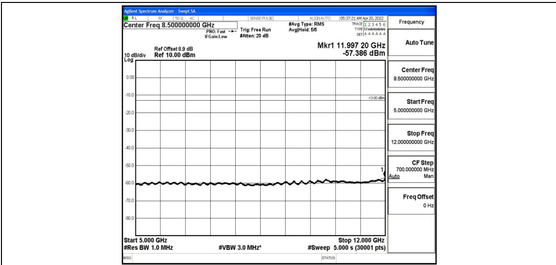
Band25-5MHz-QPSK-26365-1-0-Low-5000-12000--57.39-PASS
