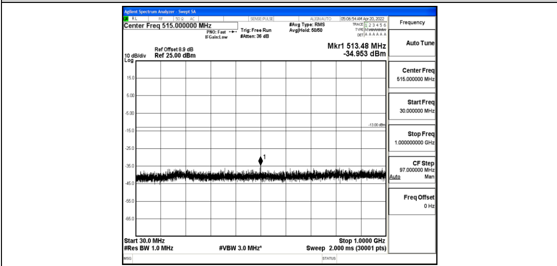
Band25-3MHz-QPSK-26675-1-0-High-30-1000--34.95-PASS
