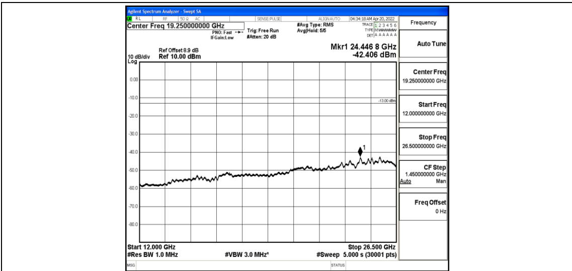
Band25-1.4MHz-QPSK-26047-1-0-Low-12000-26500--42.41-PASS
