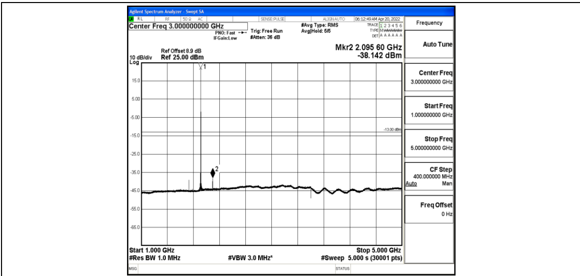
Band25-10MHz-QPSK-26640-1-0-High-1000-5000--38.14-PASS
