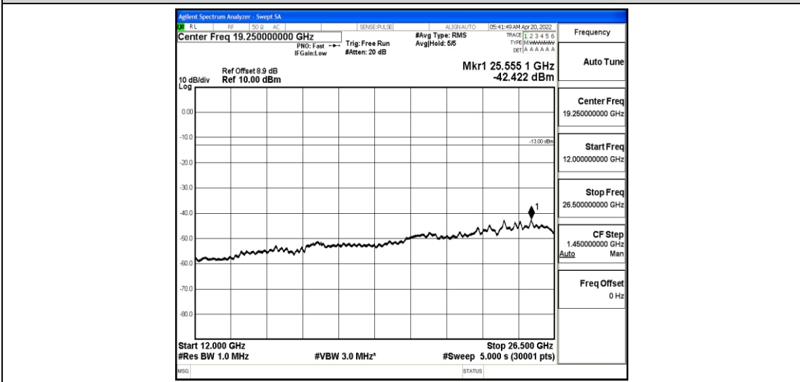
Band25-5MHz-QPSK-26665-1-0-High-12000-26500--42.42-PASS
