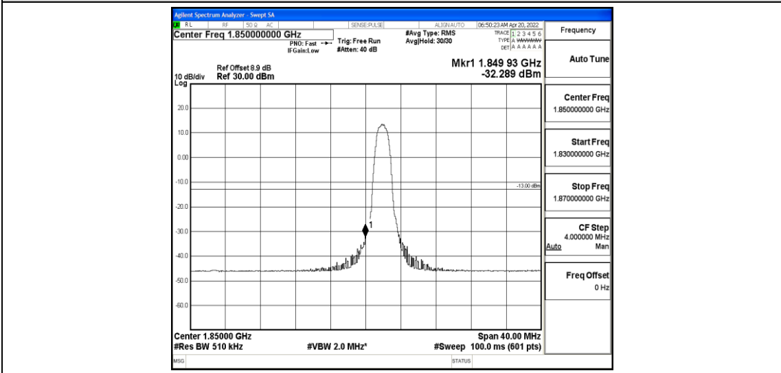
Band25-20MHz-QPSK-26140-6-0-Low--32.29-PASS
