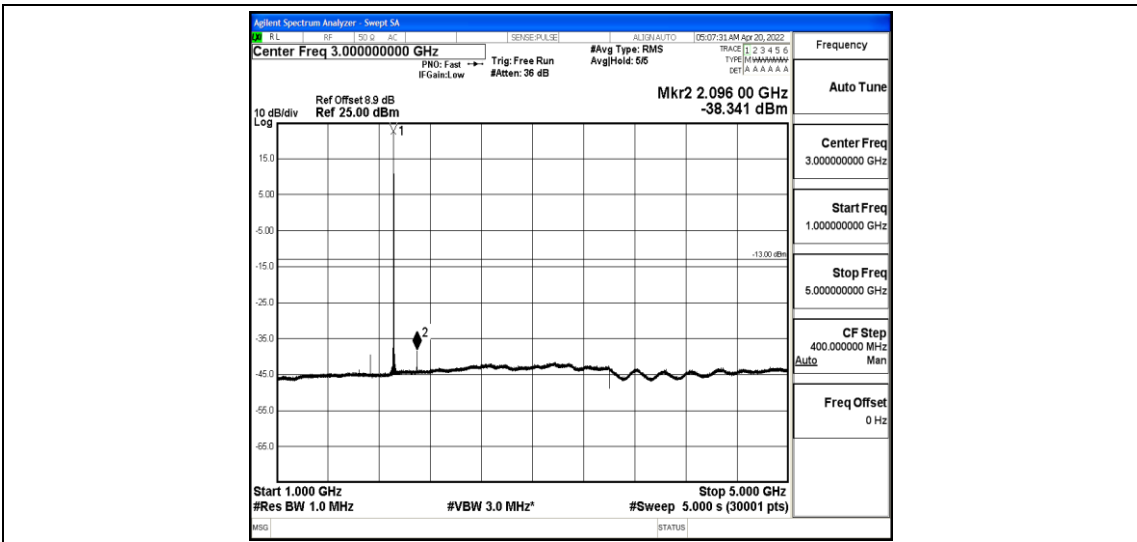
Band25-3MHz-QPSK-26675-1-0-High-1000-5000--38.34-PASS
