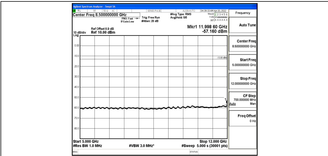
Band25-1.4MHz-16QAM-26365-1-0-Low-5000-12000--57.16-PASS
