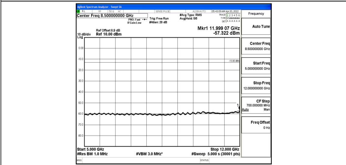
Band25-5MHz-16QAM-26665-1-0-High-5000-12000--57.32-PASS
