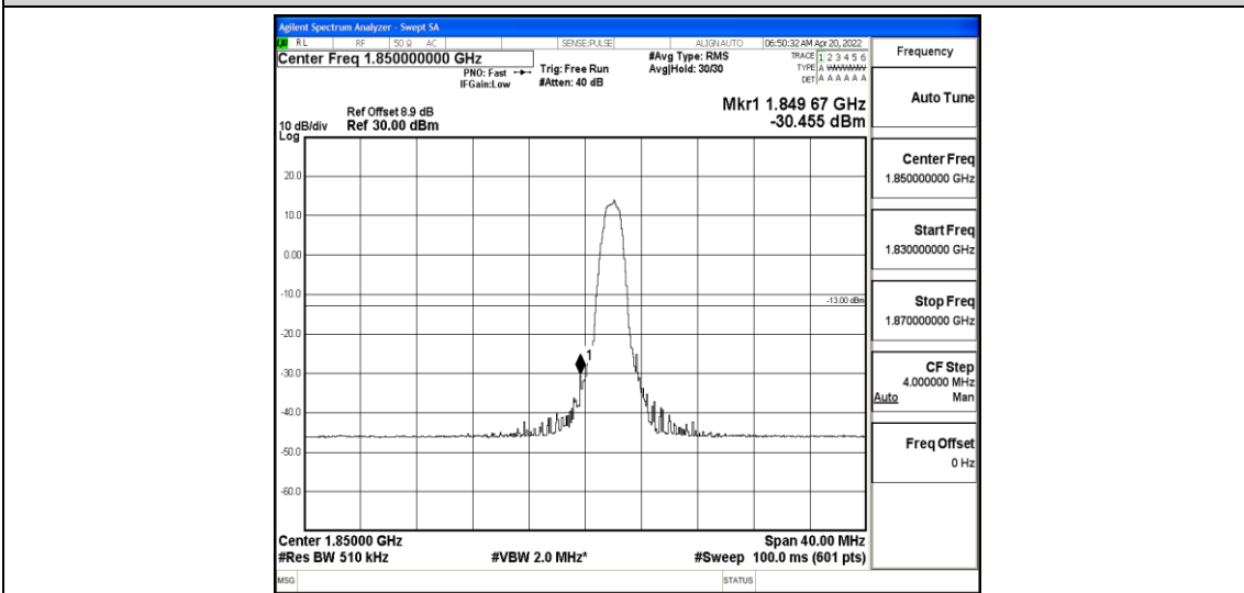
Band25-20MHz-16QAM-26140-6-0-Low--30.45-PASS
