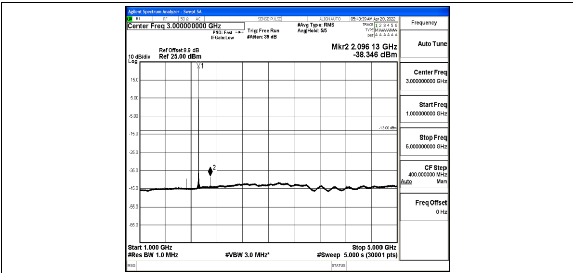
Band25-5MHz-QPSK-26665-1-0-High-1000-5000--38.35-PASS
