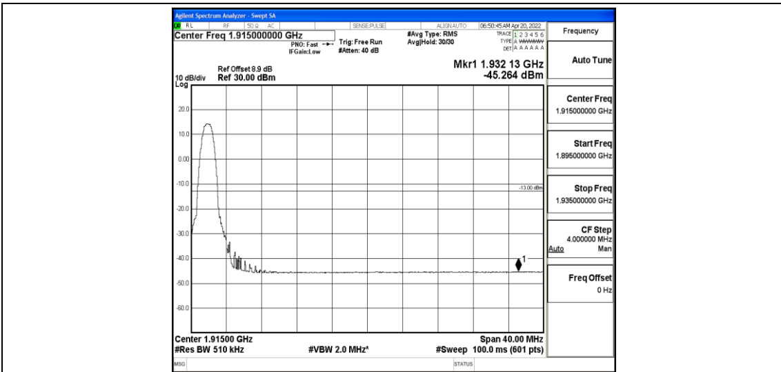
Band25-20MHz-QPSK-26590-6-0-Low--45.26-PASS
