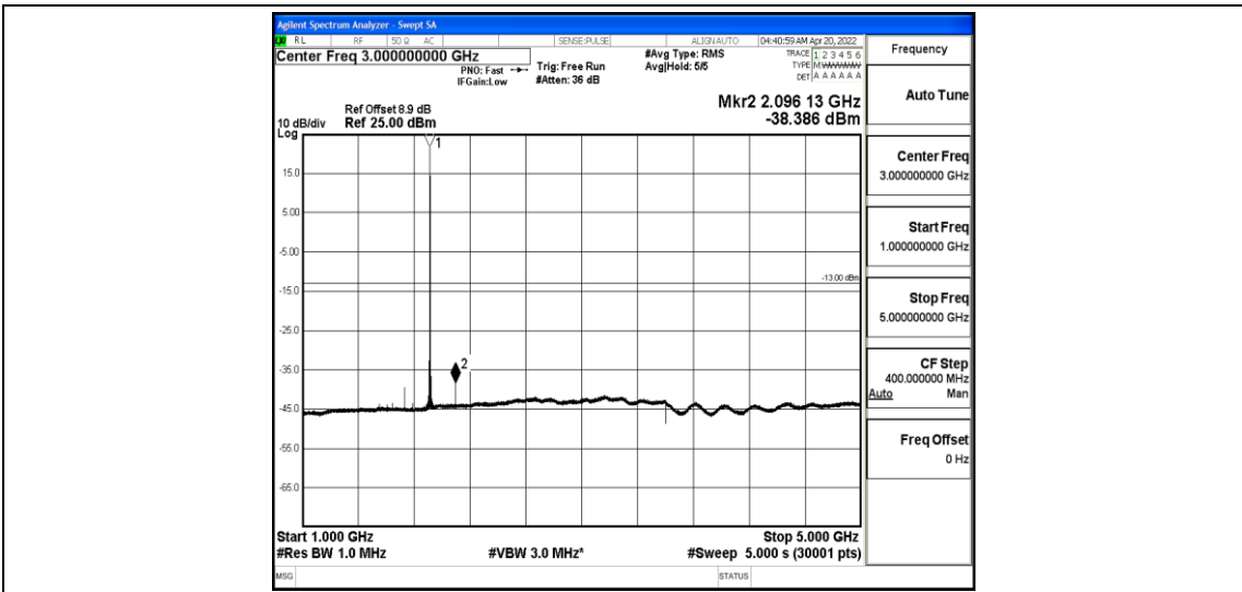
Band25-1.4MHz-QPSK-26683-1-0-High-1000-5000--38.39-PASS
