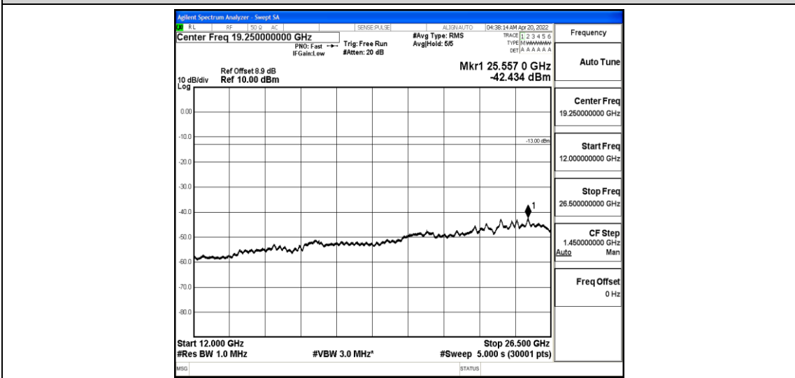
Band25-1.4MHz-QPSK-26365-1-0-Low-12000-26500--42.43-PASS
