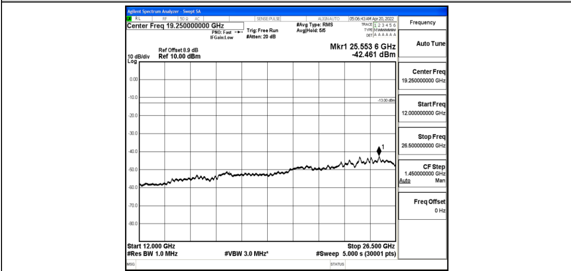
Band25-3MHz-16QAM-26365-1-0-Low-12000-26500--42.46-PASS
