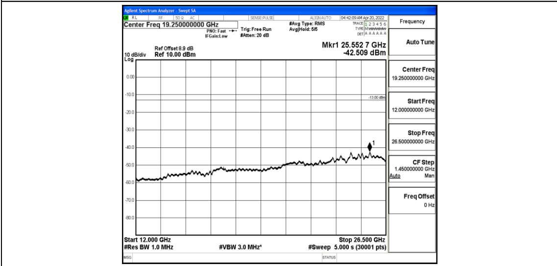
Band25-1.4MHz-QPSK-26683-1-0-High-12000-26500--42.51-PASS
