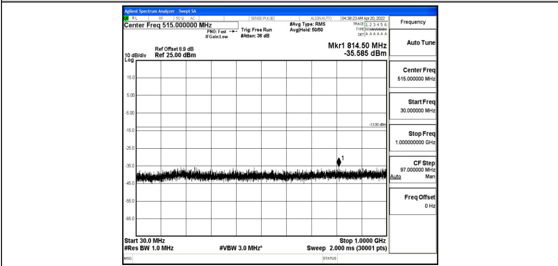
Band25-1.4MHz-16QAM-26365-1-0-Low-30-1000--35.59-PASS
