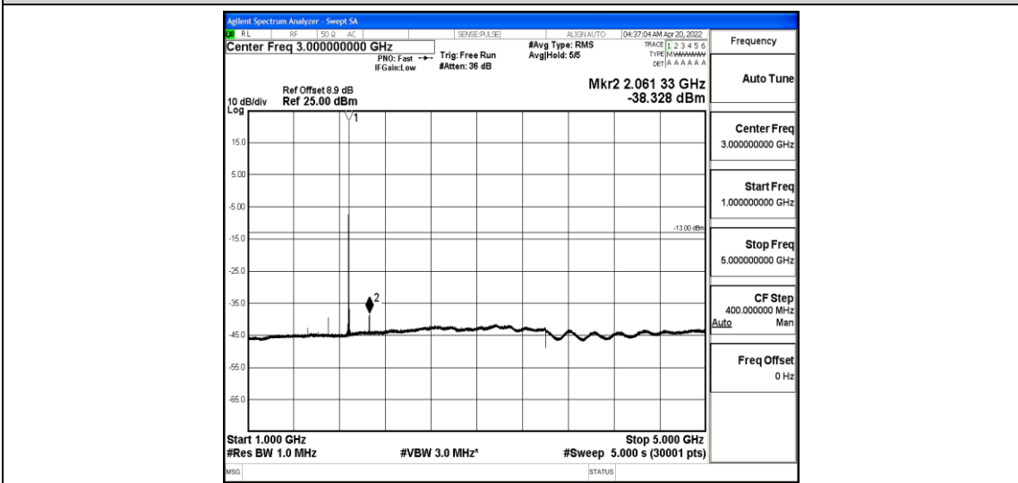
Band25-1.4MHz-QPSK-26365-1-0-Low-1000-5000--38.33-PASS
