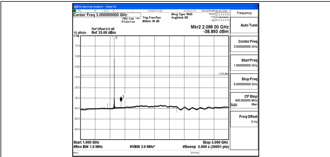
Band25-1.4MHz-16QAM-26683-1-0-High-1000-5000--38.89-PASS
