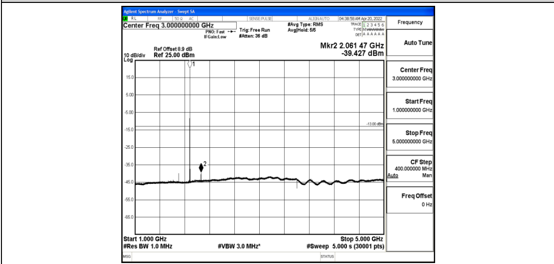
Band25-1.4MHz-16QAM-26365-1-0-Low-1000-5000--39.43-PASS
