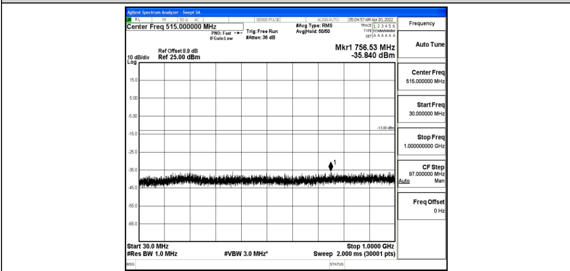
Band25-3MHz-16QAM-26365-1-0-Low-30-1000--35.84-PASS
