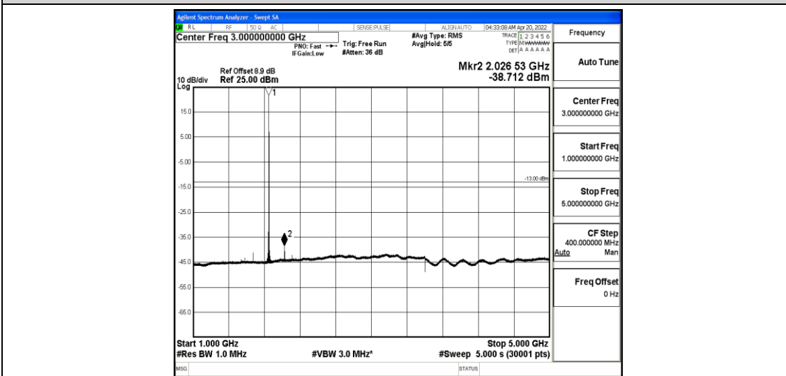
Band25-1.4MHz-QPSK-26047-1-0-Low-1000-5000--38.71-PASS
