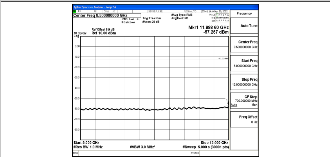
Band25-5MHz-QPSK-26665-1-0-High-5000-12000--57.26-PASS
