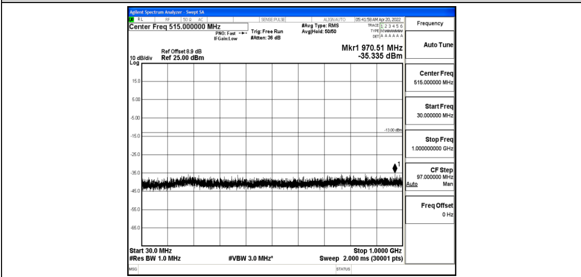
Band25-5MHz-16QAM-26665-1-0-High-30-1000--35.34-PASS
