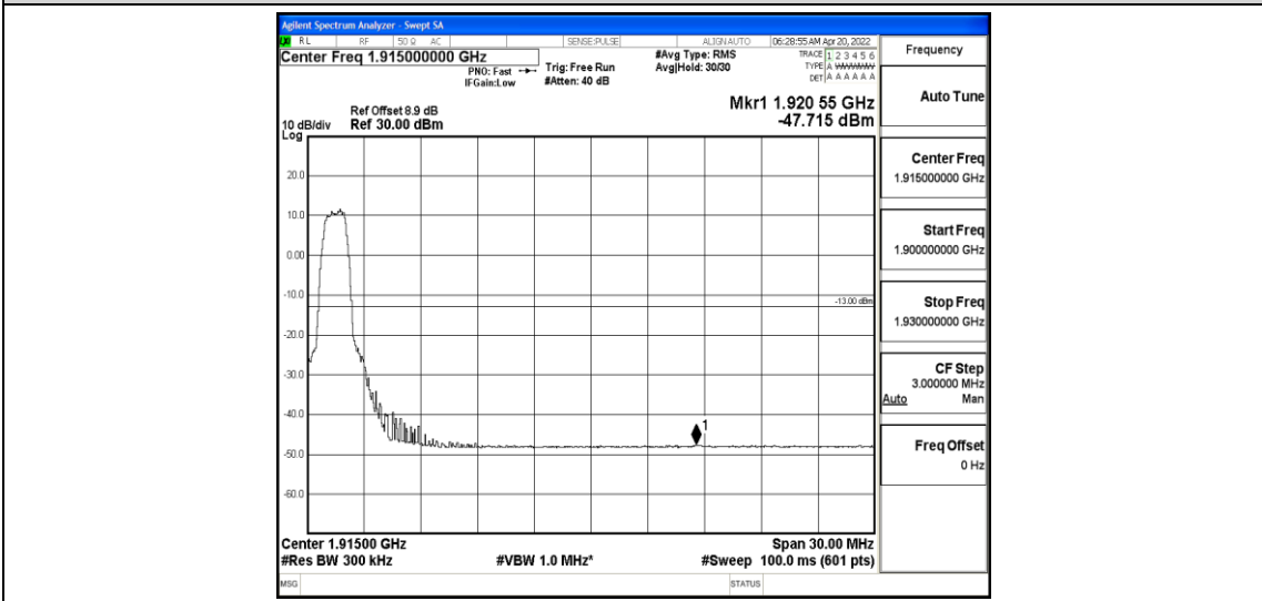
Band25-15MHz-16QAM-26615-6-0-Low--47.71-PASS
