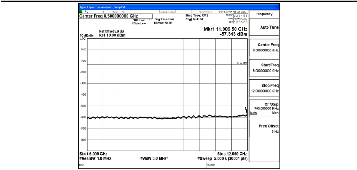
Band25-1.4MHz-16QAM-26683-1-0-High-5000-12000--57.34-PASS
