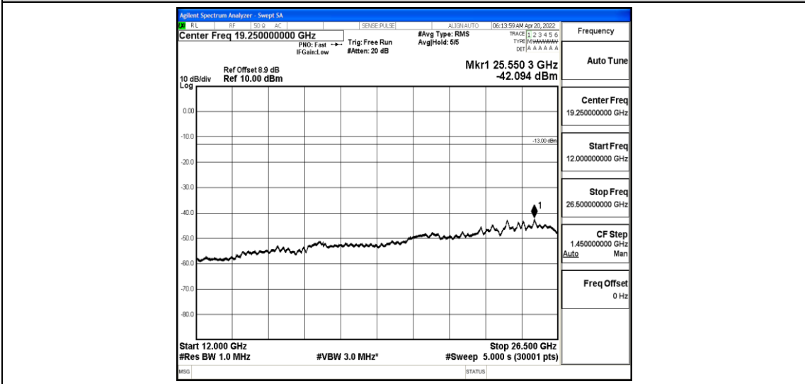
Band25-10MHz-QPSK-26640-1-0-High-12000-26500--42.09-PASS
