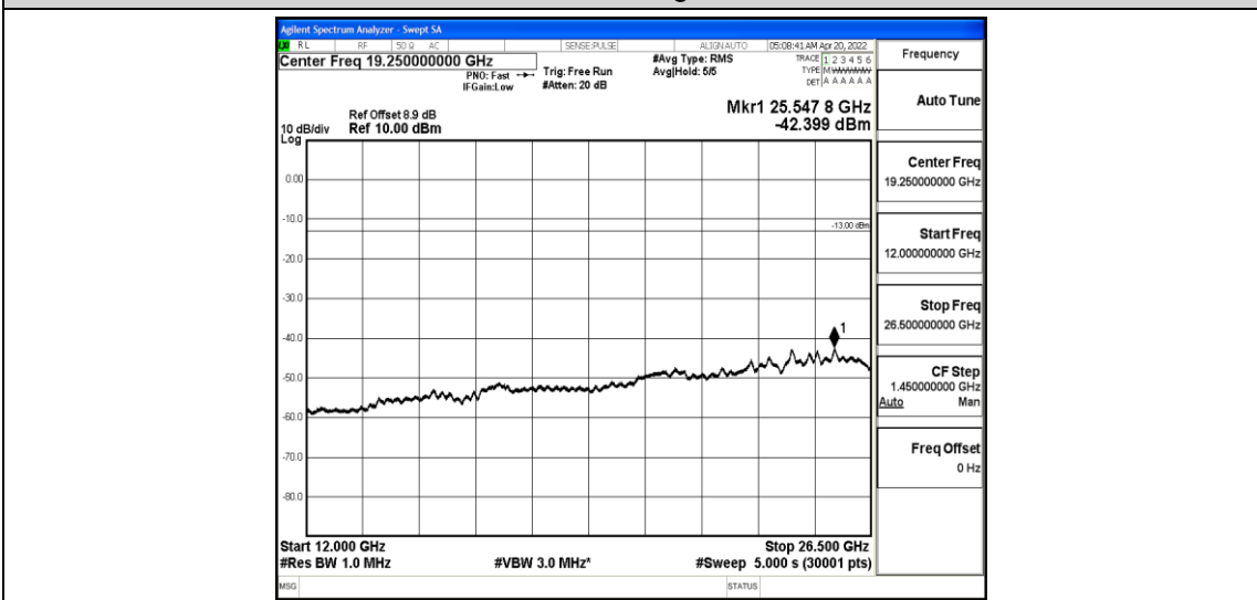
Band25-3MHz-QPSK-26675-1-0-High-12000-26500--42.4-PASS
