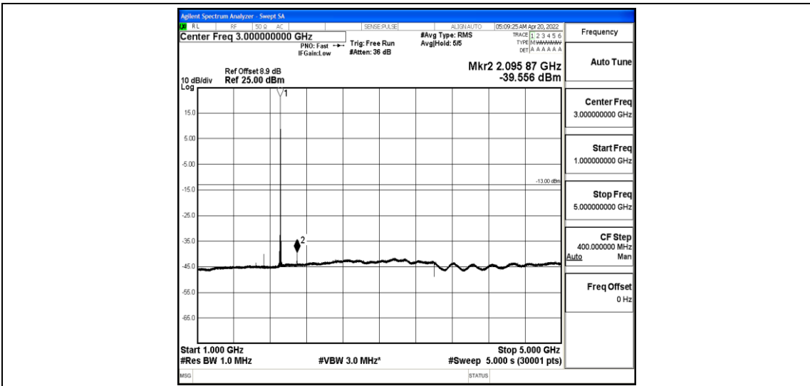
Band25-3MHz-16QAM-26675-1-0-High-1000-5000--39.56-PASS
