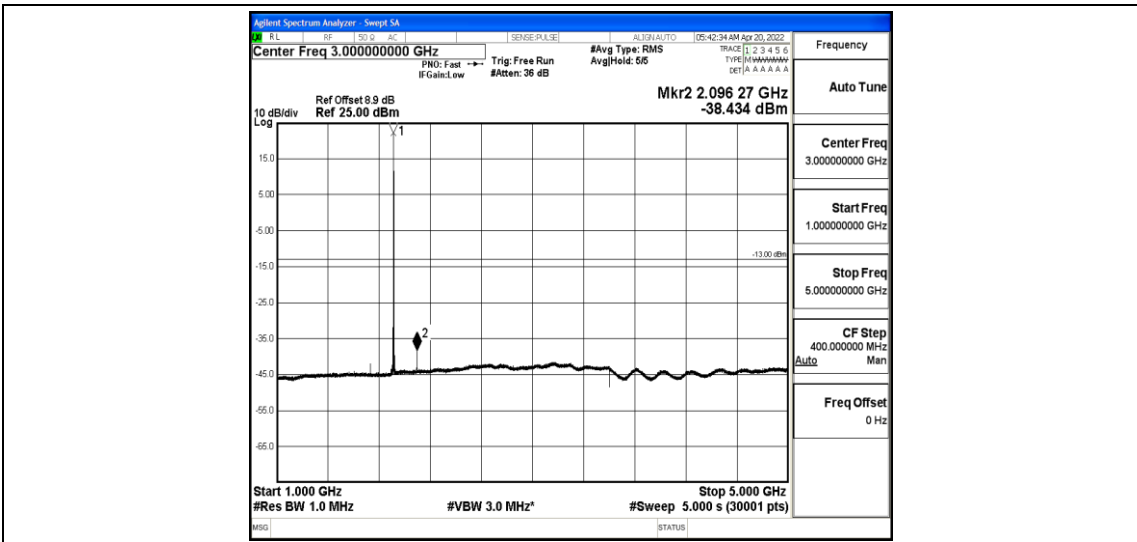
Band25-5MHz-16QAM-26665-1-0-High-1000-5000--38.43-PASS
