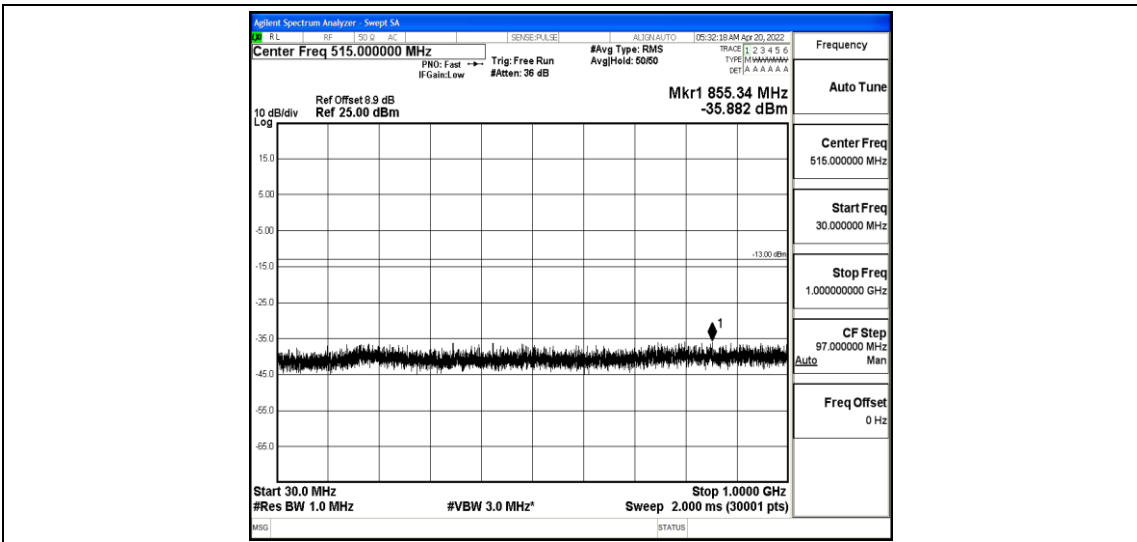
Band25-5MHz-QPSK-26065-1-0-Low-30-1000--35.88-PASS
