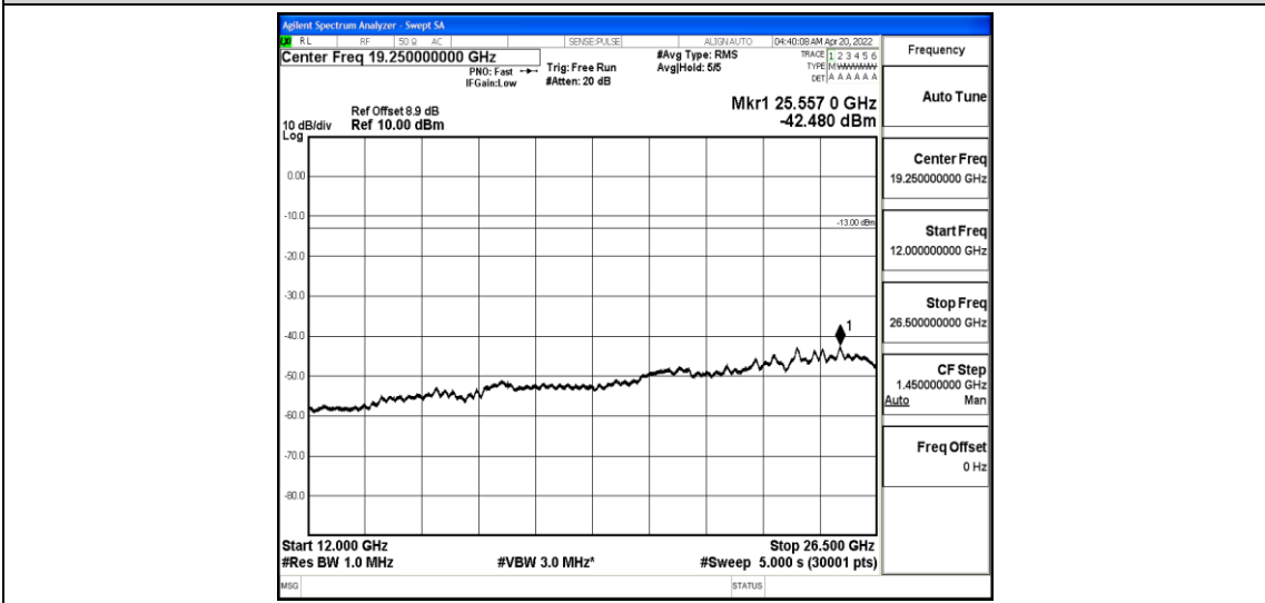
Band25-1.4MHz-16QAM-26365-1-0-Low-12000-26500--42.48-PASS
