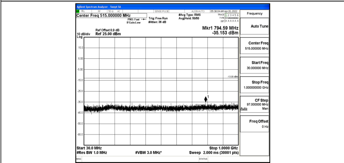
Band25-5MHz-16QAM-26365-1-0-Low-30-1000--35.15-PASS
