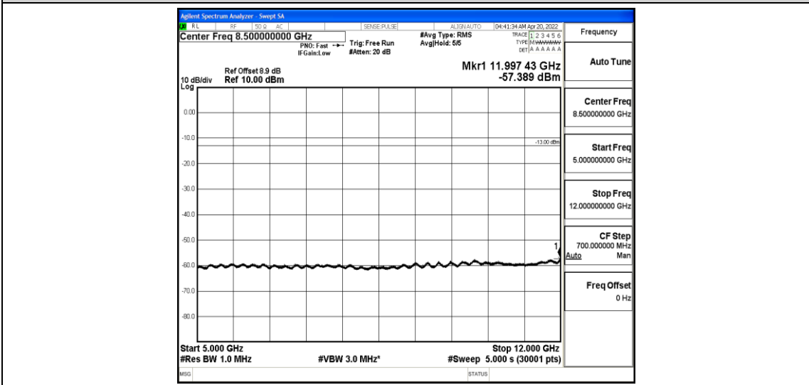
Band25-1.4MHz-QPSK-26683-1-0-High-5000-12000--57.39-PASS
