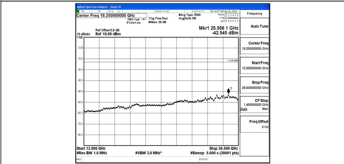
Band25-10MHz-QPSK-26365-1-0-Low-12000-26500--42.55-PASS
