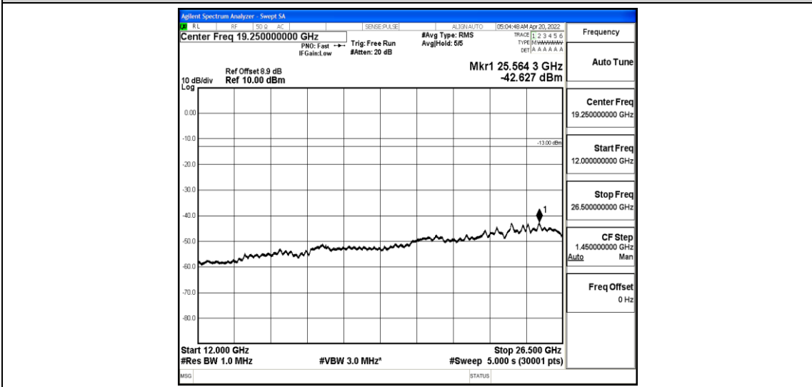
Band25-3MHz-QPSK-26365-1-0-Low-12000-26500--42.63-PASS
