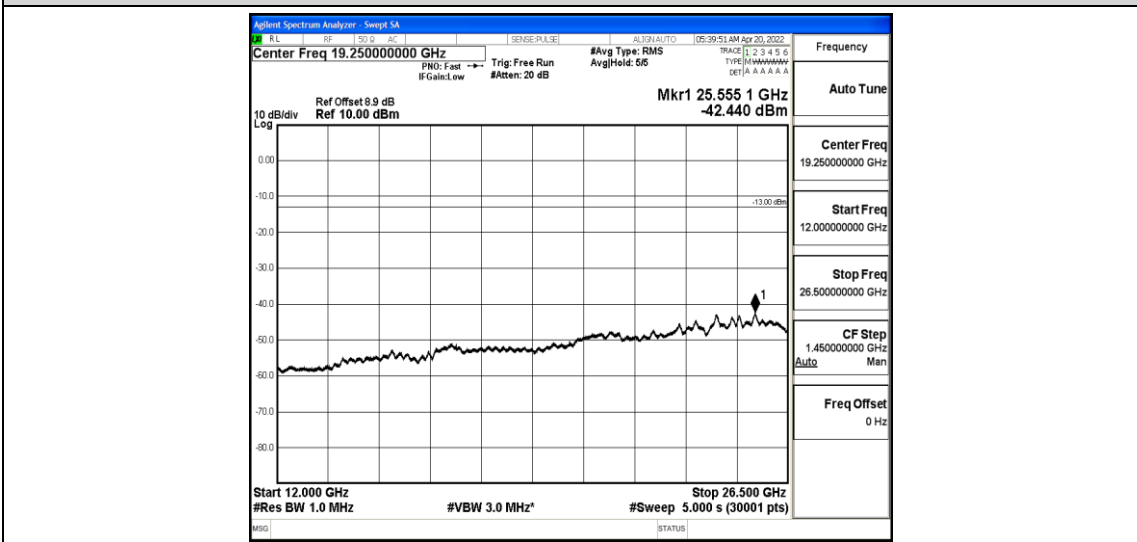
Band25-5MHz-16QAM-26365-1-0-Low-12000-26500--42.44-PASS
