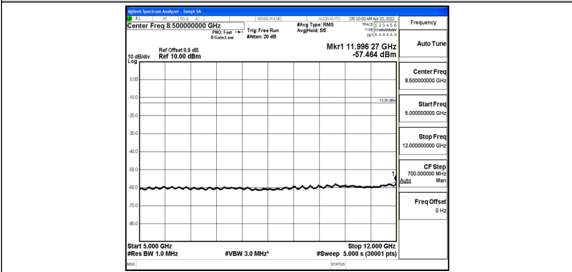
Band25-3MHz-16QAM-26675-1-0-High-5000-12000--57.46-PASS
