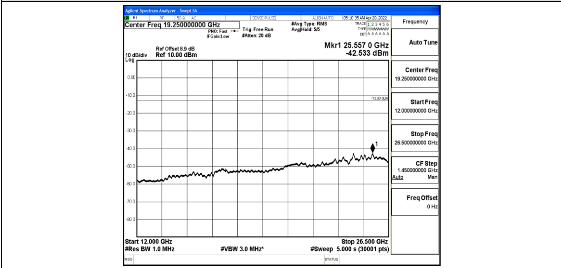
Band25-3MHz-16QAM-26675-1-0-High-12000-26500--42.53-PASS
