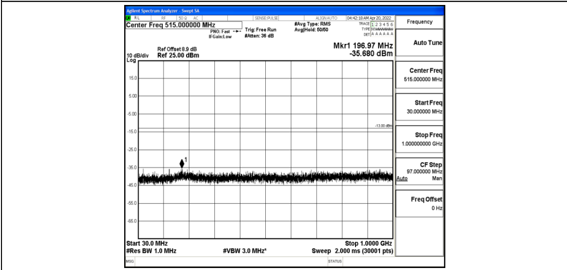
Band25-1.4MHz-16QAM-26683-1-0-High-30-1000--35.68-PASS
