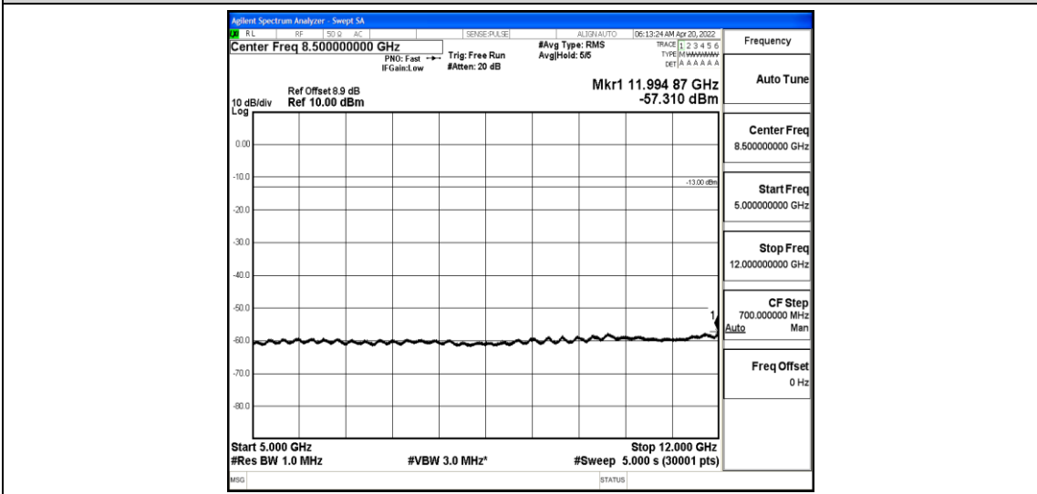
Band25-10MHz-QPSK-26640-1-0-High-5000-12000--57.31-PASS
