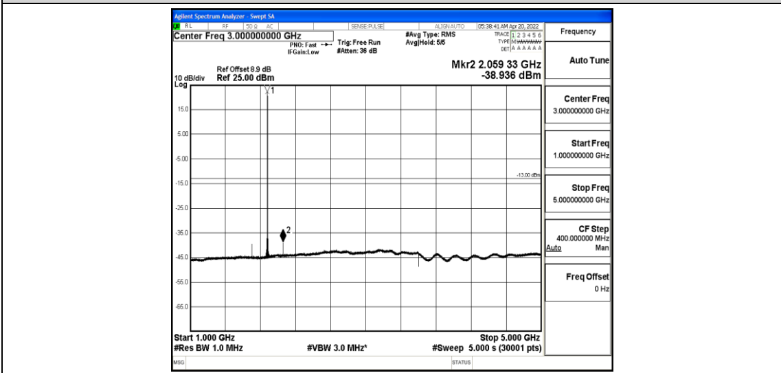
Band25-5MHz-16QAM-26365-1-0-Low-1000-5000--38.94-PASS
