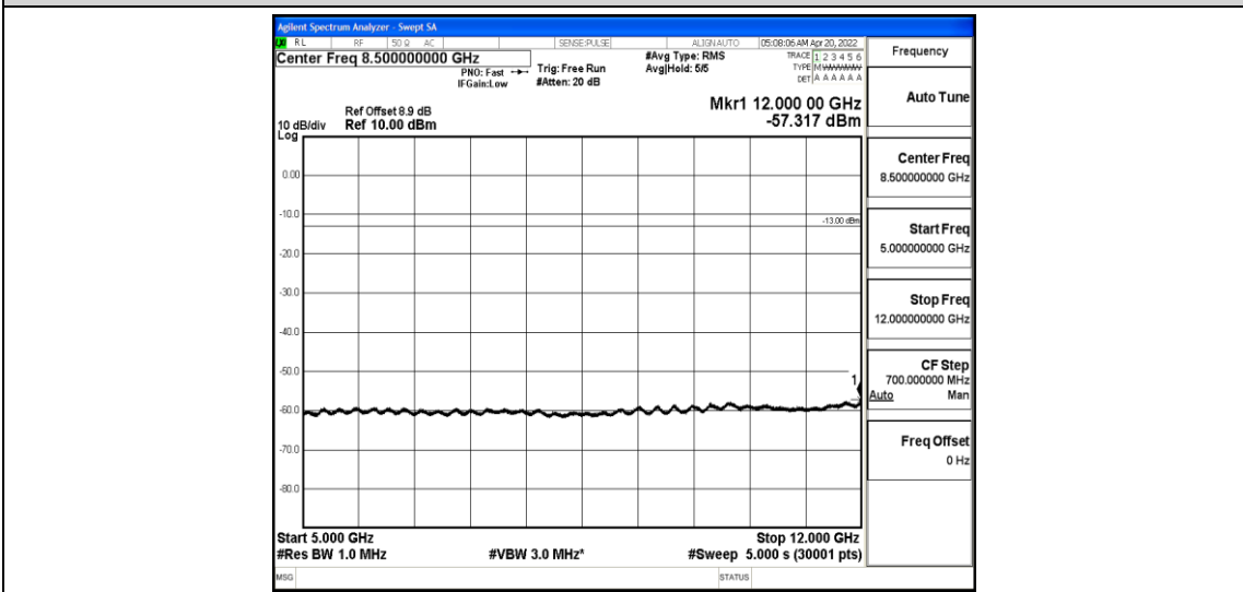
Band25-3MHz-QPSK-26675-1-0-High-5000-12000--57.32-PASS
