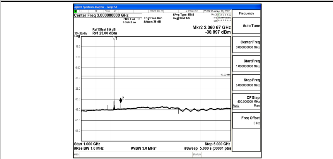
Band25-3MHz-16QAM-26365-1-0-Low-1000-5000--38.9-PASS
