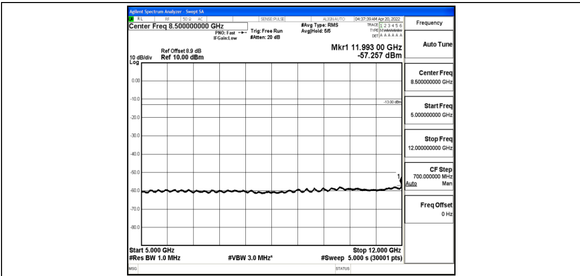
Band25-1.4MHz-QPSK-26365-1-0-Low-5000-12000--57.26-PASS
