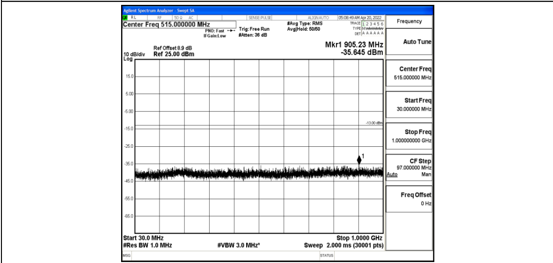
Band25-3MHz-16QAM-26675-1-0-High-30-1000--35.65-PASS
