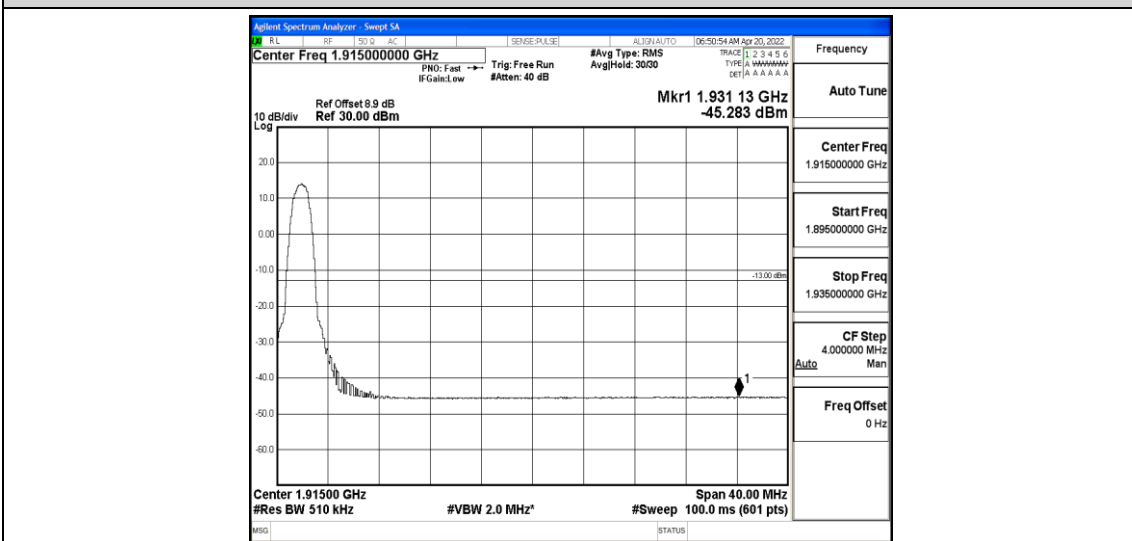
Band25-20MHz-16QAM-26590-6-0-Low--45.28-PASS
