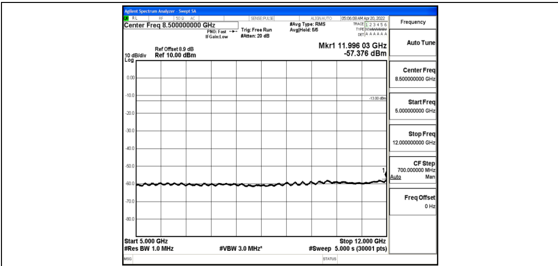
Band25-3MHz-16QAM-26365-1-0-Low-5000-12000--57.38-PASS
