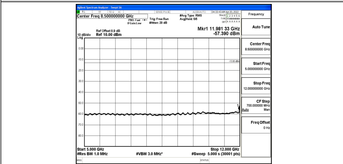
Band25-1.4MHz-QPSK-26047-1-0-Low-5000-12000--57.39-PASS
