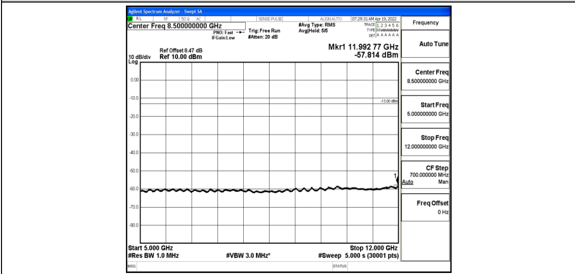
Band4-5MHz-16QAM-20375-1-0-High-5000-12000--57.81-PASS
