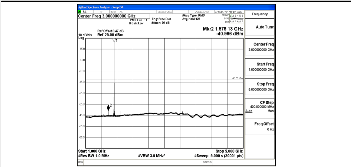
Band4-10MHz-QPSK-20175-1-0-Low-1000-5000--40.99-PASS
