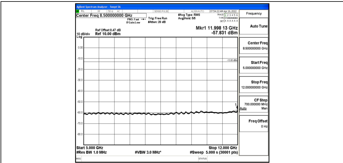
Band4-10MHz-QPSK-20175-1-0-Low-5000-12000--57.83-PASS
