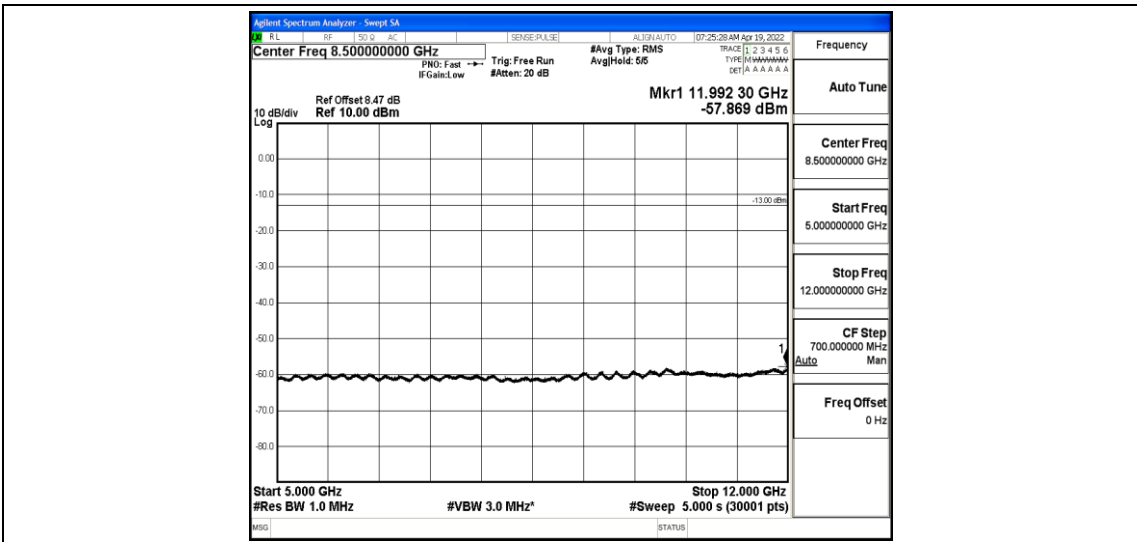
Band4-5MHz-16QAM-20175-1-0-Low-5000-12000--57.87-PASS
