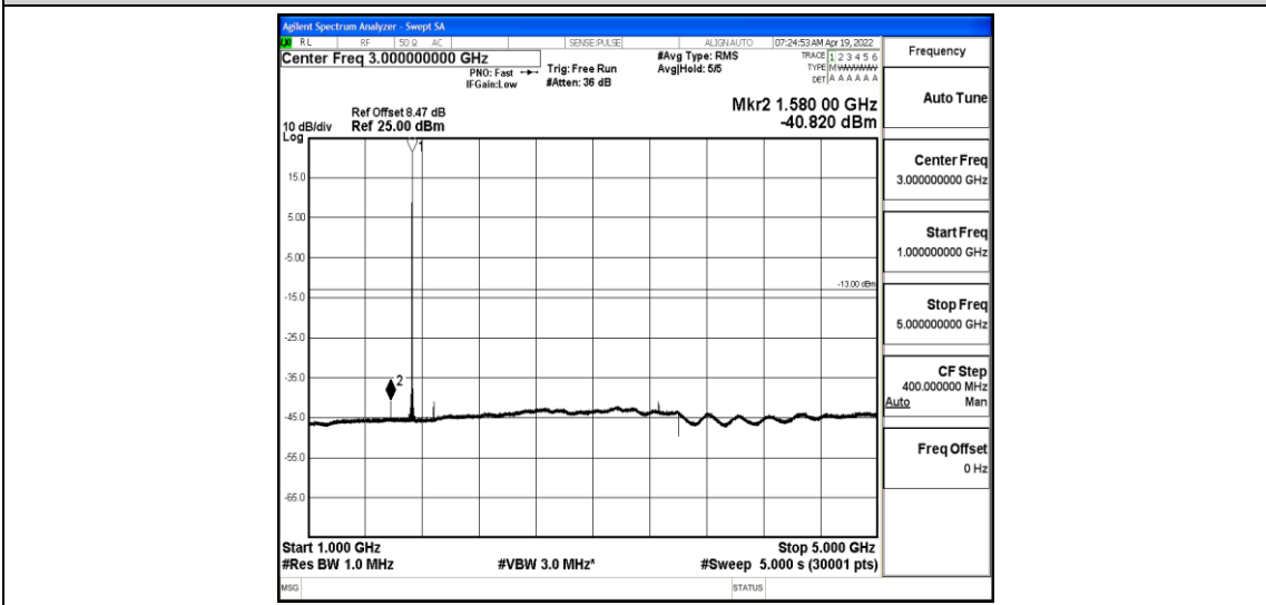
Band4-5MHz-16QAM-20175-1-0-Low-1000-5000--40.82-PASS
