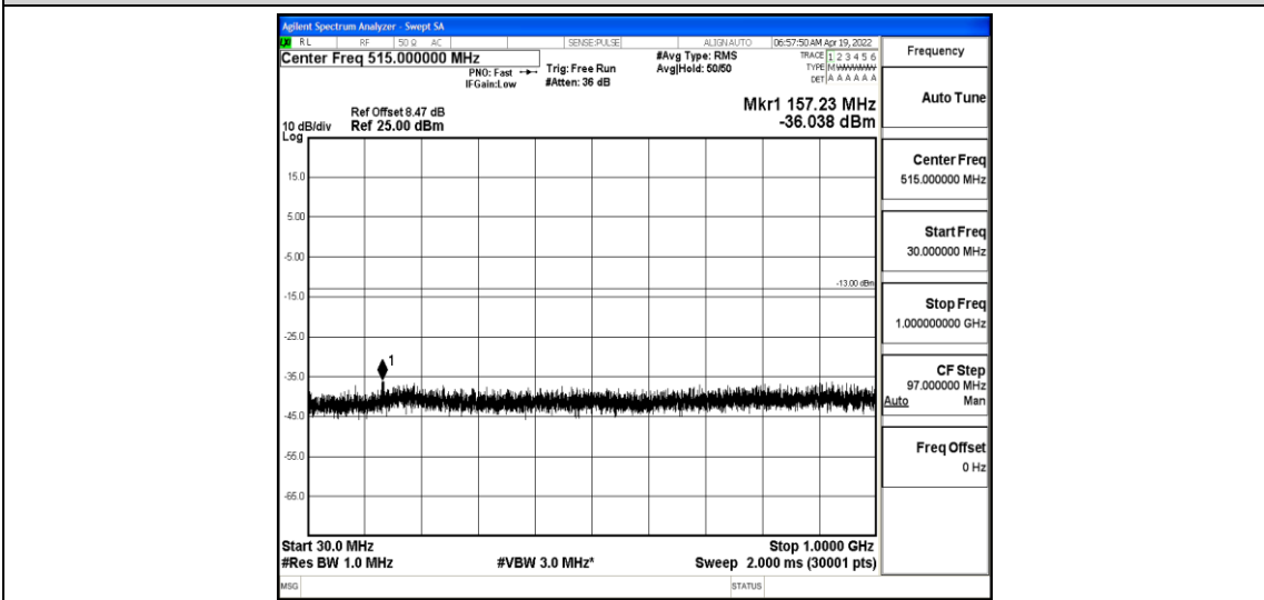
Band4-3MHz-QPSK-20385-1-0-High-30-1000--36.04-PASS
