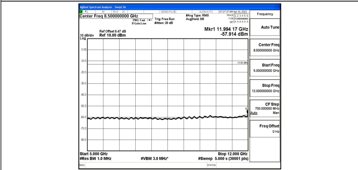
Band4-5MHz-QPSK-20375-1-0-High-5000-12000--57.91-PASS
