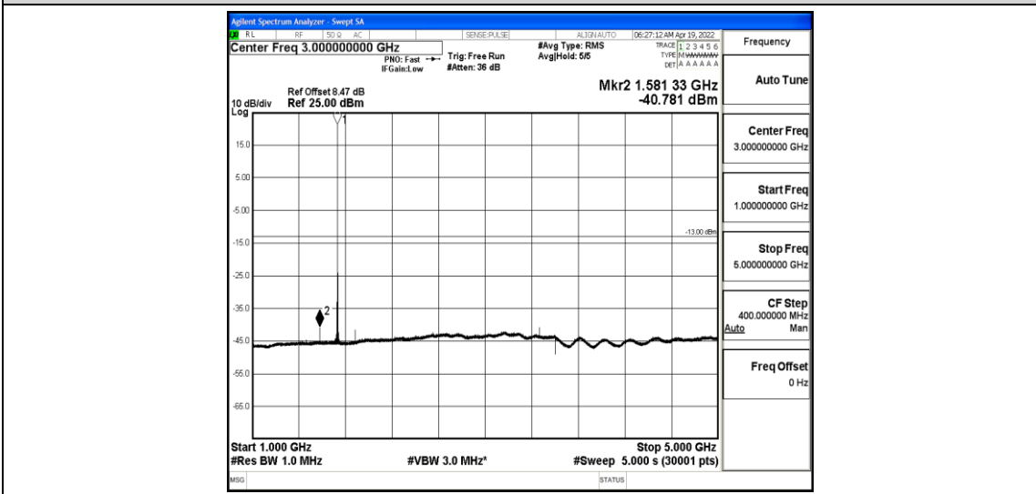
Band4-1.4MHz-QPSK-20175-1-0-Low-1000-5000--40.78-PASS
