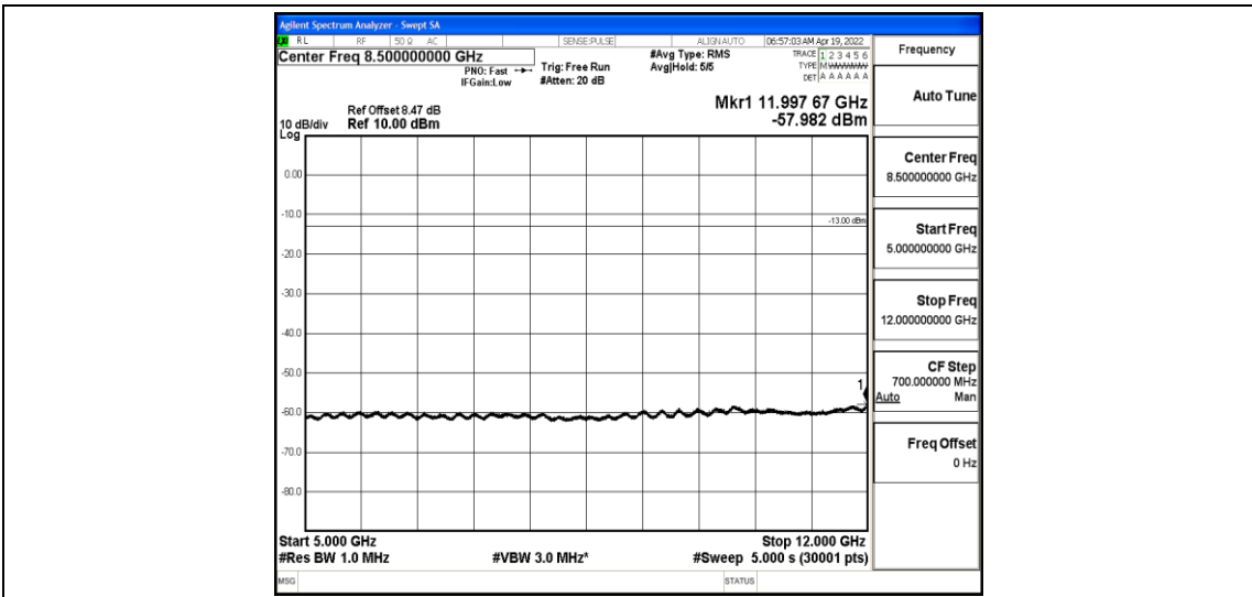
Band4-3MHz-16QAM-20175-1-0-Low-5000-12000--57.98-PASS
