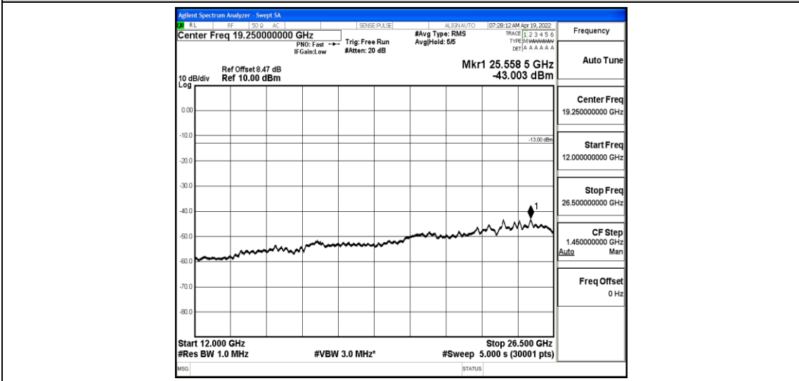
Band4-5MHz-QPSK-20375-1-0-High-12000-26500--43-PASS
