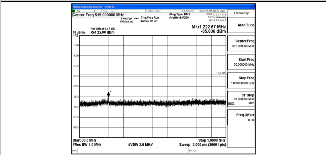
Band4-3MHz-16QAM-20385-1-0-High-30-1000--35.61-PASS
