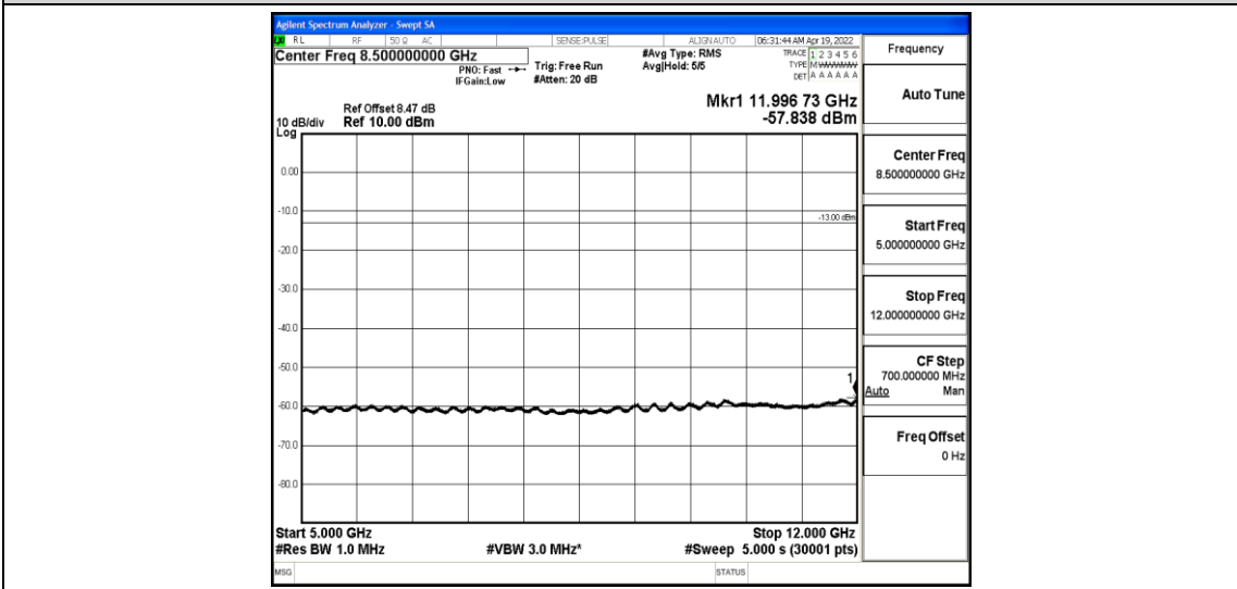
Band4-1.4MHz-QPSK-20393-1-0-High-5000-12000--57.84-PASS
