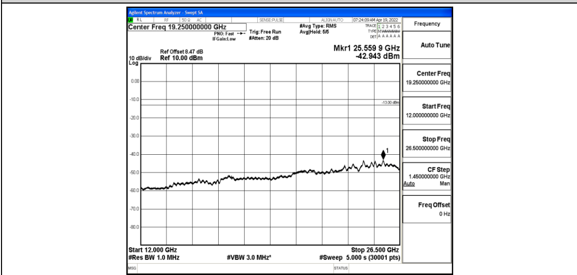
Band4-5MHz-QPSK-20175-1-0-Low-12000-26500--42.94-PASS
