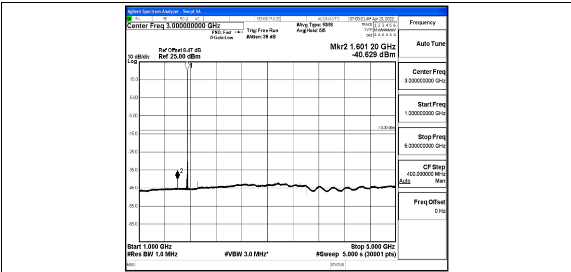
Band4-3MHz-16QAM-20385-1-0-High-1000-5000--40.63-PASS
