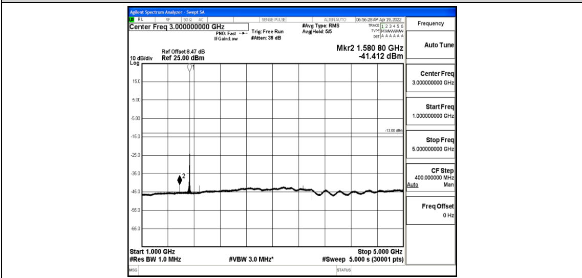
Band4-3MHz-16QAM-20175-1-0-Low-1000-5000--41.41-PASS
