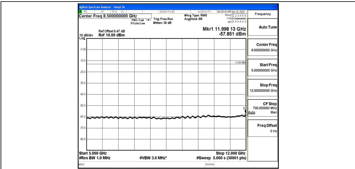
Band4-1.4MHz-16QAM-20175-1-0-Low-5000-12000--57.85-PASS
