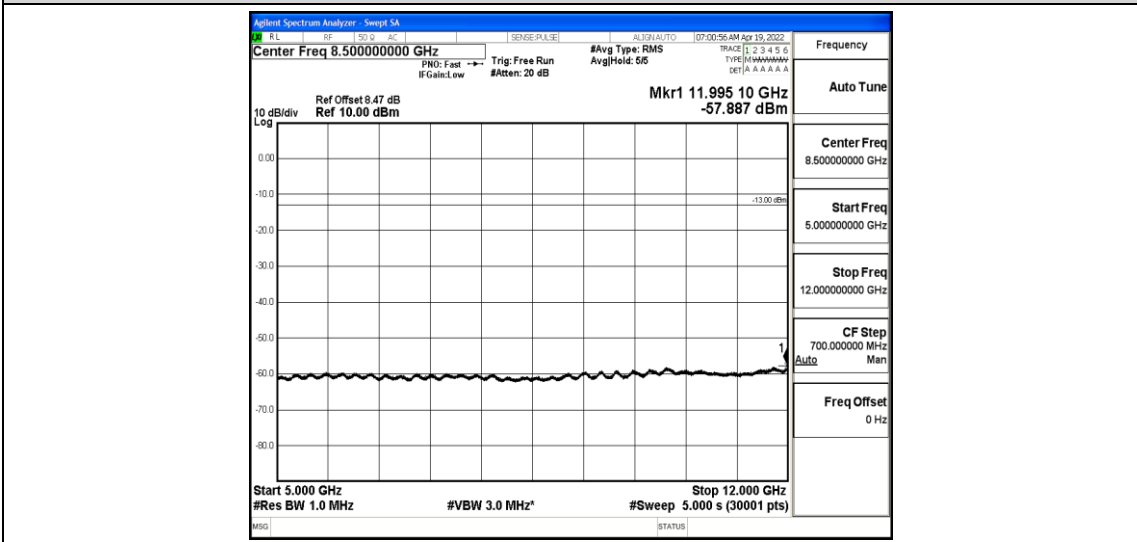
Band4-3MHz-16QAM-20385-1-0-High-5000-12000--57.89-PASS
