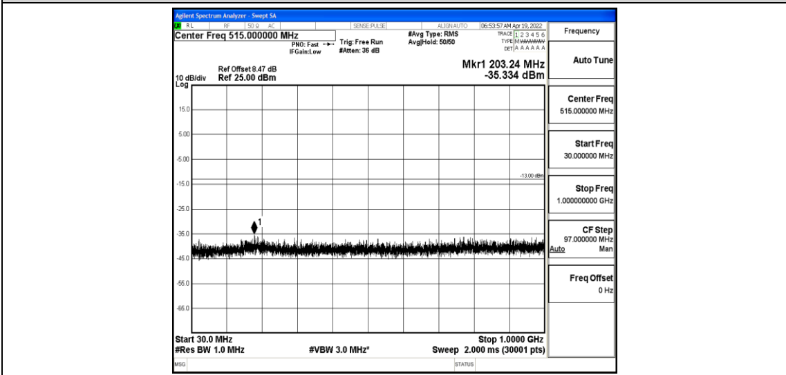
Band4-3MHz-QPSK-20175-1-0-Low-30-1000--35.33-PASS
