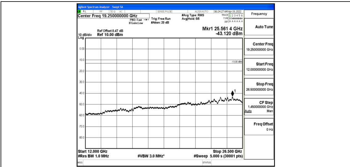
Band4-1.4MHz-QPSK-19957-1-0-Low-12000-26500--43.12-PASS
