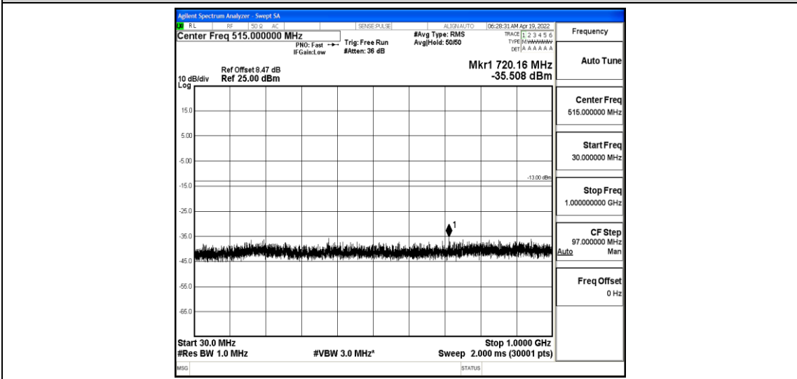
Band4-1.4MHz-16QAM-20175-1-0-Low-30-1000--35.51-PASS
