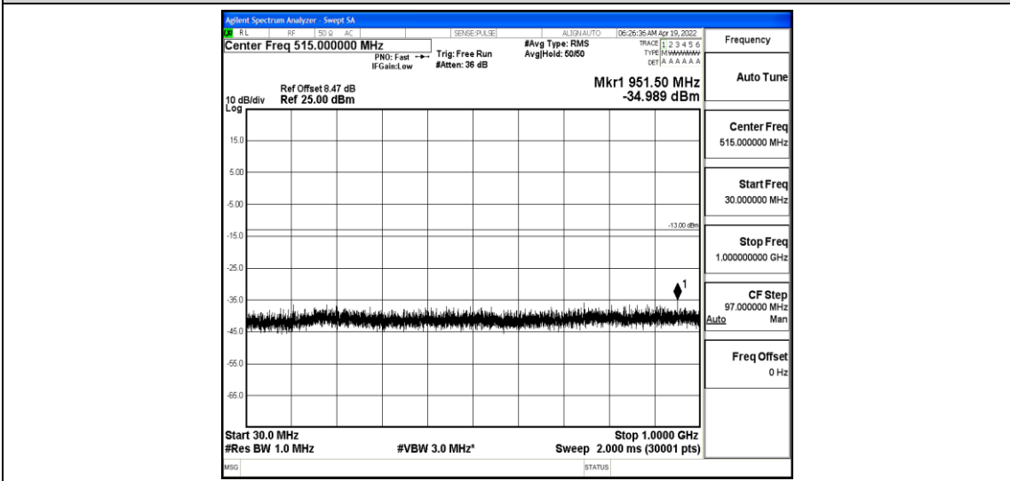
Band4-1.4MHz-QPSK-20175-1-0-Low-30-1000--34.99-PASS
