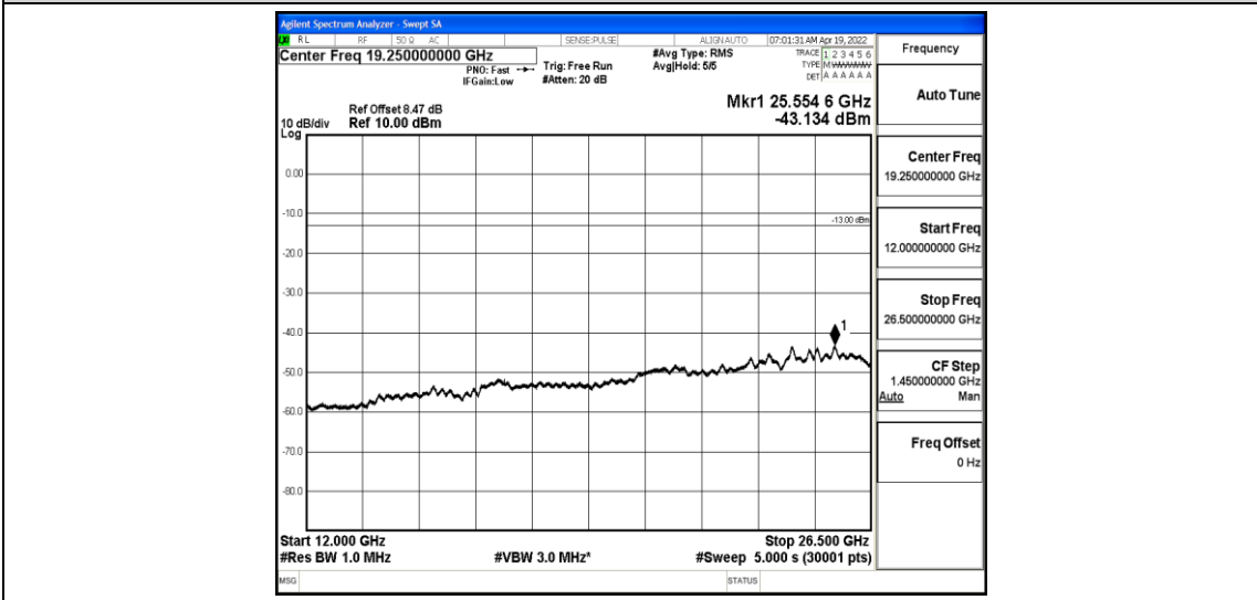
Band4-3MHz-16QAM-20385-1-0-High-12000-26500--43.13-PASS
