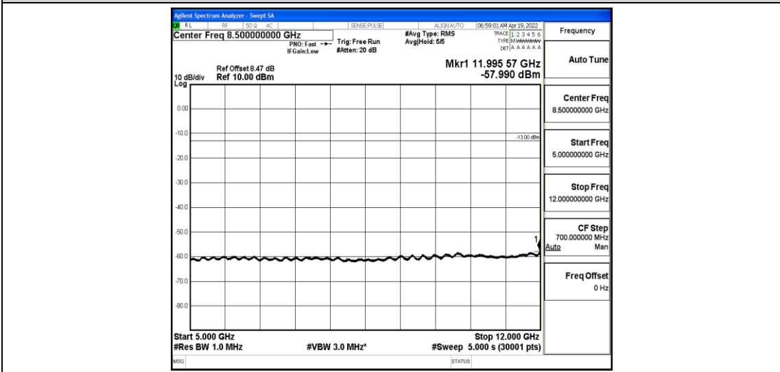
Band4-3MHz-QPSK-20385-1-0-High-5000-12000--57.99-PASS
