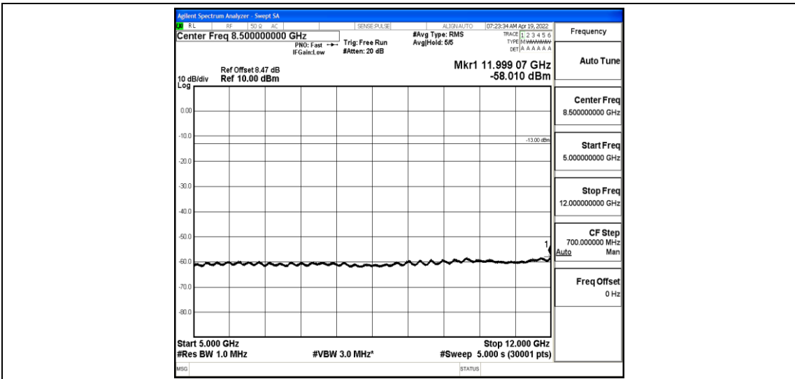
Band4-5MHz-QPSK-20175-1-0-Low-5000-12000--58.01-PASS
