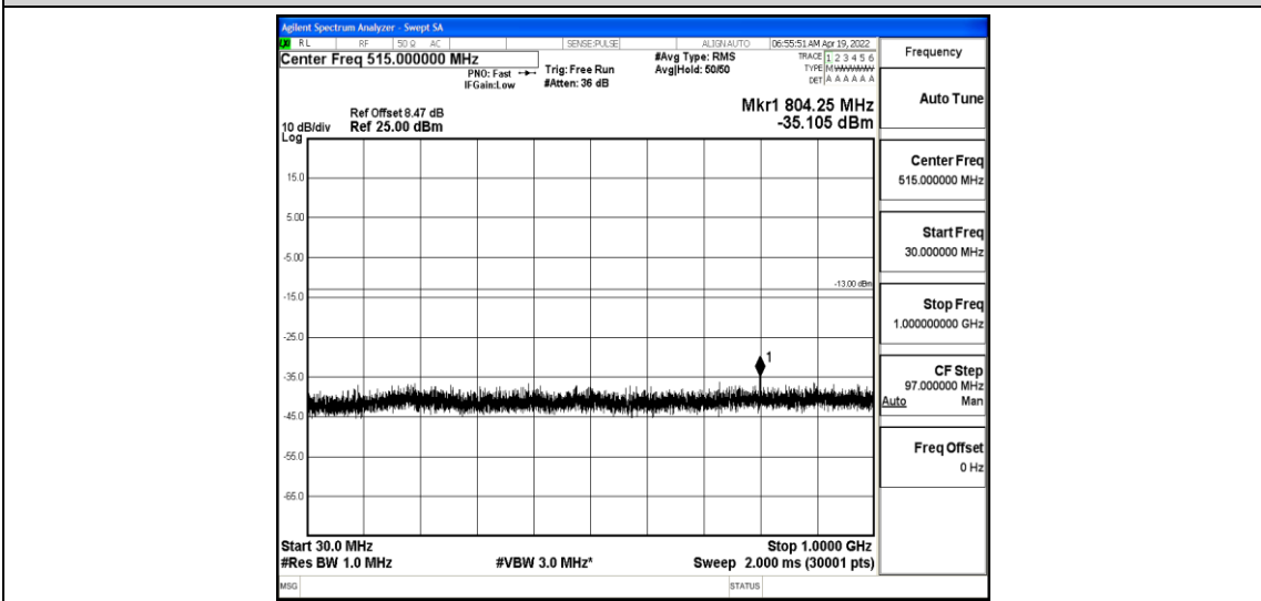
Band4-3MHz-16QAM-20175-1-0-Low-30-1000--35.11-PASS
