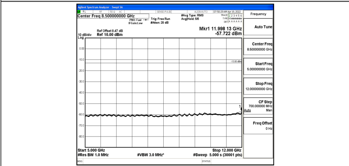
Band4-10MHz-QPSK-20000-1-0-Low-5000-12000--57.72-PASS
