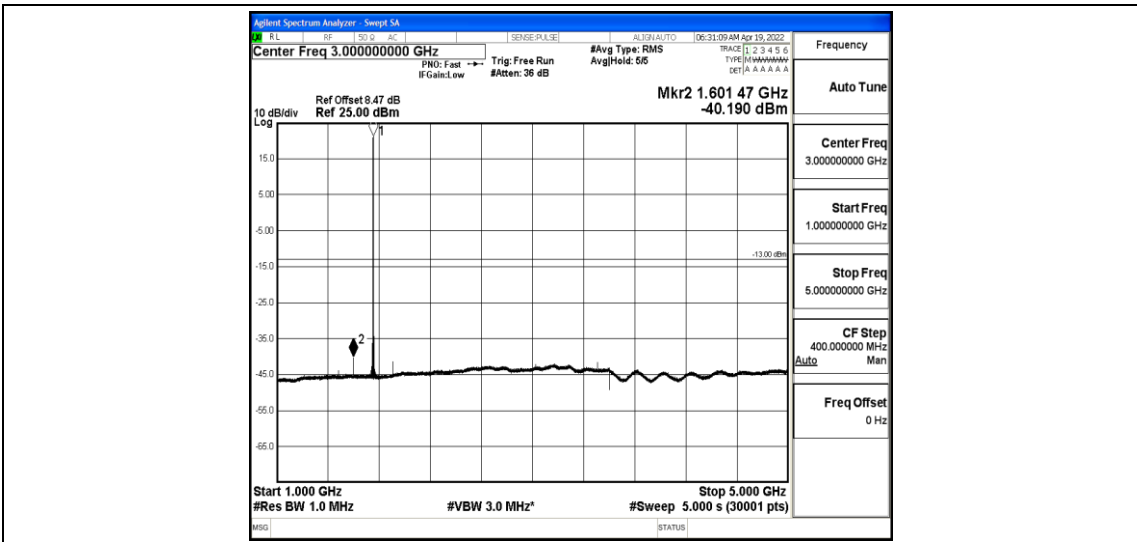
Band4-1.4MHz-QPSK-20393-1-0-High-1000-5000--40.19-PASS
