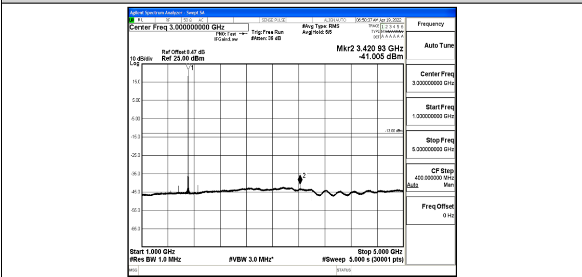
Band4-3MHz-QPSK-19965-1-0-Low-1000-5000--41.01-PASS
