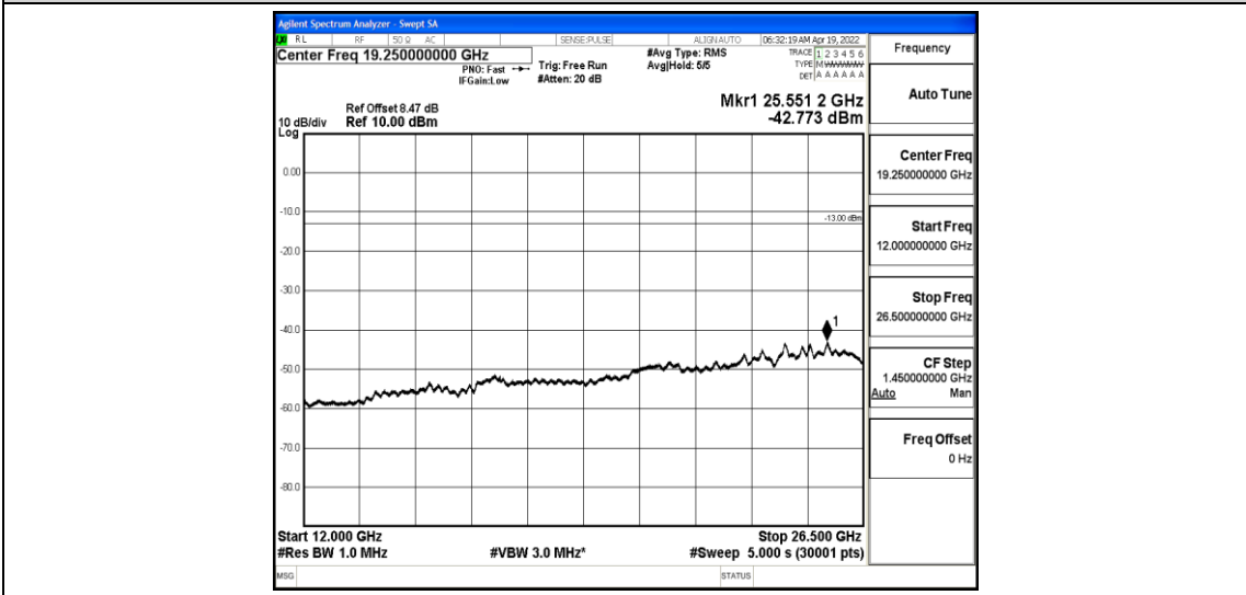
Band4-1.4MHz-QPSK-20393-1-0-High-12000-26500--42.77-PASS
