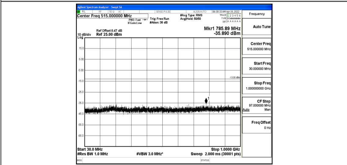
Band4-1.4MHz-QPSK-20393-1-0-High-30-1000--35.89-PASS
