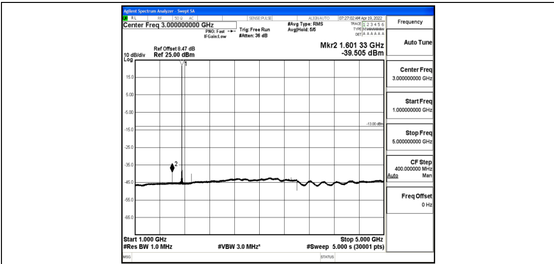
Band4-5MHz-QPSK-20375-1-0-High-1000-5000--39.51-PASS
