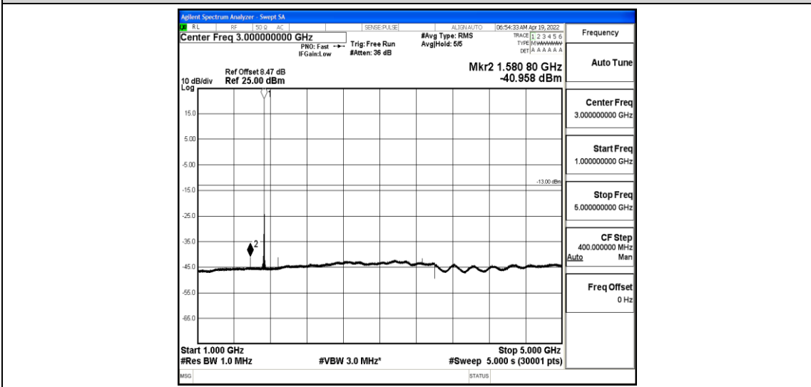
Band4-3MHz-QPSK-20175-1-0-Low-1000-5000--40.96-PASS
