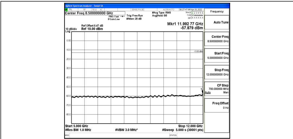
Band4-1.4MHz-QPSK-20175-1-0-Low-5000-12000--57.88-PASS
