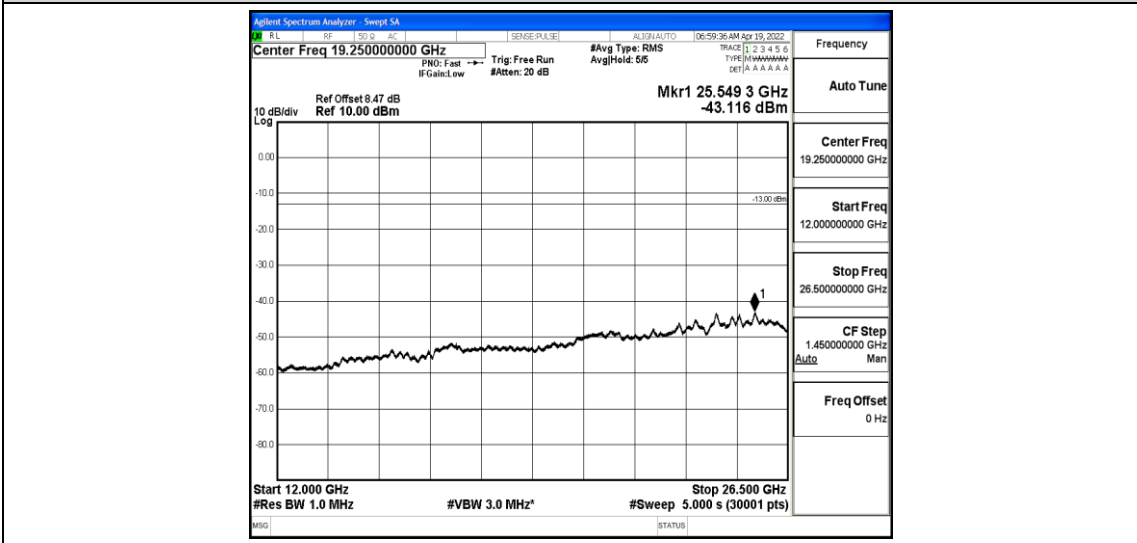
Band4-3MHz-QPSK-20385-1-0-High-12000-26500--43.12-PASS
