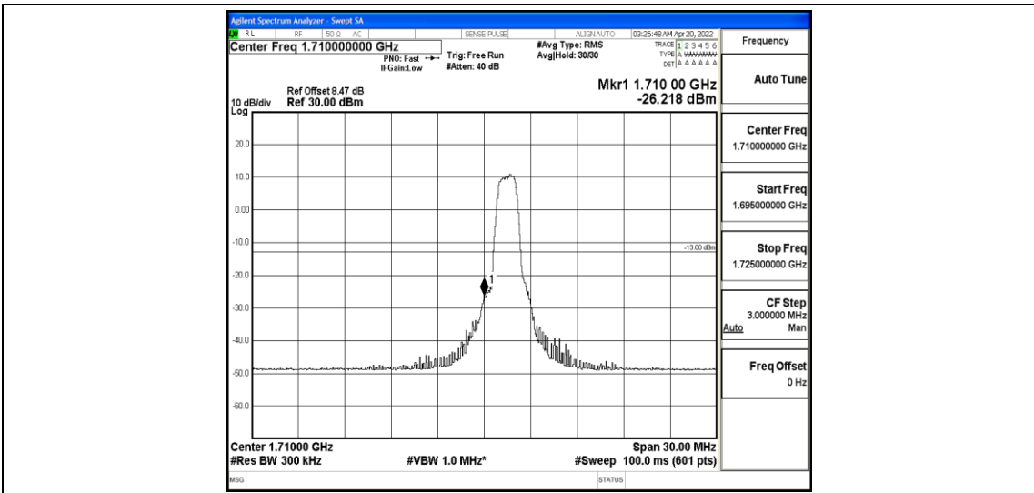
Band4-15MHz-16QAM-20025-6-0-Low--26.22-PASS
