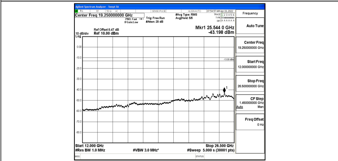
Band4-10MHz-QPSK-20175-1-0-Low-12000-26500--43.2-PASS
