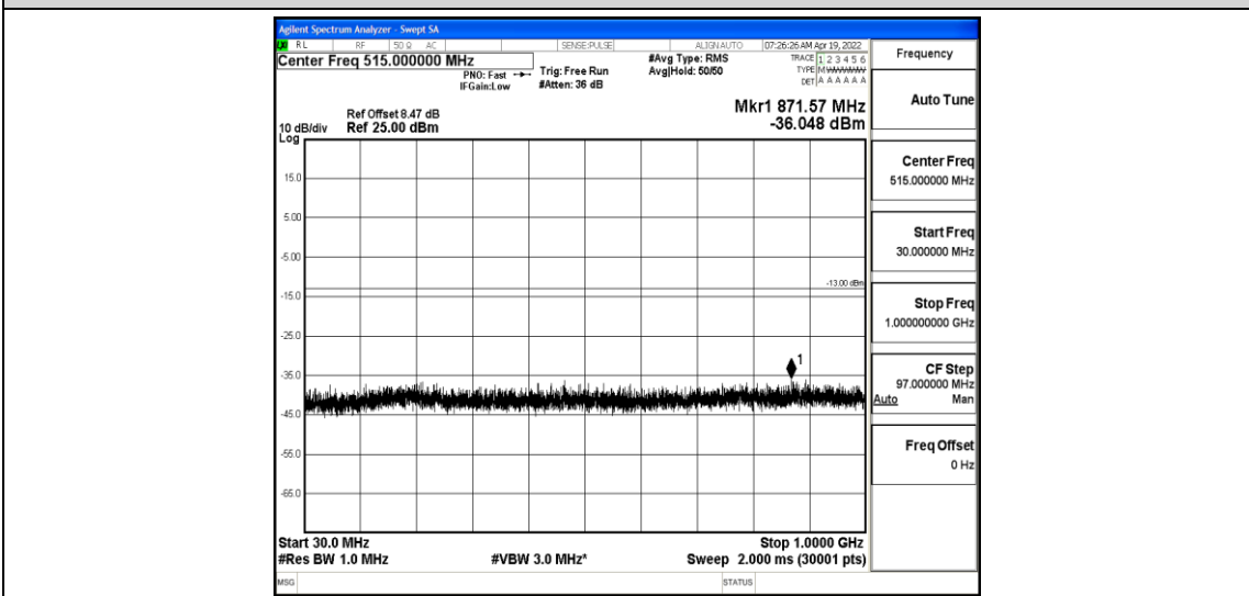
Band4-5MHz-QPSK-20375-1-0-High-30-1000--36.05-PASS
