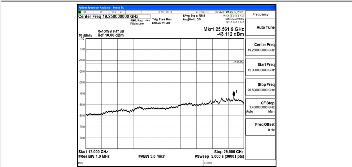
Band4-5MHz-16QAM-20175-1-0-Low-12000-26500--43.11-PASS
