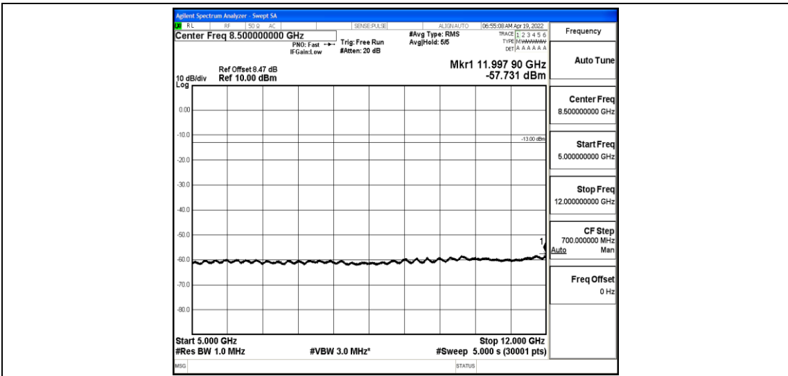
Band4-3MHz-QPSK-20175-1-0-Low-5000-12000--57.73-PASS
