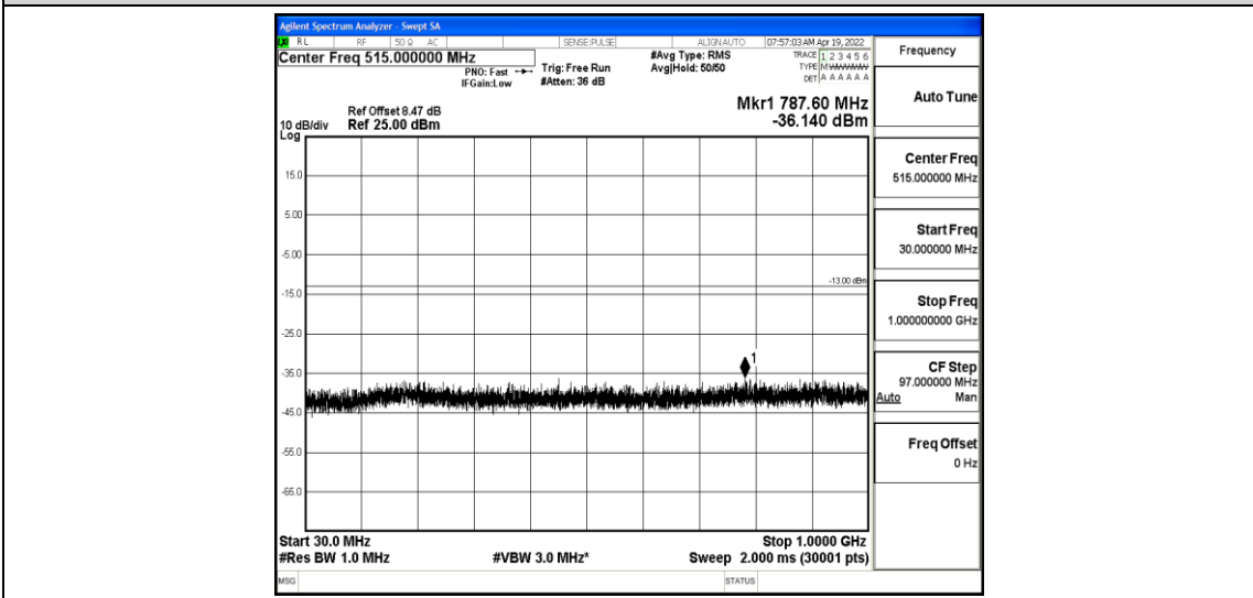
Band4-10MHz-QPSK-20350-1-0-High-30-1000--36.14-PASS
