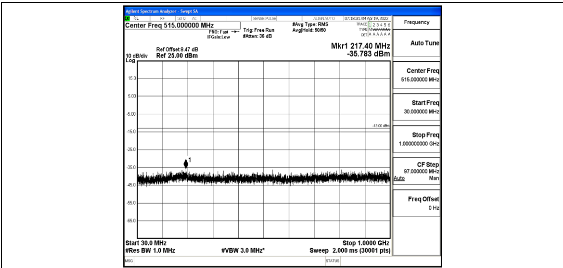
Band4-5MHz-QPSK-19975-1-0-Low-30-1000--35.78-PASS
