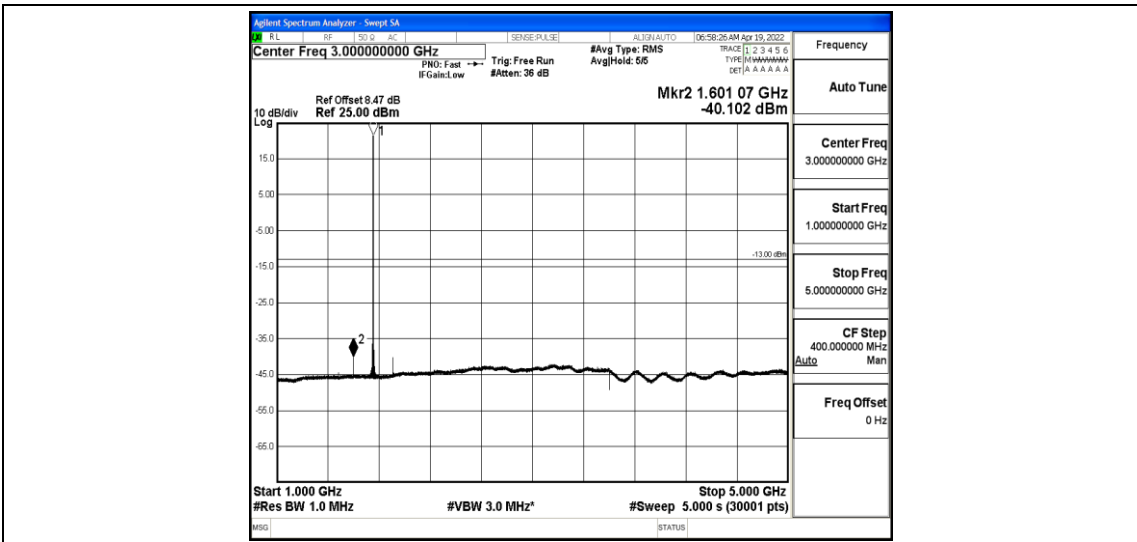
Band4-3MHz-QPSK-20385-1-0-High-1000-5000--40.1-PASS
