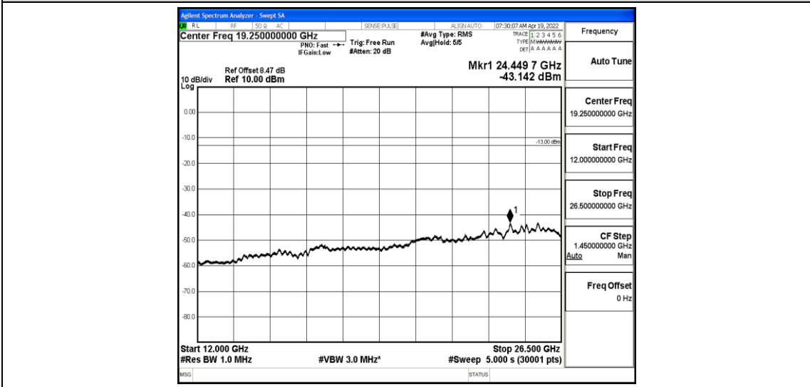
Band4-5MHz-16QAM-20375-1-0-High-12000-26500--43.14-PASS
