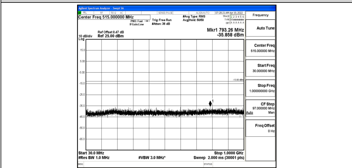
Band4-5MHz-16QAM-20375-1-0-High-30-1000--35.86-PASS
