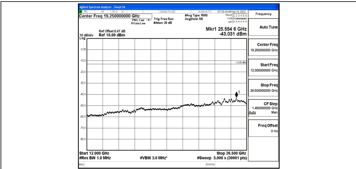
Band4-5MHz-QPSK-19975-1-0-Low-12000-26500--43.03-PASS
