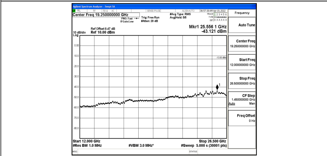
Band4-3MHz-16QAM-20175-1-0-Low-12000-26500--43.12-PASS
