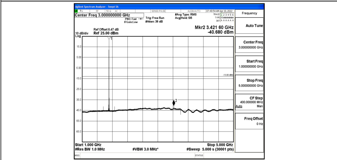
Band4-10MHz-QPSK-20000-1-0-Low-1000-5000--40.68-PASS
