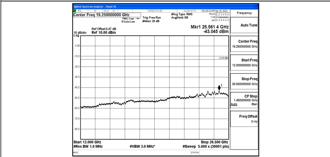
Band4-1.4MHz-QPSK-20175-1-0-Low-12000-26500--43.05-PASS
