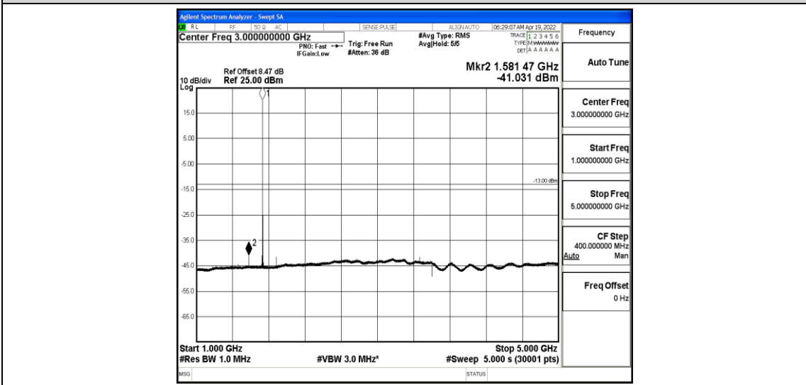
Band4-1.4MHz-16QAM-20175-1-0-Low-1000-5000--41.03-PASS
