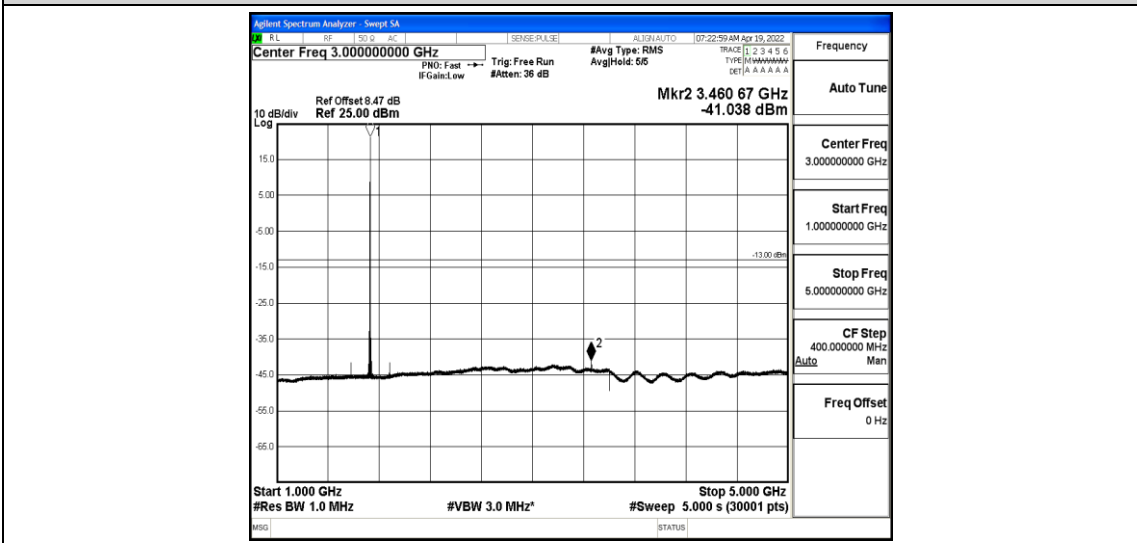
Band4-5MHz-QPSK-20175-1-0-Low-1000-5000--41.04-PASS
