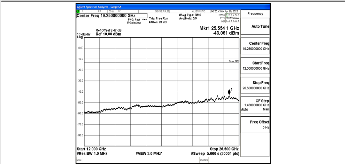
Band4-3MHz-QPSK-20175-1-0-Low-12000-26500--43.06-PASS
