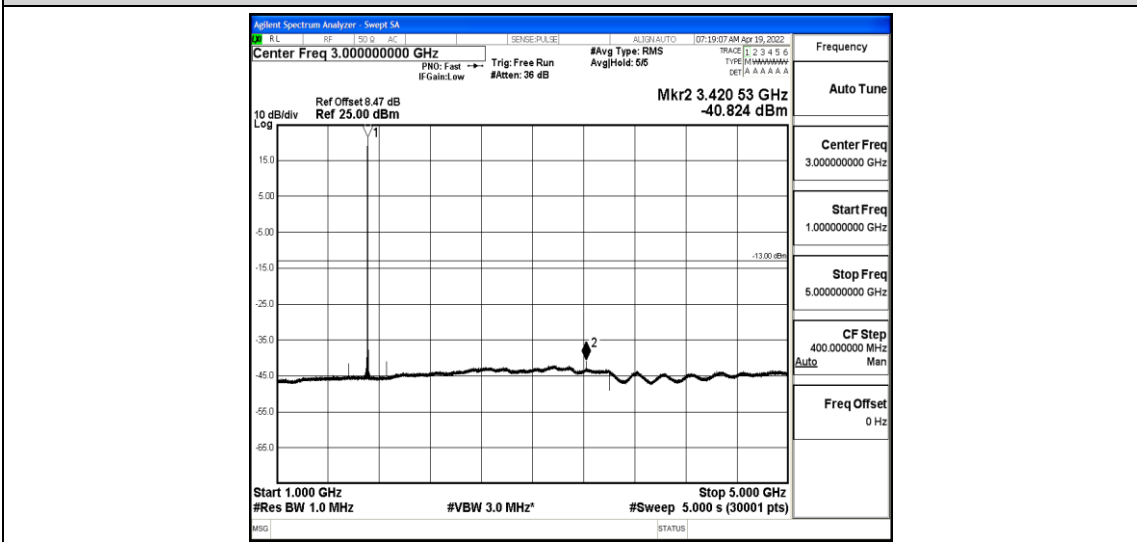
Band4-5MHz-QPSK-19975-1-0-Low-1000-5000--40.82-PASS
