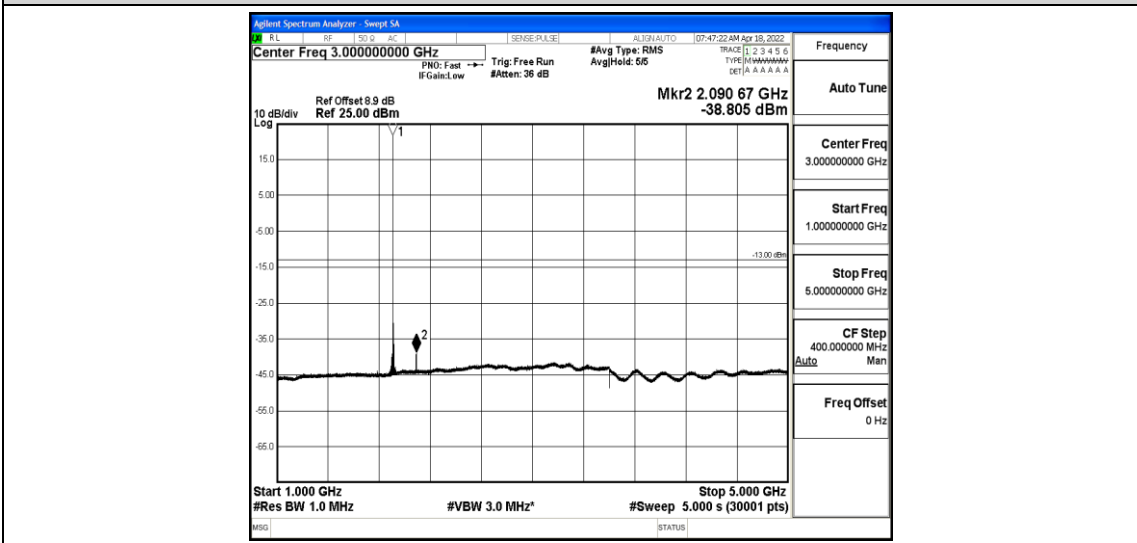
Band2-3MHz-16QAM-19185-1-0-High-1000-5000--38.81-PASS
