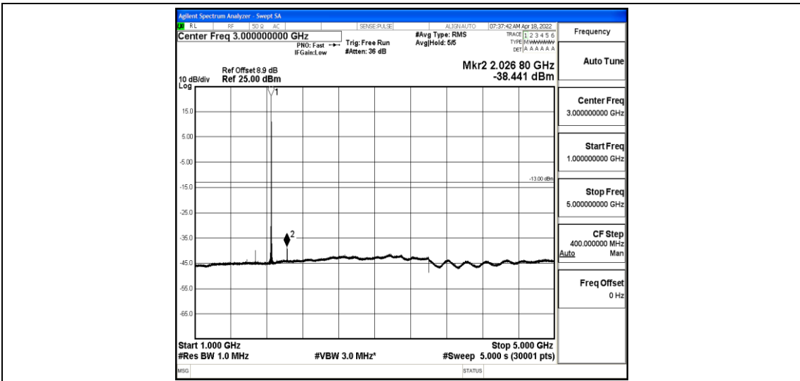
Band2-3MHz-QPSK-18615-1-0-Low-1000-5000--38.44-PASS
