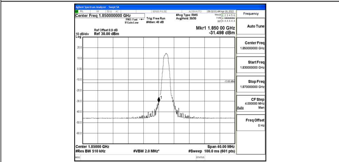
Band2-20MHz-QPSK-18700-6-0-Low--31.50-PASS
