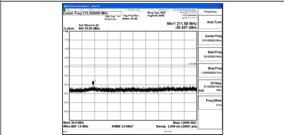
Band2-1.4MHz-QPSK-19193-1-0-High-30-1000--35.56-PASS
