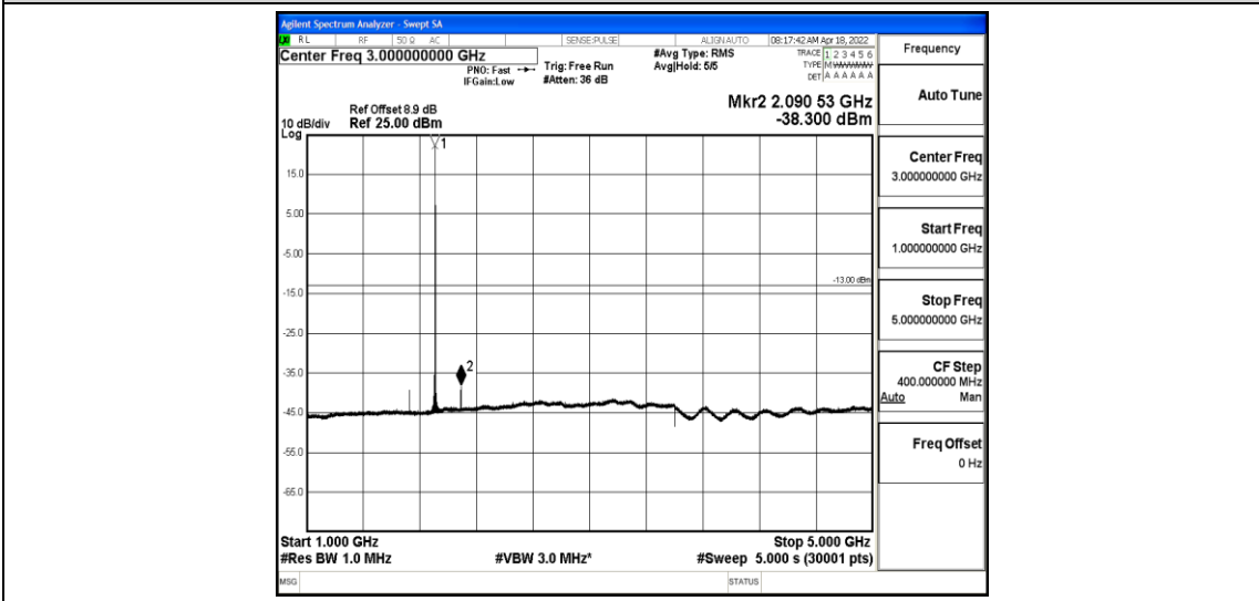
Band2-5MHz-QPSK-19175-1-0-High-1000-5000--38.3-PASS
