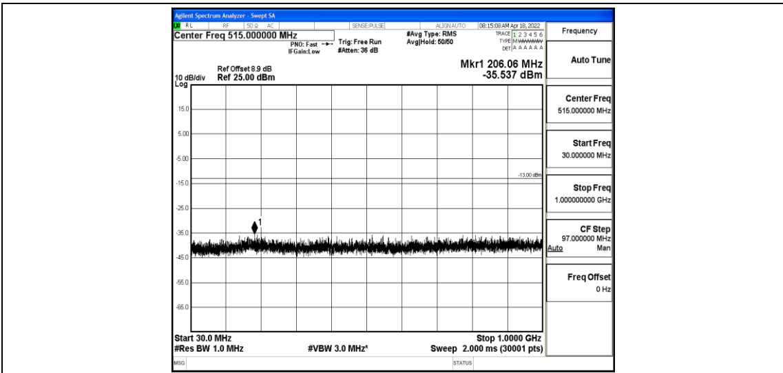
Band2-5MHz-16QAM-18900-1-0-Low-30-1000--35.54-PASS
