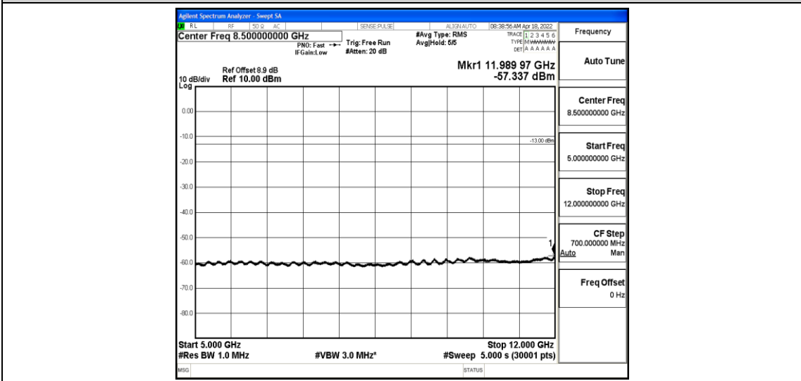
Band2-10MHz-QPSK-18650-1-0-Low-5000-12000--57.34-PASS
