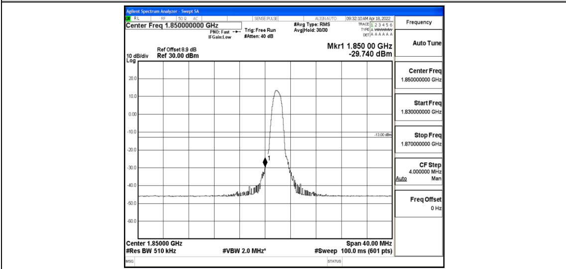
Band2-20MHz-16QAM-18700-6-0-Low--29.74-PASS
