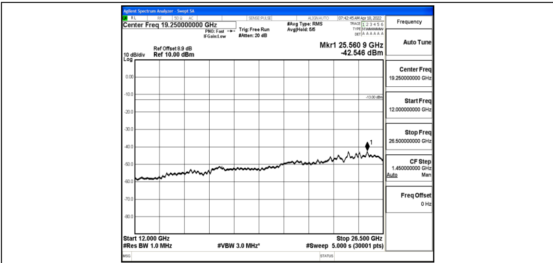
Band2-3MHz-QPSK-18900-1-0-Low-12000-26500--42.55-PASS
