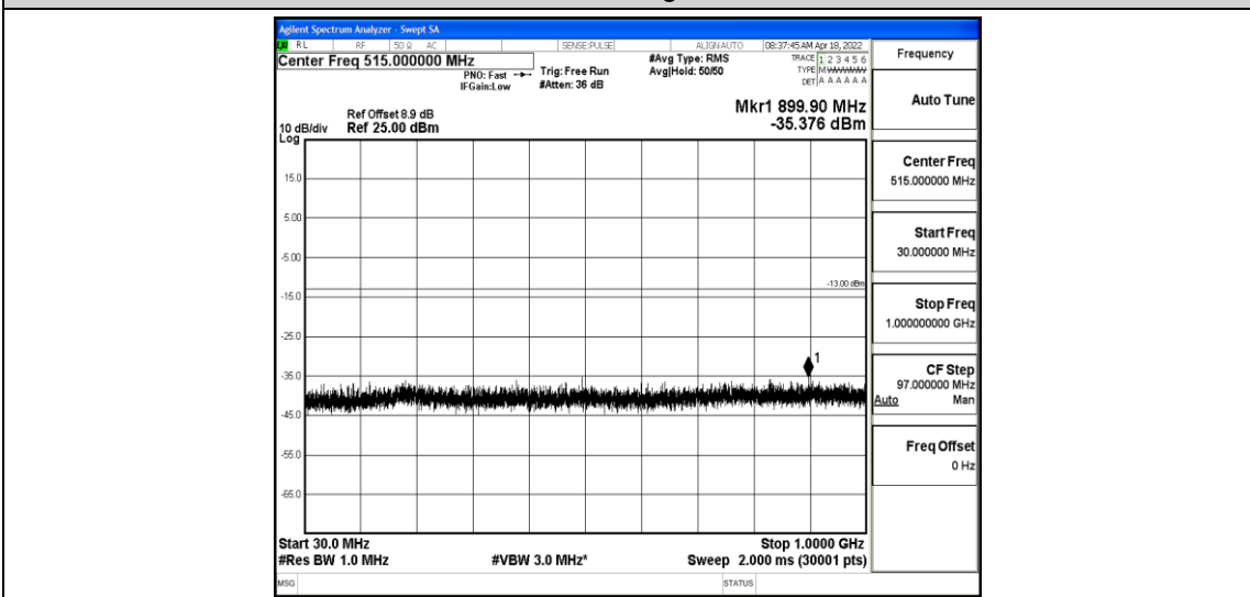
Band2-10MHz-QPSK-18650-1-0-Low-30-1000--35.38-PASS
