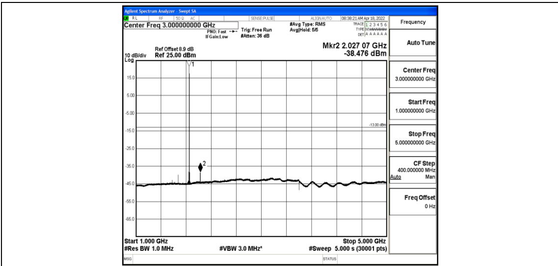
Band2-10MHz-QPSK-18650-1-0-Low-1000-5000--38.48-PASS
