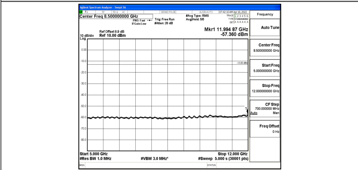
Band2-3MHz-QPSK-18900-1-0-Low-5000-12000--57.36-PASS
