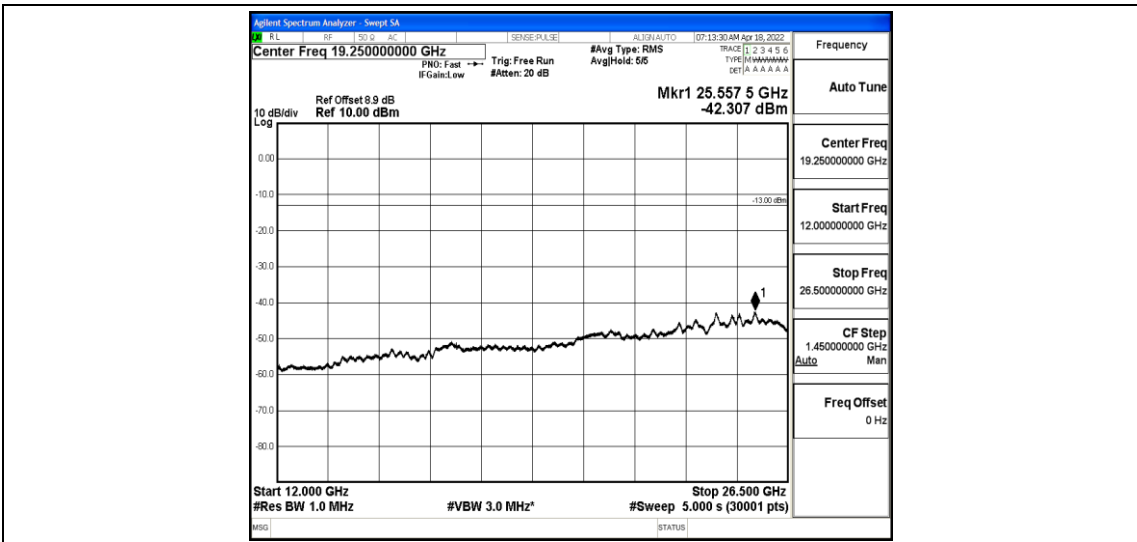
Band2-1.4MHz-QPSK-18900-1-0-Low-12000-26500--42.31-PASS
