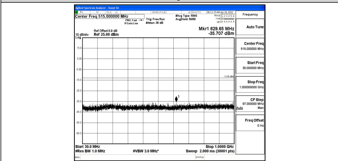
Band2-5MHz-16QAM-18625-1-0-Low-30-1000--35.71-PASS
