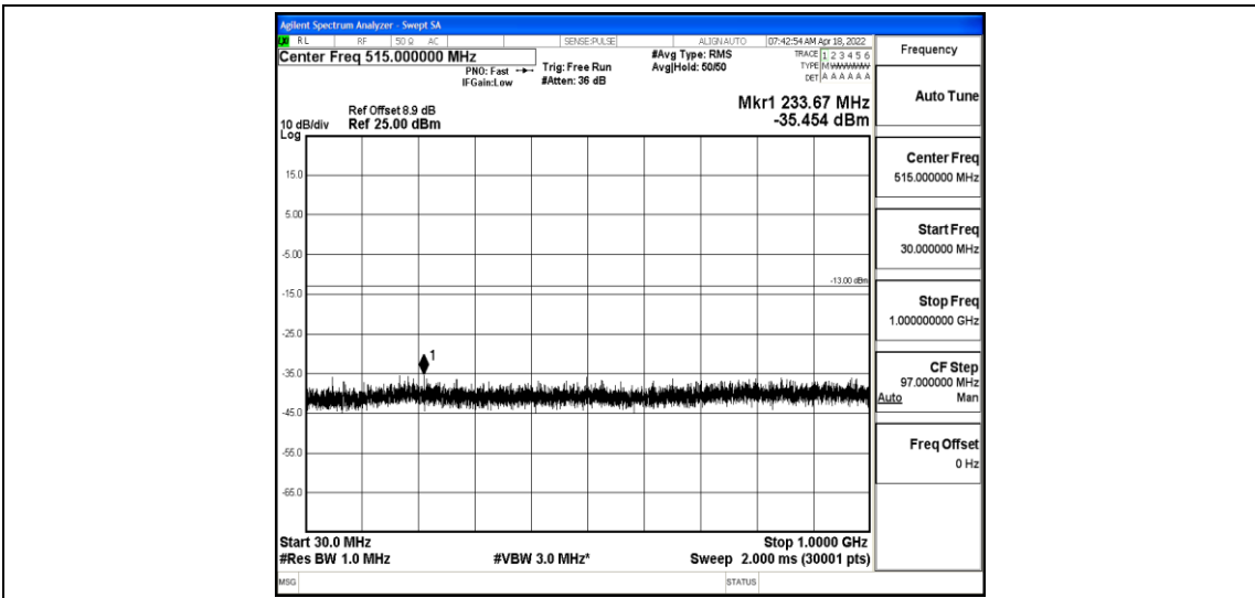
Band2-3MHz-16QAM-18900-1-0-Low-30-1000--35.45-PASS
