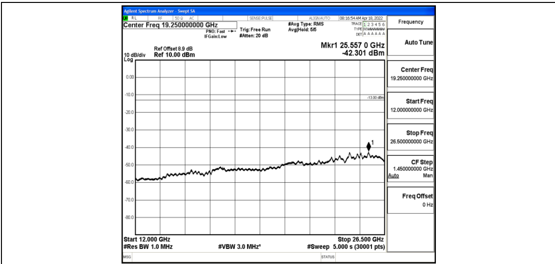
Band2-5MHz-16QAM-18900-1-0-Low-12000-26500--42.3-PASS
