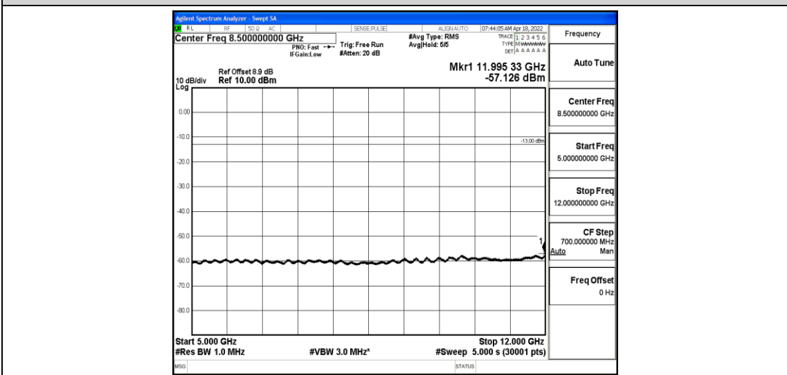
Band2-3MHz-16QAM-18900-1-0-Low-5000-12000--57.13-PASS
