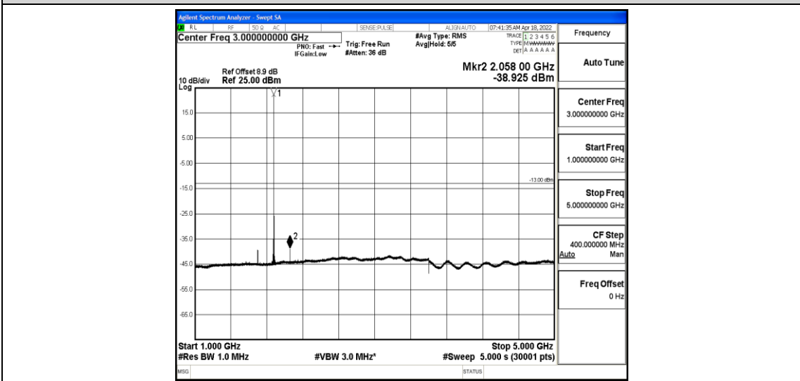
Band2-3MHz-QPSK-18900-1-0-Low-1000-5000--38.93-PASS
