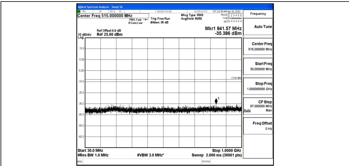
Band2-1.4MHz-16QAM-18900-1-0-Low-30-1000--35.39-PASS
