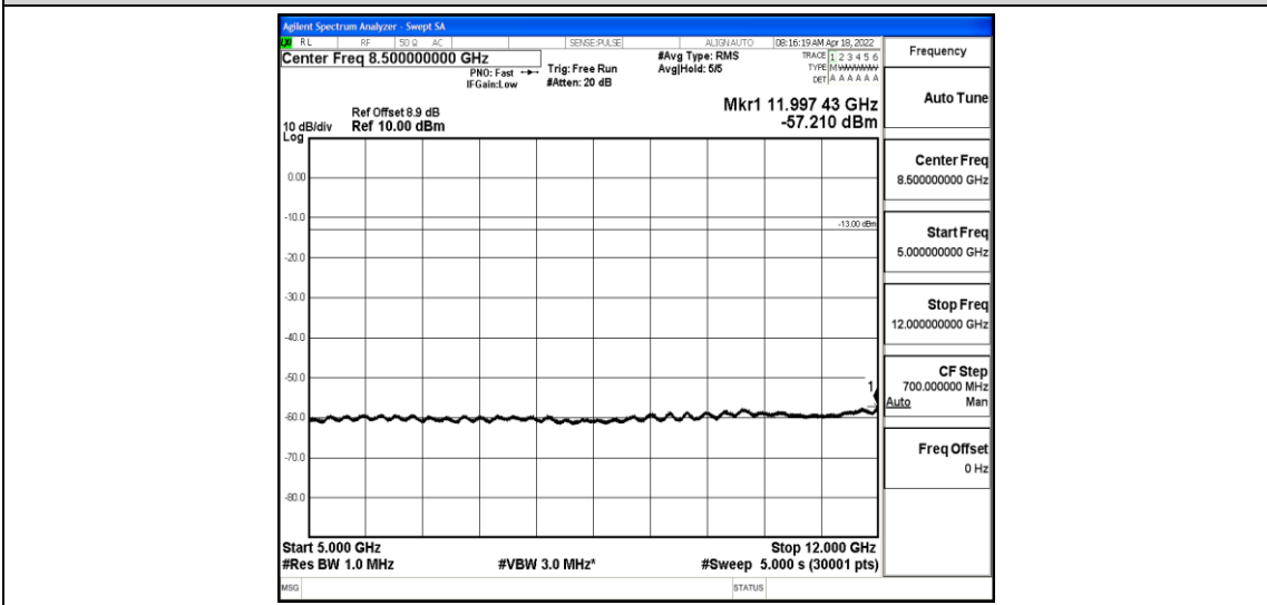
Band2-5MHz-16QAM-18900-1-0-Low-5000-12000--57.21-PASS
