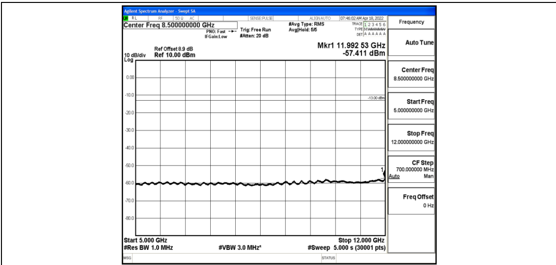
Band2-3MHz-QPSK-19185-1-0-High-5000-12000--57.41-PASS
