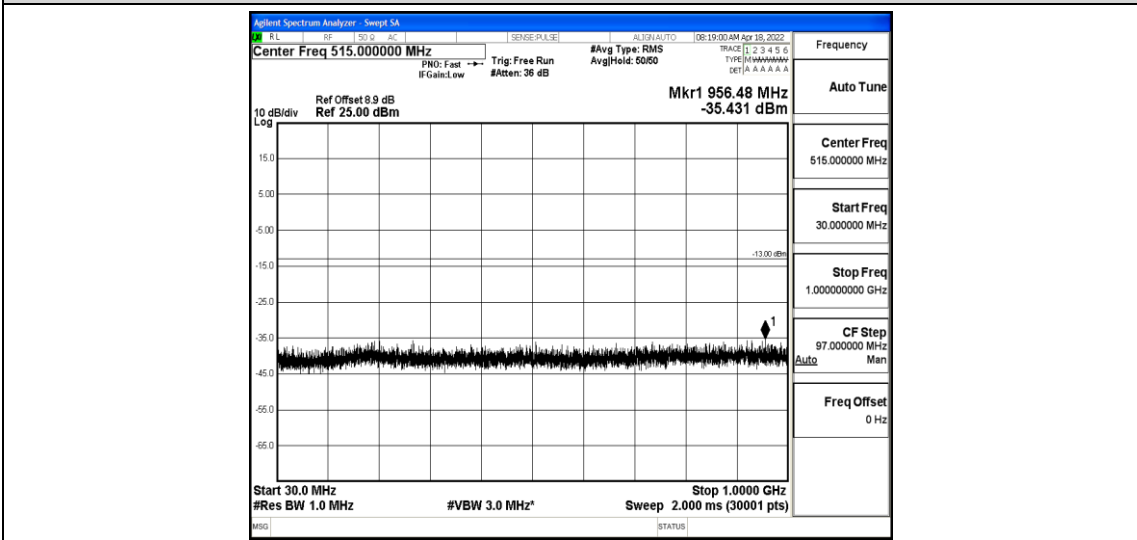
Band2-5MHz-16QAM-19175-1-0-High-30-1000--35.43-PASS
