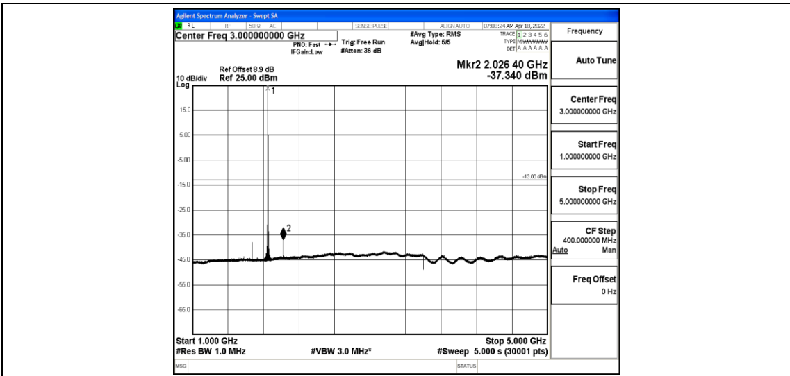
Band2-1.4MHz-QPSK-18607-1-0-Low-1000-5000--37.34-PASS
