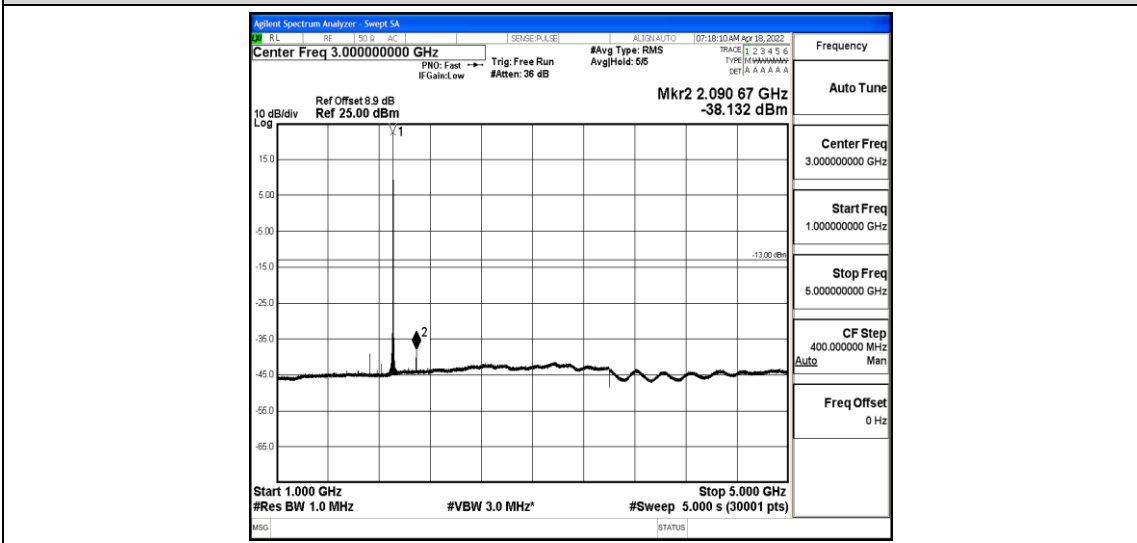
Band2-1.4MHz-16QAM-19193-1-0-High-1000-5000--38.13-PASS
