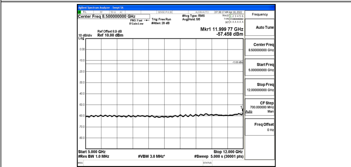
Band2-3MHz-QPSK-18615-1-0-Low-5000-12000--57.46-PASS
