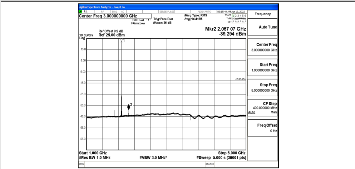
Band2-5MHz-16QAM-18900-1-0-Low-1000-5000--39.29-PASS
