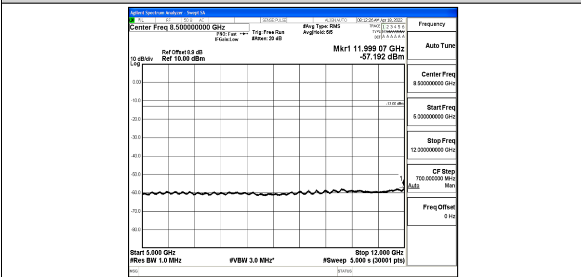
Band2-5MHz-16QAM-18625-1-0-Low-5000-12000--57.19-PASS
