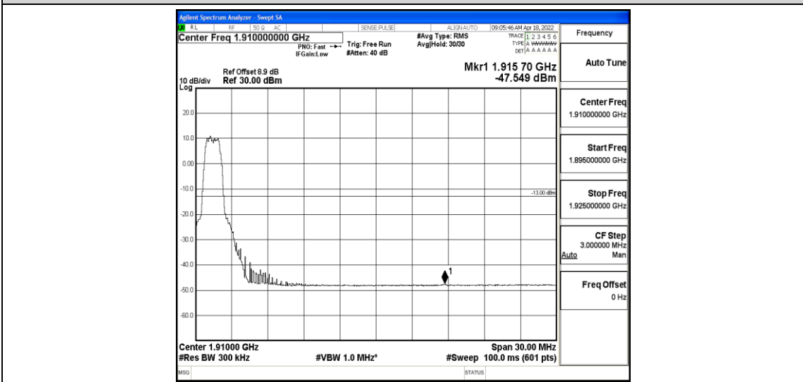
Band2-15MHz-16QAM-19125-6-0-Low--47.55-PASS
