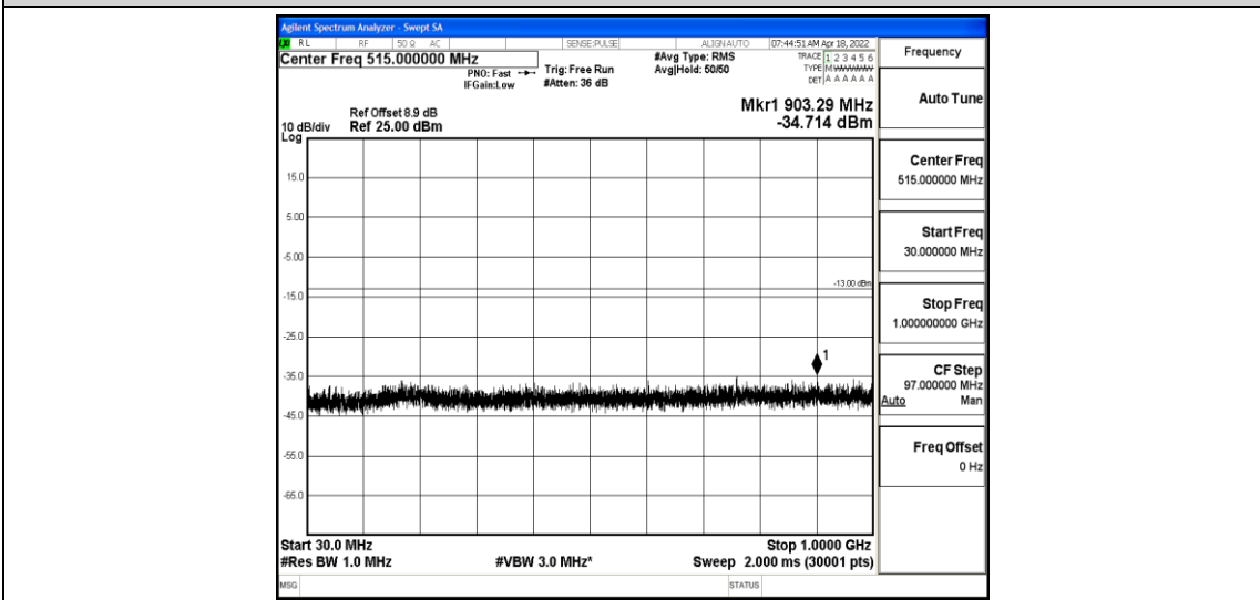
Band2-3MHz-QPSK-19185-1-0-High-30-1000--34.71-PASS
