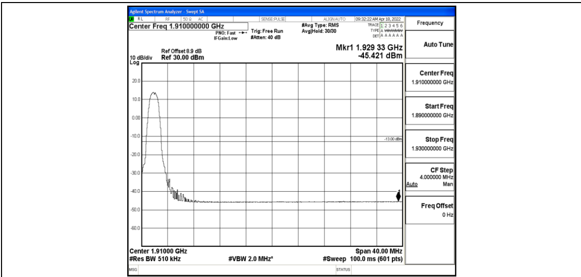
Band2-20MHz-QPSK-19100-6-0-Low--45.42-PASS
