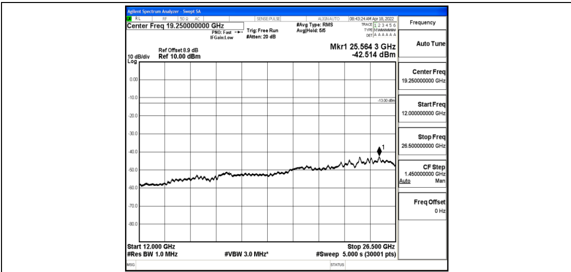
Band2-10MHz-QPSK-18900-1-0-Low-12000-26500--42.51-PASS
