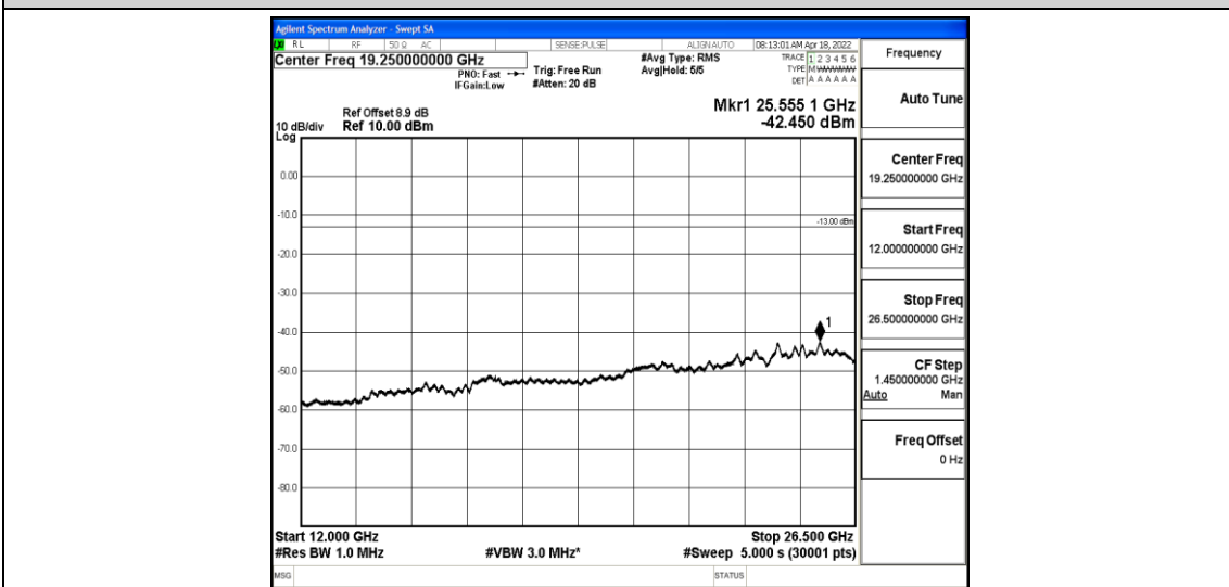
Band2-5MHz-16QAM-18625-1-0-Low-12000-26500--42.45-PASS
