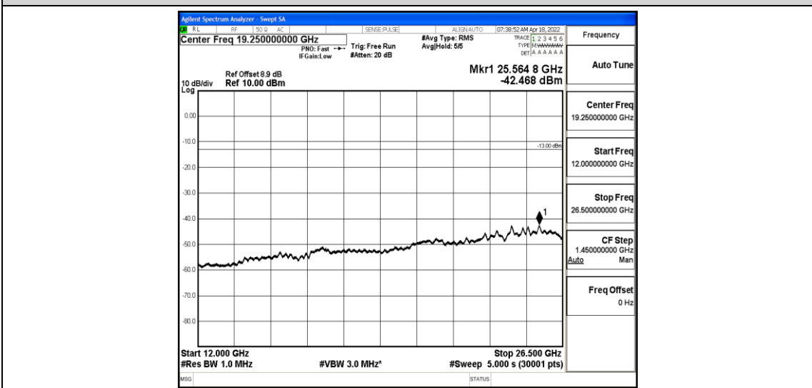
Band2-3MHz-QPSK-18615-1-0-Low-12000-26500--42.47-PASS
