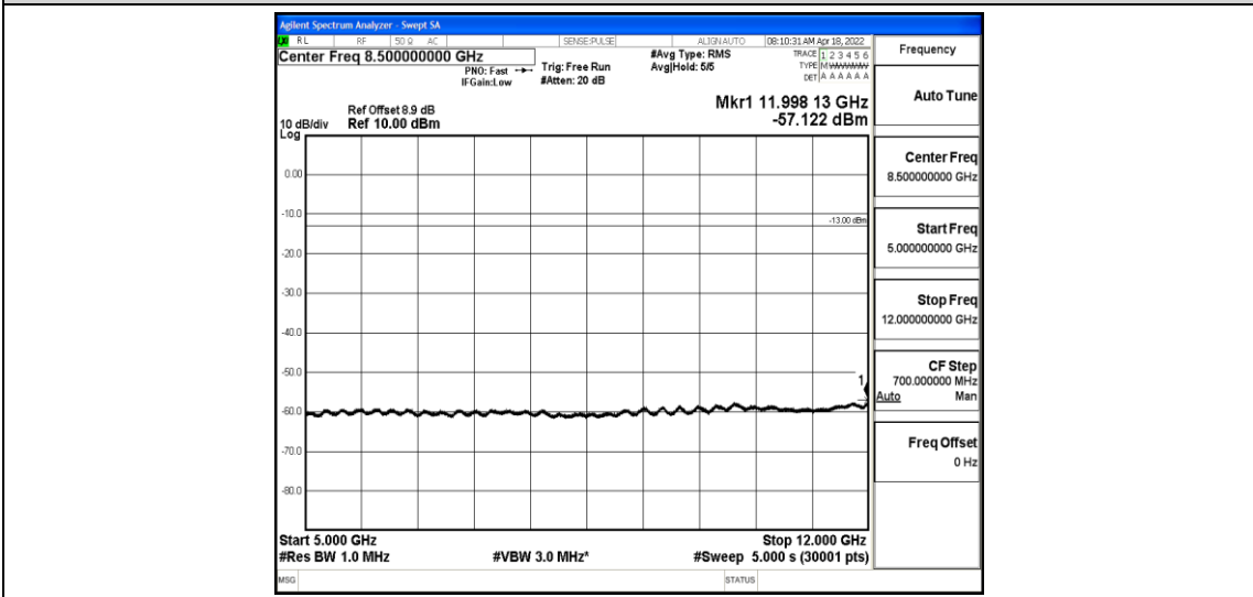
Band2-5MHz-QPSK-18625-1-0-Low-5000-12000--57.12-PASS
