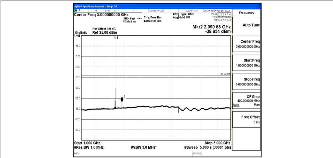
Band2-5MHz-16QAM-19175-1-0-High-1000-5000--38.63-PASS
