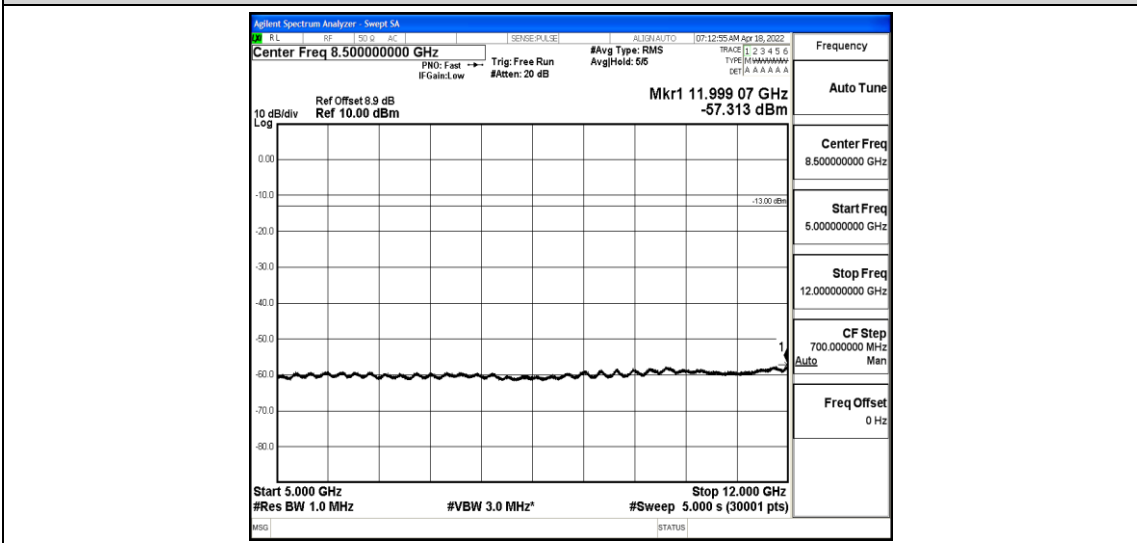
Band2-1.4MHz-QPSK-18900-1-0-Low-5000-12000--57.31-PASS
