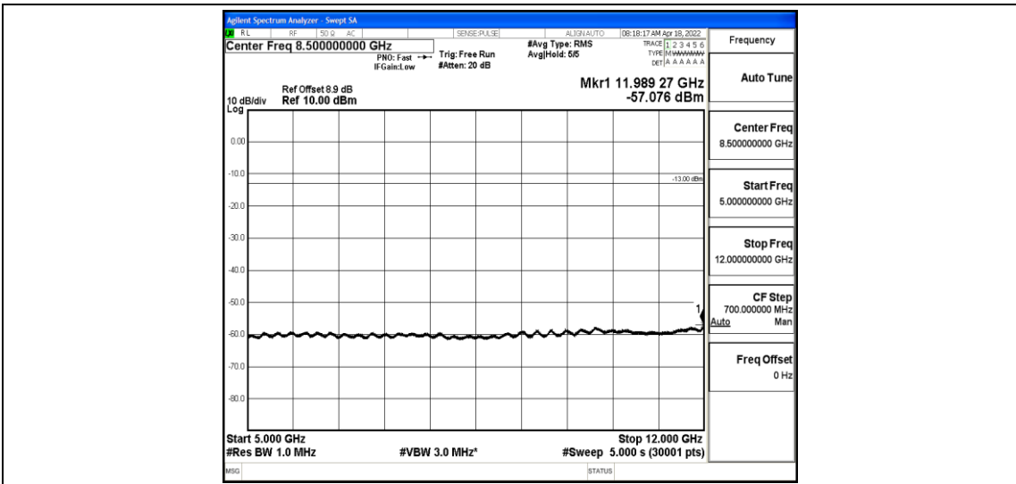
Band2-5MHz-QPSK-19175-1-0-High-5000-12000--57.08-PASS
