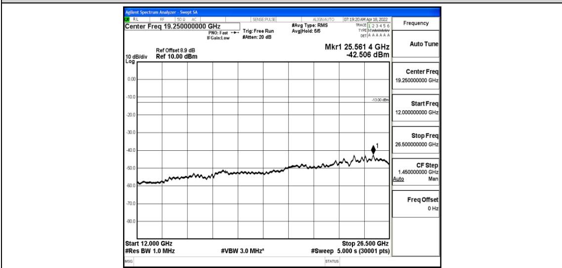
Band2-1.4MHz-16QAM-19193-1-0-High-12000-26500--42.51-PASS
