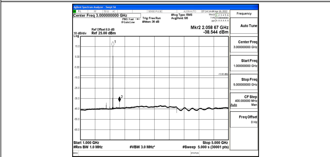
Band2-1.4MHz-16QAM-18900-1-0-Low-1000-5000--38.54-PASS
