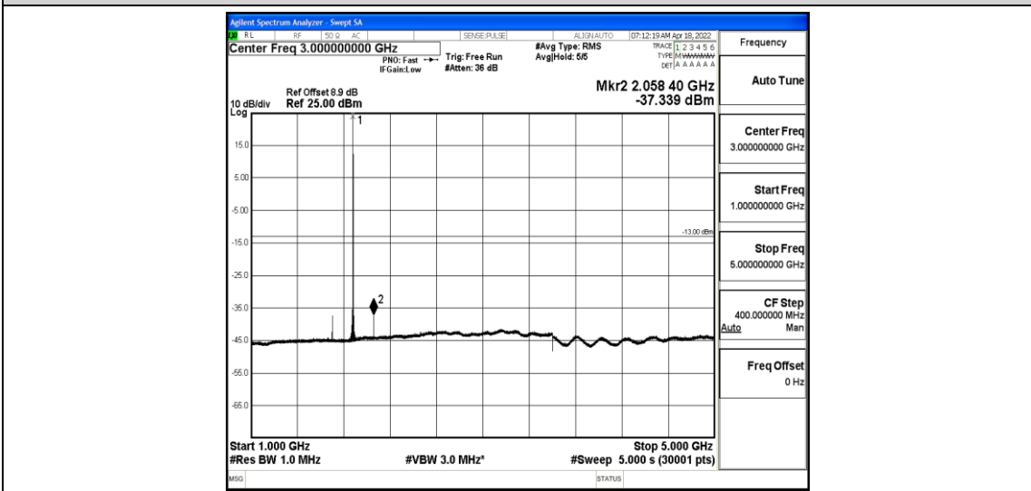
Band2-1.4MHz-QPSK-18900-1-0-Low-1000-5000--37.34-PASS
