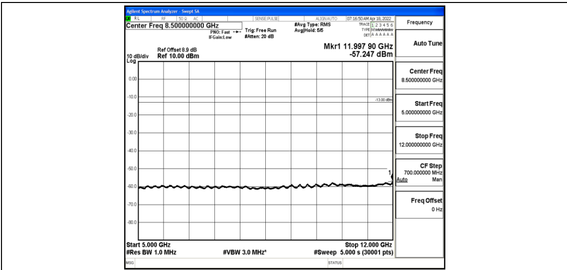
Band2-1.4MHz-QPSK-19193-1-0-High-5000-12000--57.25-PASS
