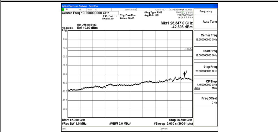
Band2-3MHz-16QAM-19185-1-0-High-12000-26500--42.4-PASS
