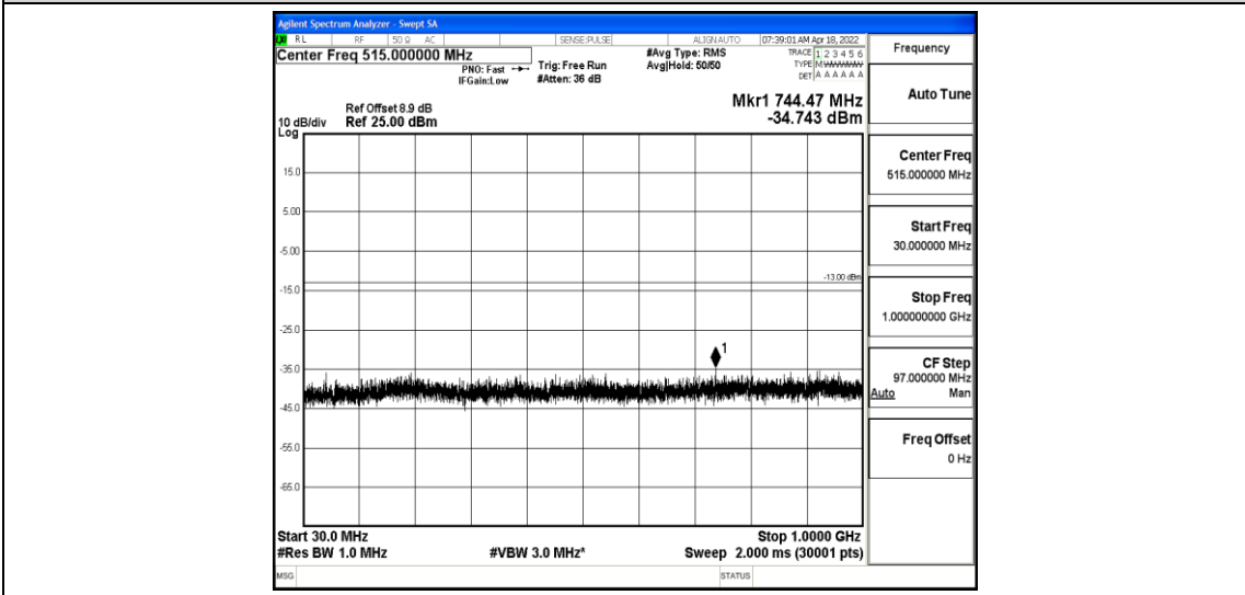
Band2-3MHz-16QAM-18615-1-0-Low-30-1000--34.74-PASS
