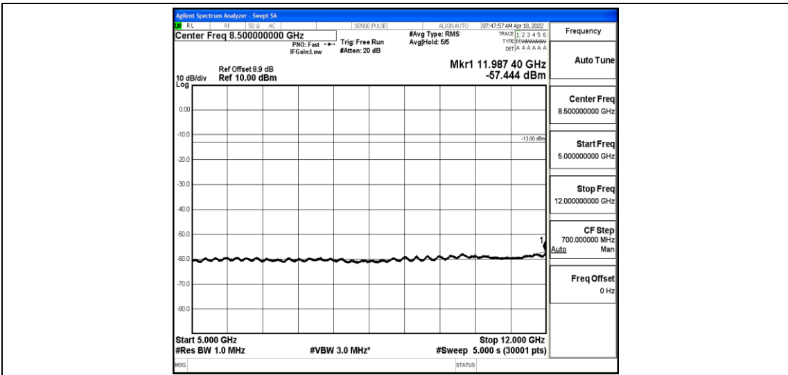
Band2-3MHz-16QAM-19185-1-0-High-5000-12000--57.44-PASS
