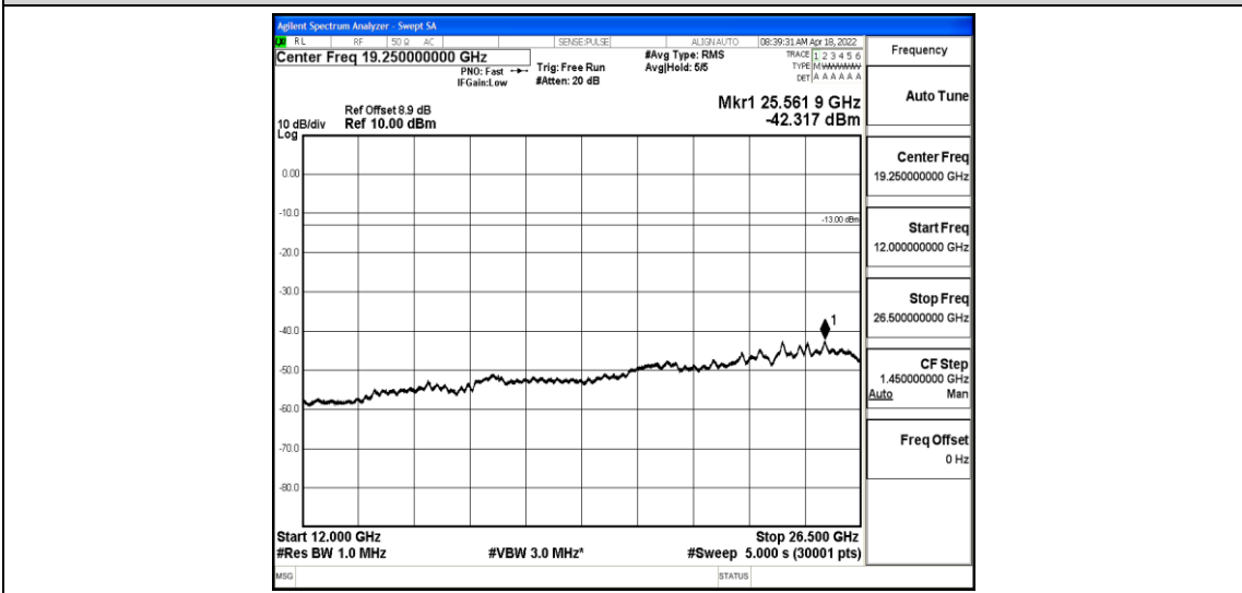
Band2-10MHz-QPSK-18650-1-0-Low-12000-26500--42.32-PASS
