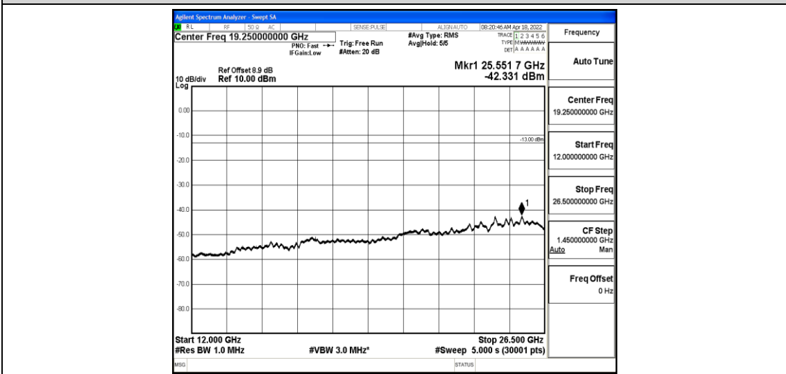
Band2-5MHz-16QAM-19175-1-0-High-12000-26500--42.33-PASS
