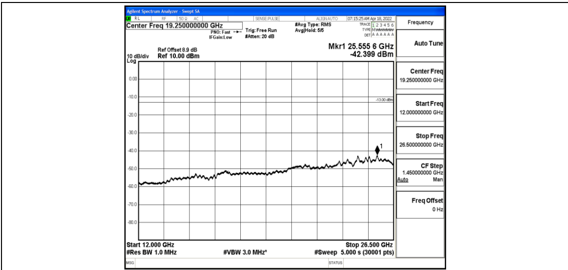
Band2-1.4MHz-16QAM-18900-1-0-Low-12000-26500--42.4-PASS
