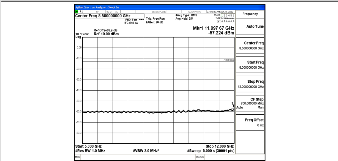
Band2-1.4MHz-QPSK-18607-1-0-Low-5000-12000--57.22-PASS
