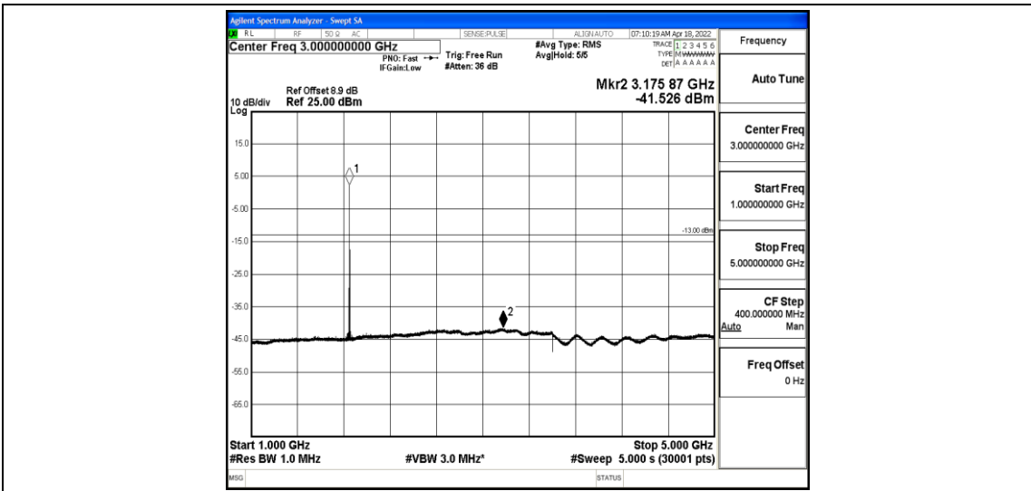
Band2-1.4MHz-16QAM-18607-1-0-Low-1000-5000--41.53-PASS
