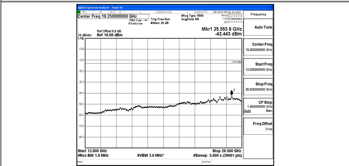
Band2-5MHz-QPSK-19175-1-0-High-12000-26500--42.44-PASS
