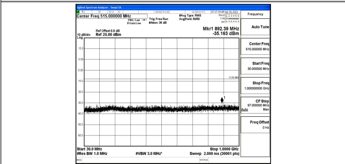
Band2-1.4MHz-16QAM-19193-1-0-High-30-1000--35.16-PASS
