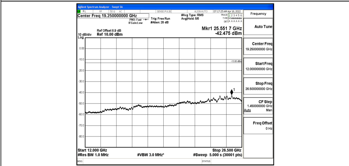
Band2-1.4MHz-QPSK-19193-1-0-High-12000-26500--42.48-PASS
