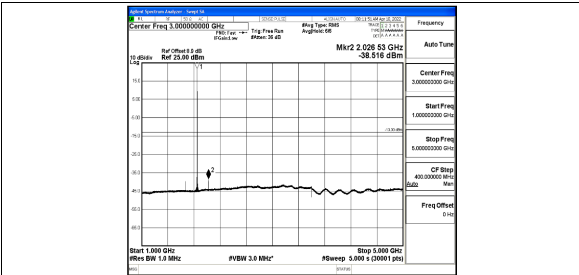
Band2-5MHz-16QAM-18625-1-0-Low-1000-5000--38.52-PASS
