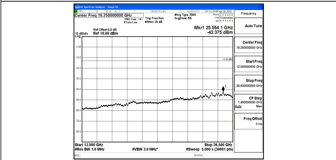
Band2-1.4MHz-16QAM-18607-1-0-Low-12000-26500--42.38-PASS
