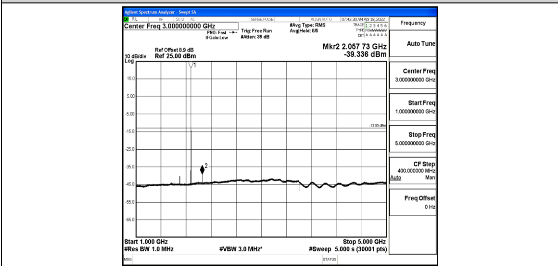
Band2-3MHz-16QAM-18900-1-0-Low-1000-5000--39.34-PASS
