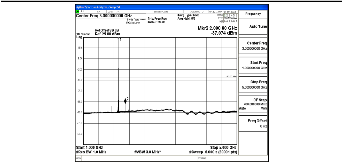
Band2-1.4MHz-QPSK-19193-1-0-High-1000-5000--37.07-PASS
