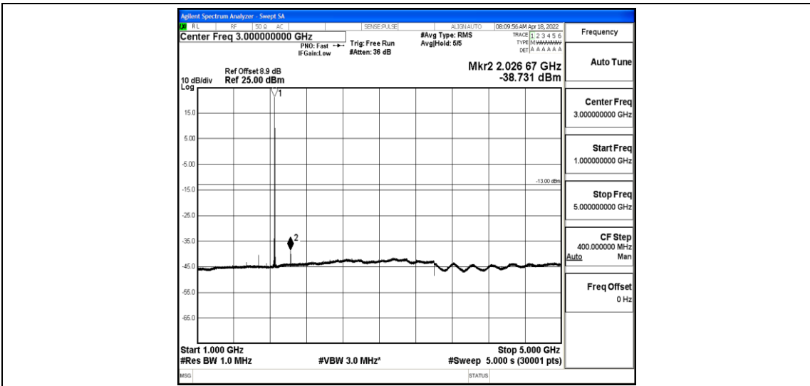
Band2-5MHz-QPSK-18625-1-0-Low-1000-5000--38.73-PASS
