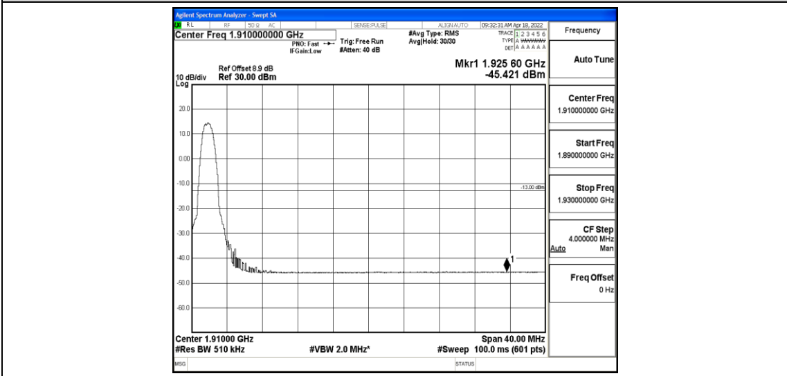
Band2-20MHz-16QAM-19100-6-0-Low--45.42-PASS
