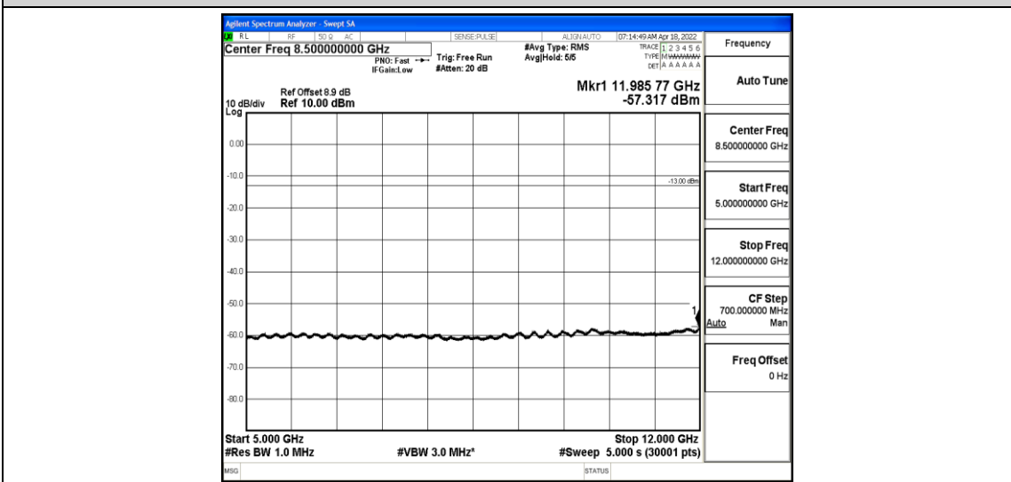
Band2-1.4MHz-16QAM-18900-1-0-Low-5000-12000--57.32-PASS
