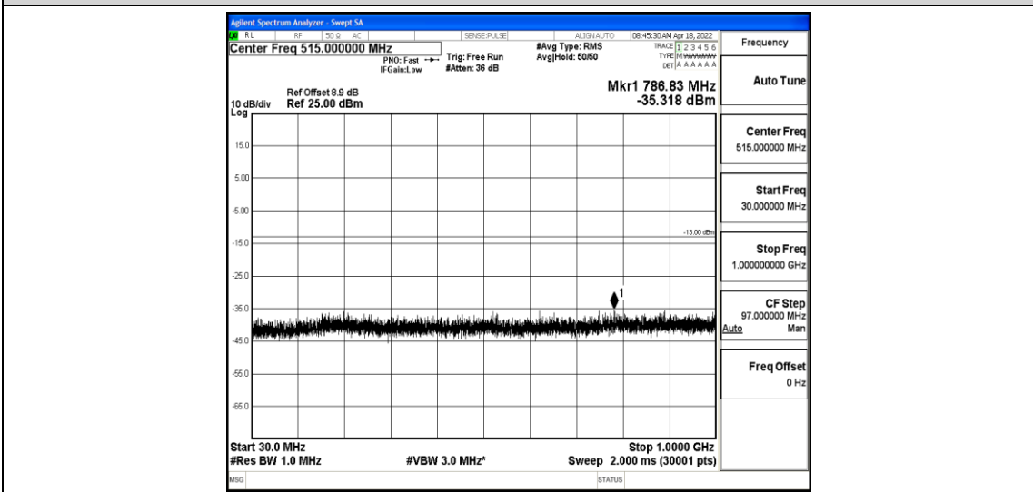
Band2-10MHz-QPSK-19150-1-0-High-30-1000--35.32-PASS
