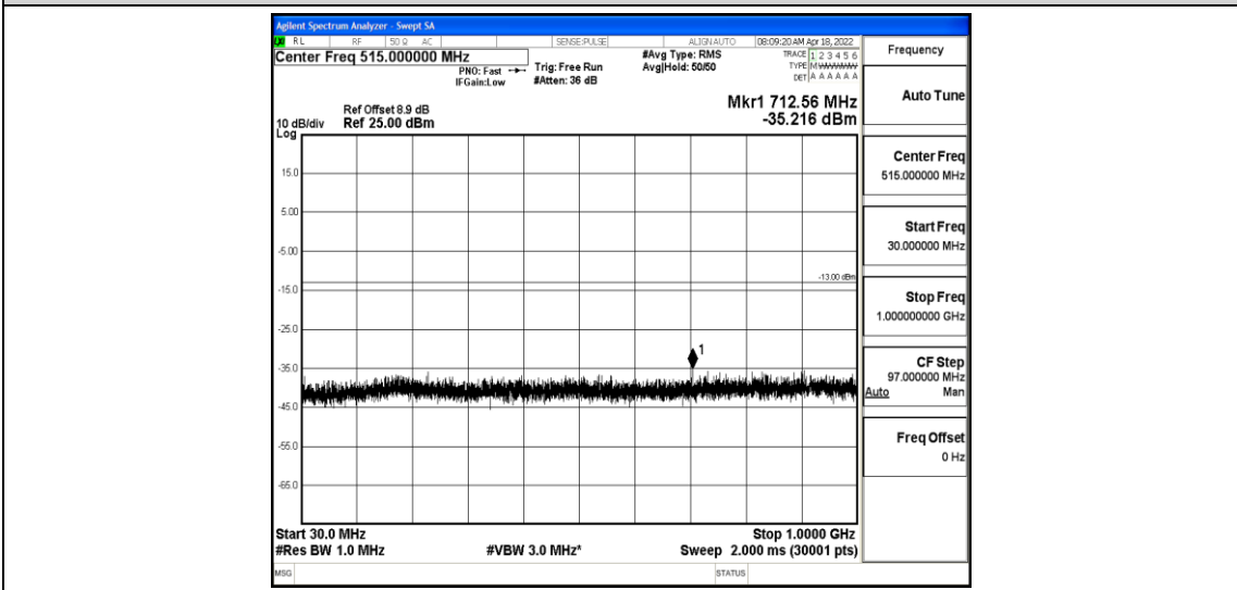
Band2-5MHz-QPSK-18625-1-0-Low-30-1000--35.22-PASS
