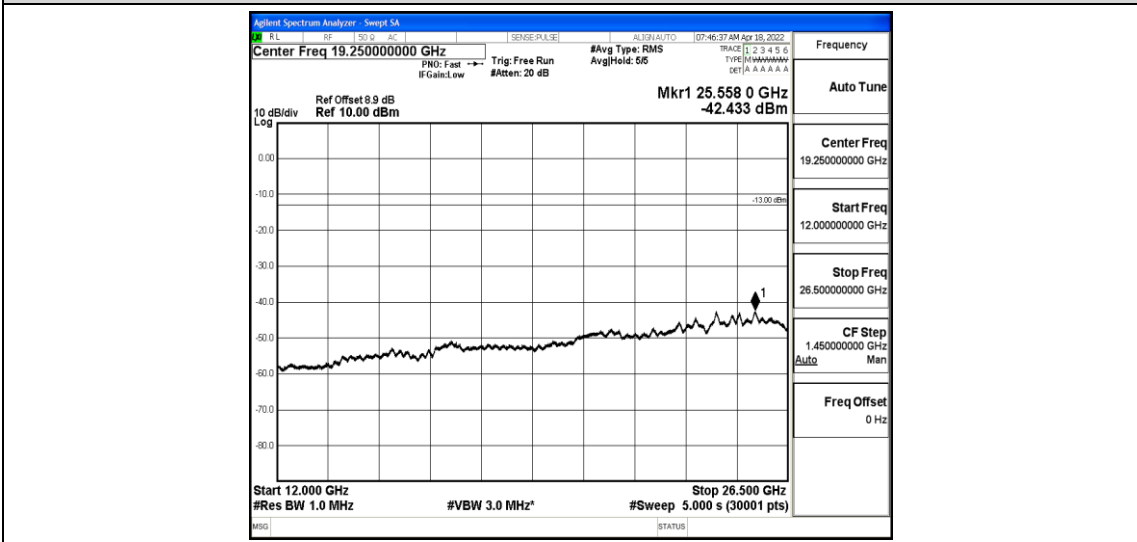
Band2-3MHz-QPSK-19185-1-0-High-12000-26500--42.43-PASS
