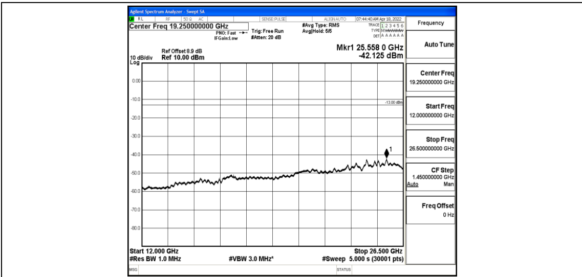
Band2-3MHz-16QAM-18900-1-0-Low-12000-26500--42.13-PASS
