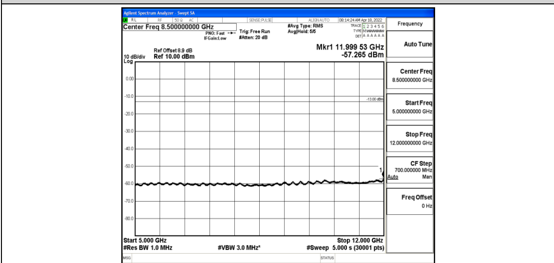
Band2-5MHz-QPSK-18900-1-0-Low-5000-12000--57.27-PASS
