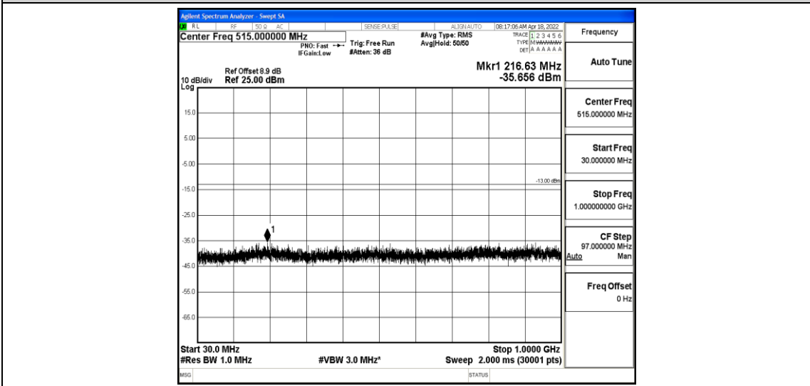
Band2-5MHz-QPSK-19175-1-0-High-30-1000--35.66-PASS
