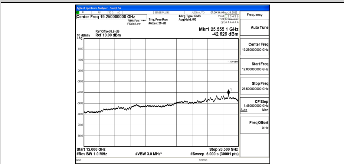
Band2-1.4MHz-QPSK-18607-1-0-Low-12000-26500--42.63-PASS
