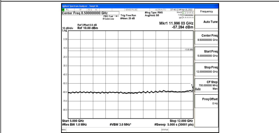
Band2-3MHz-16QAM-18615-1-0-Low-5000-12000--57.28-PASS
