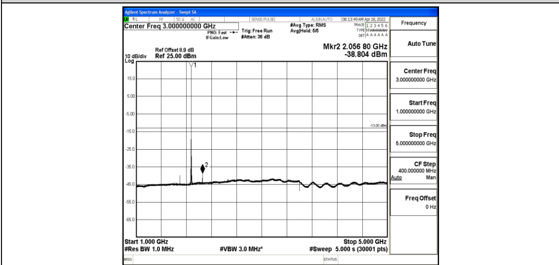
Band2-5MHz-QPSK-18900-1-0-Low-1000-5000--38.8-PASS
