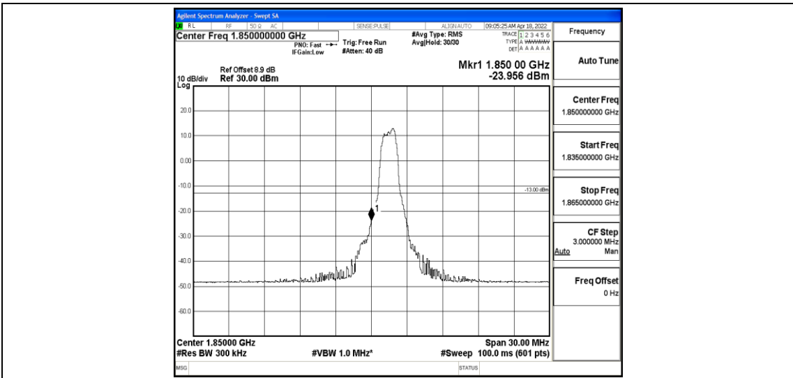
Band2-15MHz-16QAM-18675-6-0-Low--23.96-PASS
