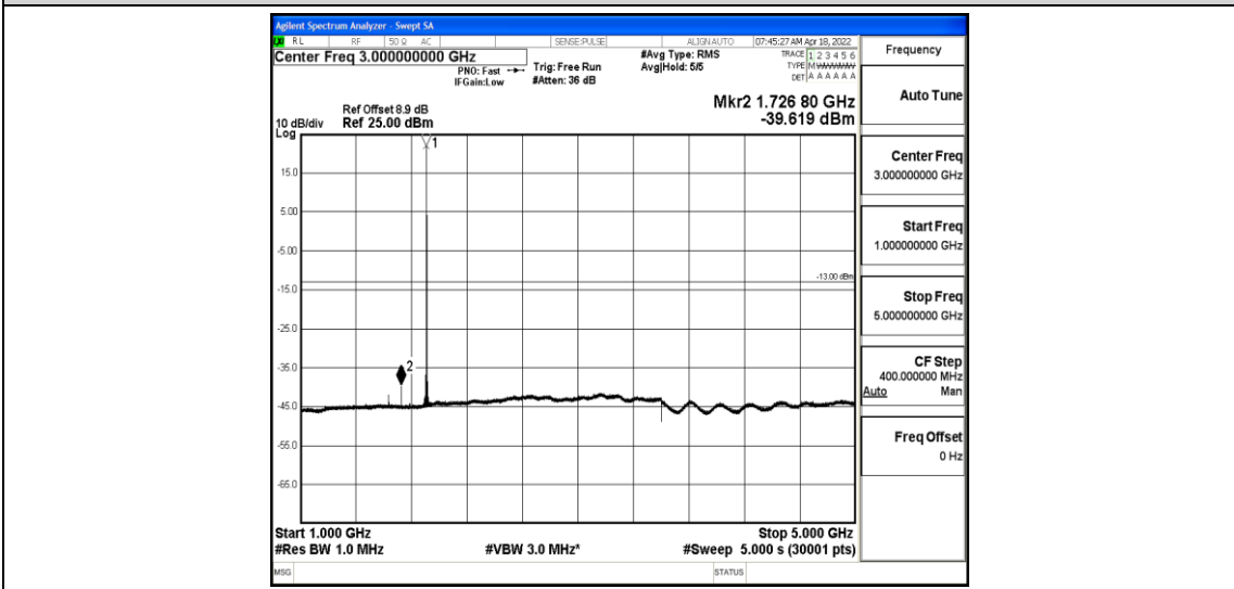
Band2-3MHz-QPSK-19185-1-0-High-1000-5000--39.62-PASS
