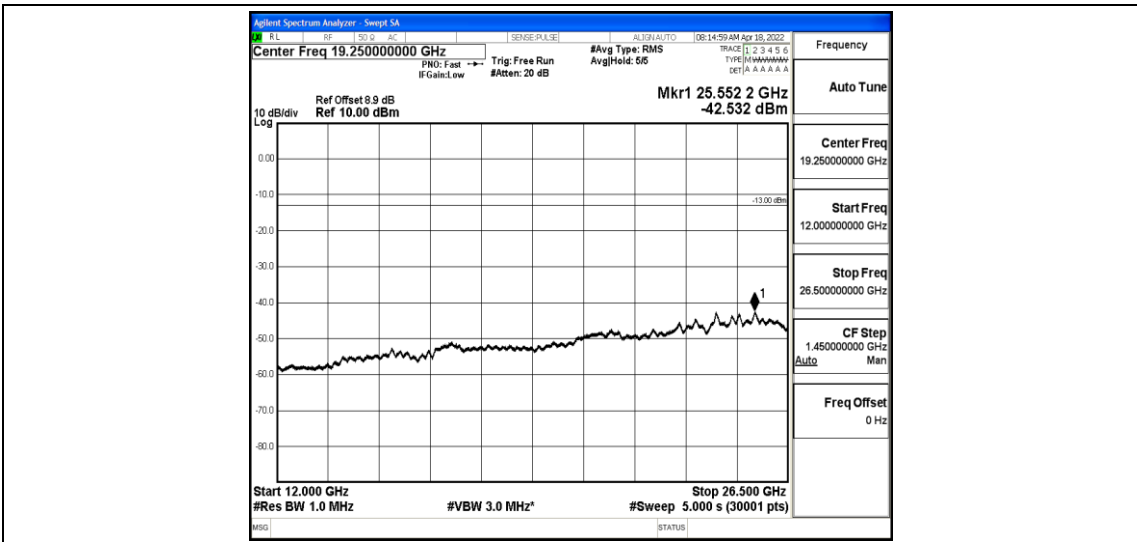
Band2-5MHz-QPSK-18900-1-0-Low-12000-26500--42.53-PASS
