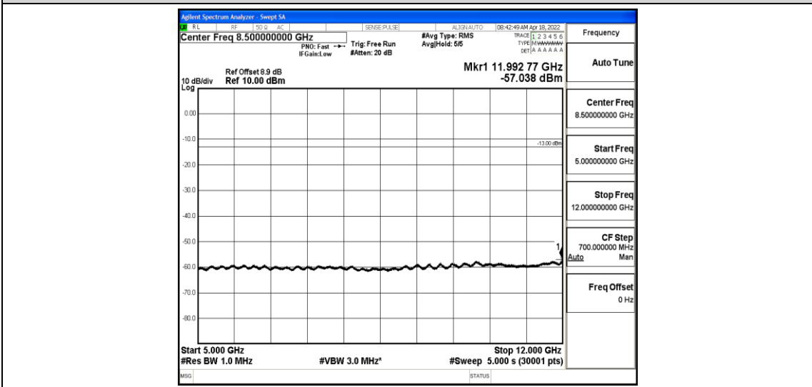
Band2-10MHz-QPSK-18900-1-0-Low-5000-12000--57.04-PASS
