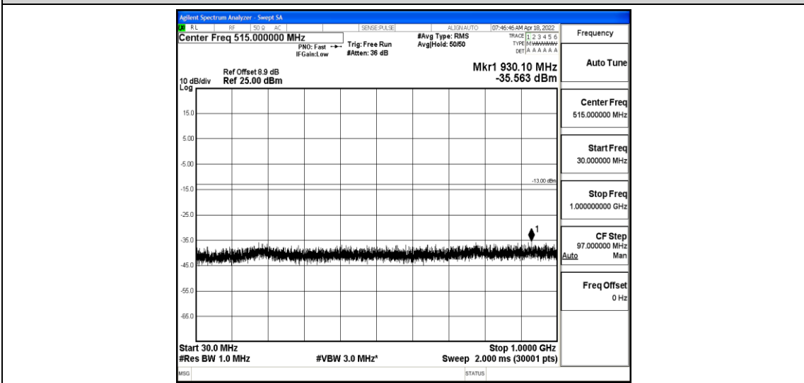
Band2-3MHz-16QAM-19185-1-0-High-30-1000--35.56-PASS
