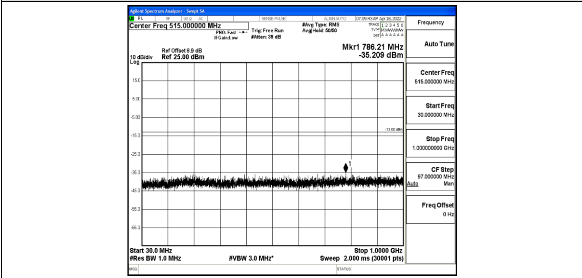
Band2-1.4MHz-16QAM-18607-1-0-Low-30-1000--35.21-PASS
