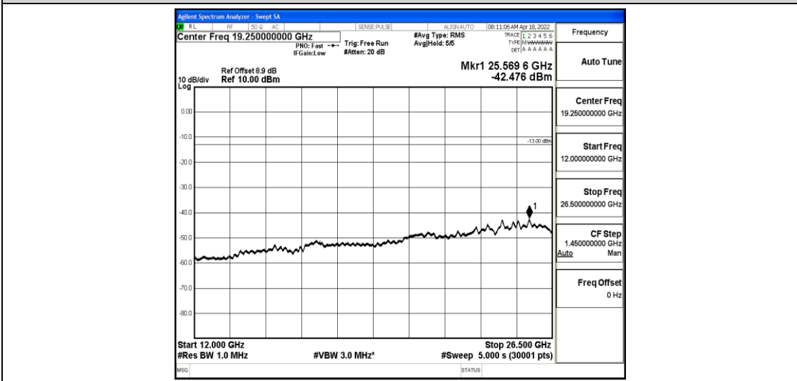
Band2-5MHz-QPSK-18625-1-0-Low-12000-26500--42.48-PASS
