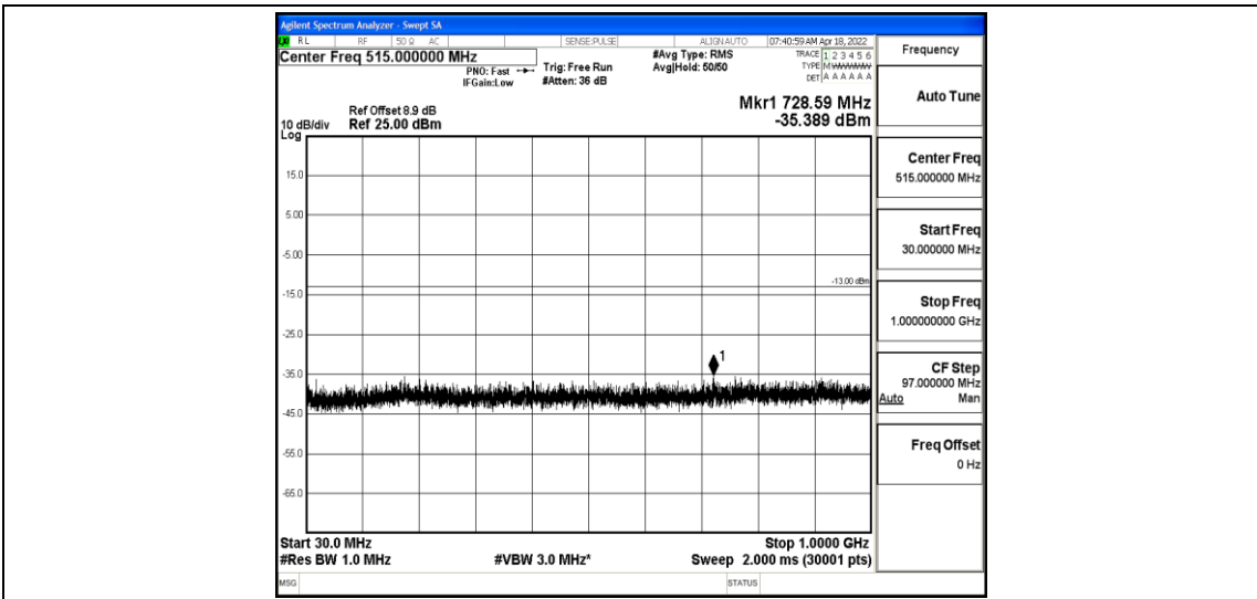
Band2-3MHz-QPSK-18900-1-0-Low-30-1000--35.39-PASS
