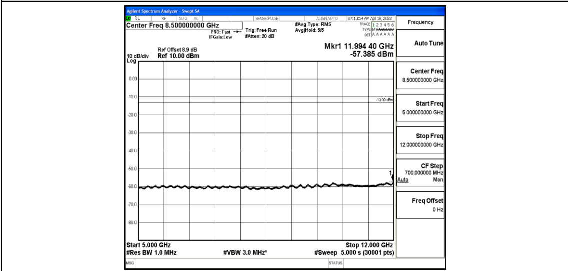
Band2-1.4MHz-16QAM-18607-1-0-Low-5000-12000--57.39-PASS
