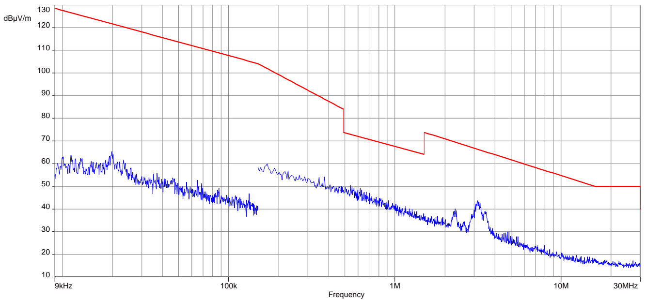
Plot 2: 9 kHz – 30 MHz, magnetic emissions (90 degree)
