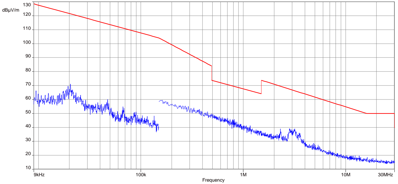
Plot 1: 9 kHz – 30 MHz, magnetic emissions (0 degree)
