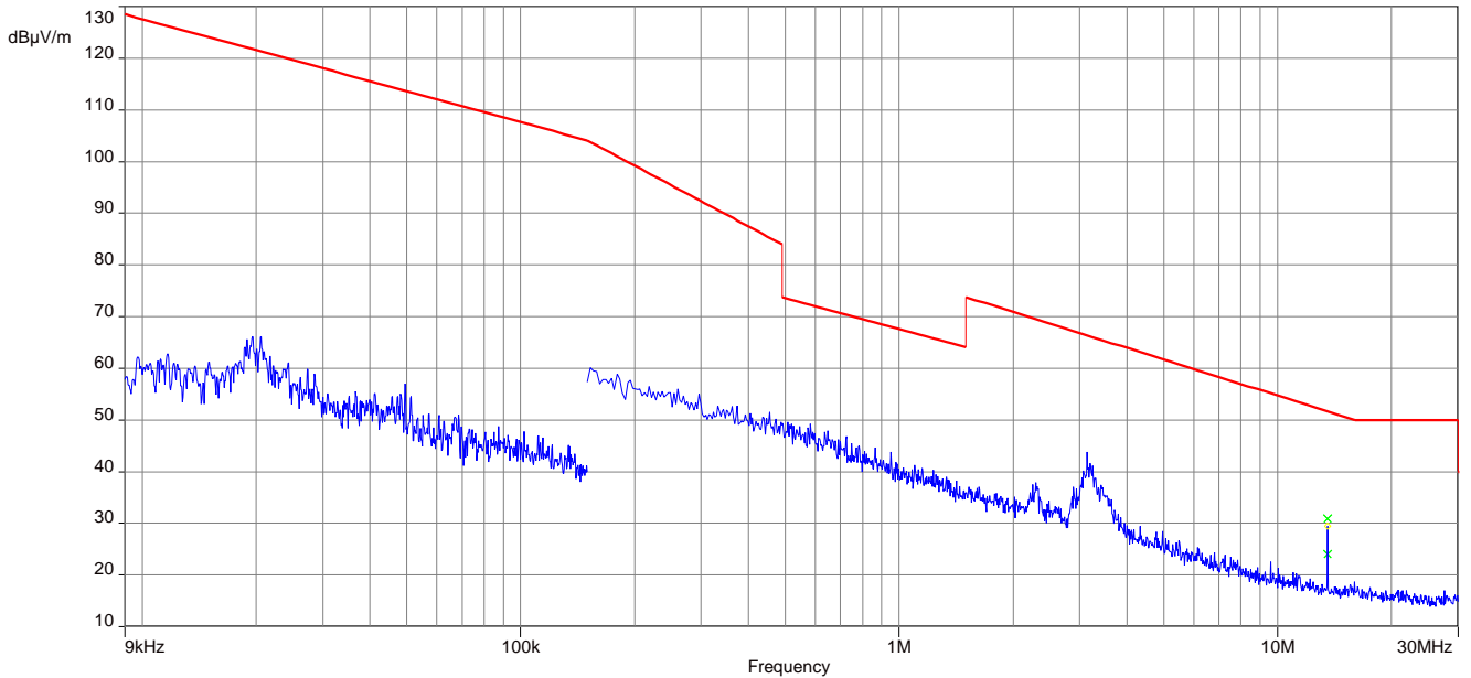
Plot 3: 9 kHz – 30 MHz, magnetic emissions (Antenna position horizontally w.r.t EUT)
