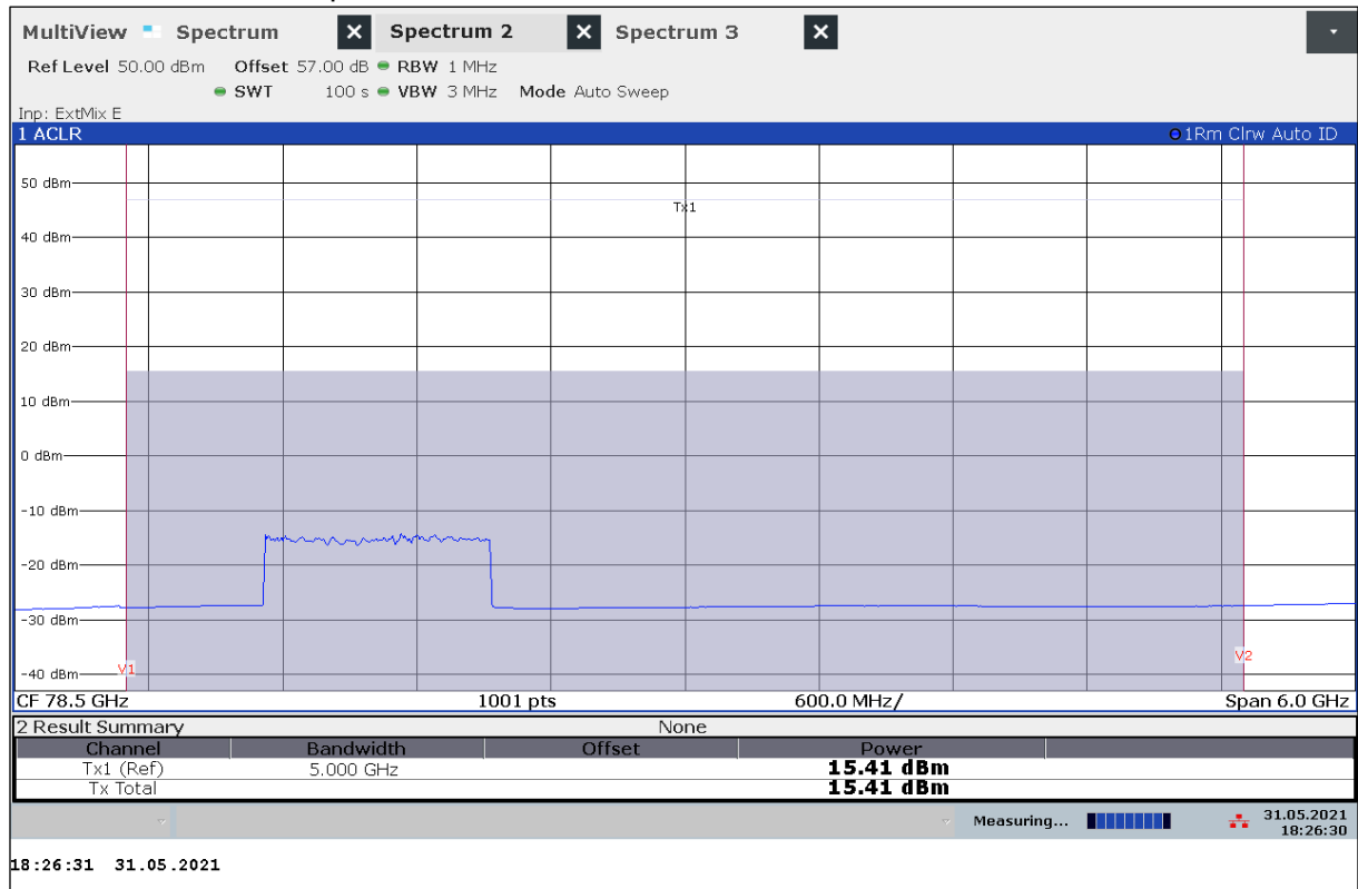
Plot 3: Mode2_4262 – Mean power
