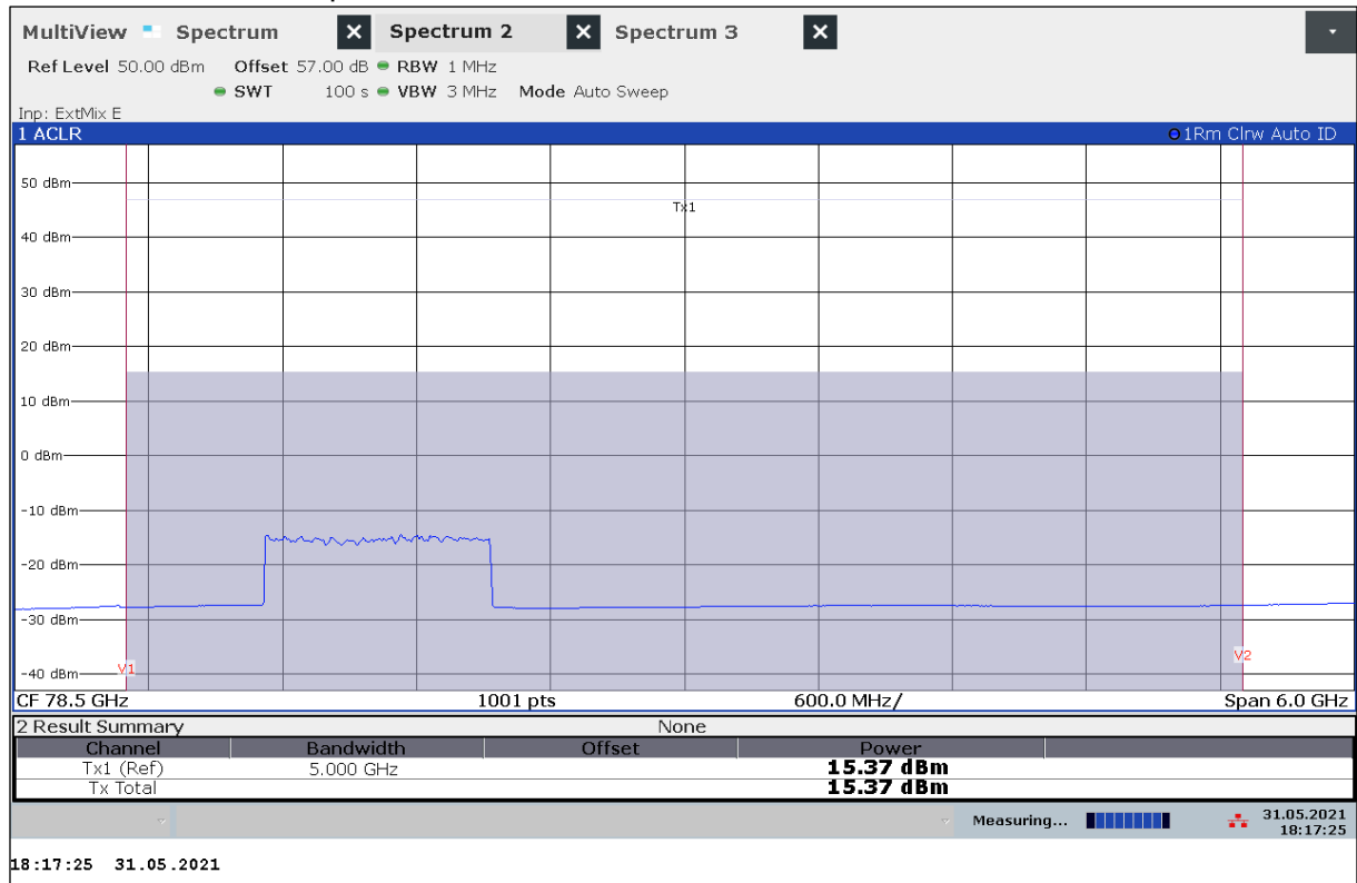
Plot 4: Mode2_4672 – Mean power
