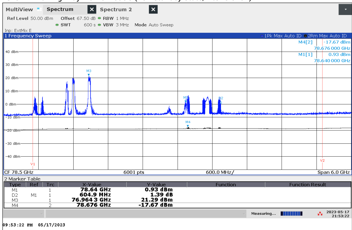
Plot 45: OBW with Highway Traffic Mode 3 (EUT Standby State, Interferer On)
