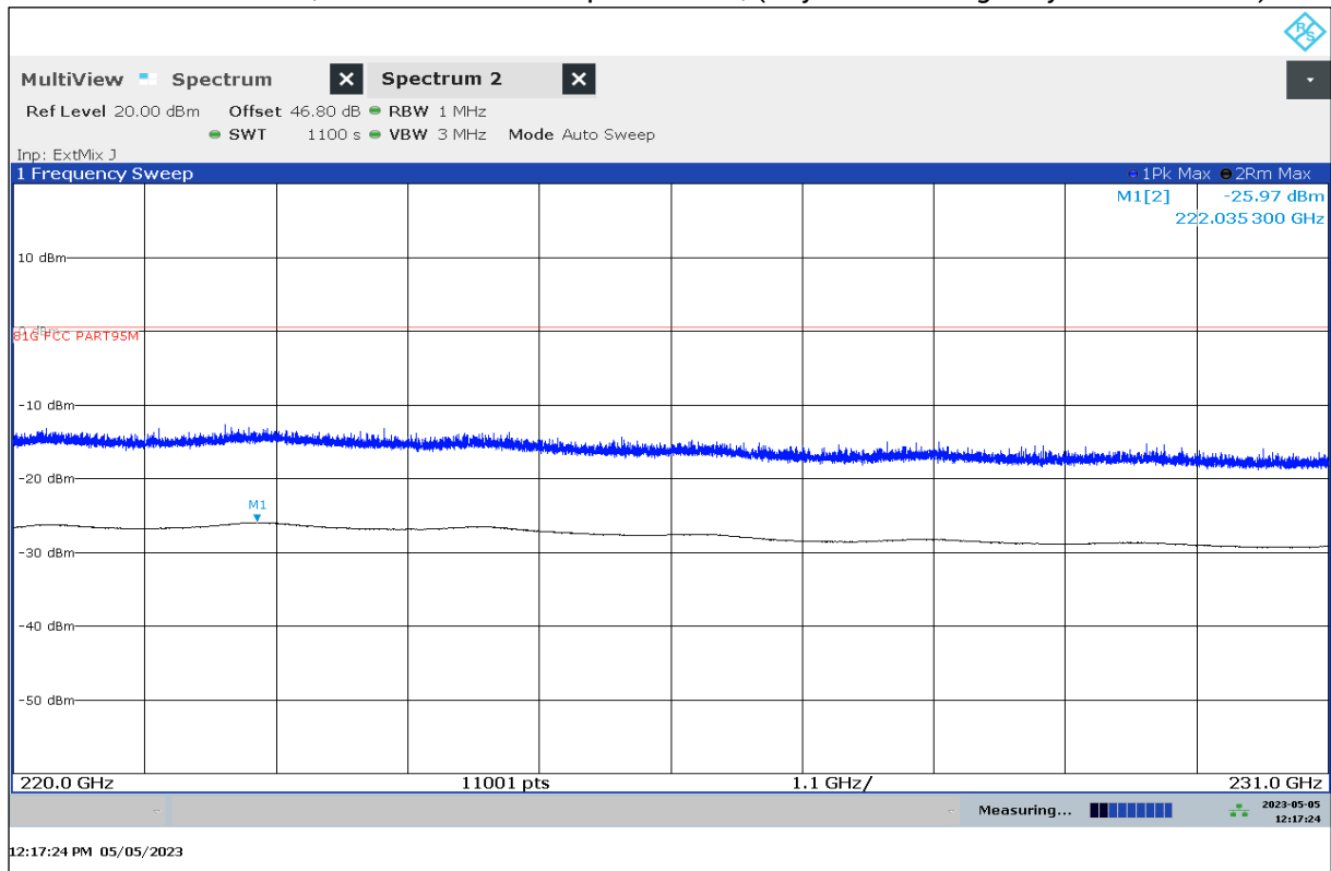
Plot 31: 220 GHz – 231 GHz, vertical / horizontal polarization, (City Mode 3 / Highway Traffic Mode 3).
