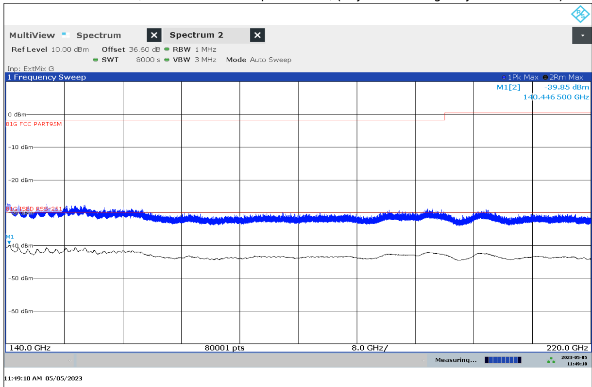
Plot 29: 140 GHz – 220 GHz, vertical / horizontal polarization, (City Mode 3 / Highway Traffic Mode 3).
