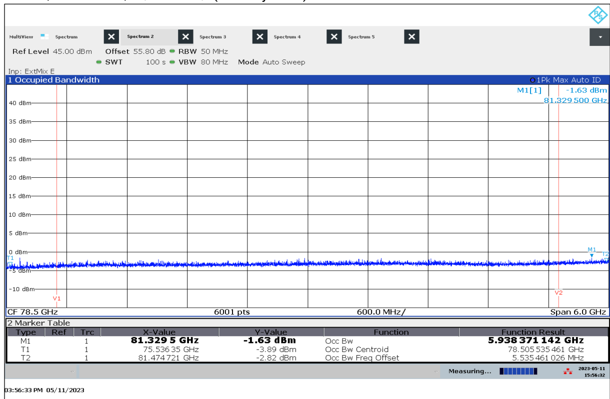
Plot 7: OBW, Peak Power, T_{\text{nom}} / V_{\text{min-max}} (StandBy State)
