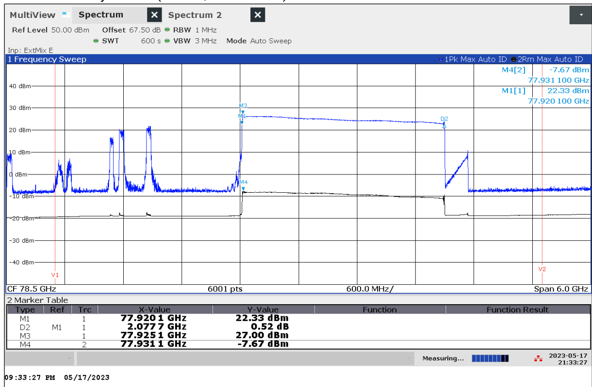
Plot 44: OBW with City Mode 3 (EUT On, Interferer On)
