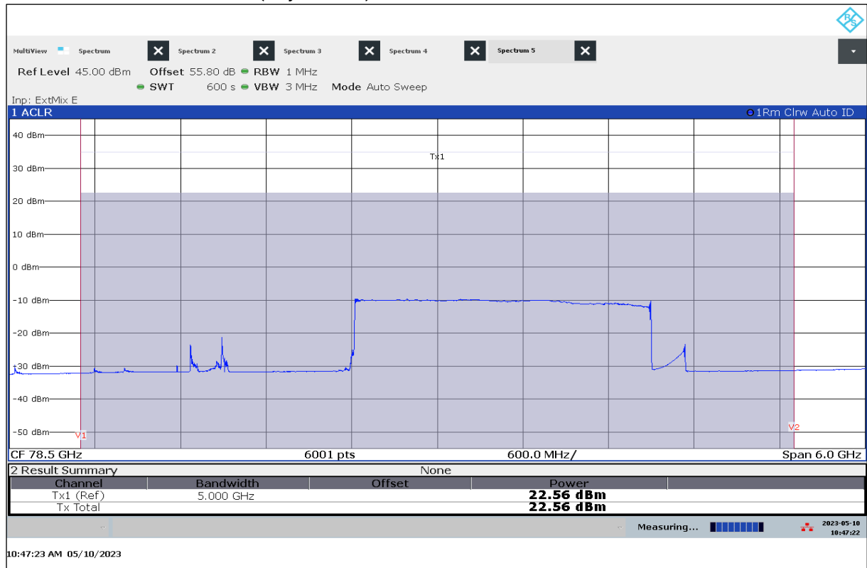
Plot 3: Mean Power, T_{\text{nom}} / V_{\text{min-max}} (City Mode 3)
