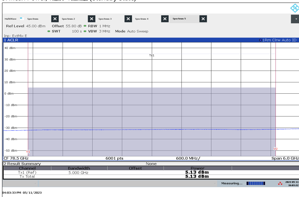
Plot 9: Mean Power, T_{\text{nom}} / V_{\text{min-max}} (StandBy State)
