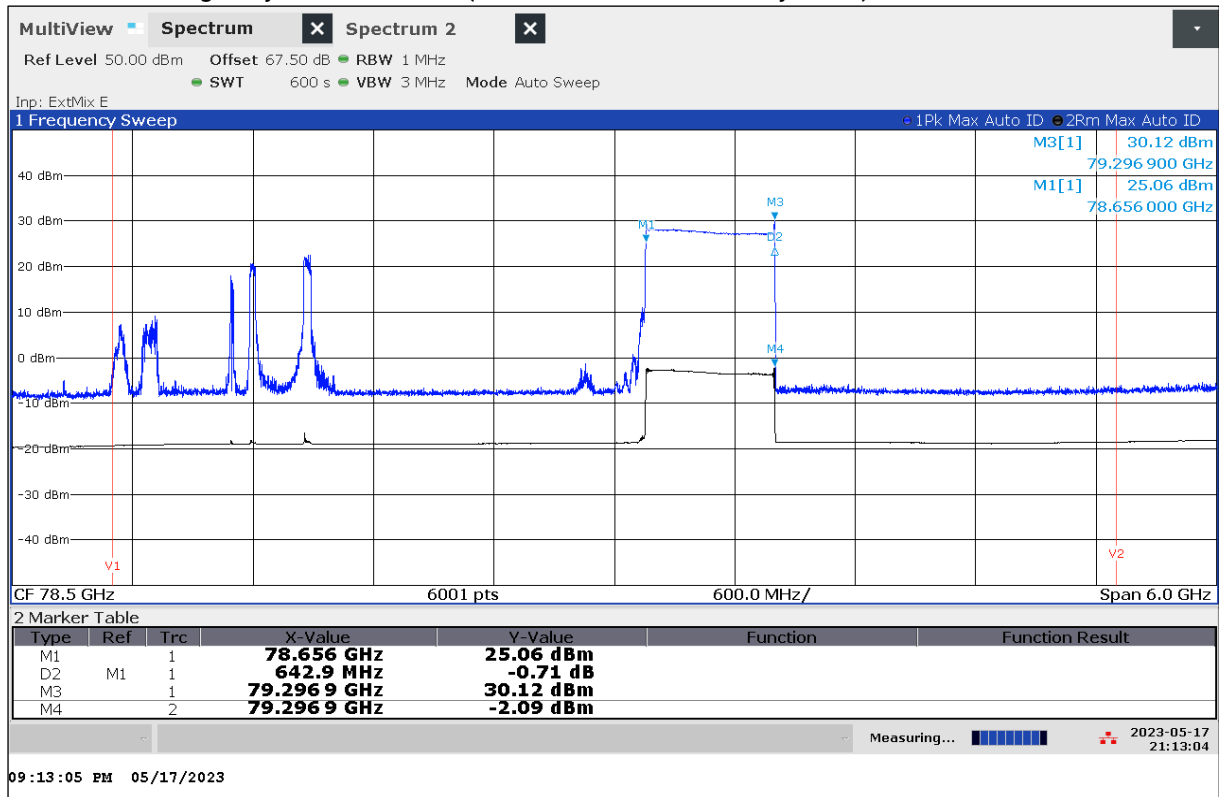
Plot 46: OBW with Highway Traffic Mode 3 (EUT On, Interferer Standby State)
