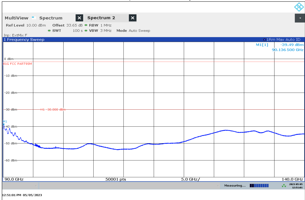
Plot 28: 90 GHz – 140 GHz, vertical / horizontal polarization, Standby State
