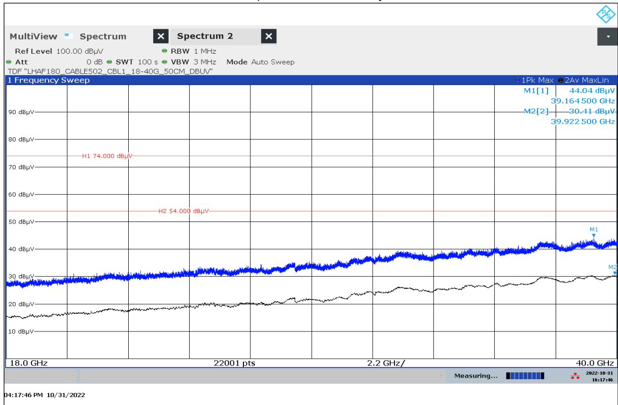
Plot 19: 18 GHz – 40 GHz, vertical / horizontal polarization, Standby State
