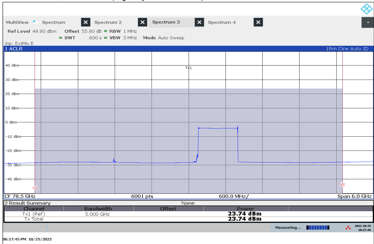
Plot 4: Mean Power, T_{\text{nom}} / V_{\text{min-max}} (Highway Traffic Mode 3)
