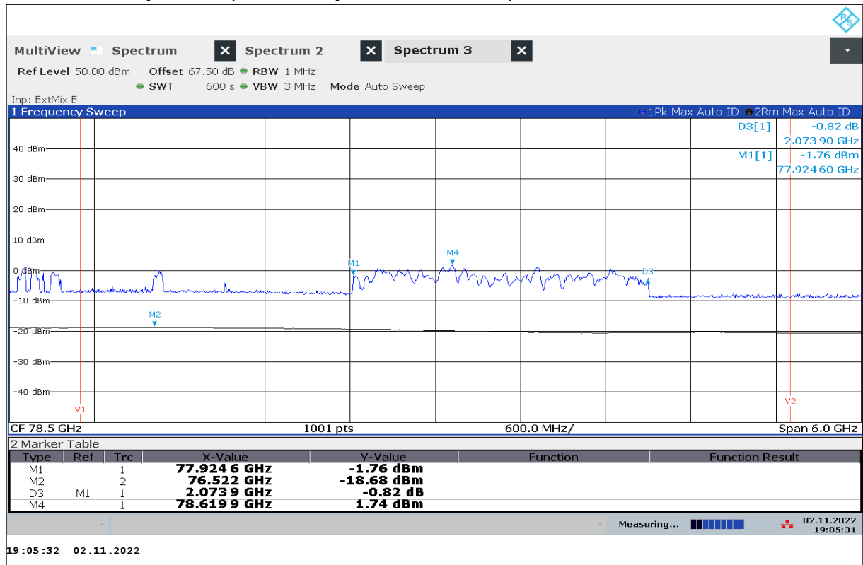
Plot 41: OBW with City Mode 3 (EUT Standby State, Interferer On)
