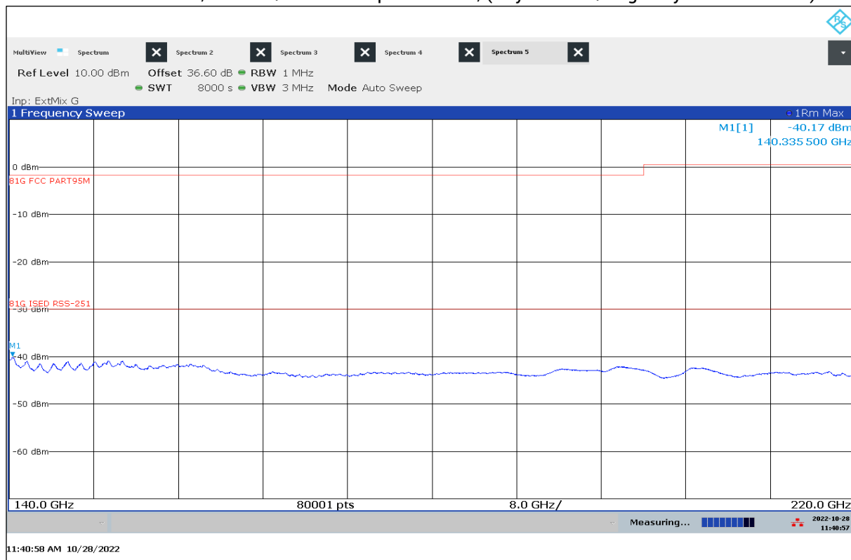
Plot 28: 140 GHz – 220 GHz, vertical / horizontal polarization, (City Mode 3 / Highway Traffic Mode 3).
