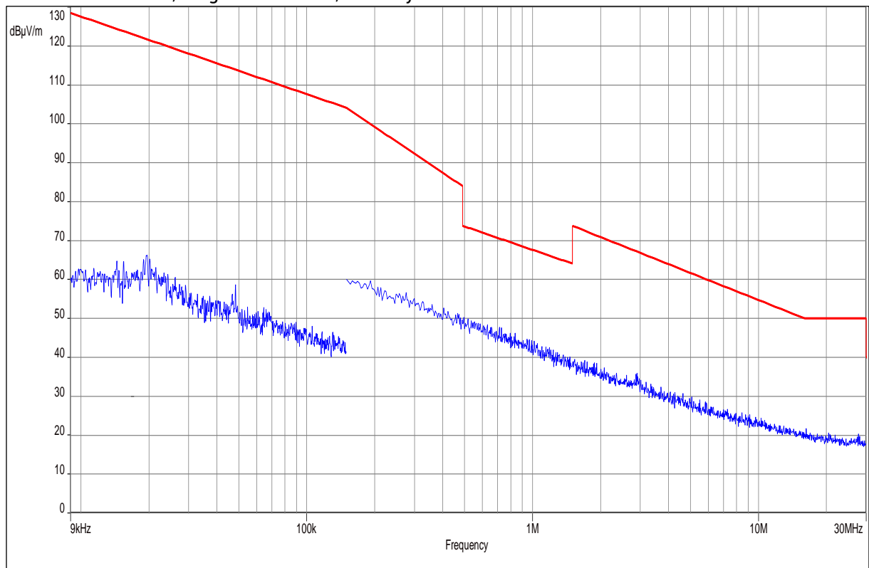
Plot 10: 9 kHz – 30 MHz, Magnetic antenna, Standby State
