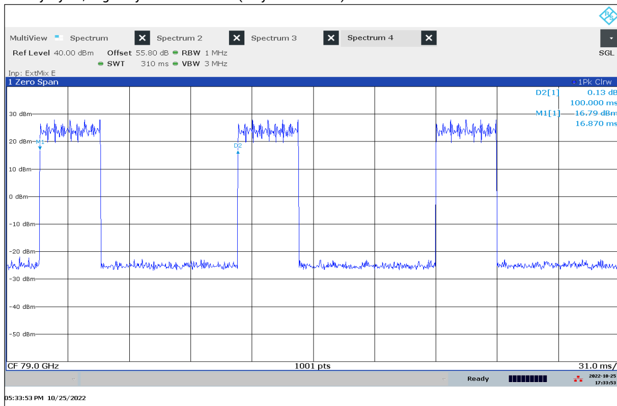
Plot 8: Duty Cycle, Highway Traffic Mode 3 (only informative)
