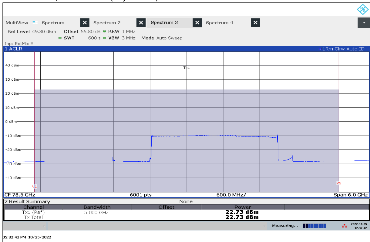
Plot 2: Mean Power, T nom / V min-max (City Mode 3)
