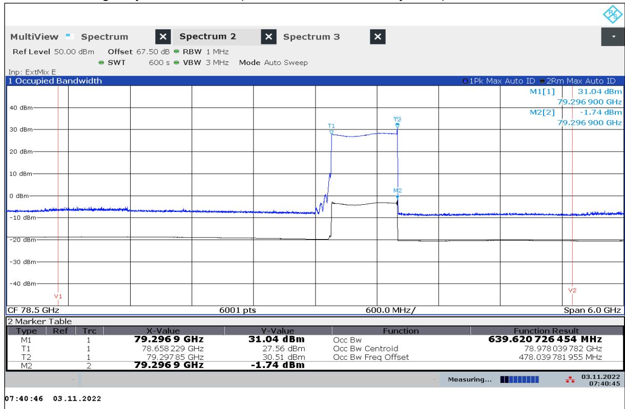
Plot 45: OBW with Highway Traffic Mode 3 (EUT On, Interferer Standby State)
