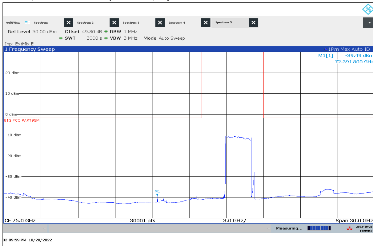
Plot 23: OOB, vertical / horizontal polarization, City Mode 3
