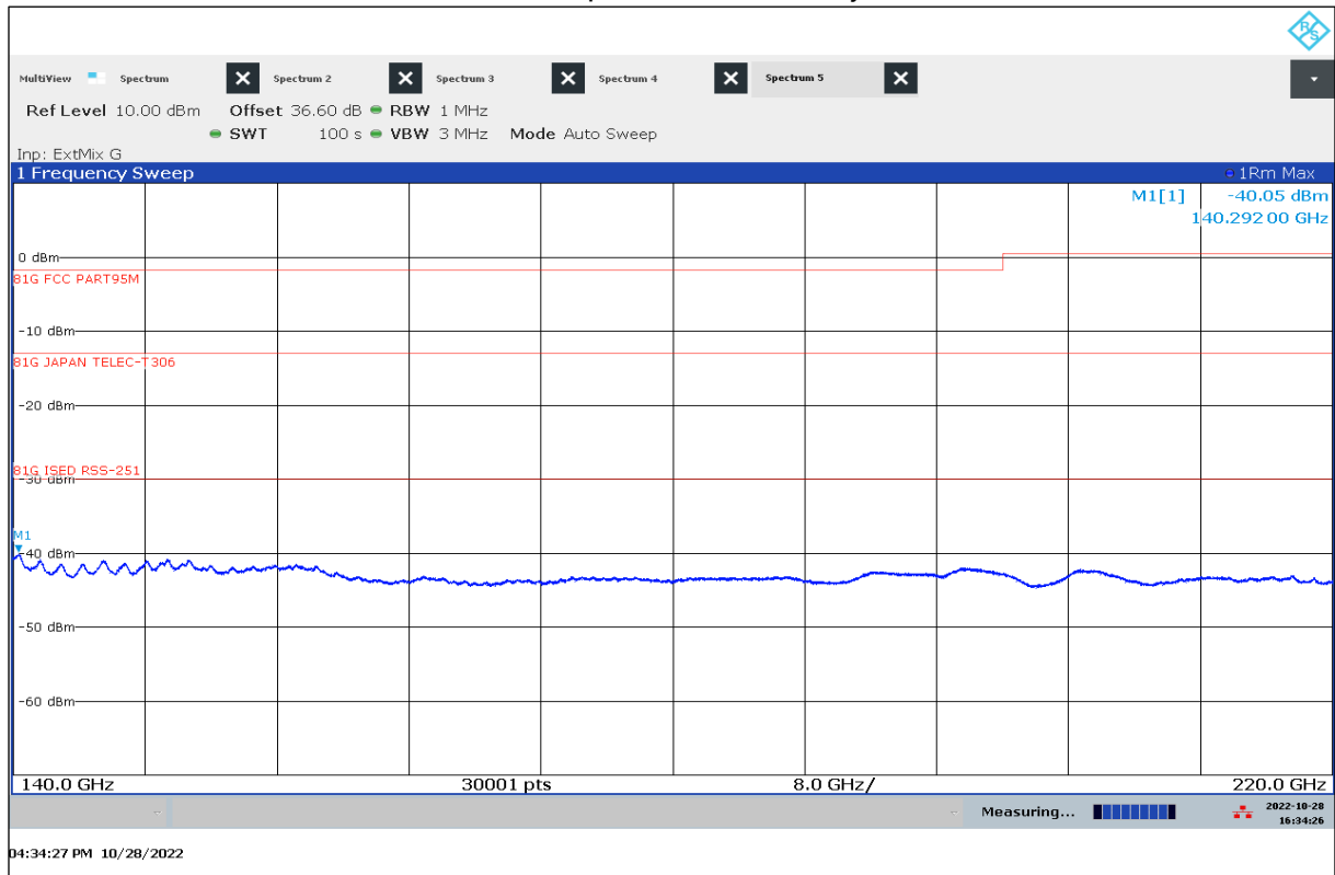
Plot 29: 140 GHz – 220 GHz, vertical / horizontal polarization, Standby State
