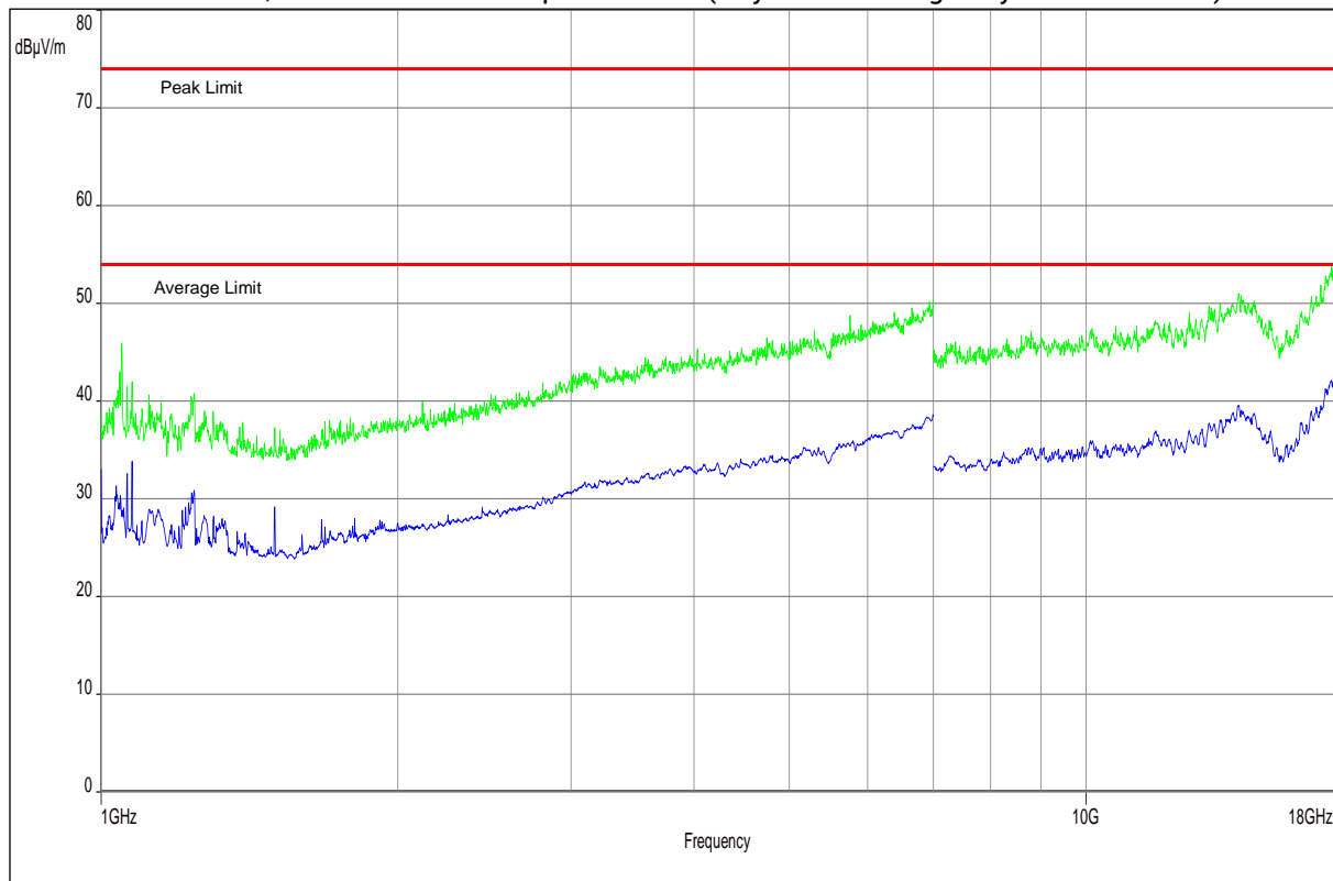
Plot 13: 1 GHz – 18 GHz, vertical / horizontal polarization (City Mode 3 / Highway Traffic Mode 3)
