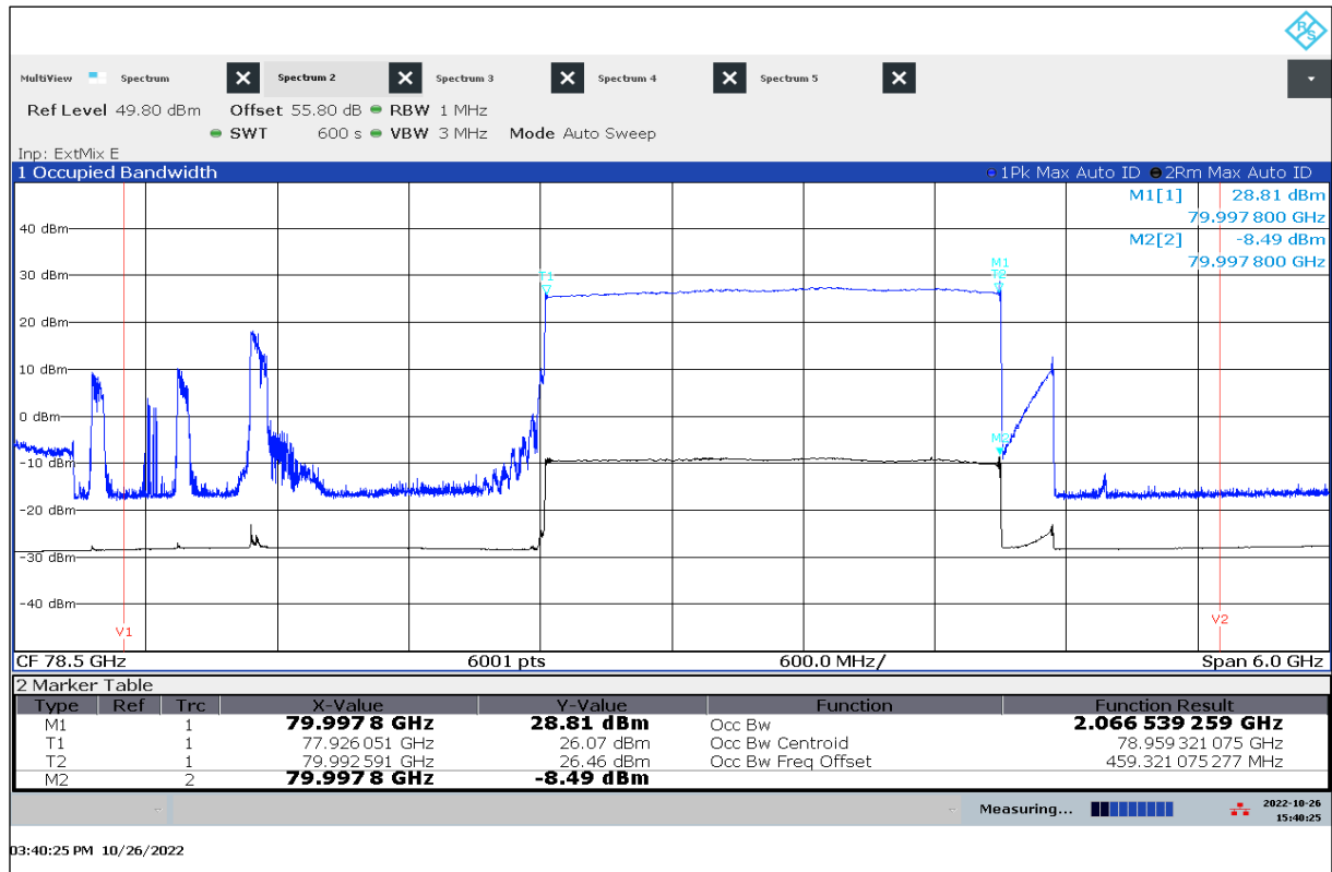
Plot 34: OBW, 0 °C / V_{nom}
