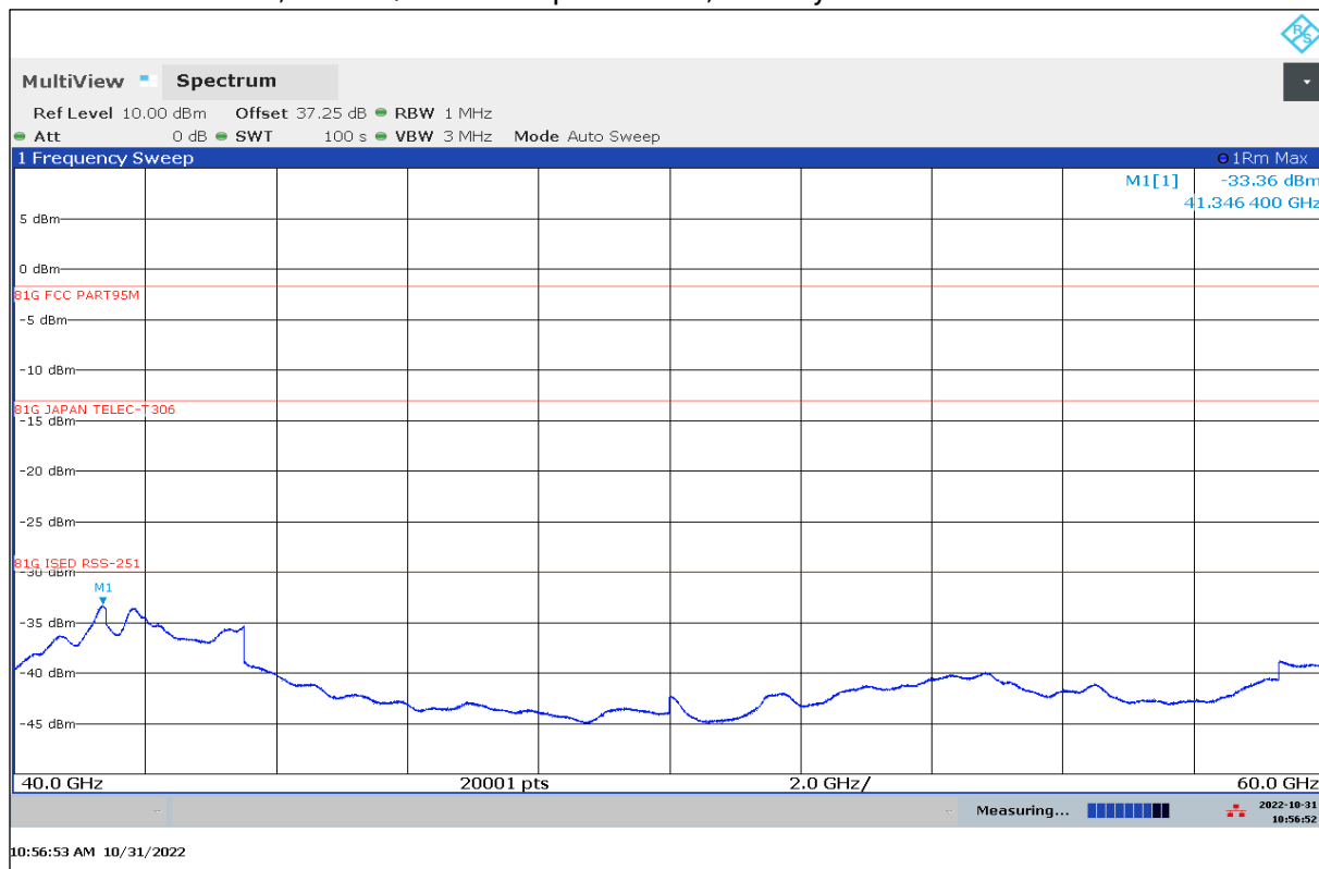
Plot 22: 40 GHz – 60 GHz, vertical / horizontal polarization, Standby State
