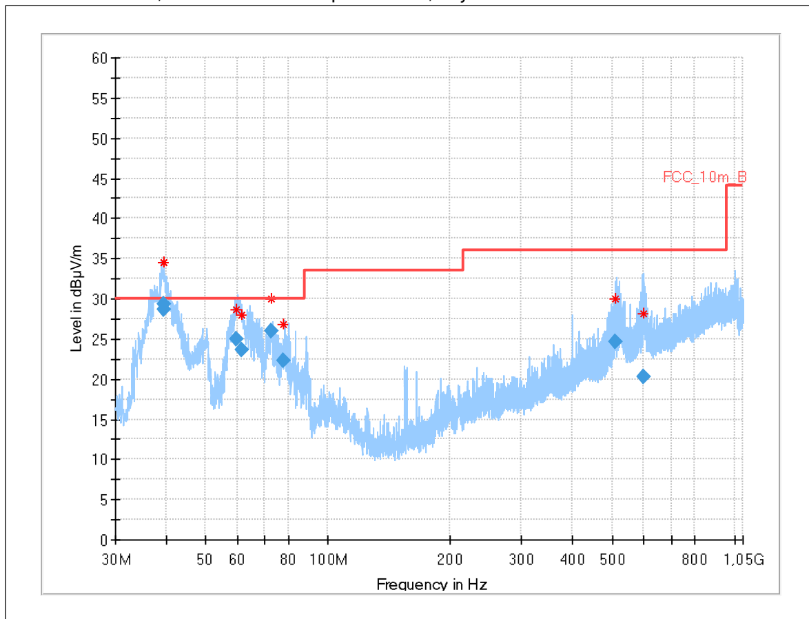
Plot 11: 30 MHz – 1 GHz, vertical / horizontal polarization, City Mode 3
