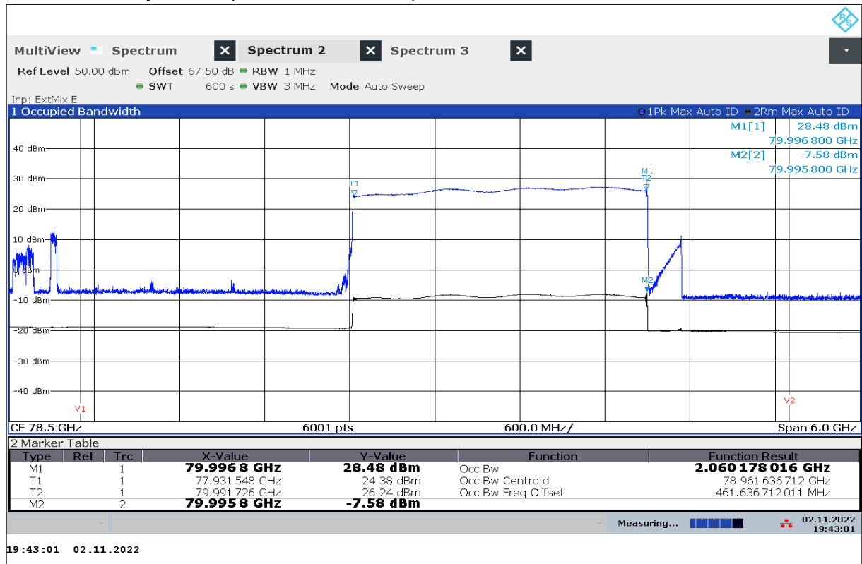
Plot 43: OBW with City Mode 3 (EUT On, Interferer On)
