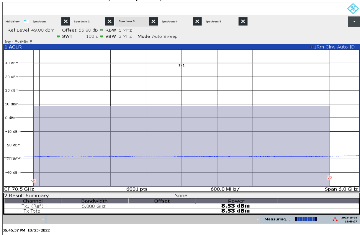
Plot 6: Mean Power, T nom / V min-max (StandBy State)
