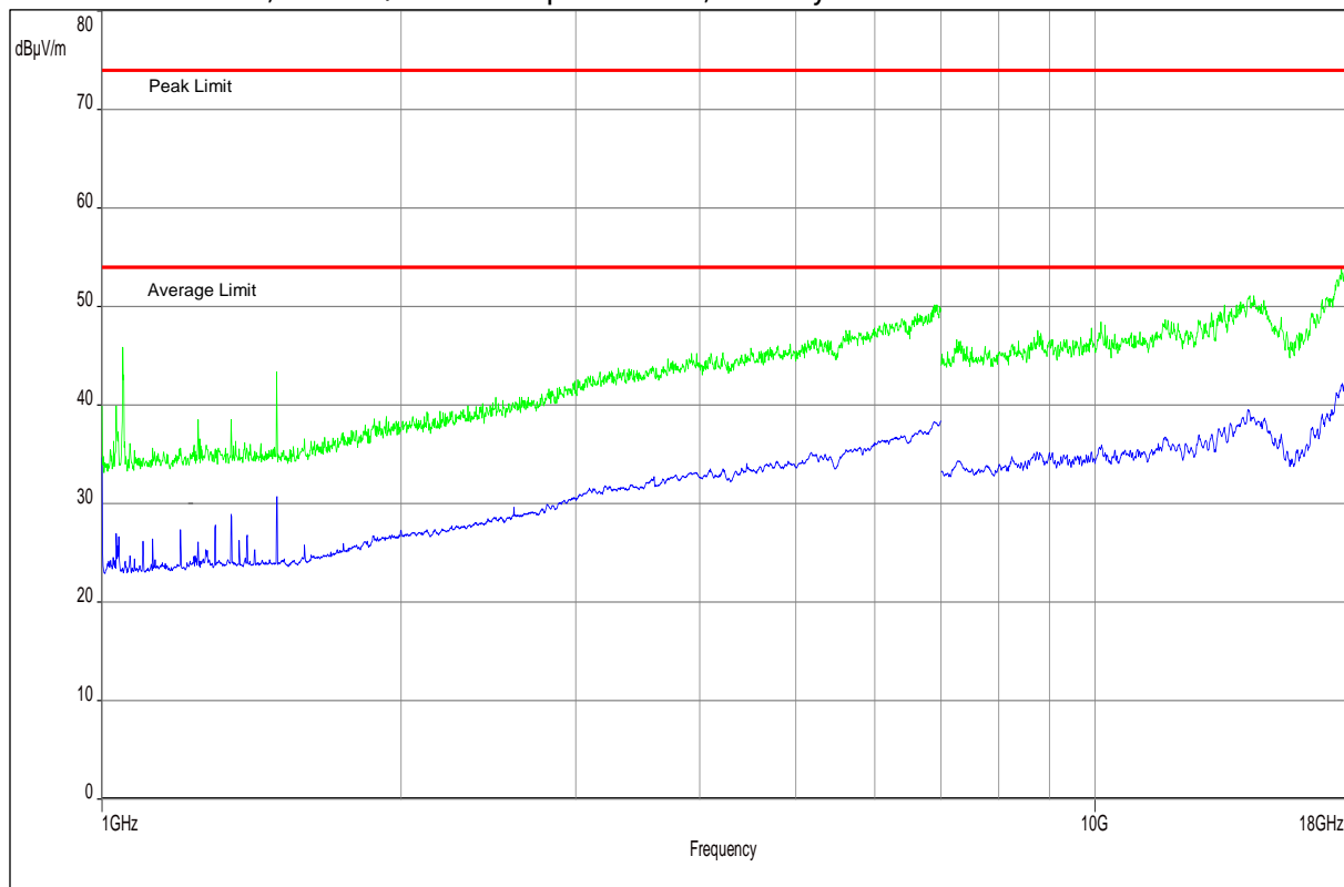
Plot 14: 1 GHz – 18 GHz, vertical / horizontal polarization, Standby State
