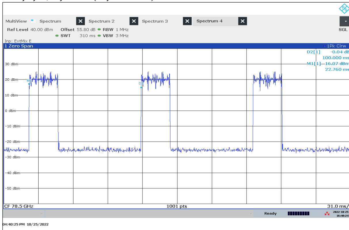
Plot 7: Duty Cycle, City Mode 3 (only informative)
