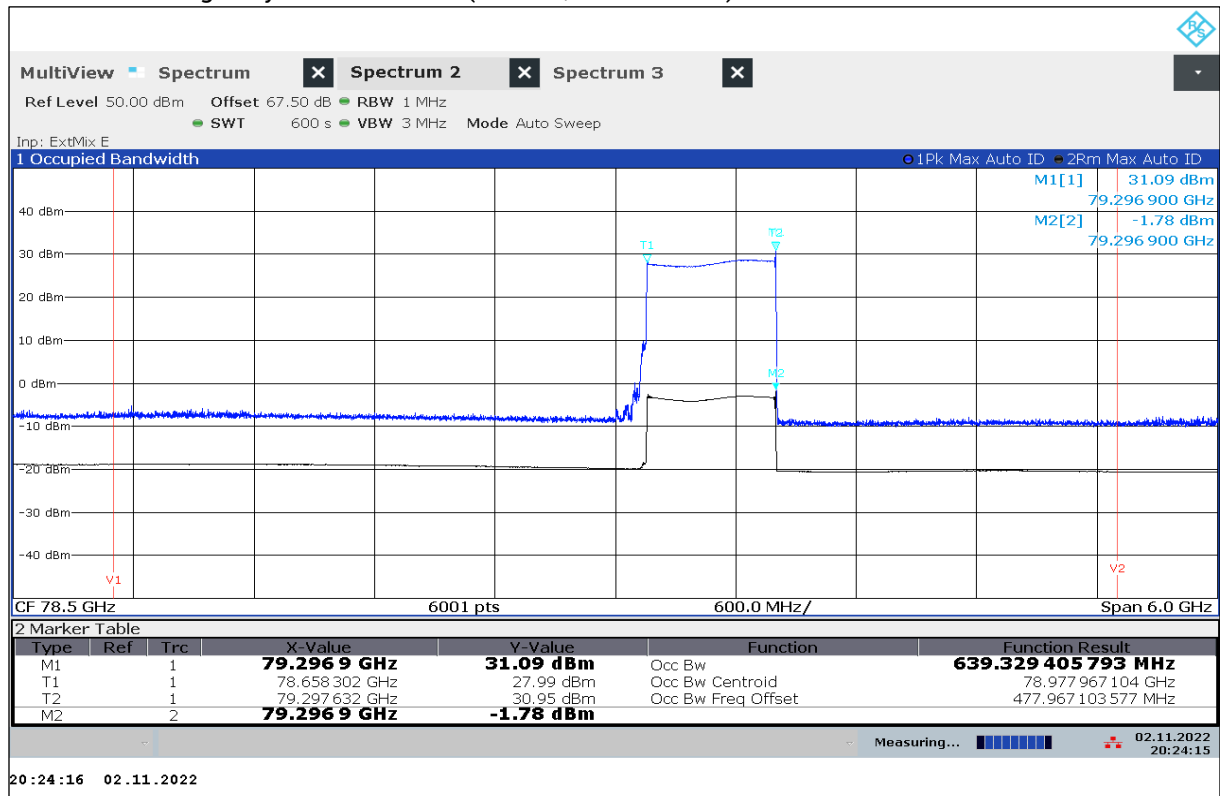
Plot 46: OBW with Highway Traffic Mode 3 (EUT On, Interferer On)
