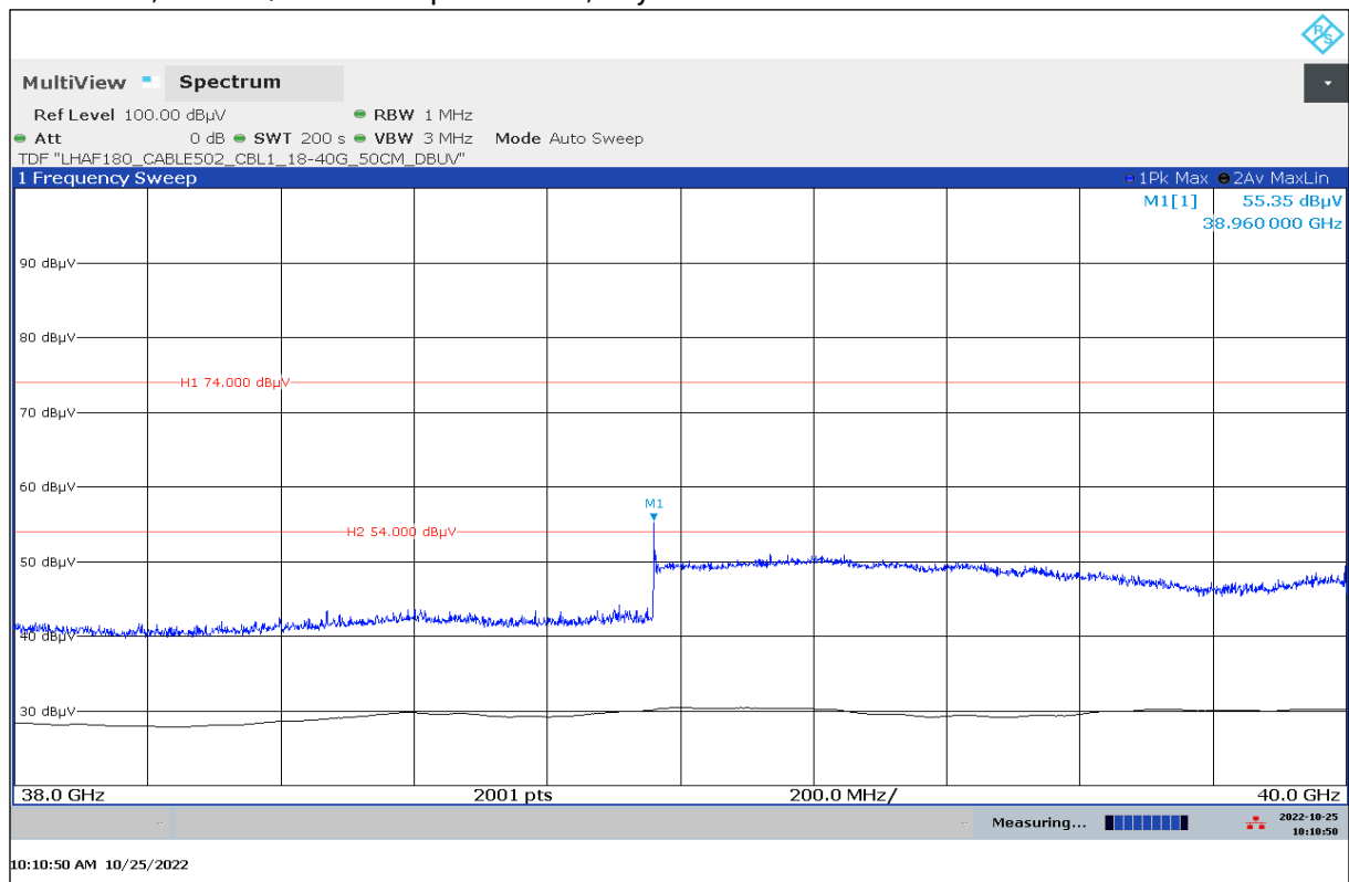
Plot 16: 38 GHz, vertical / horizontal polarization, City Mode 3
