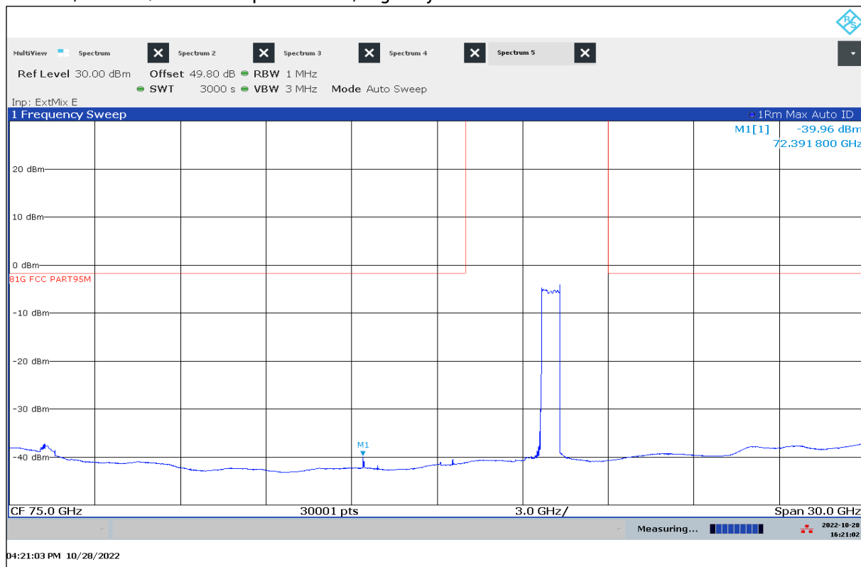
Plot 24: OOB, vertical / horizontal polarization, Highway Traffic Mode 3
