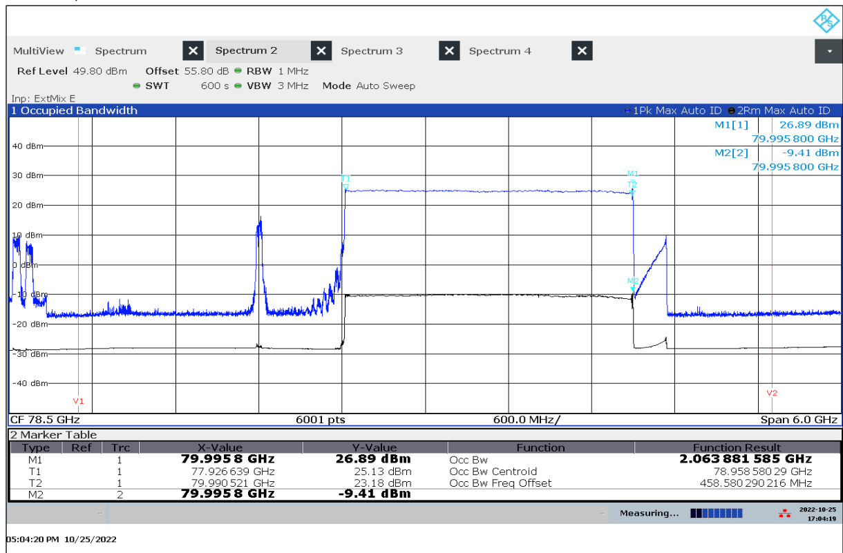
Plot 36: OBW, 20 °C / V min-max
