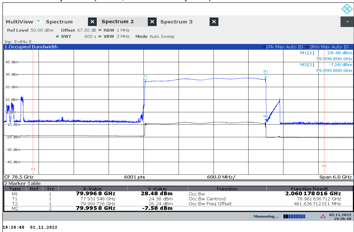
Plot 42: OBW with City Mode 3 (EUT On, Interferer Standby State)
