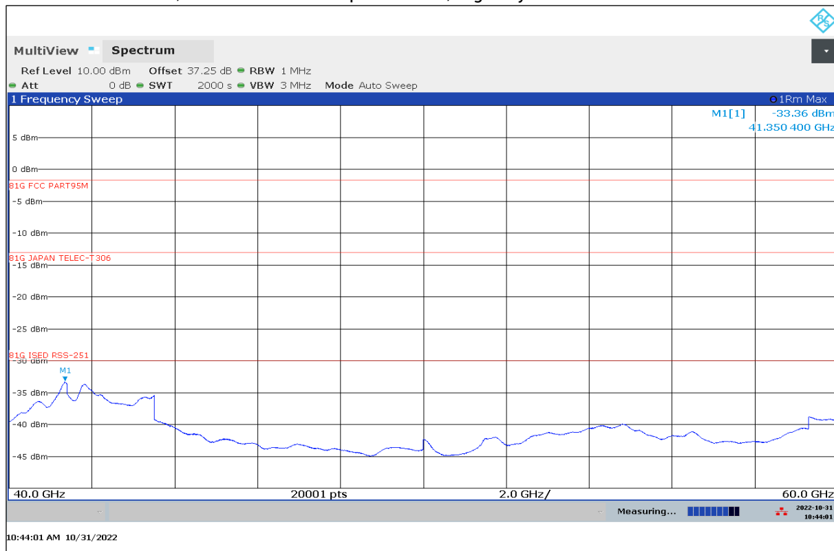
Plot 21: 40 GHz – 60 GHz, vertical / horizontal polarization, Highway Traffic Mode 3
