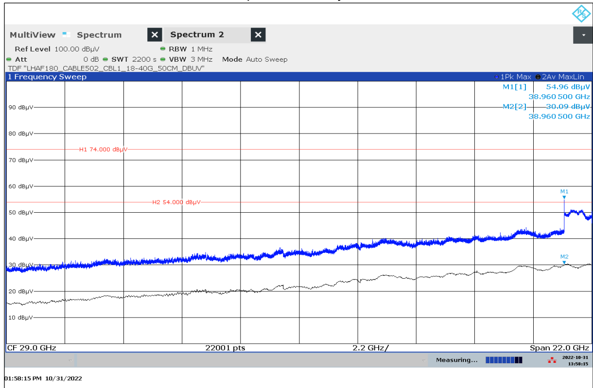
Plot 15: 18 GHz – 40 GHz, vertical / horizontal polarization, City Mode 3
