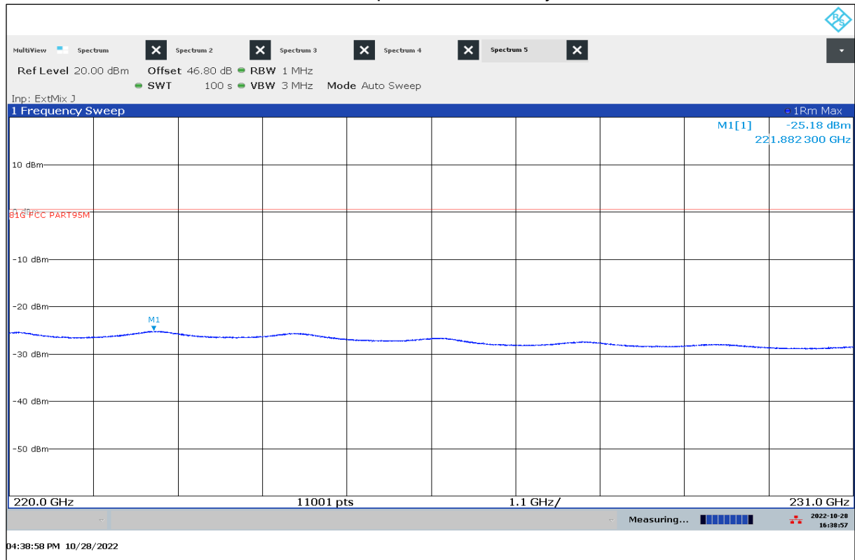
Plot 31: 220 GHz – 231 GHz, vertical / horizontal polarization, Standby State
