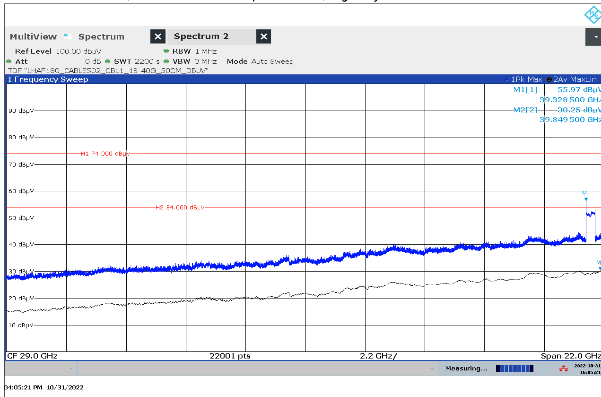
Plot 17: 18 GHz – 40 GHz, vertical / horizontal polarization, Highway Traffic Mode 3
