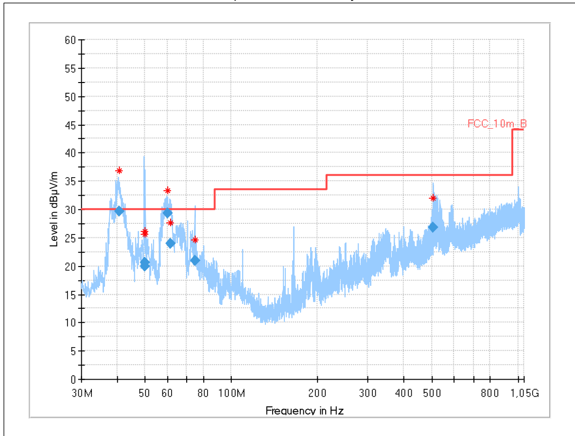
Plot 12: 30 MHz – 1 GHz, vertical / horizontal polarization, Standby State
