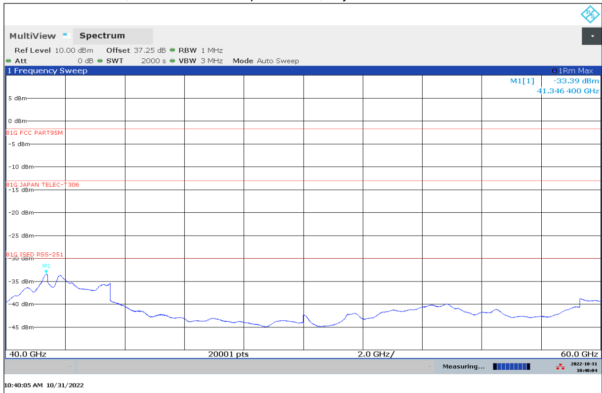
Plot 20: 40 GHz – 60 GHz, vertical / horizontal polarization, City Mode 3
