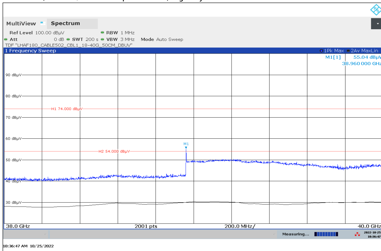
Plot 18: 38 GHz, vertical / horizontal polarization, Highway Traffic Mode 3
