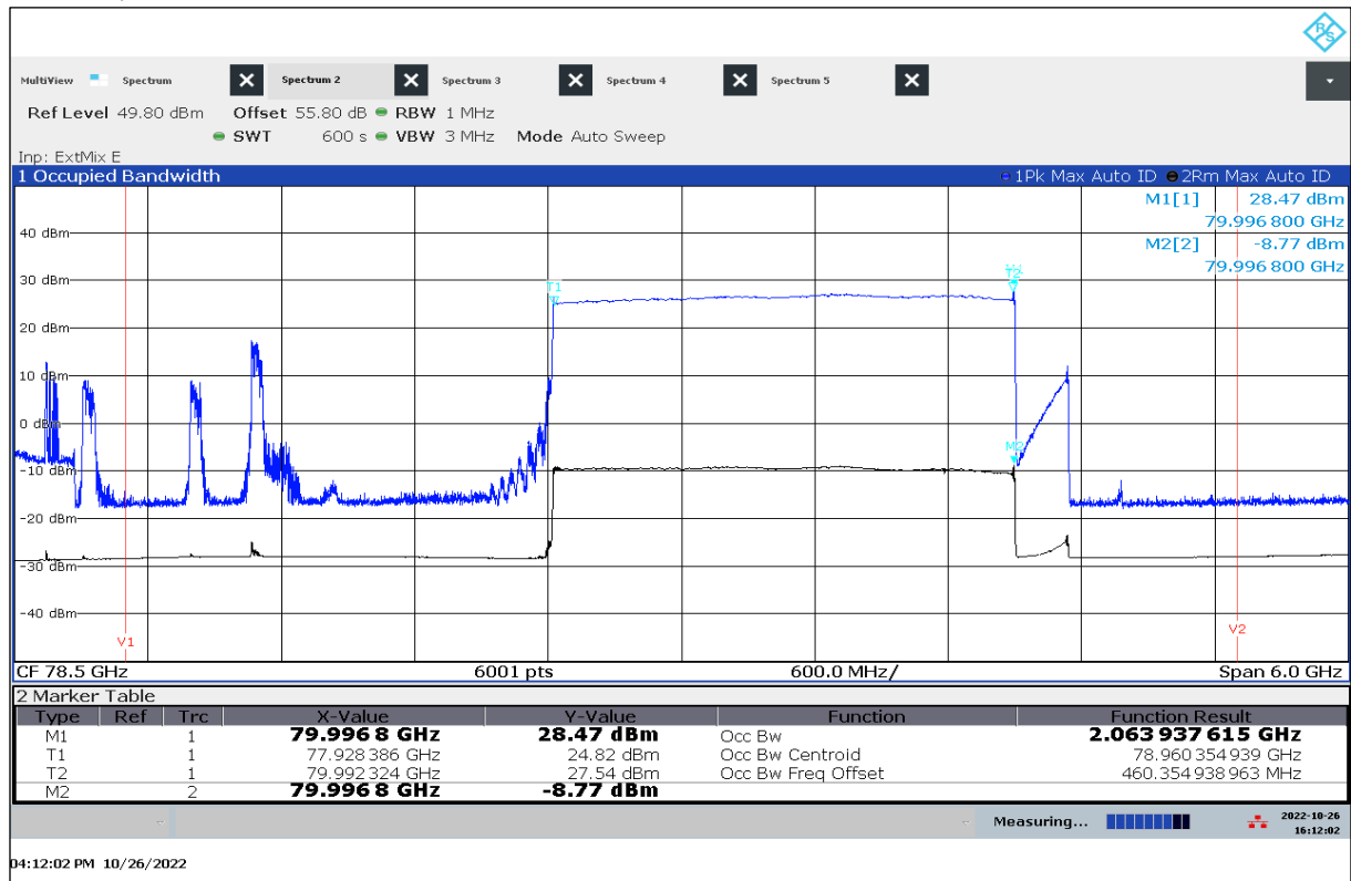
Plot 35: OBW, 10 °C / V_{nom}
