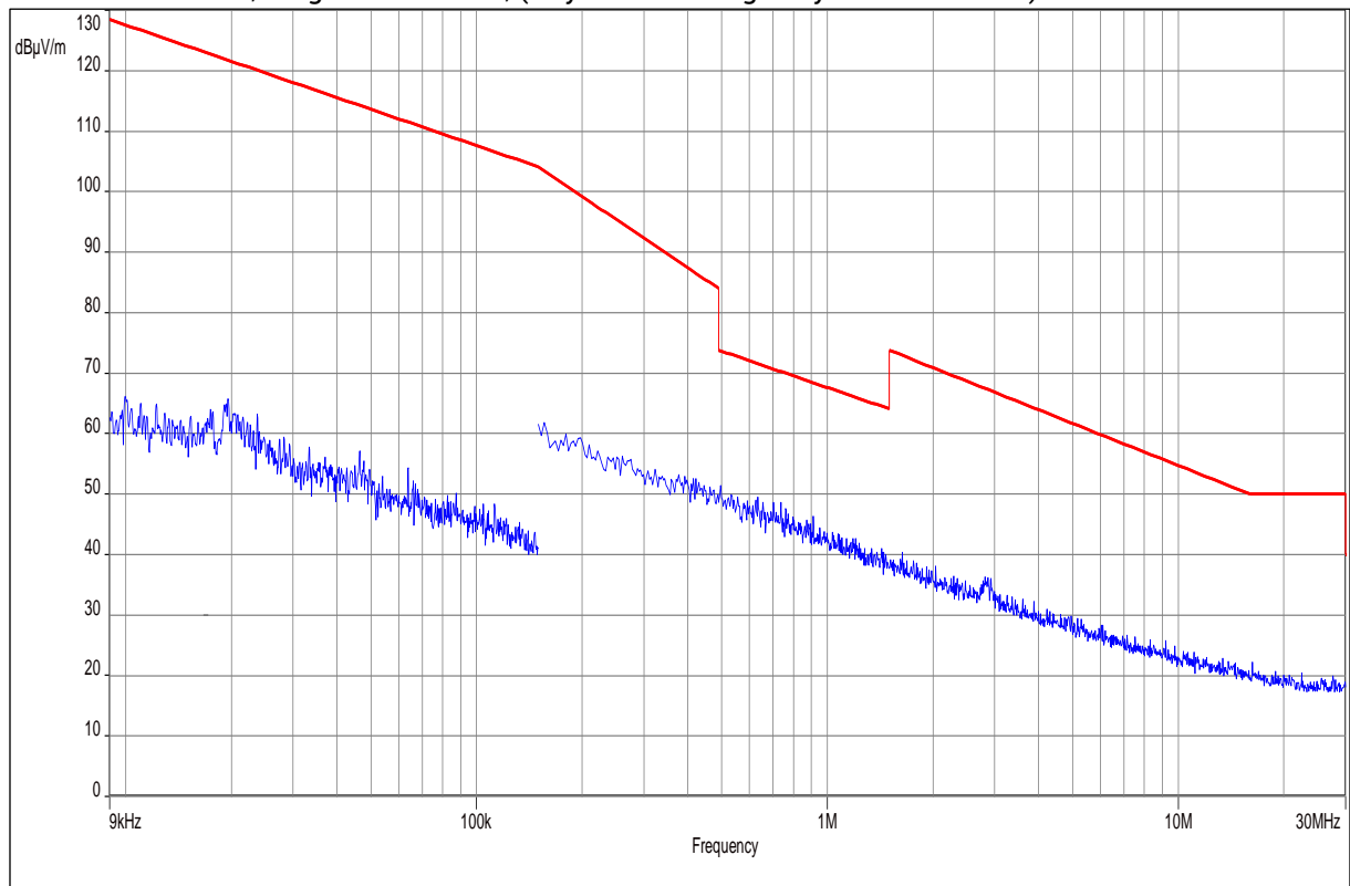
Plot 9: 9 kHz – 30 MHz, Magnetic antenna, (City Mode 3 / Highway Traffic Mode 3)
