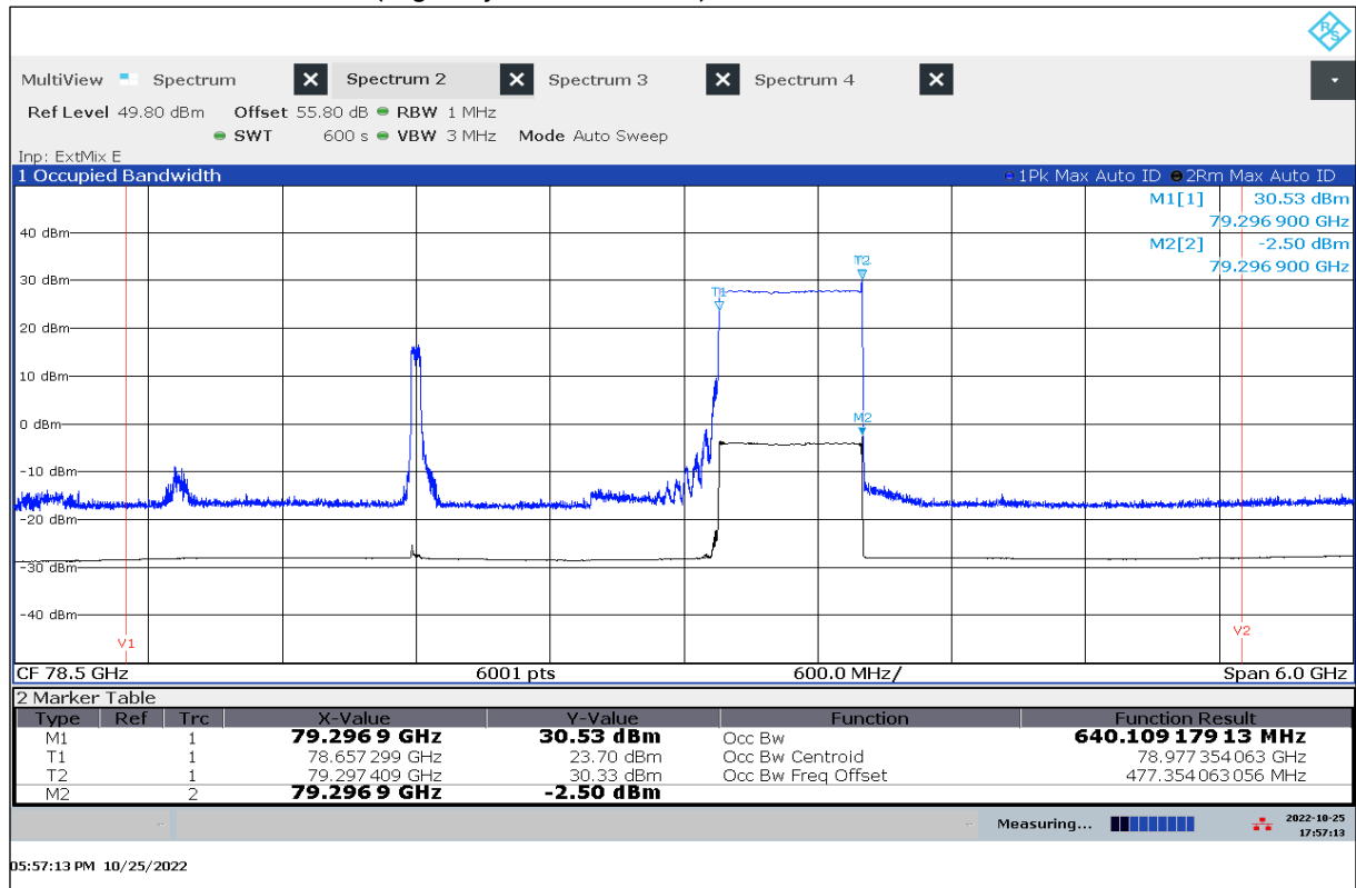
Plot 3: OBW, PSD, T_{\text{nom}} / V_{\text{min-max}} (Highway Traffic Mode 3)
