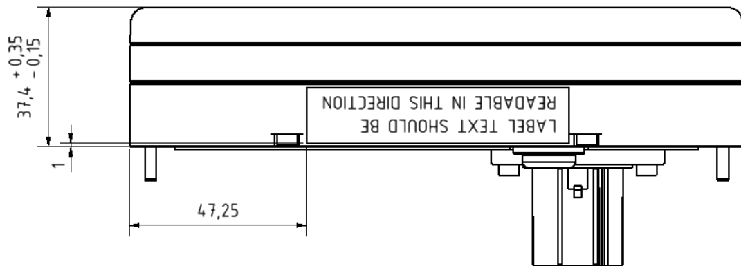
Label Location
