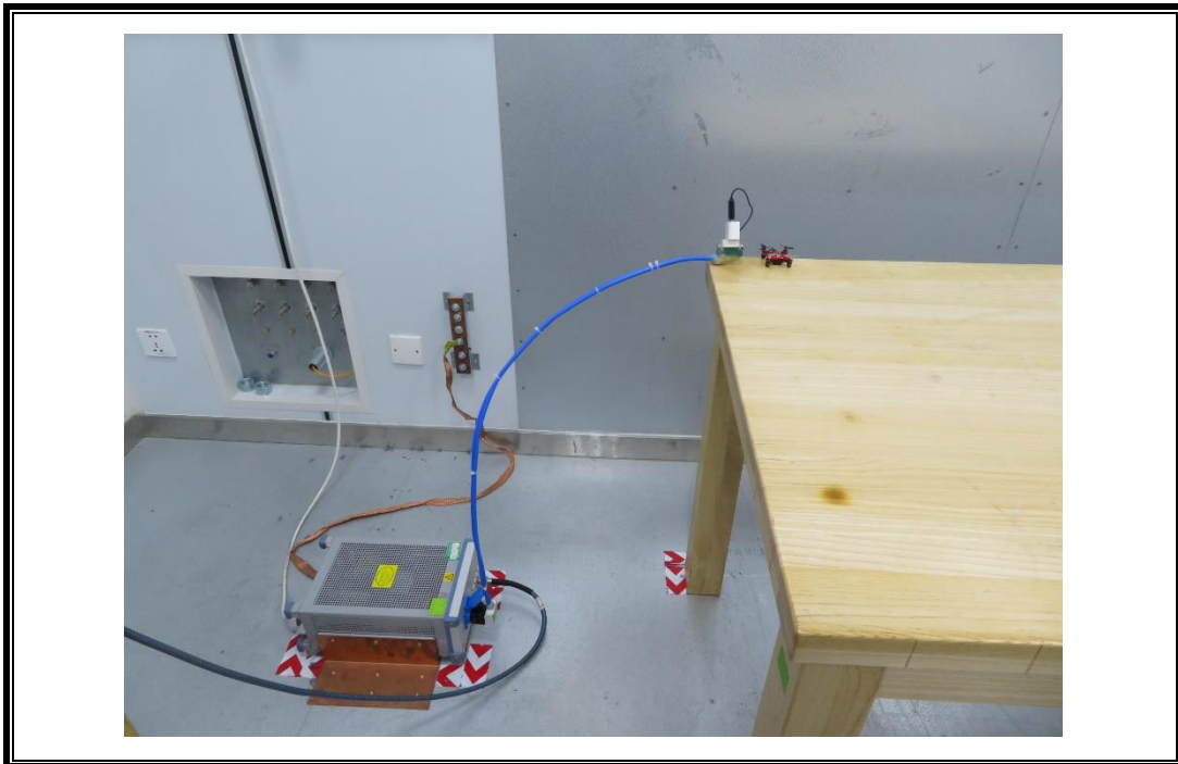
AC POWER LINE CONDUCTED EMISSIONS SETUP
