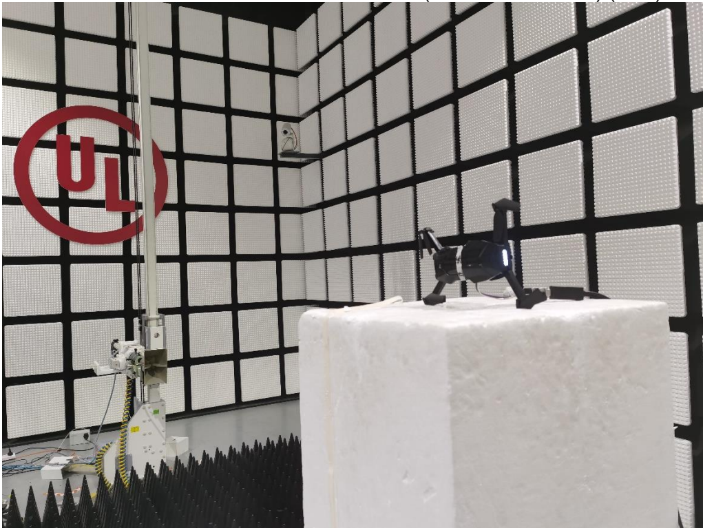
RADIATED RF MEASUREMENT SETUP (Above 1G – Z axis) (WiFi)
