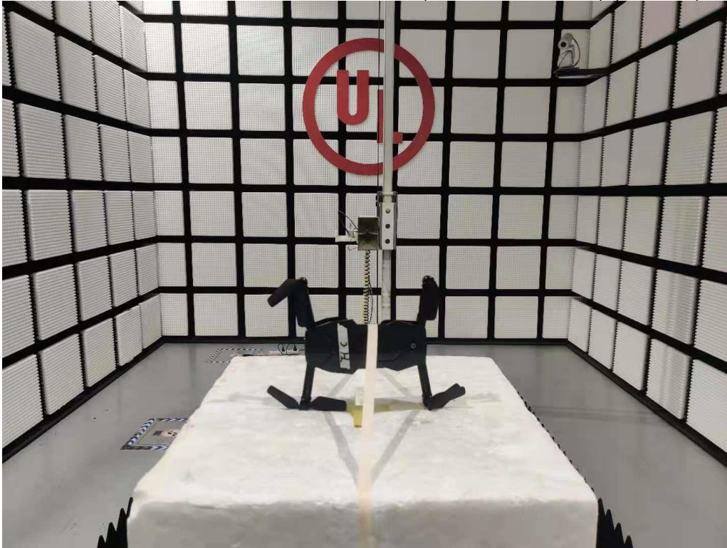
Radiated Disturbance Below 1 GHz and Above 30 MHz (WiFi)
