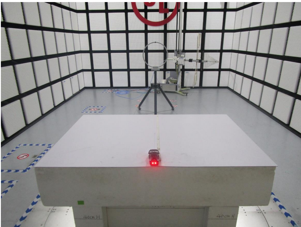
Radiated Disturbance Below 30 MHz (2.4 GHz)
