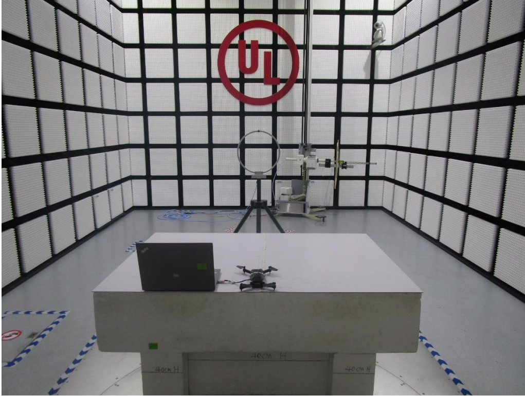
Radiated Disturbance Below 30 MHz (WiFi)
