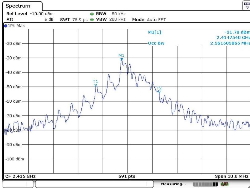
99% OCCUPIED BANDWIDTH LOW CH
