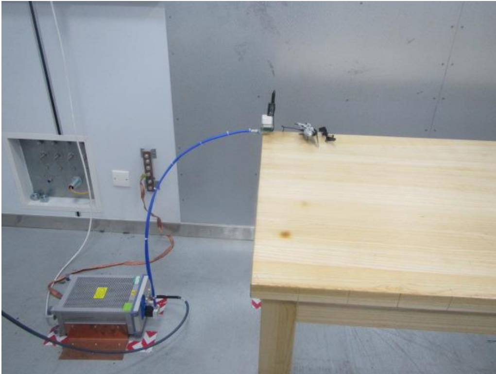
Conducted Disturbance
