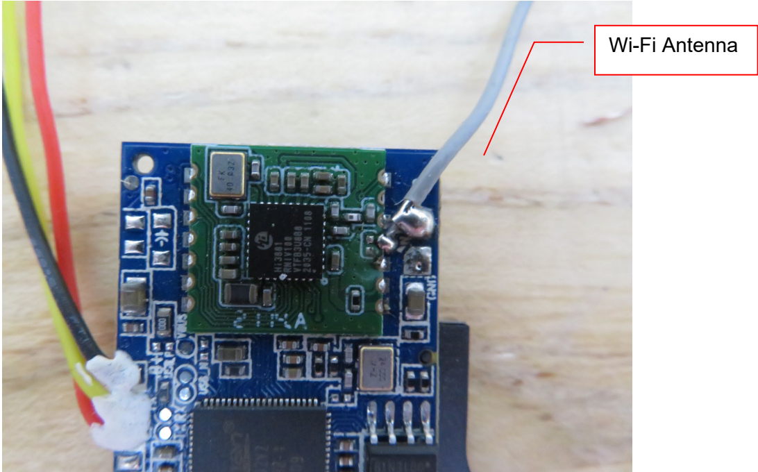
Internal View of EUT-8
