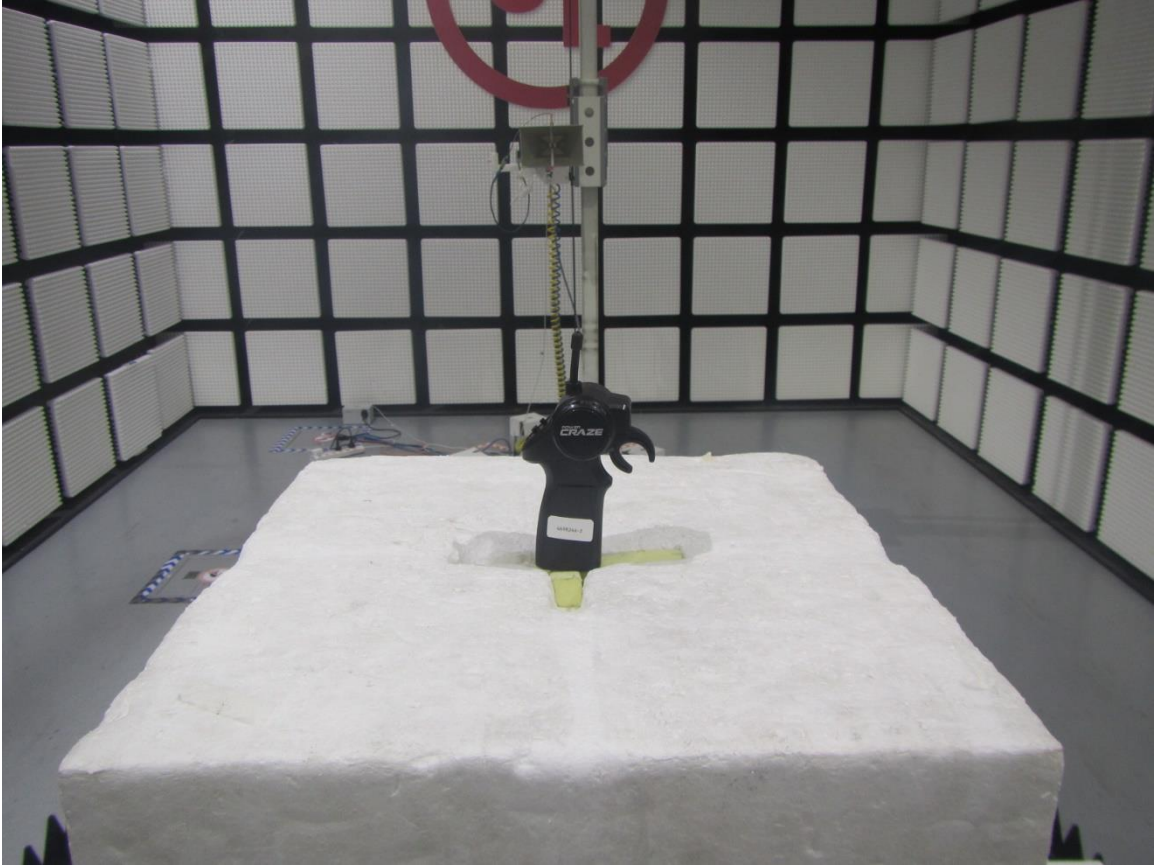
Radiated Disturbance Setup (Above 1 GHz – X axis)
