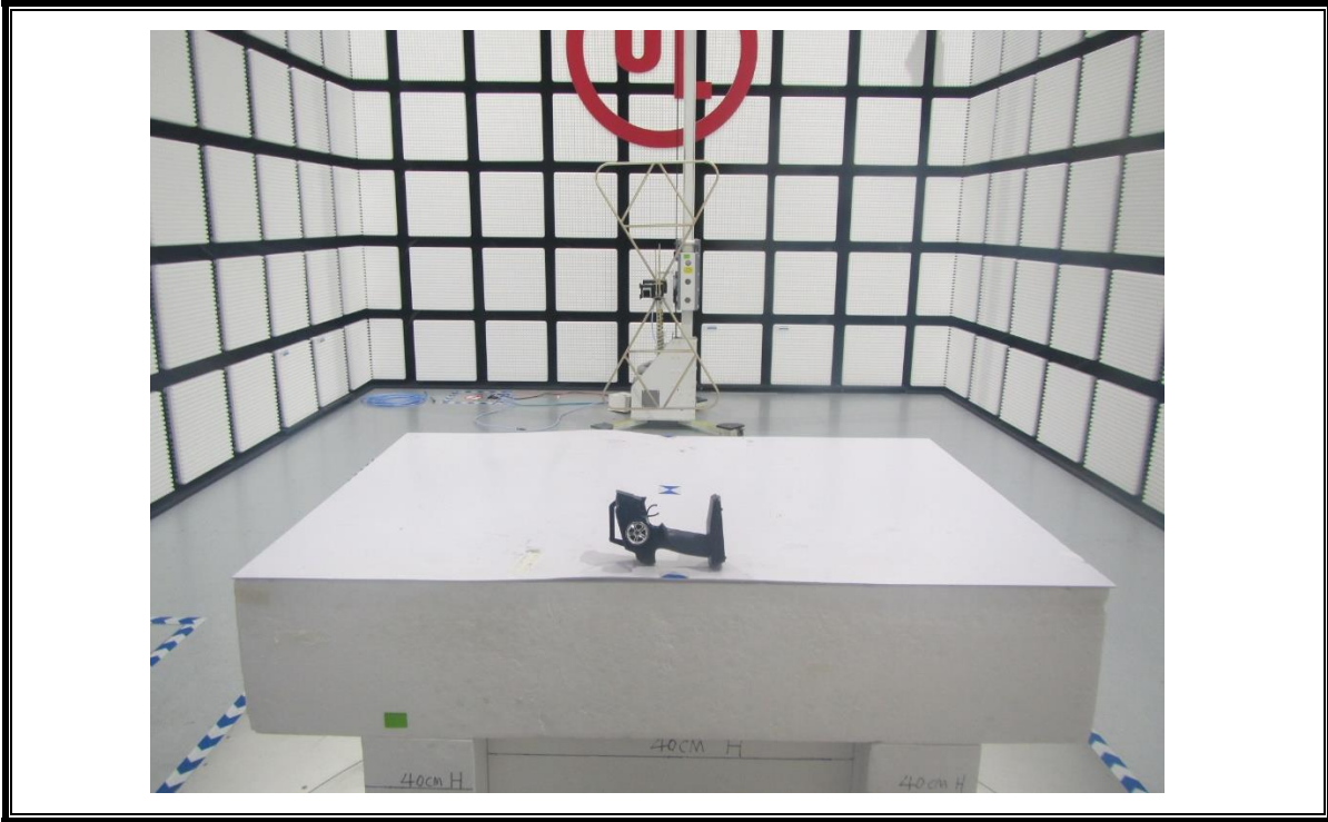
RADIATED RF MEASUREMENT SETUP (30MHz ~ 1 GHz)
