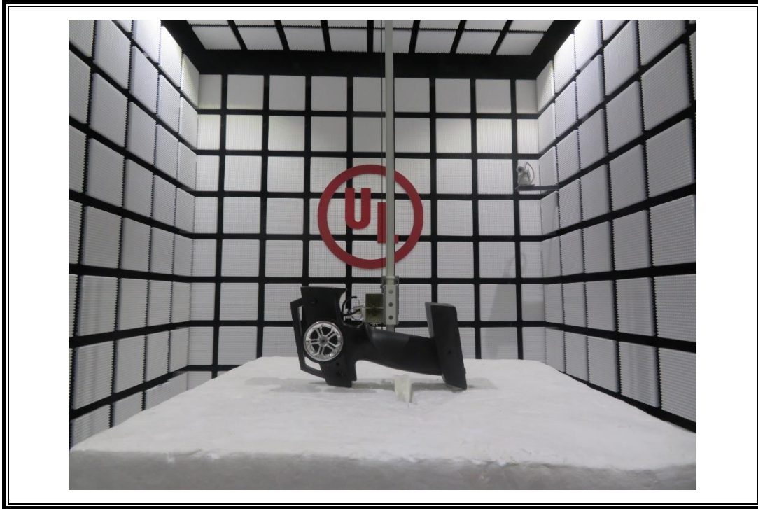
RADIATED RF MEASUREMENT SETUP (Above 1G – Z axis)
