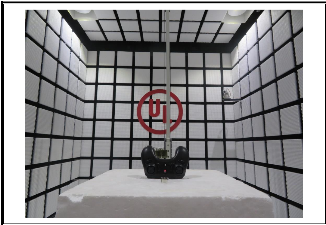
RADIATED RF MEASUREMENT SETUP (Above 1G – Z axis)
