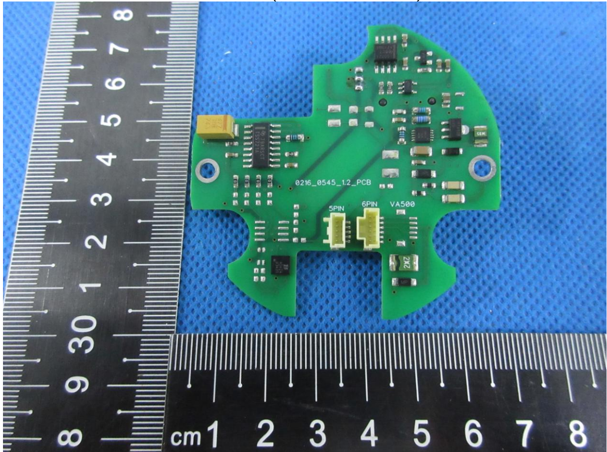
Photo16 (Model 3: S402 M-Bus)
