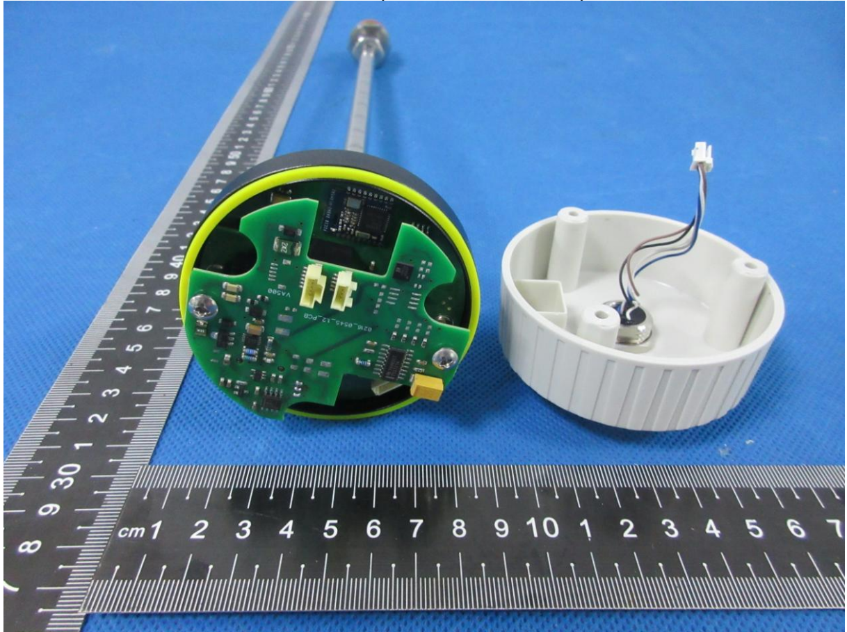
Photo14 (Model 3: S402 M-Bus)
