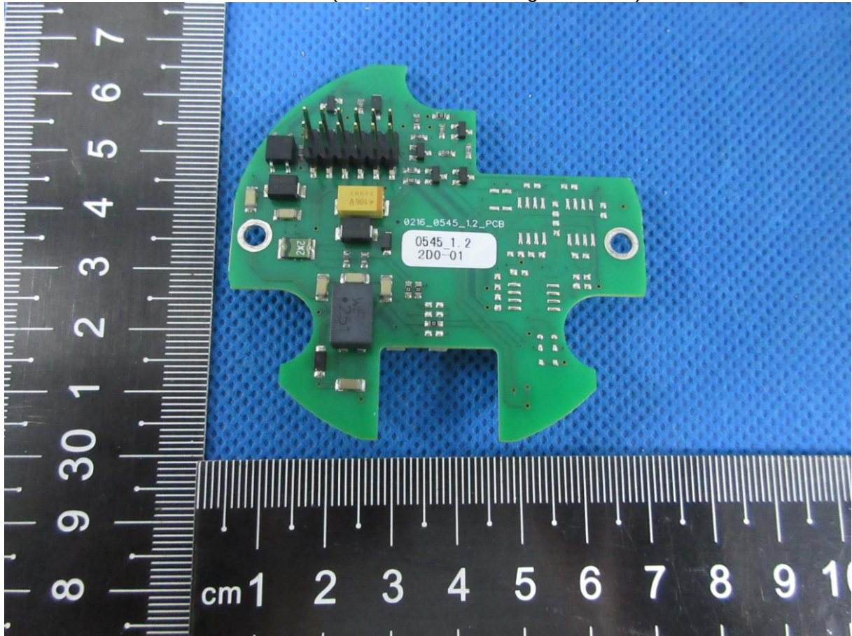
Photo10 (Model 2: S402 Analog and Pulse)
