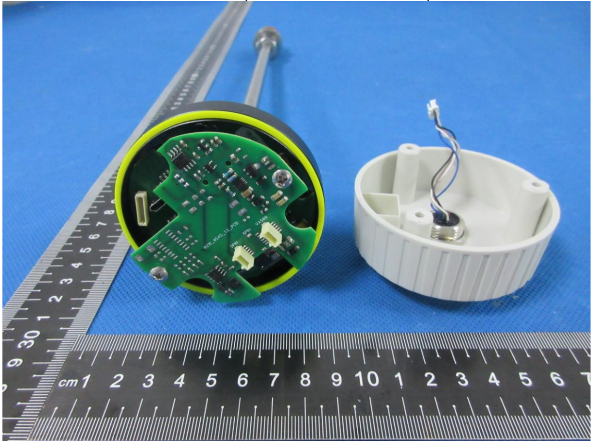
Photo2 (Model 1: S402 Modbus RTU)
