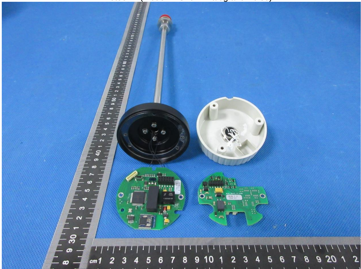
Photo8 (Model 2: S402 Analog and Pulse)
