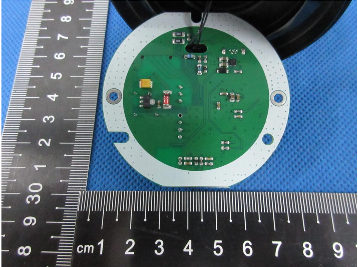
Photo6 (Model 1: S402 Modbus RTU)
