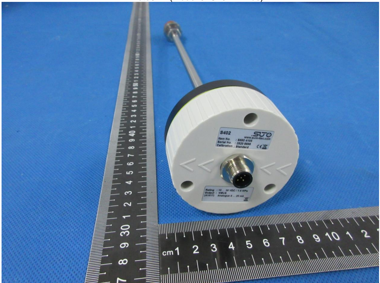
Photo6 (Model 3: S402 M-Bus)
