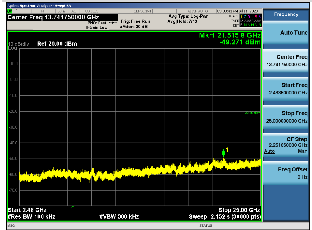
Test_Graph_ANT1_2441_1Mbps_Higher Band Emissions
