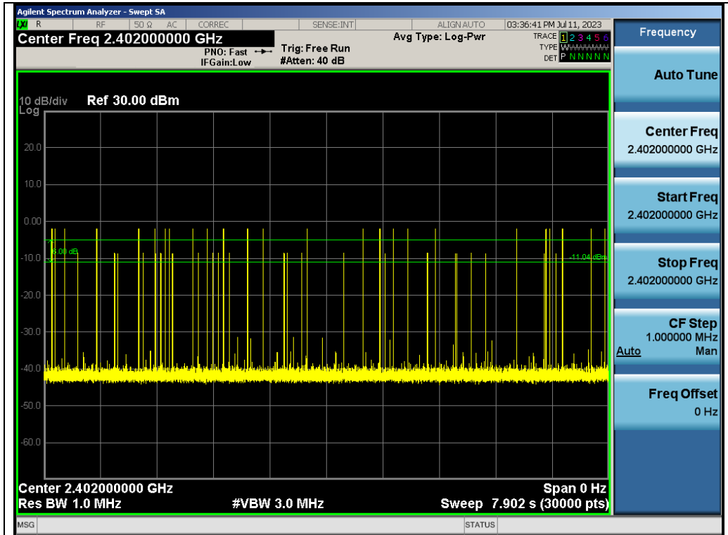
Test_Graph_HOP_ANT1_NA_1Mbps_2402_Number of Burst
