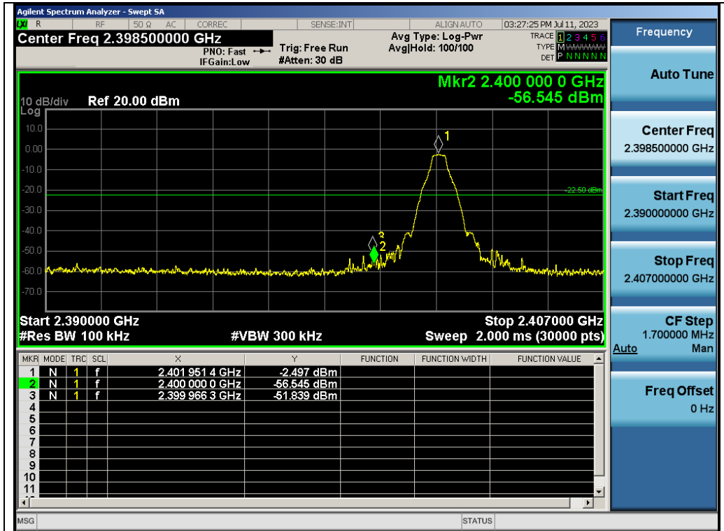
Test_Graph_ANT1_2402_1Mbps_Lower Band Edge Emissions
