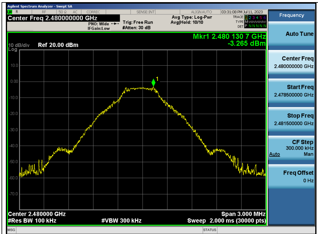
Test_Graph_ANT1_2480_1Mbps_Reference Level
