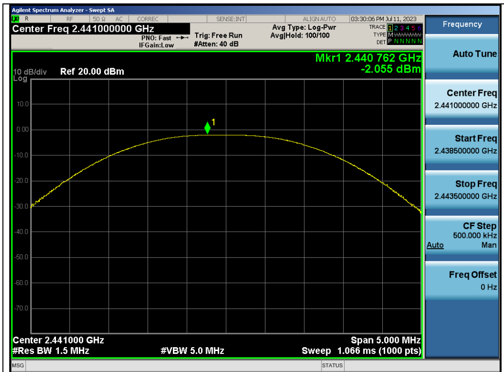
Test_Graph_ANT1_2441_1Mbps_Peak Power
