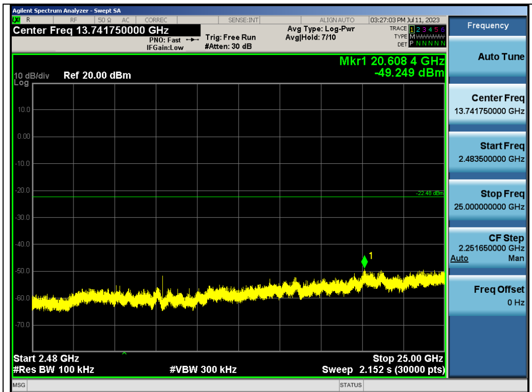
Test_Graph_ANT1_2402_1Mbps_Higher Band Emissions
