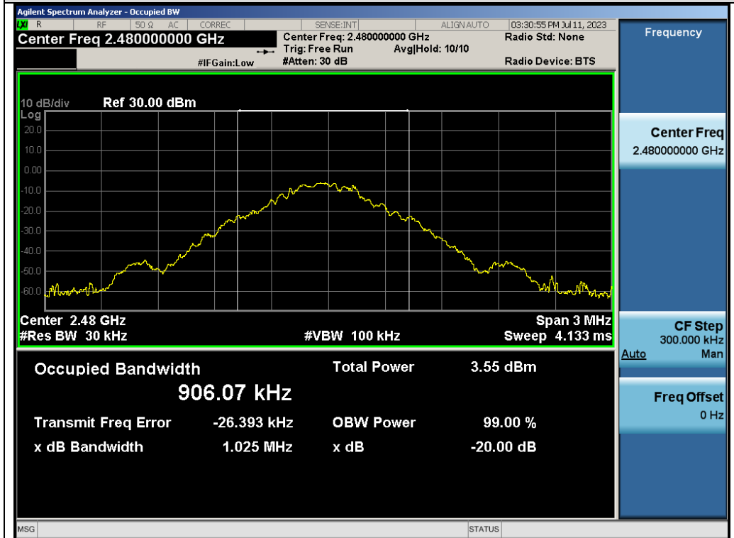
Test_Graph_ANT1_2480_1Mbps_OBW
