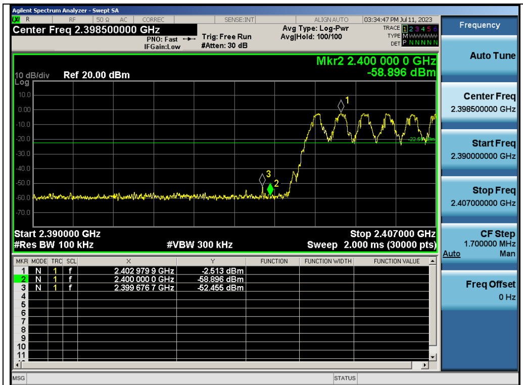
Test_Graph_HOP_ANT1_NA_1Mbps_Lower Band Edge Emissions
