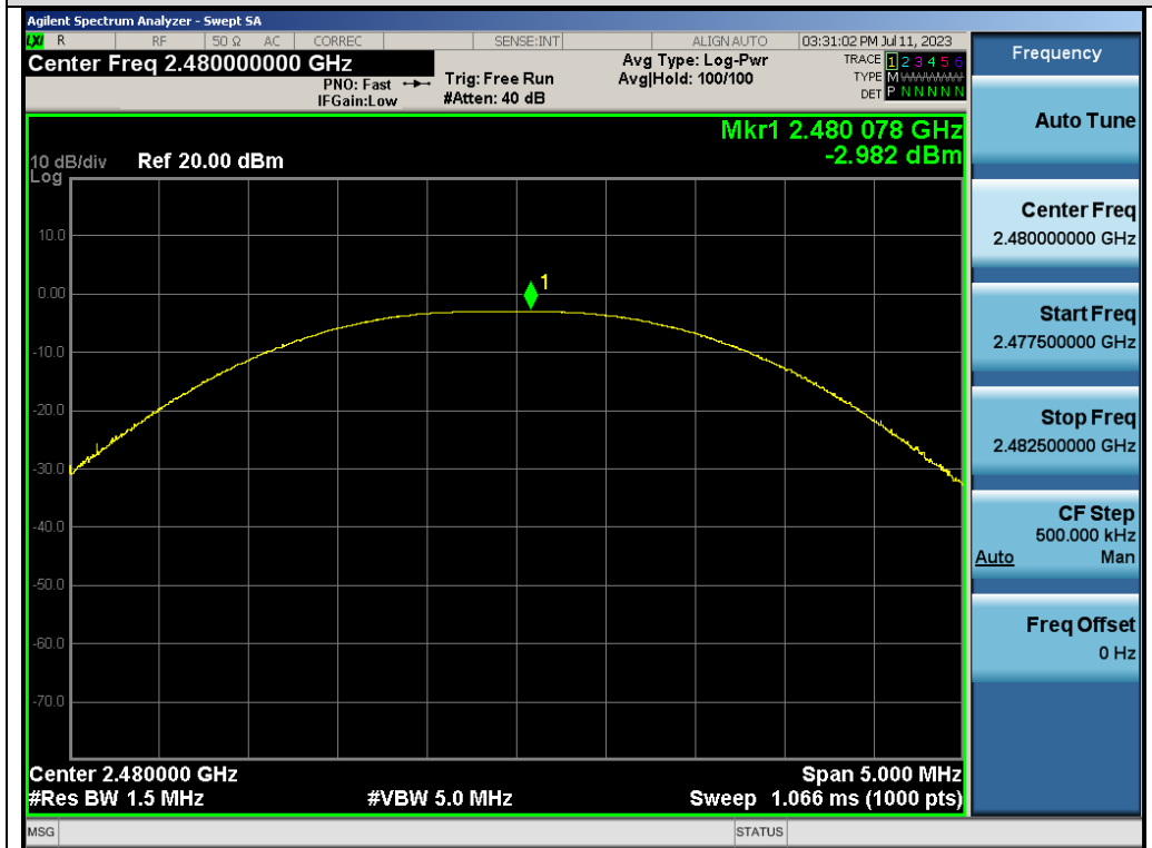
Test_Graph_ANT1_2480_1Mbps_Peak Power
