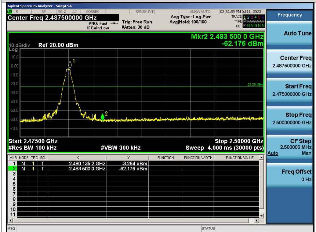
Test_Graph_ANT1_2480_1Mbps_Higher Band Edge Emissions
