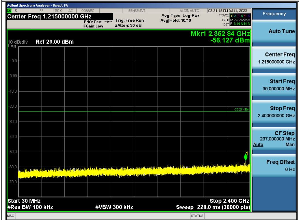
Test_Graph_ANT1_2480_1Mbps_Lower Band Emissions
