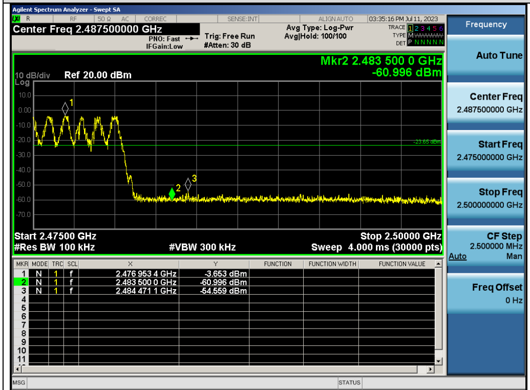
Test_Graph_HOP_ANT1_NA_1Mbps_Higher Band Edge Emissions
