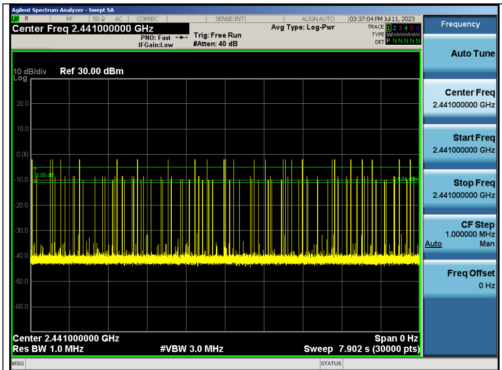
Test_Graph_HOP_ANT1_NA_1Mbps_2441_Number of Burst
