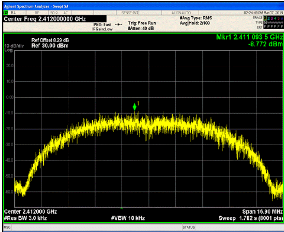
Mode: TX 11b channel 1
