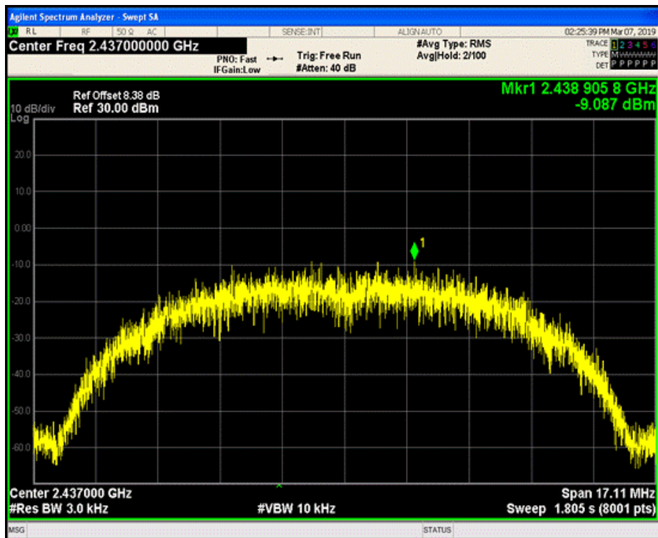
Mode: TX 11b channel 6
