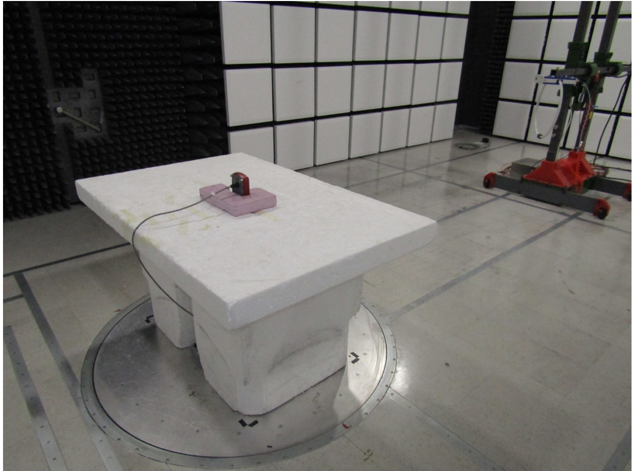
Figure 2: Radiated Emissions – Back – Below 30MHz
