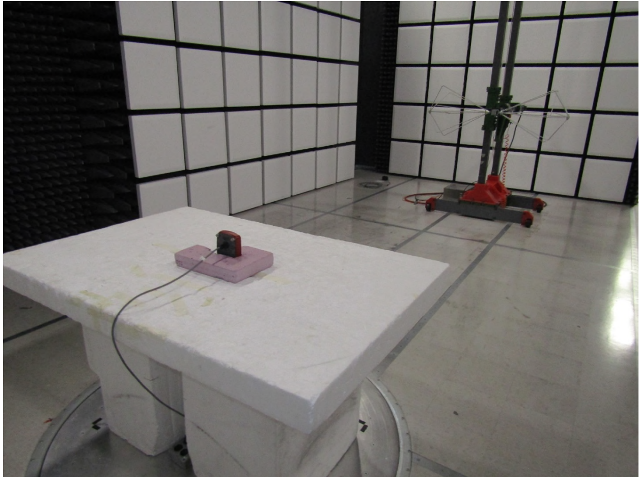
Figure 3: Radiated Emissions – Back – Above 30MHz
