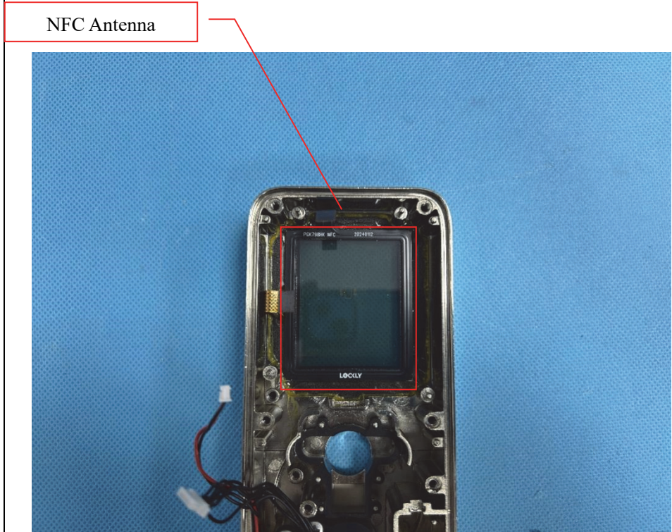
Antenna View 2
