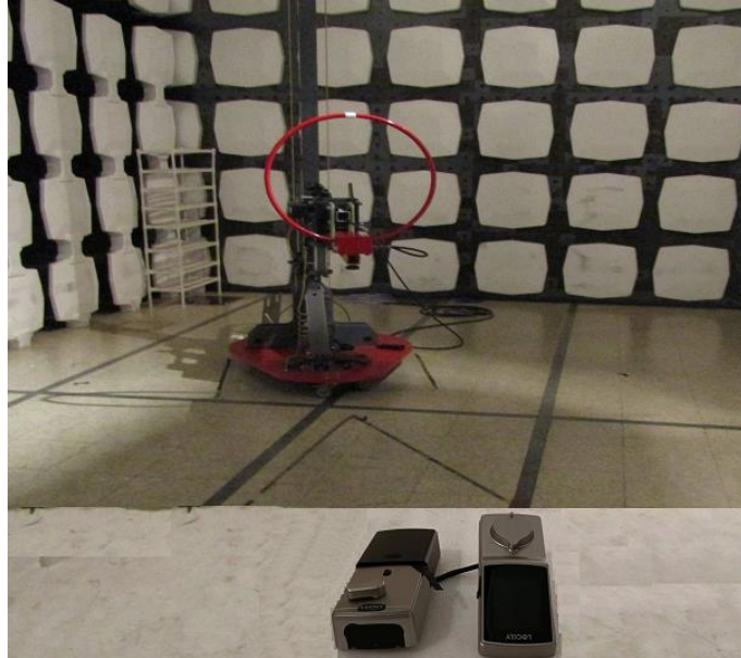
Measurement of Radiated Emission Test Set Up
