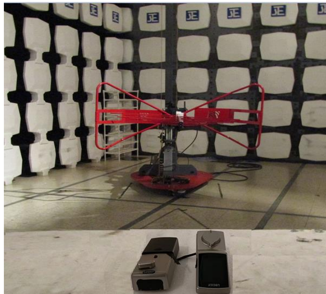
Measurement of Radiated Emission Test Set Up
