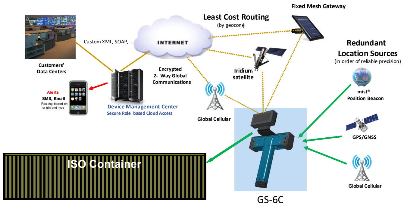
Figure 8 - GS-6C Communication Interfaces
