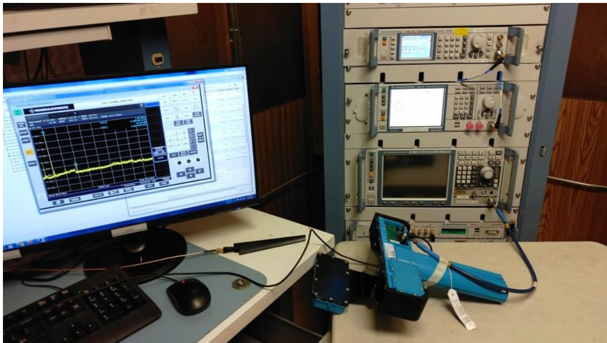
Figure 1: Equipment Under Test – Radiated Emissions – Antenna Port Conducted Measurements
