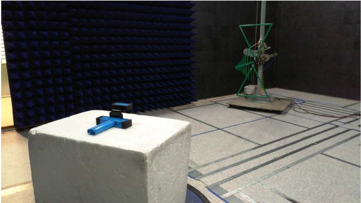
Figure 3: Equipment Under Test – Radiated Emissions <1GHz
