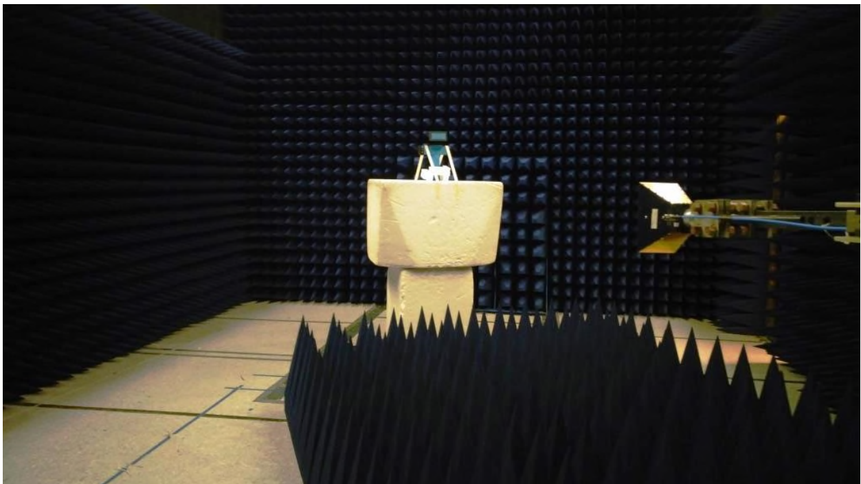
Figure 4: Equipment Under Test – Radiated Emissions >1GHz
