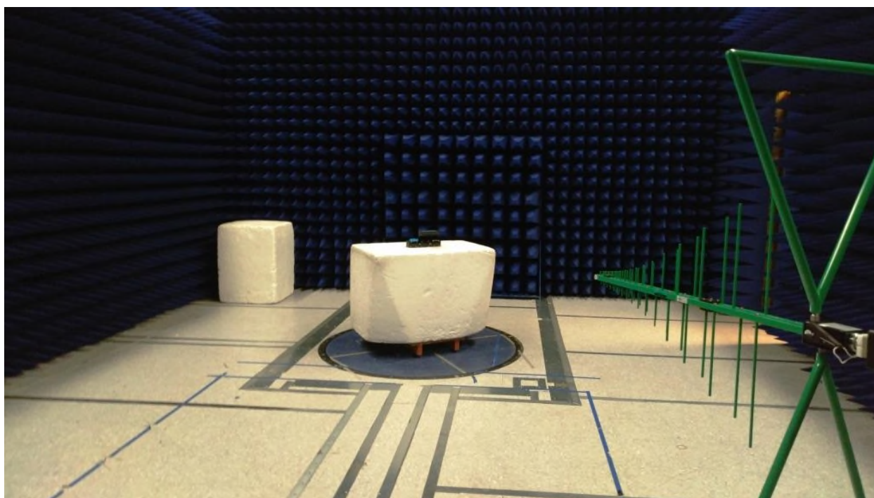
Figure 2: Equipment Under Test – Radiated Emissions <1GHz
