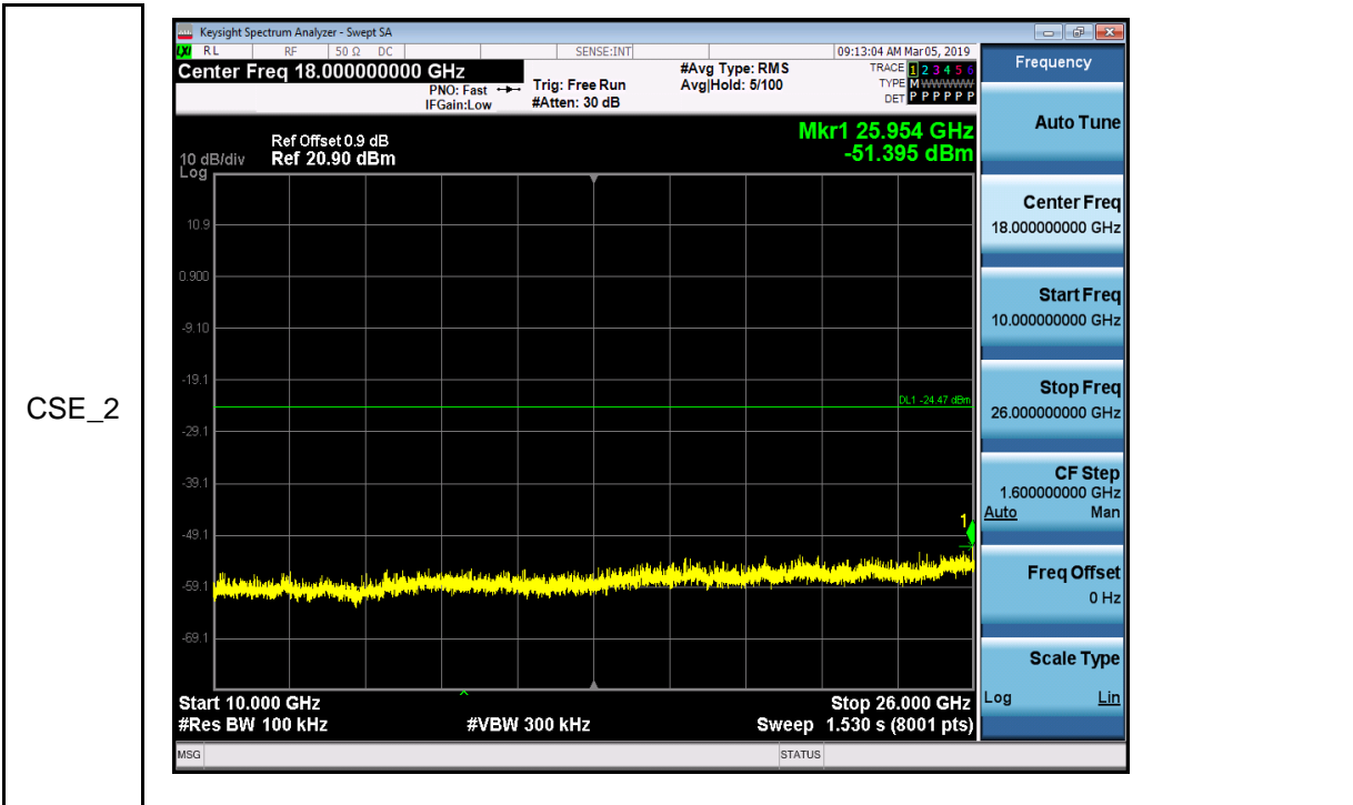
RF Conducted Spurious Emissions_DH5_2441
