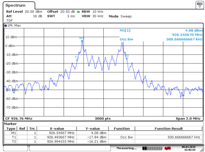
Figure 8.6-6: %99 occupied bandwidth on high channel
