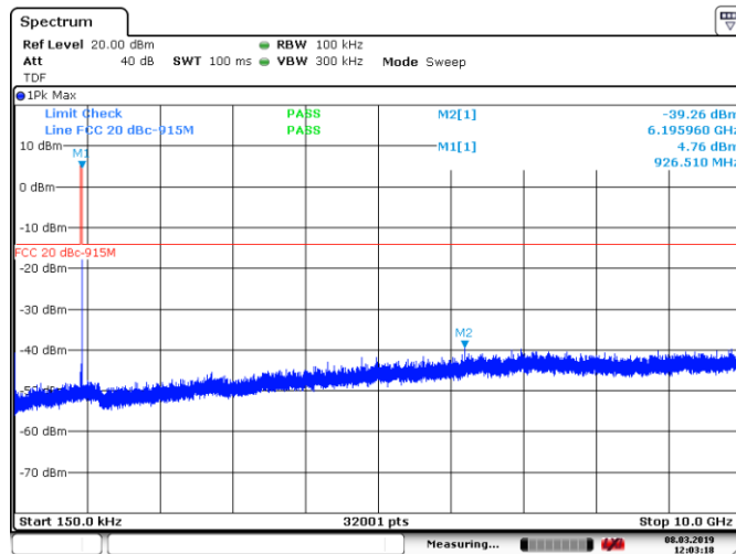
Figure 8.8-12: Conducted spurious emissions, Tx FHSS mode High channel
