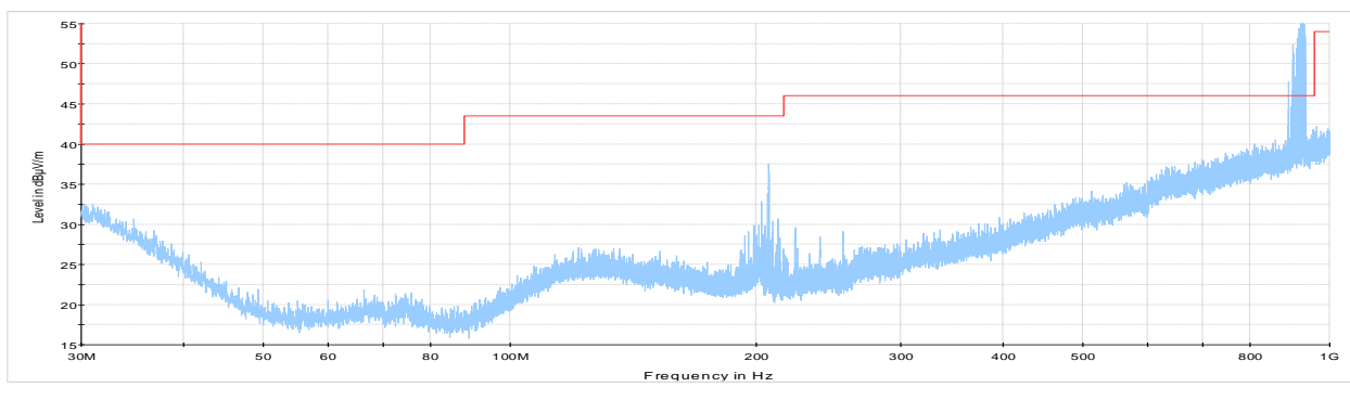
Figure 8.8-15: Radiated spurious emissions 30 MHz to 1 GHz, Tx DTS mode hi channel with external antenna
