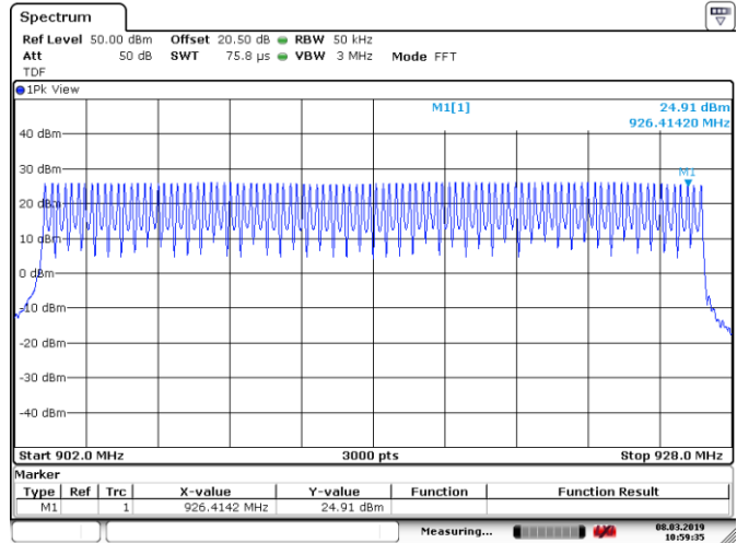
Figure 8.4-8: Number of hopping channels
