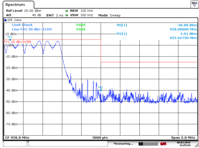
Figure 8.8-6: Conducted spurious emissions at upper band edge, Hopping mode
