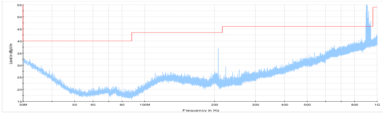
Figure 8.8-13: Radiated spurious emissions 30 MHz to 1 GHz, Tx DTS mode Low channel with external antenna
