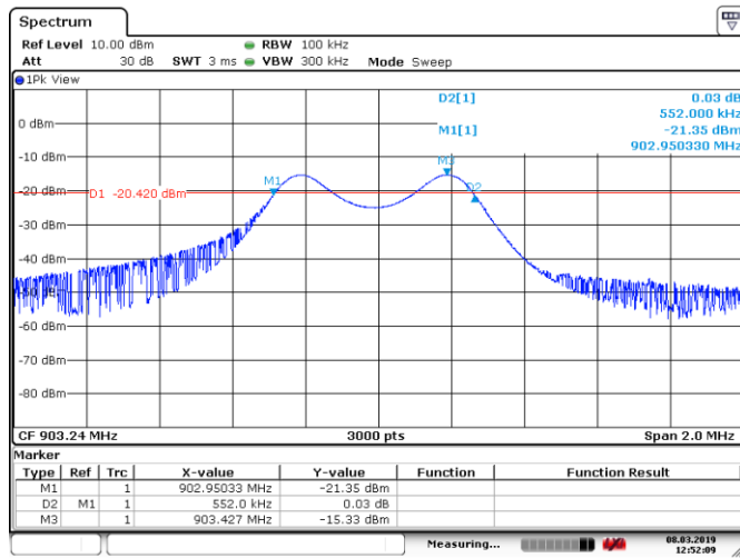
Figure 8.6-1: 6 dB bandwidth on low channel
