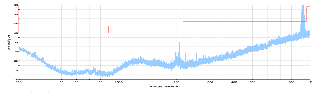
Figure 8.8-14: Radiated spurious emissions 30 MHz to 1 GHz, Tx DTS mode mid channel with external antenna
