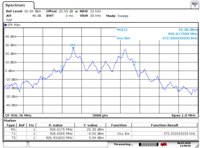
Figure 8.4-6: %99 occupied bandwidth on high channel
