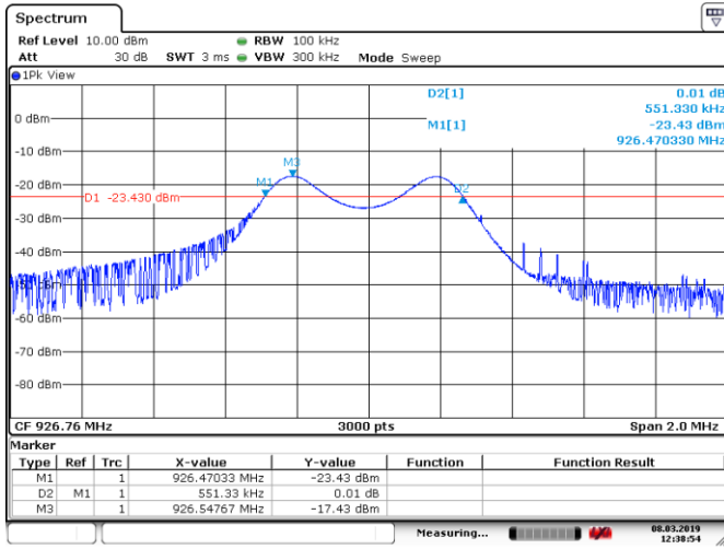
Figure 8.6-3: 6 dB bandwidth on high channel
