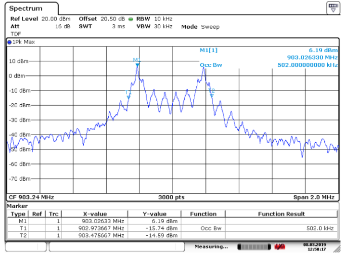
Figure 8.6-4: %99 occupied bandwidth on low channel
