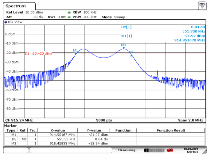
Figure 8.6-2: 6 dB bandwidth on mid channel
