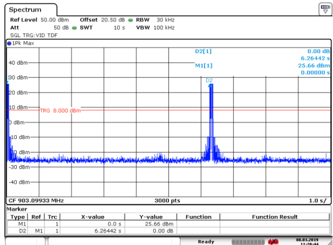
Figure 8.4-10: Dwell time, 10 s
