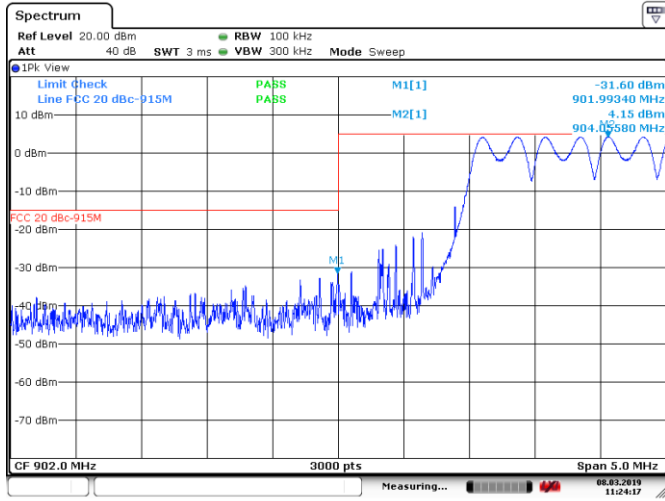
Figure 8.8-5: Conducted spurious emission at lower band edge, Hopping mode
