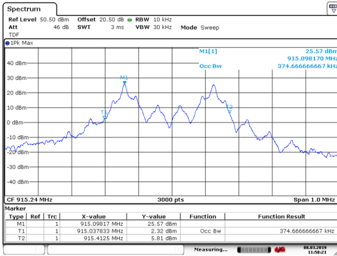
Figure 8.4-5: %99 occupied bandwidth on mid channel
