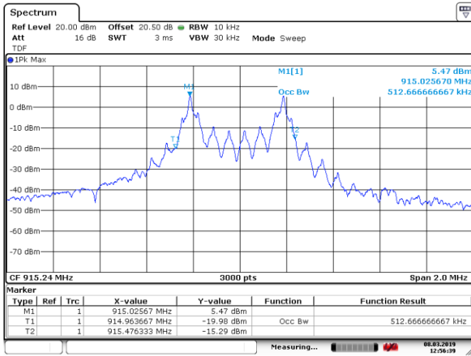
Figure 8.6-5: %99 occupied bandwidth on mid channel
