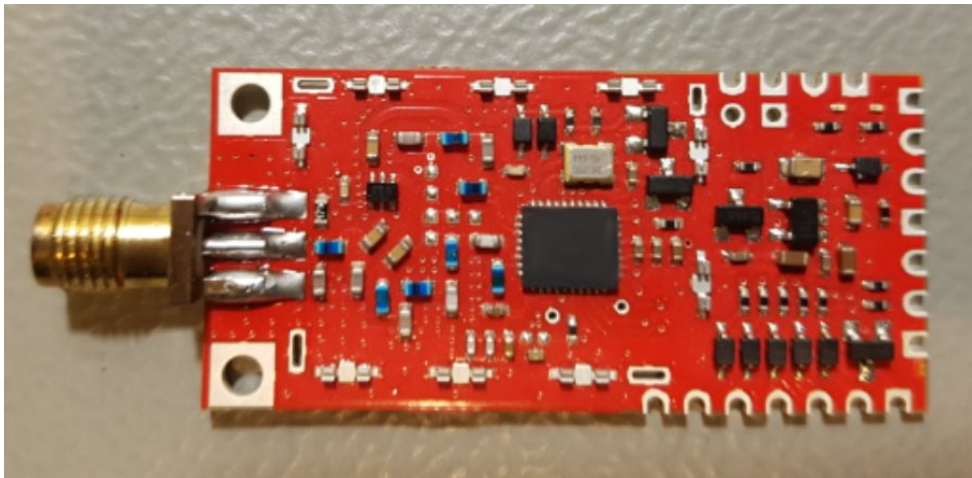
Front View (RF-Shield removed)
