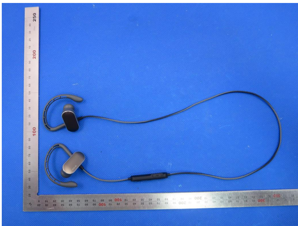
BTS-2X(Midnight) TOP VIEW OF EUT
