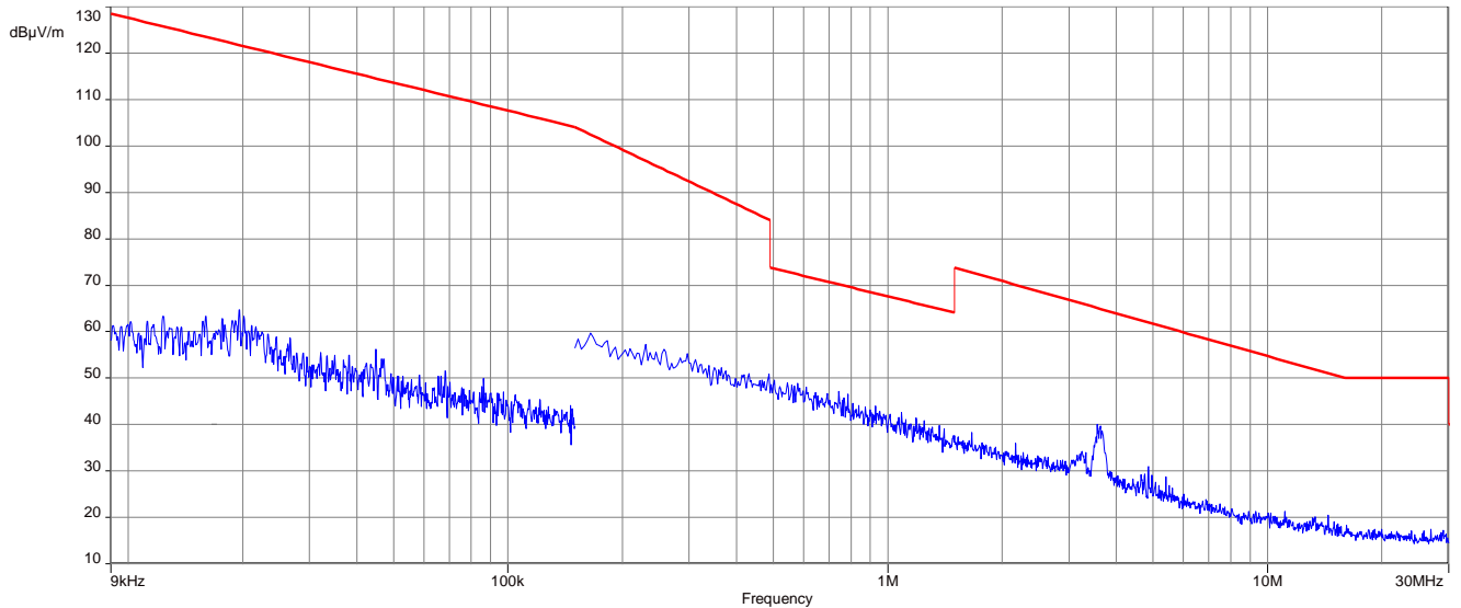
Plot 5: 9 kHz to 30 MHz, 2440 MHz, transmit mode, 2 Msps
