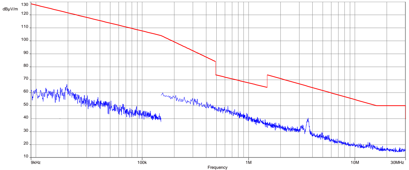
Plot 3: 9 kHz to 30 MHz, 2480 MHz, transmit mode, 1 Msps
