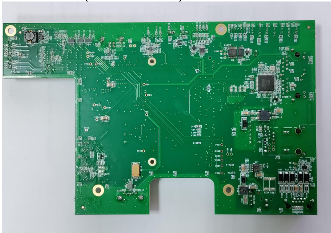
Photograph No.4 DDU (Dedicate Radio Console) PCB second side view
