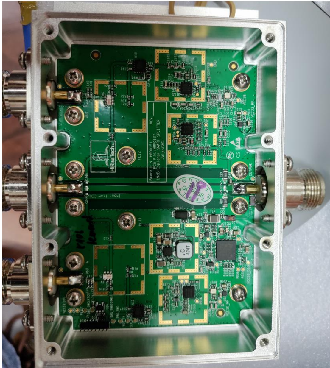
Photograph No.8 18dB Smart splitter top view
