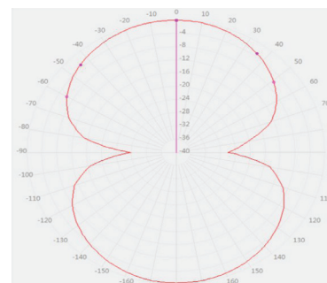
E Plane
