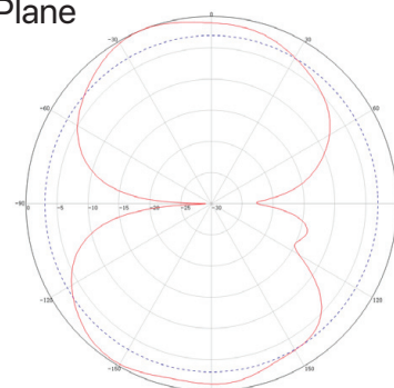
E Plane
