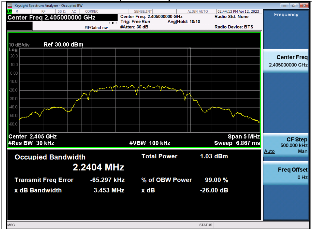
Test_Graph_2.4G_ANT1_2405_2Mbps_OBW
