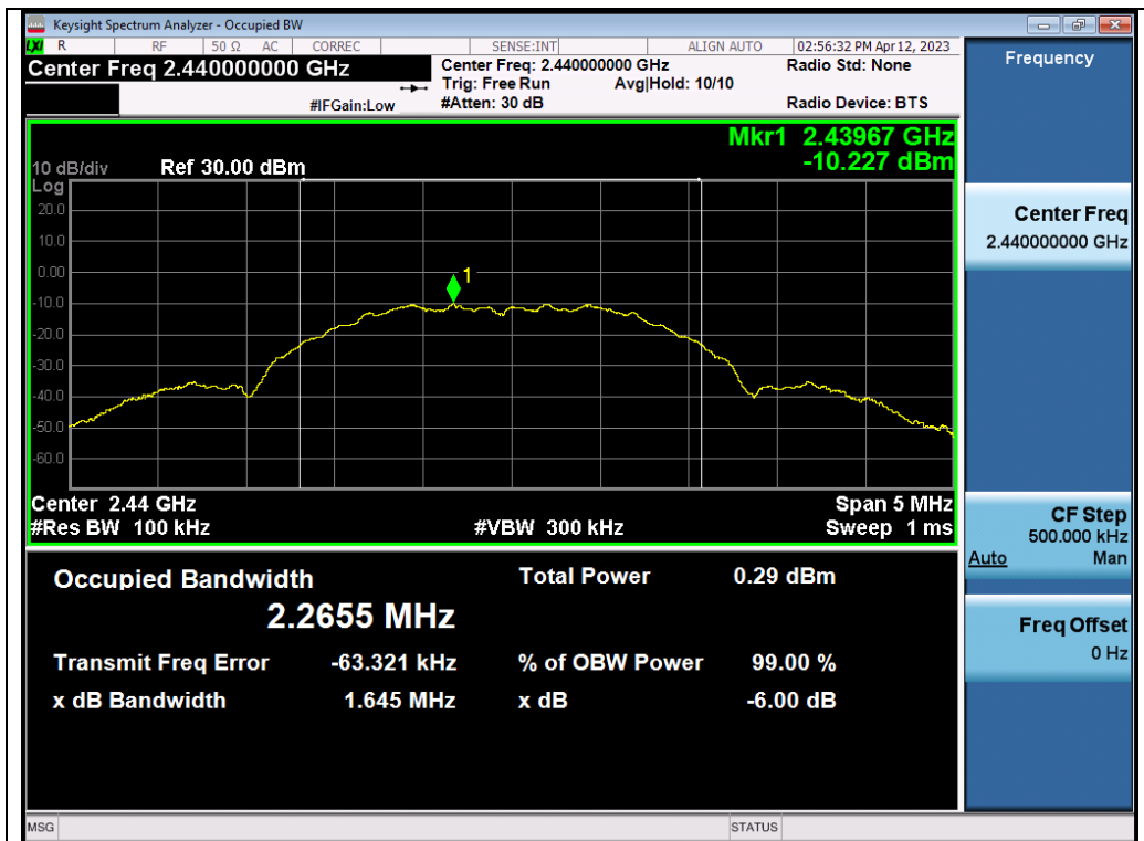
Test_Graph_2.4G_ANT1_2440_2Mbps_DTSBW
