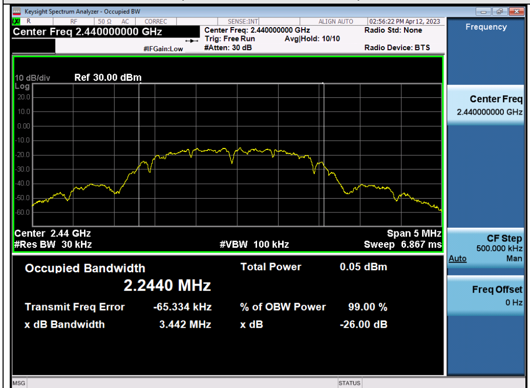
Test_Graph_2.4G_ANT1_2440_2Mbps_OBW
