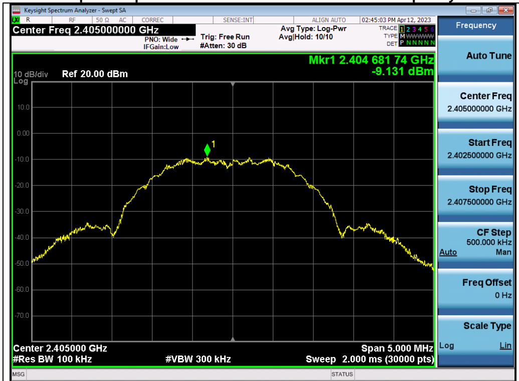
Test_Graph_2.4G_ANT1_2405_2Mbps_Reference Level
