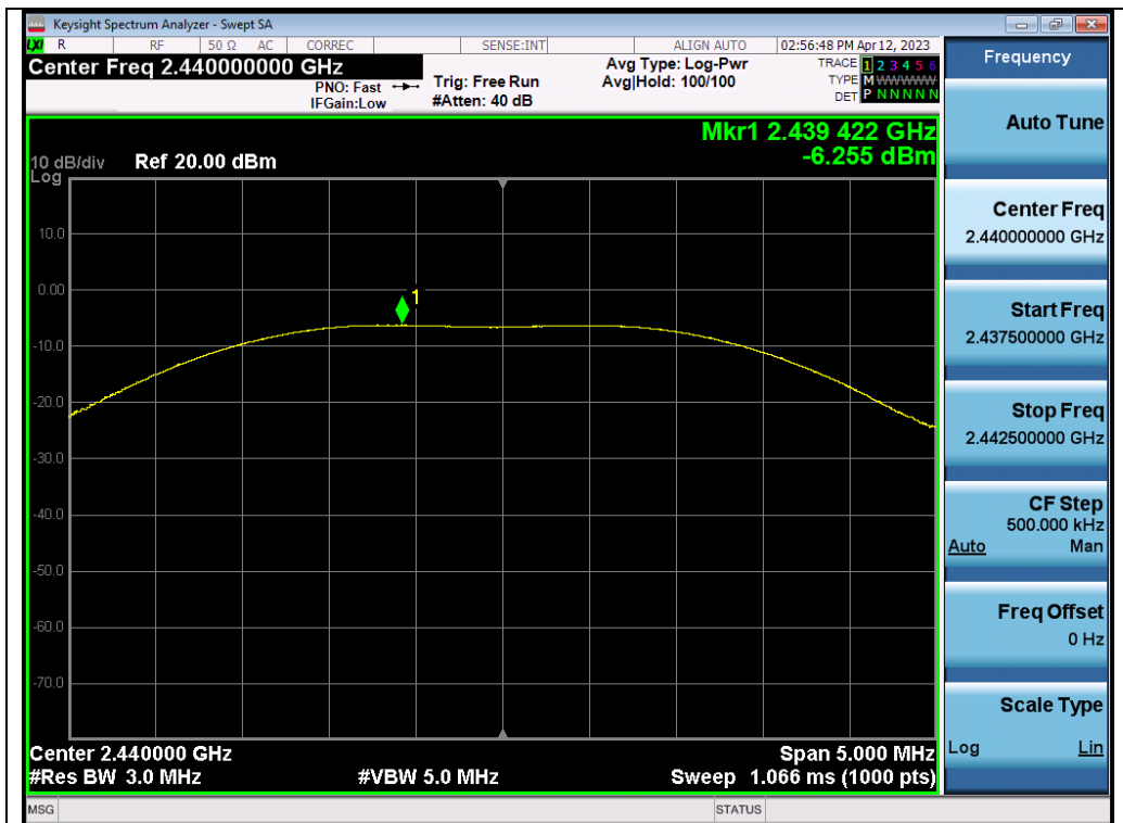
Test_Graph_2.4G_ANT1_2440_2Mbps_Peak Power
